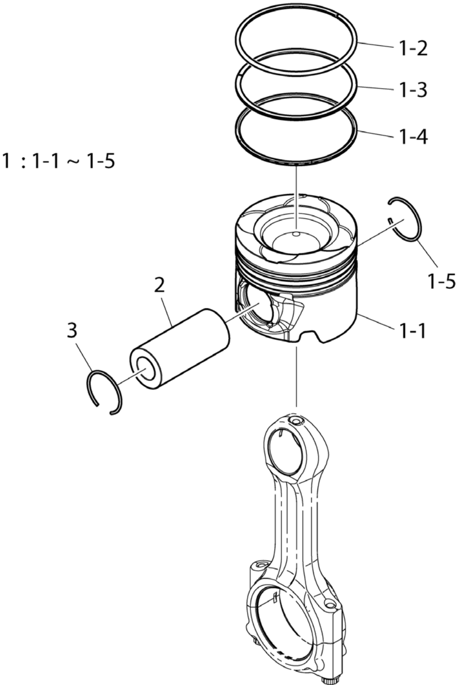
CONNECTING ROD
