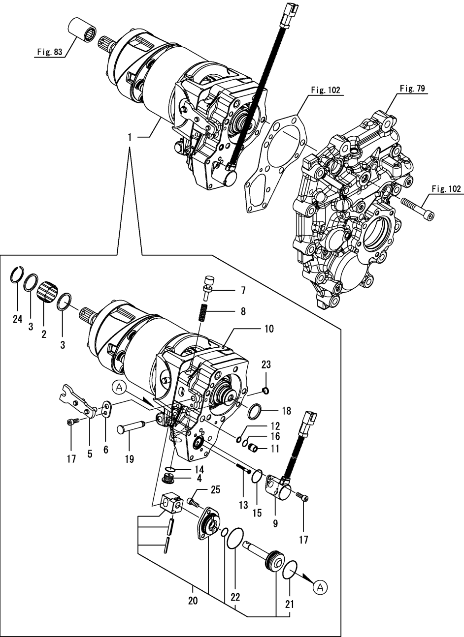
Fig.101. I-H.M.T.
