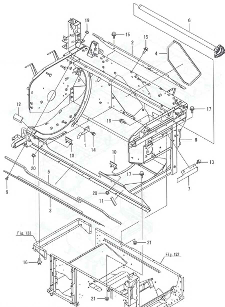
QCNP6-M03670 탈곡(1) Fig.135. 상부본체
