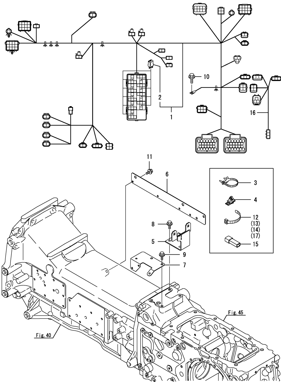
Fig.122. 배선(B)
