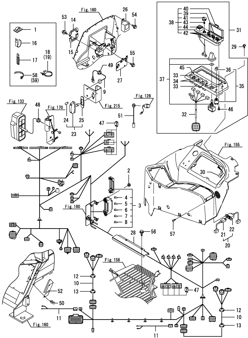
Fig.124. 배선(F)(ROPS)
