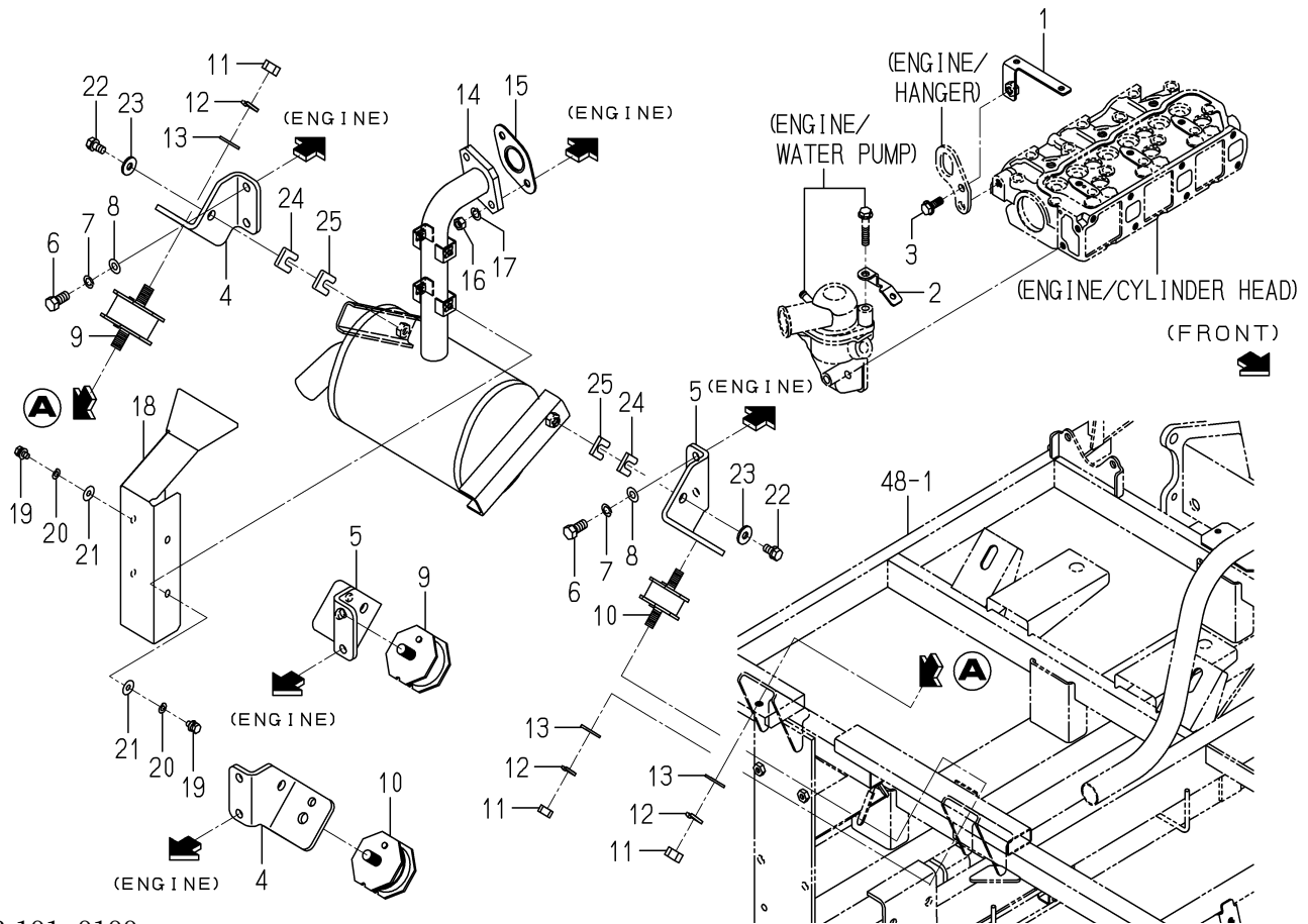
FIG. 2 GUIDE(HARNESS/ENGINE)SYSTEM(D TYPE)
