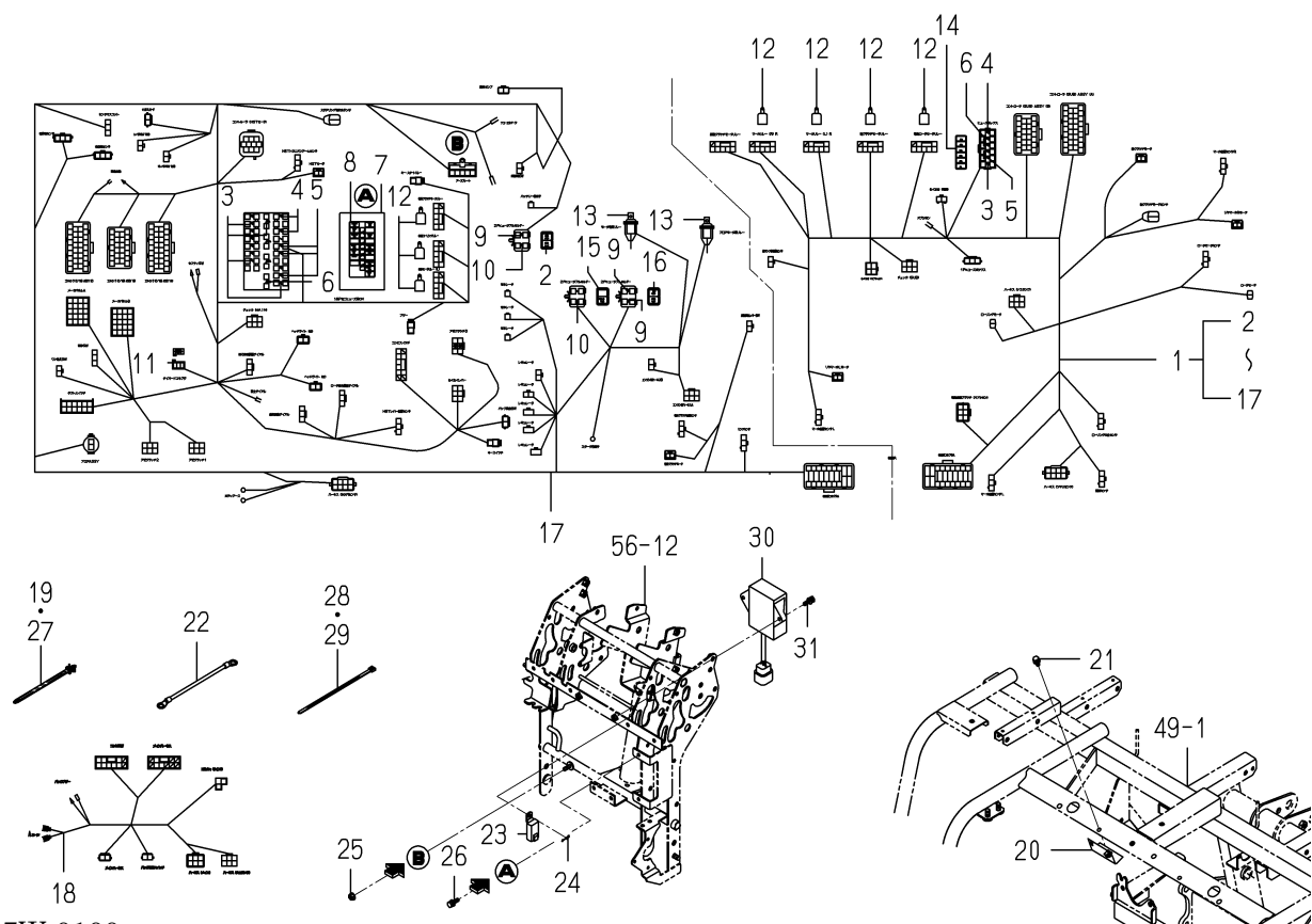
FIG. 92 HARNESS (TRAVELING SECTION)SYSTEM(G TYPE)
