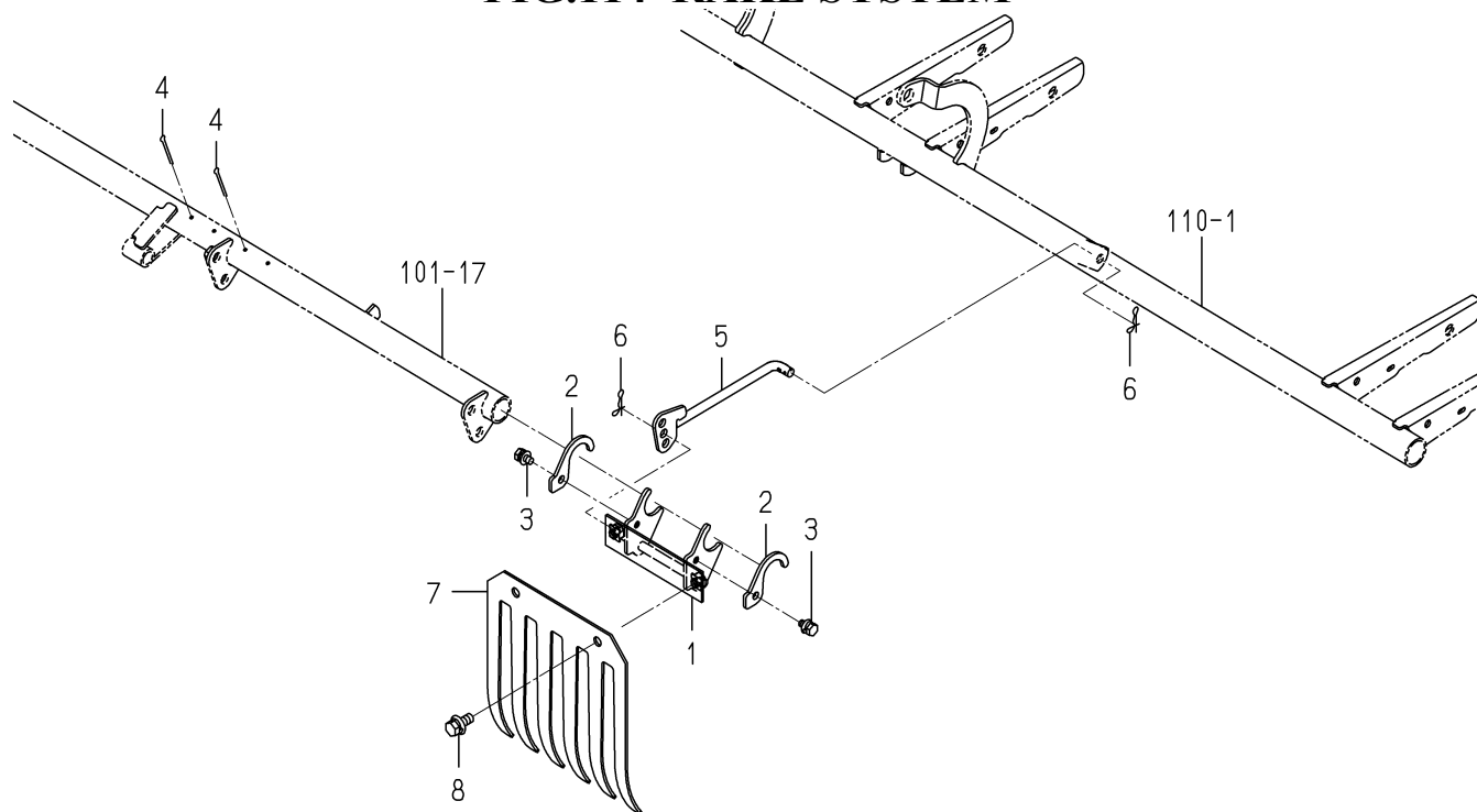
FIG.114 RAKE SYSTEM
