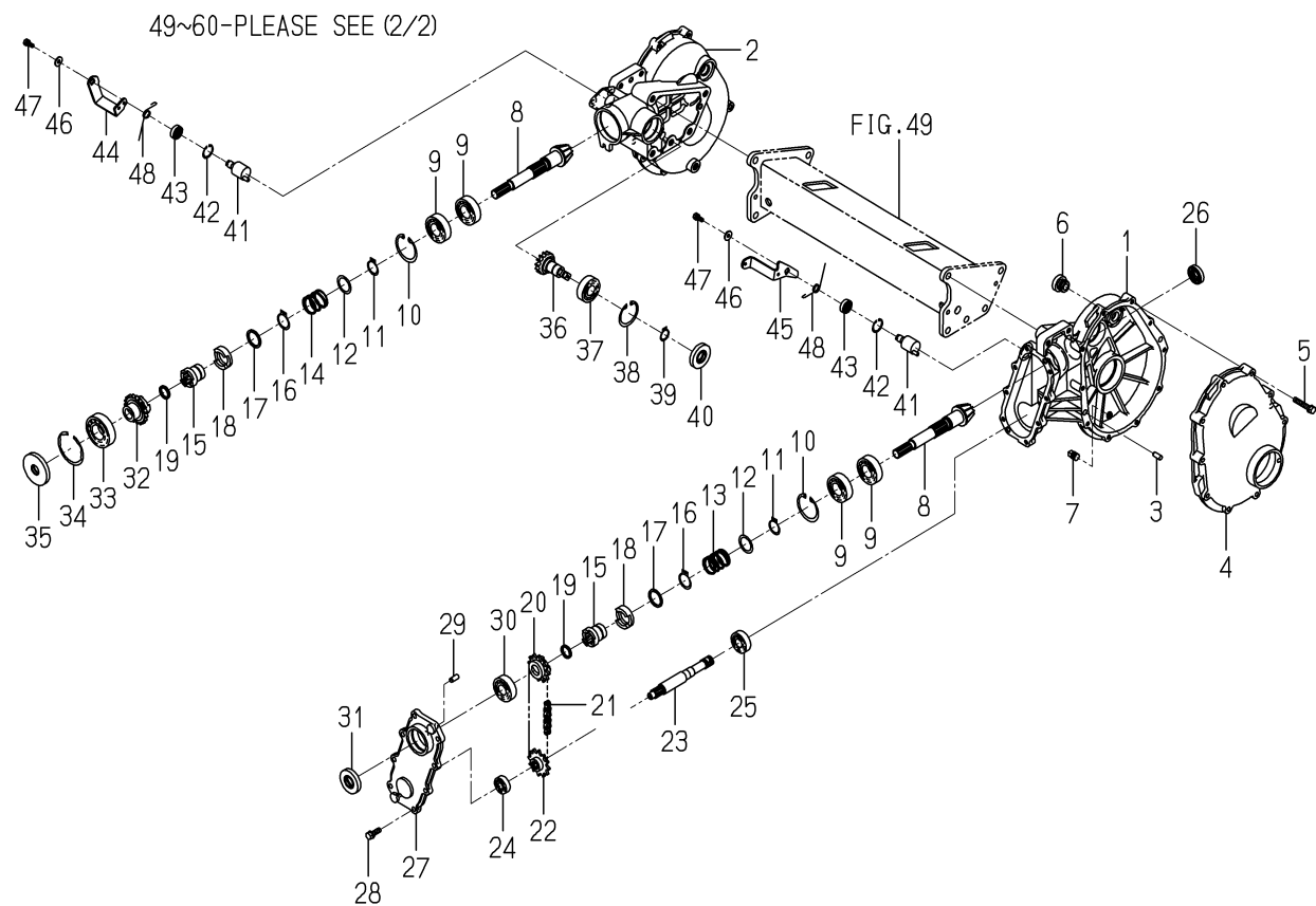
FIG. 54 CASE(REAR)SYSTEM(G TYPE)(1/2)
