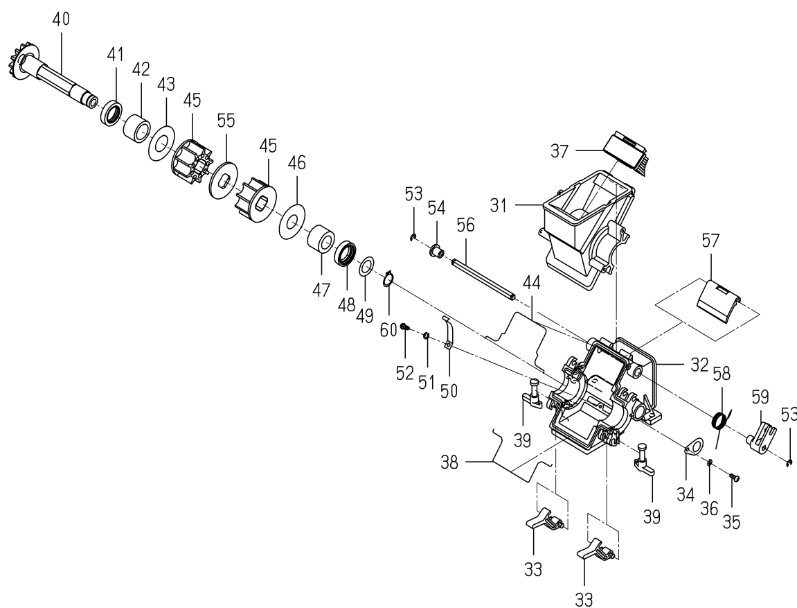
FIG.120 SEND OUT(FERTILIZER)SYSTEM(2/3)
