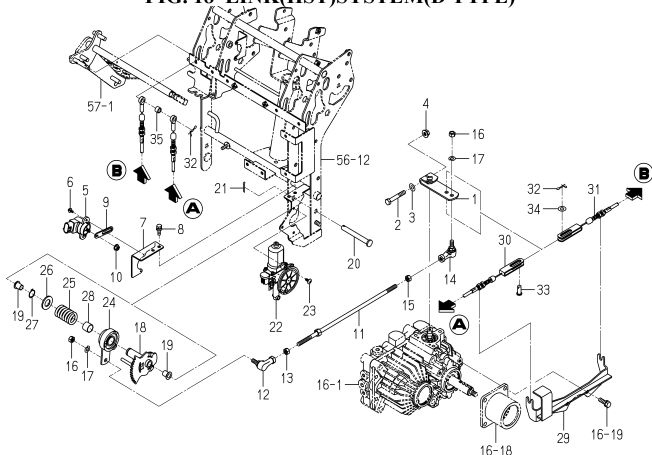
FIG. 18 LINK(HST)SYSTEM(D TYPE)
