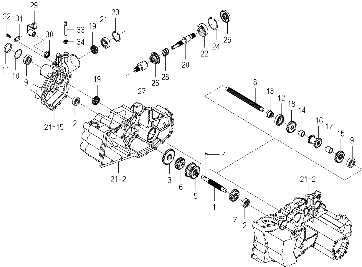
FIG. 34 SHAFT(PLANTING/OUT)SYSTEM(D TYPE)
