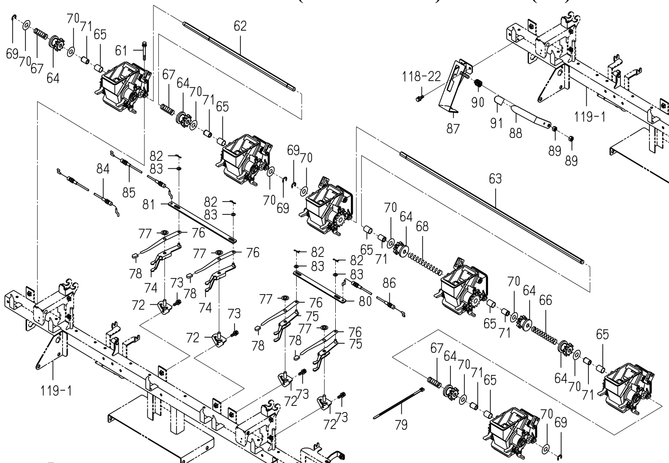
FIG.120 SEND OUT(FERTILIZER)SYSTEM(3/3)
