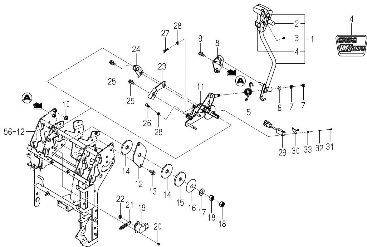
FIG. 12 LEVER(HST)SYSTEM(G TYPE)
