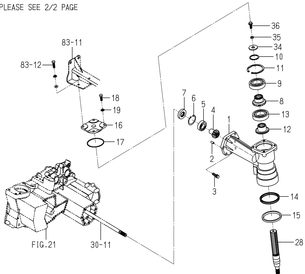
FIG. 44 CASE(FINAL)SYSTEM(D TYPE)(1/2)
