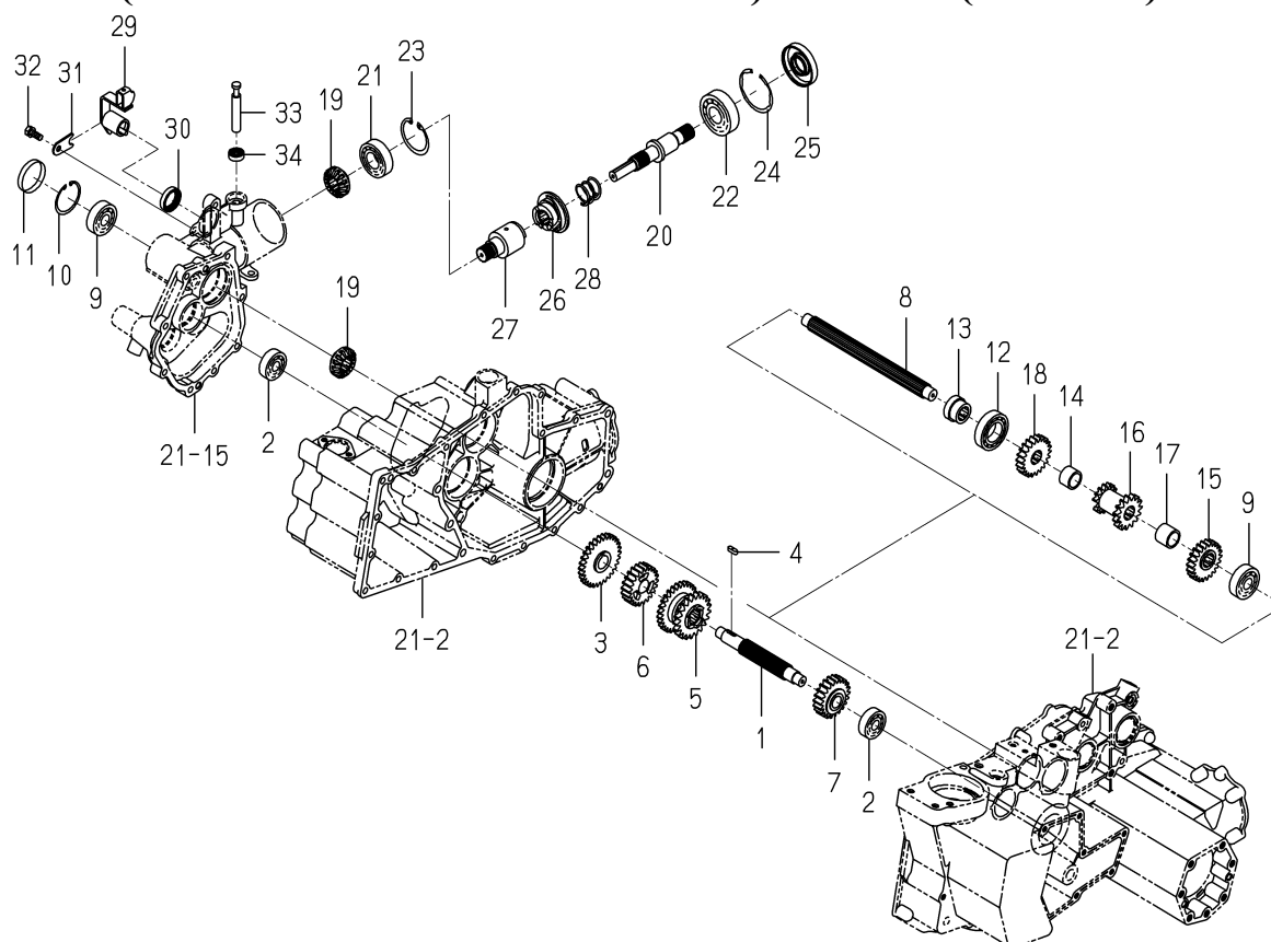
FIG. 33 SHAFT (PLANTING INTERVAL/OUT)SYSTEM(G TYPE)
