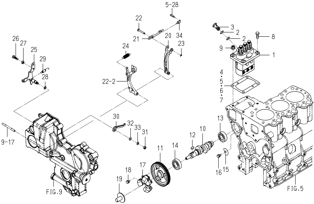
FIG. 20 INJECTION PUMP
