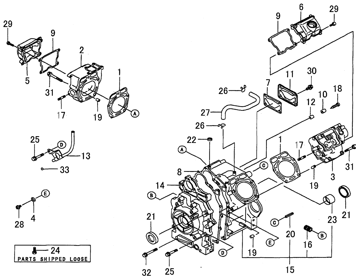
FIG. 1 CYLINDER/CRANKCASE
