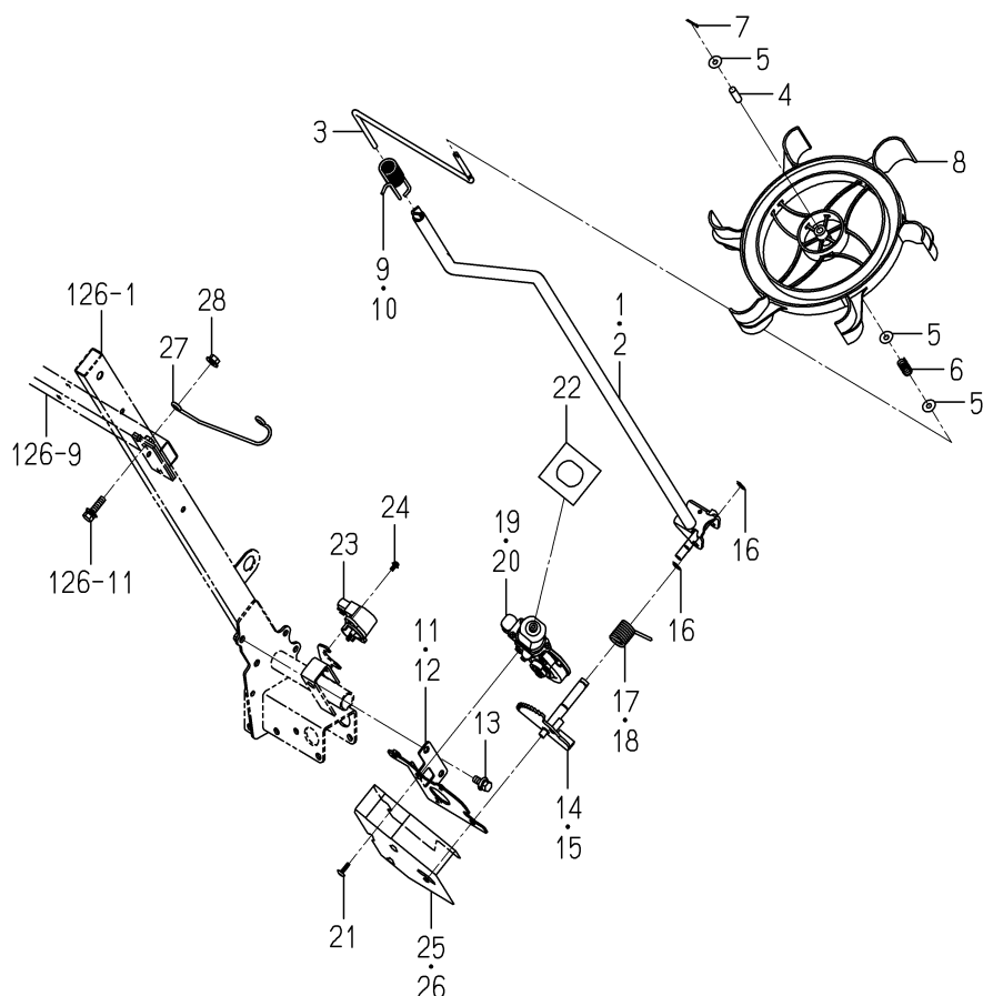
FIG.129 MARKER SYSTEM
