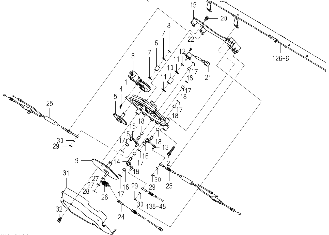
FIG. 98 CLUTCH(PLANTING)SYSTEM
