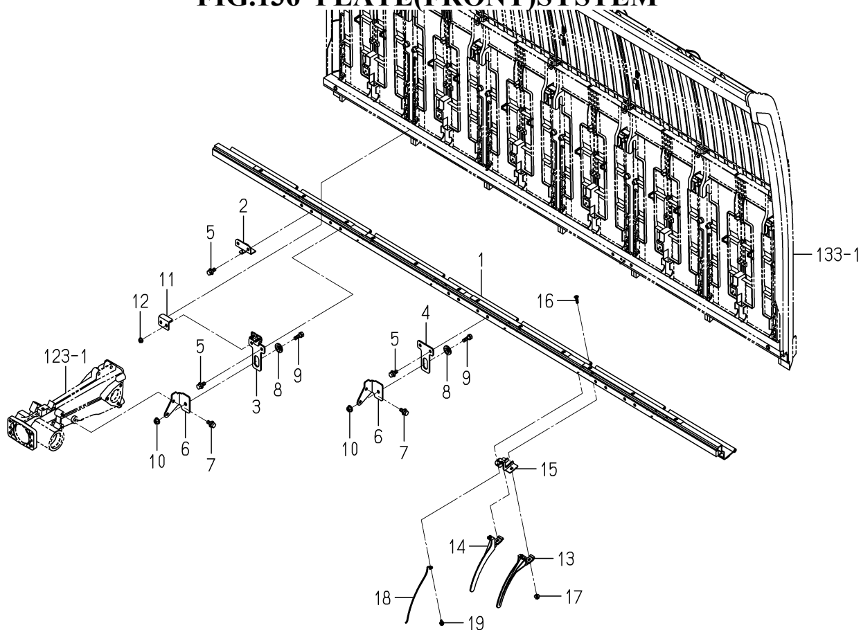
FIG.136 PLATE(FRONT)SYSTEM
