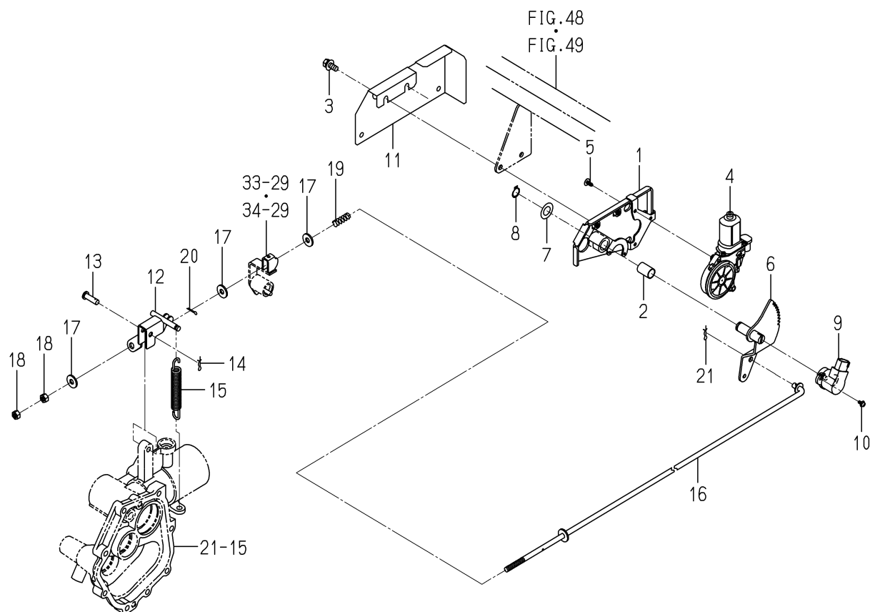
FIG. 69 CLUTCH(PLANTING)SYSTEM
