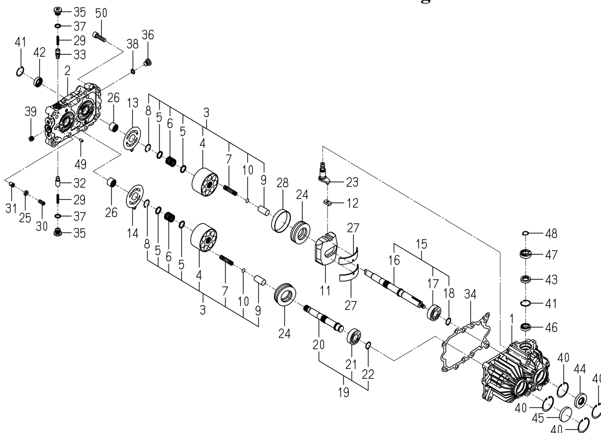
FIG.150 COMPONENT PARTS FOR K510-021-000-20 ON Fig.15
