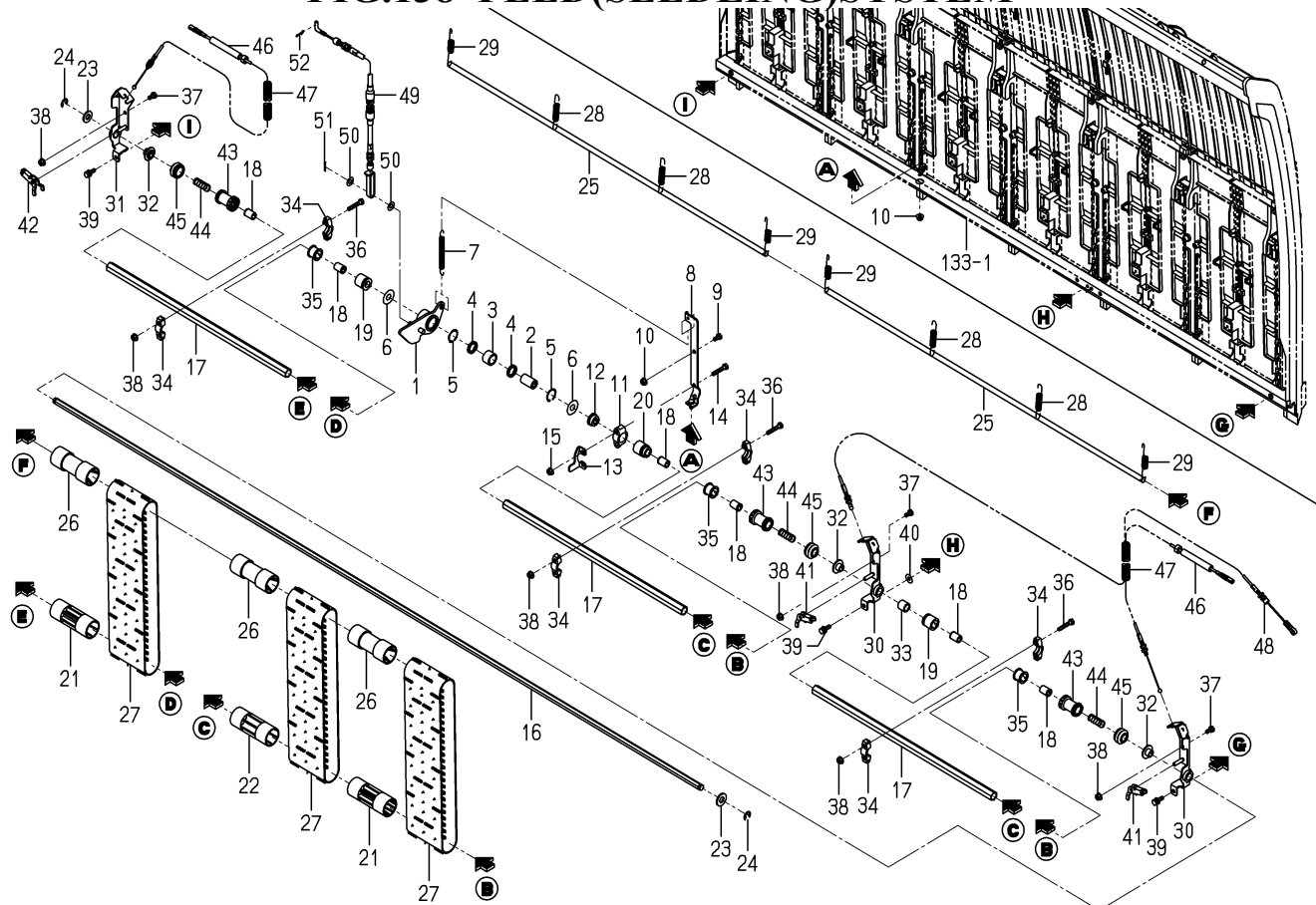
FIG.138 FEED(SEEDLING)SYSTEM
