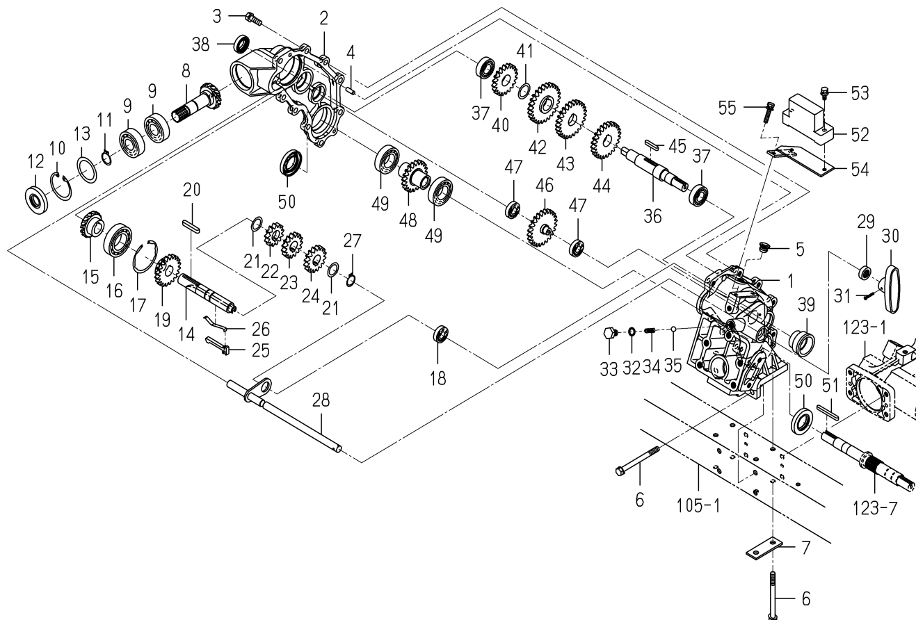
FIG.107 LINK(FLOAT)SYSTEM
