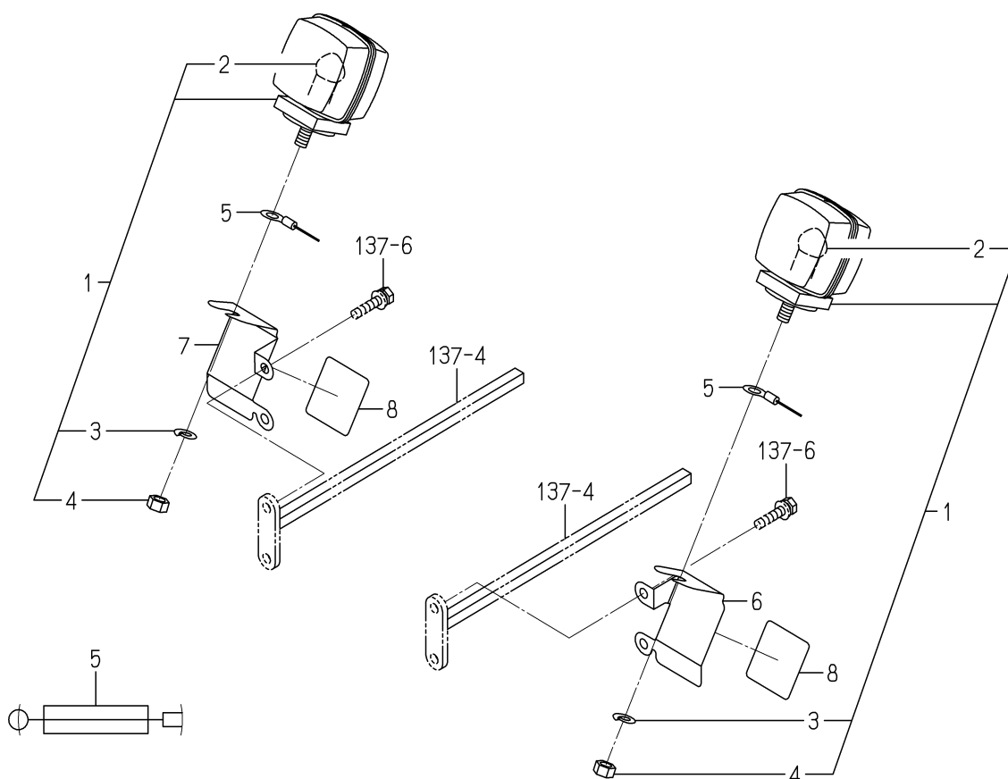
FIG.135 WINKER SYSTEM
