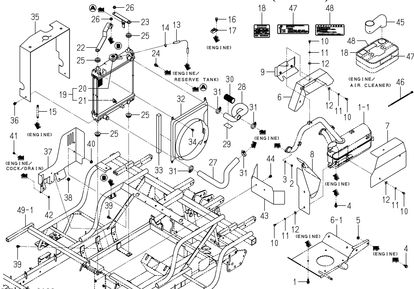
FIG. 3 RADIATOR SYSTEM(G TYPE)
