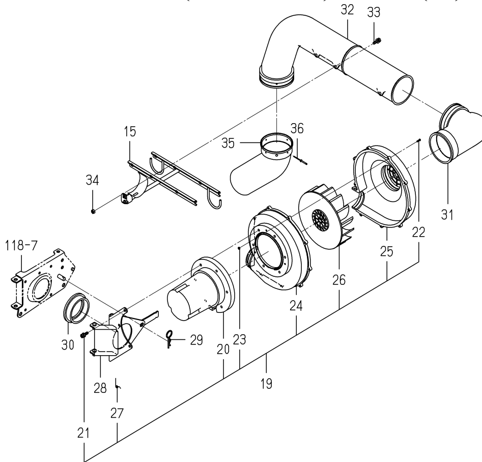
FIG.119 FRAME(FERTILIZER)SYSTEM(2/2)
