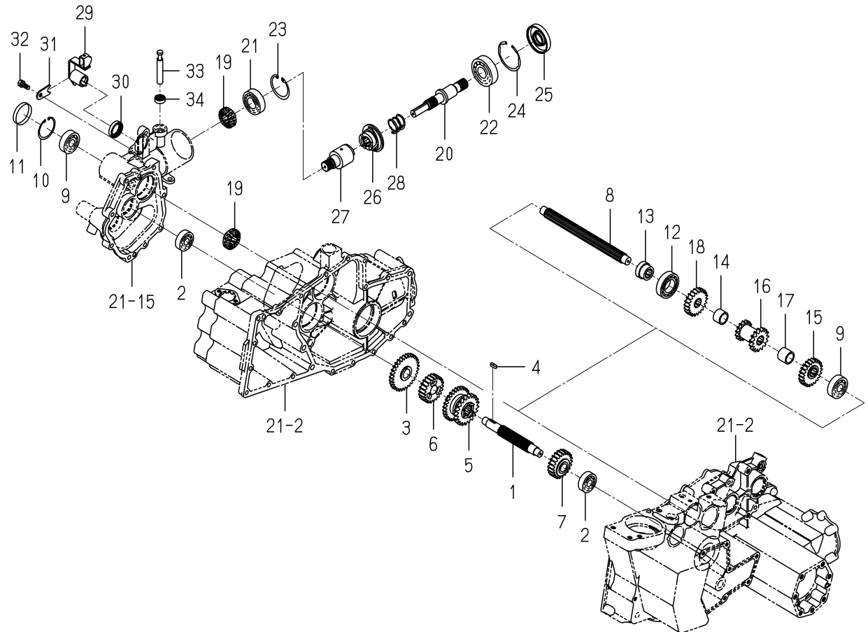
FIG. 34 SHAFT(PLANTING/OUT)SYSTEM(D TYPE)
