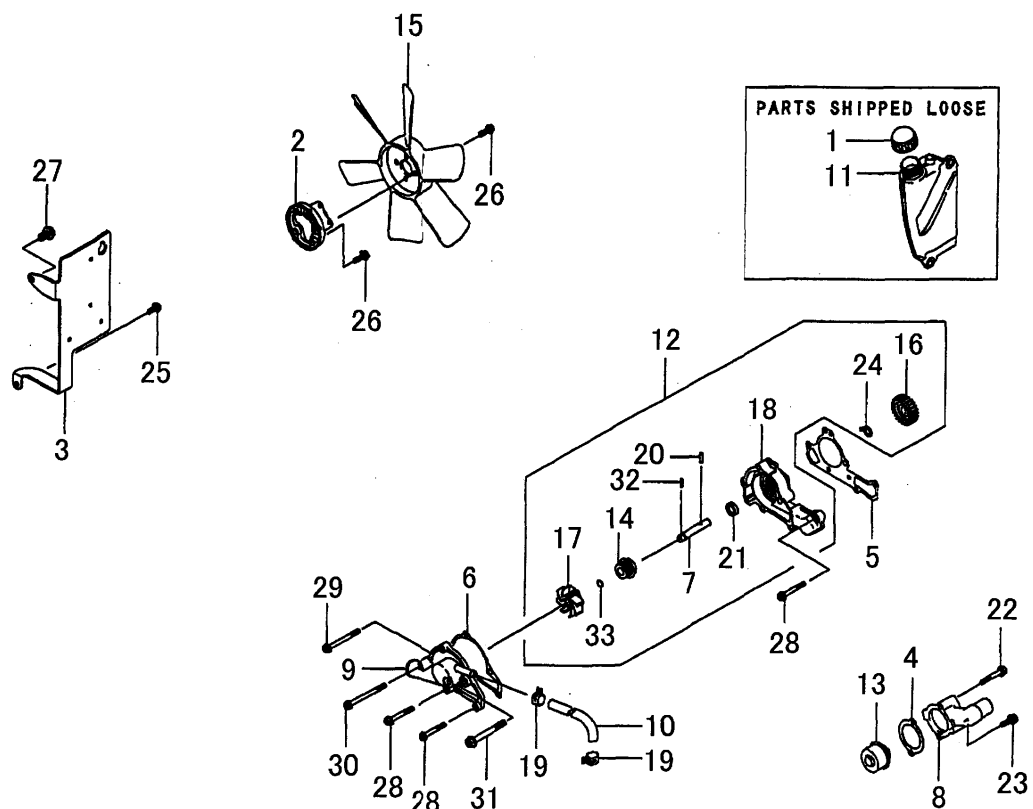
FIG. 5 COOLING-EQUIPMENT
