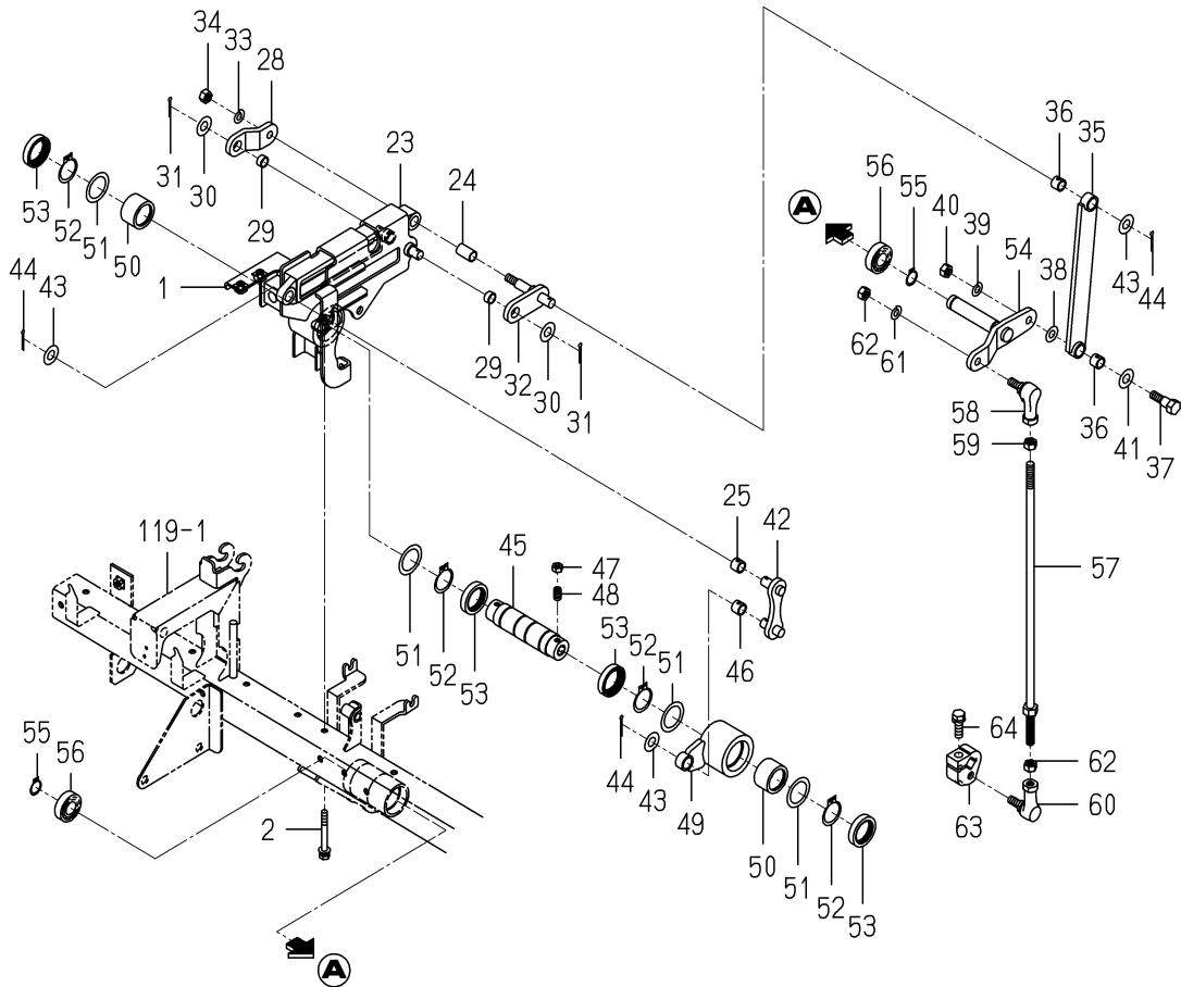
FIG.116 DRIVE(FERTILIZER)SYSTEM(D TYPE)(2/2)
