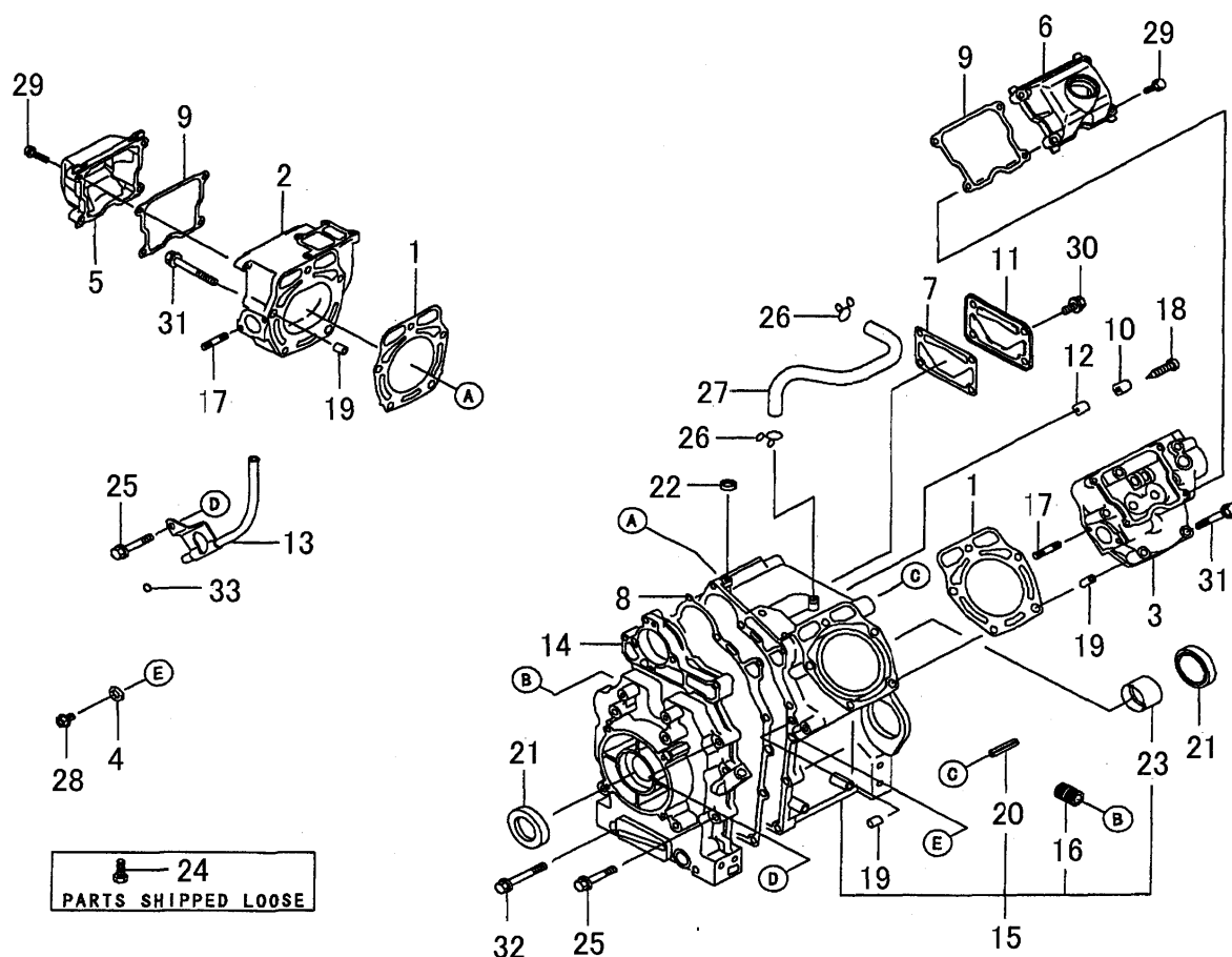
FIG. 1 CYLINDER/CRANKCASE
