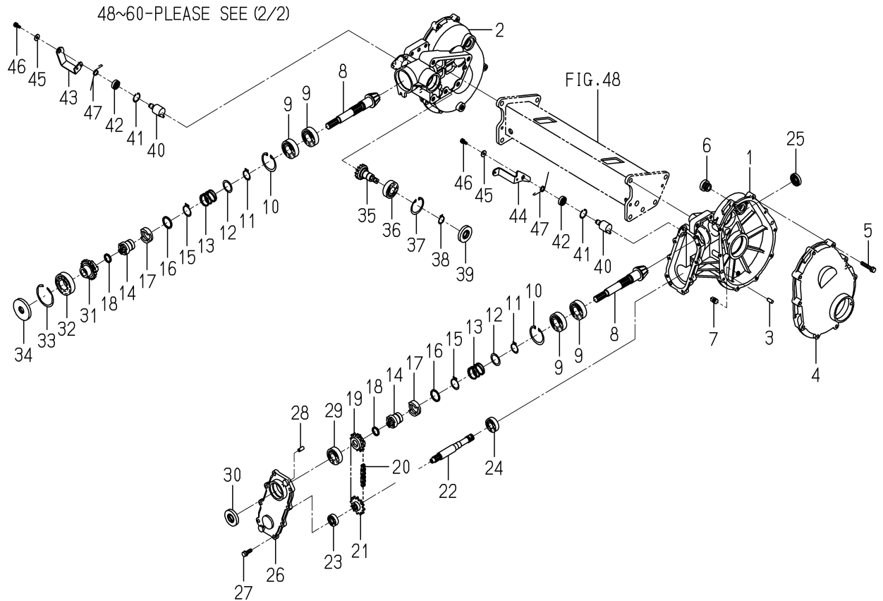
FIG. 55 CASE(REAR)SYSTEM(D TYPE)(1/2)
