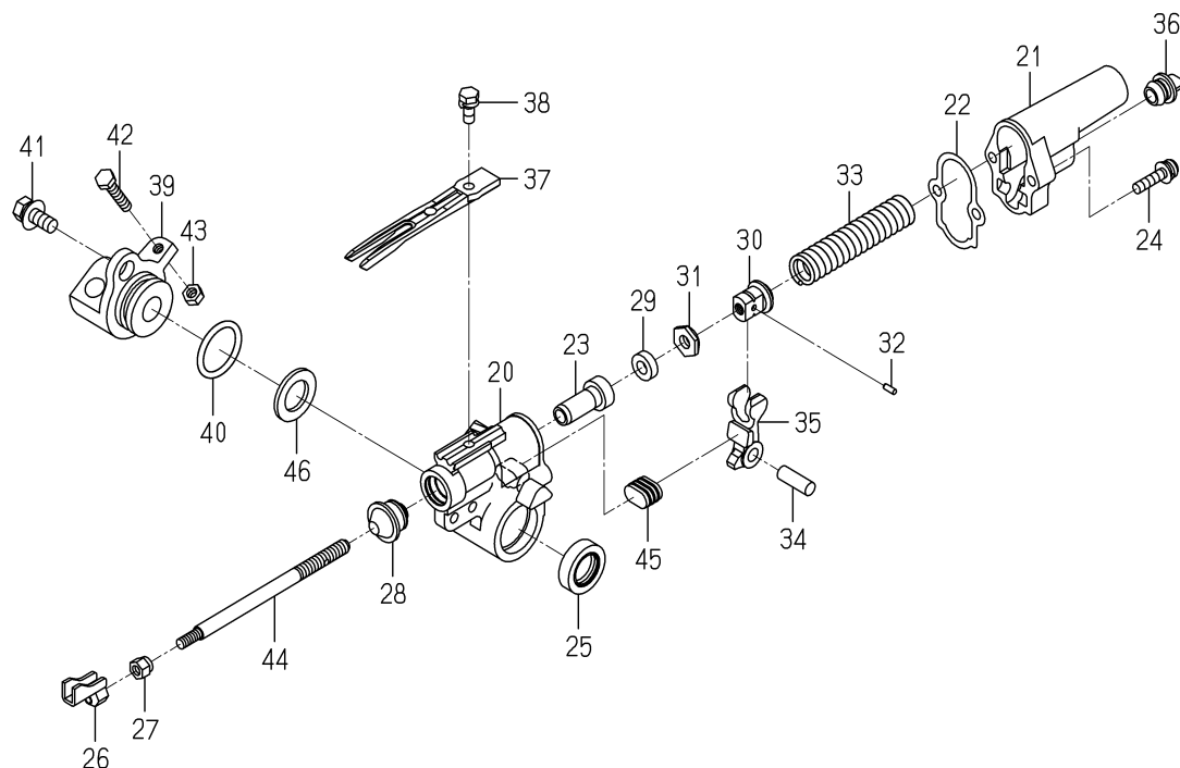
FIG.153 COMPONENT PARTS(2/2) FOR 2204-739-440-40 ON Fig.132
