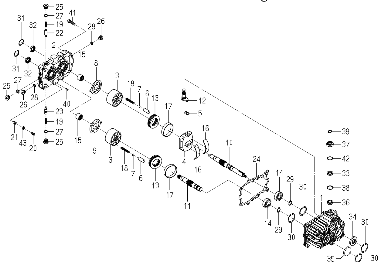
FIG.151 COMPONENT PARTS FOR K510-022-000-00 ON Fig.16
