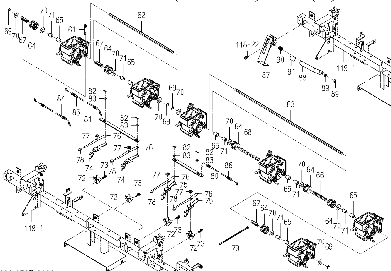
FIG.120 SEND OUT(FERTILIZER)SYSTEM(3/3)
