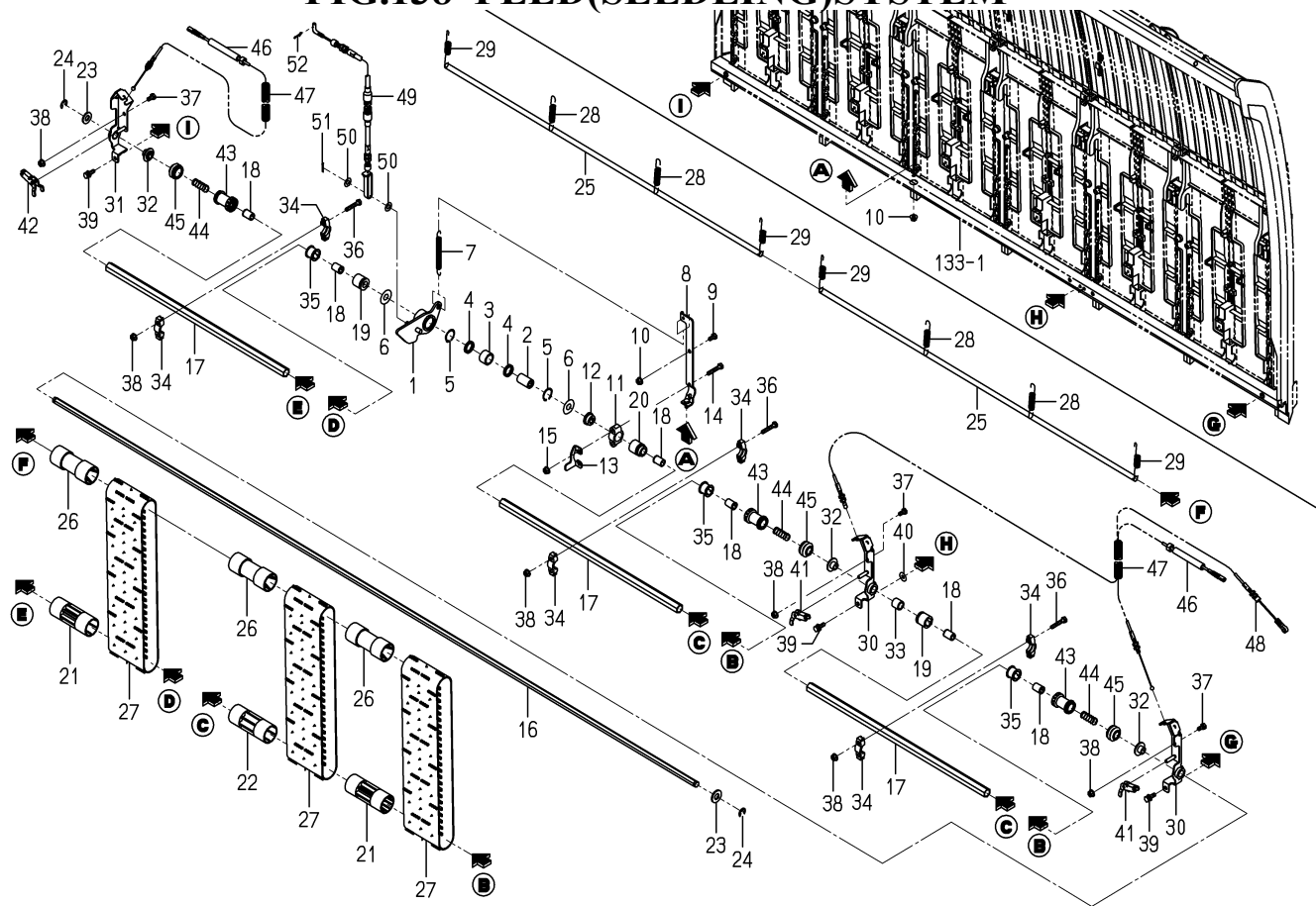
FIG.138 FEED(SEEDLING)SYSTEM
