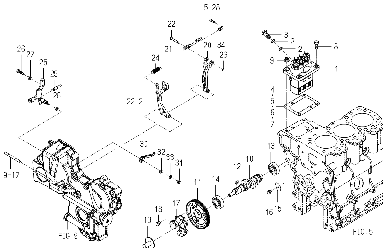
FIG. 20 INJECTION PUMP
