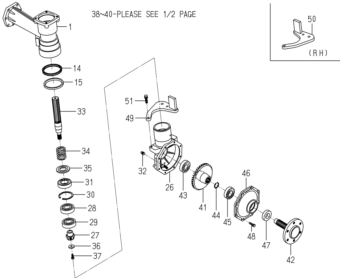
FIG. 43 CASE(FINAL)SYSTEM(G TYPE)(2/2)
