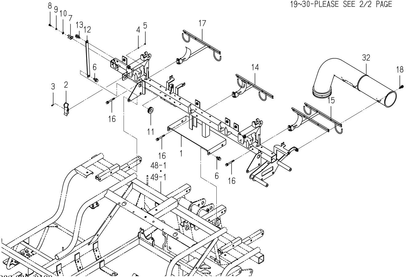
FIG.119 FRAME(FERTILIZER)SYSTEM(1/2)
