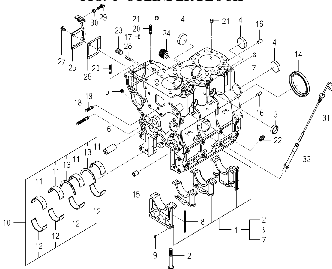
FIG. 5 CYLINDER BLOCK
