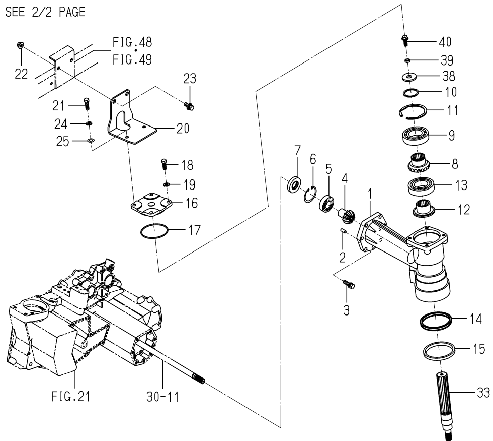
FIG. 43 CASE(FINAL)SYSTEM(G TYPE)(1/2)
