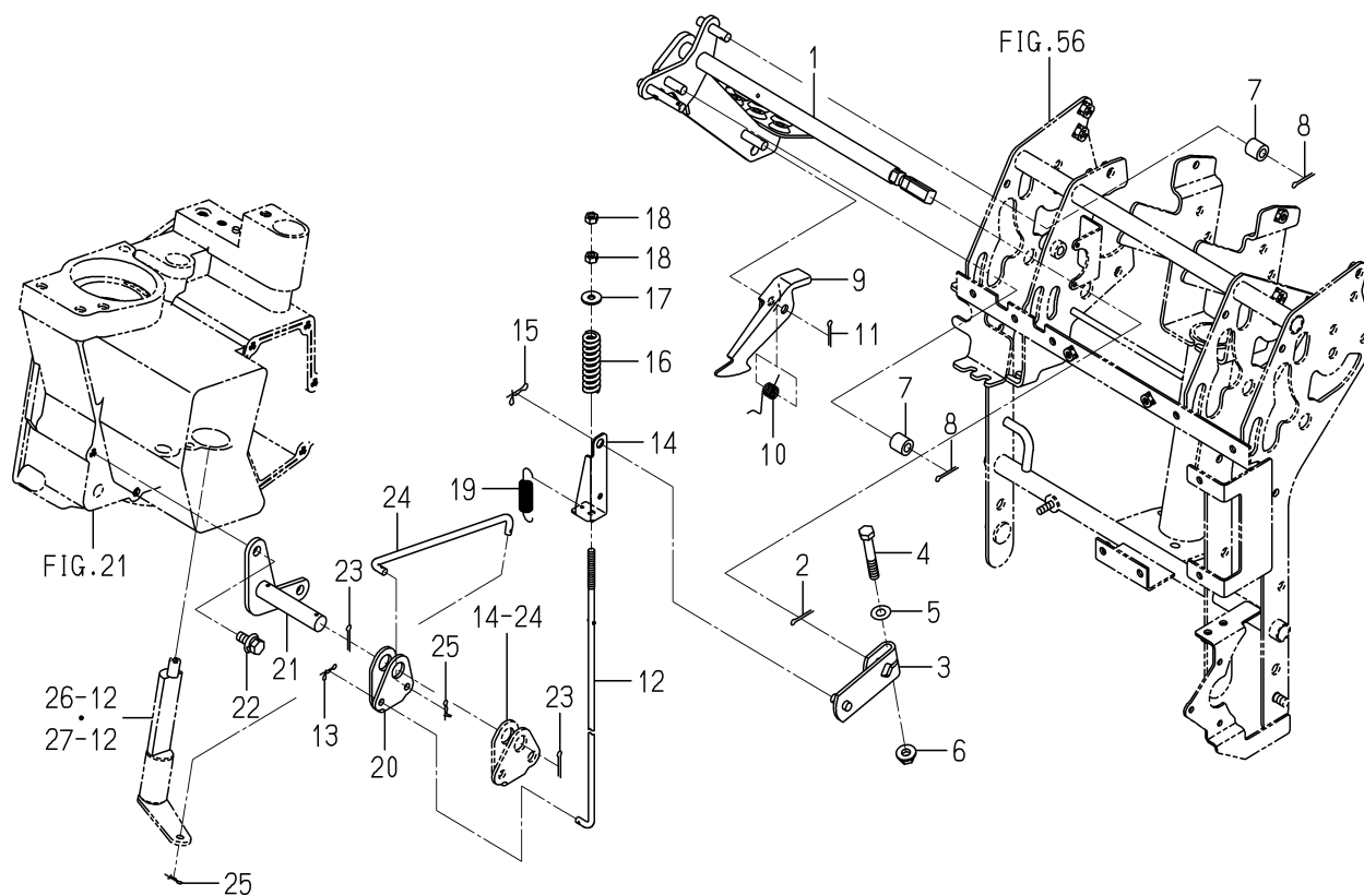
FIG. 57 PEDAL(BRAKE)SYSTEM
