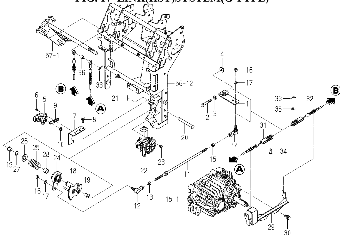
FIG. 17 LINK(HST)SYSTEM(G TYPE)
