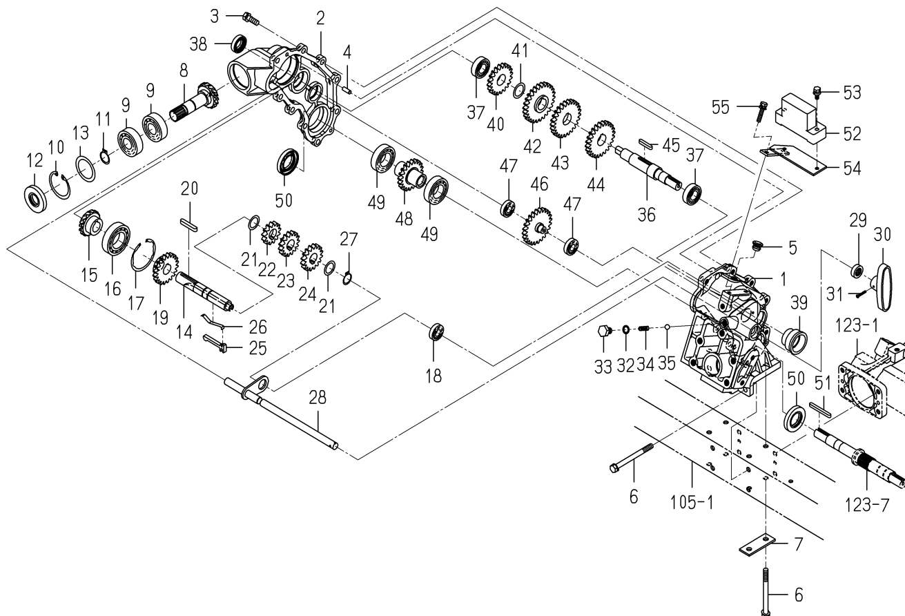
FIG.107 LINK(FLOAT)SYSTEM
