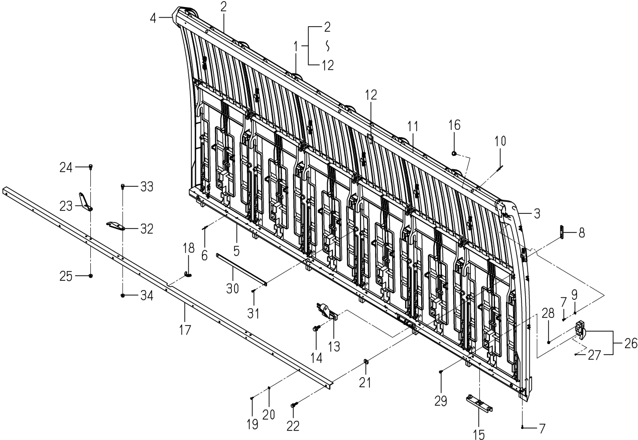
FIG.133 TANK(SEEDLING)SYSTEM
