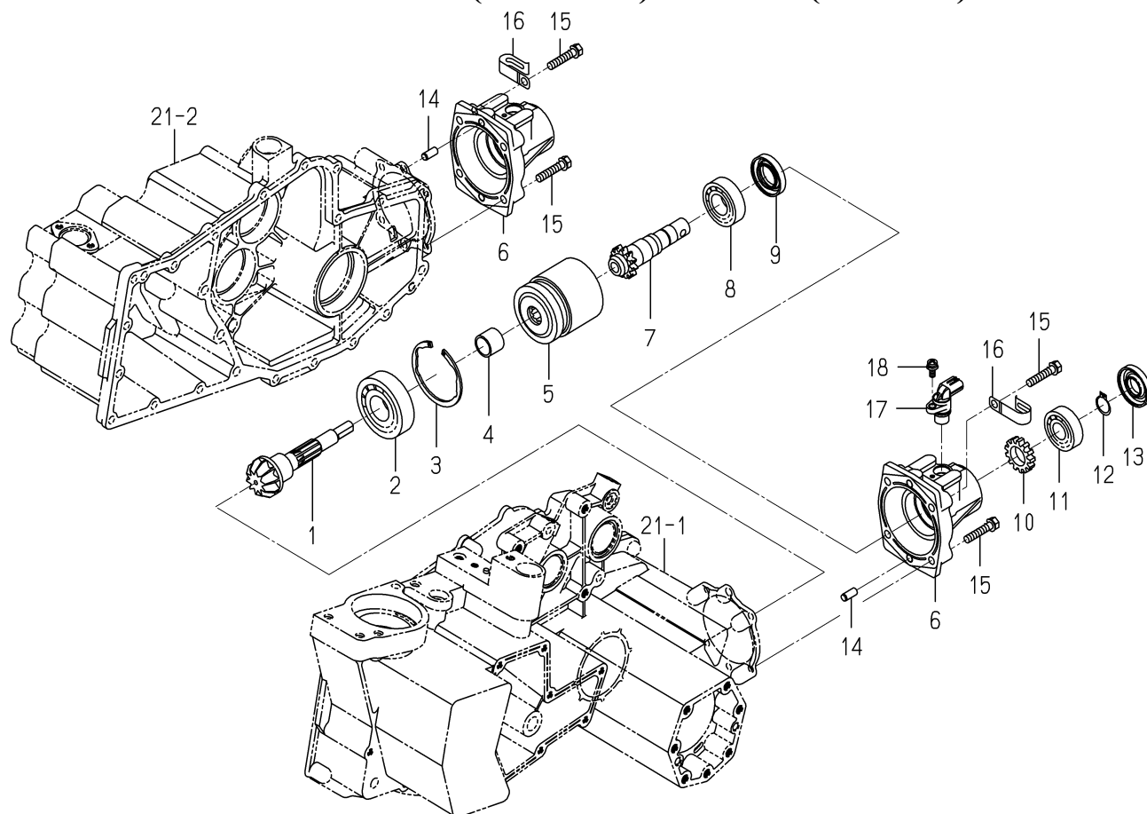
FIG. 29 SHAFT(OUTPUT)SYSTEM(D TYPE)
