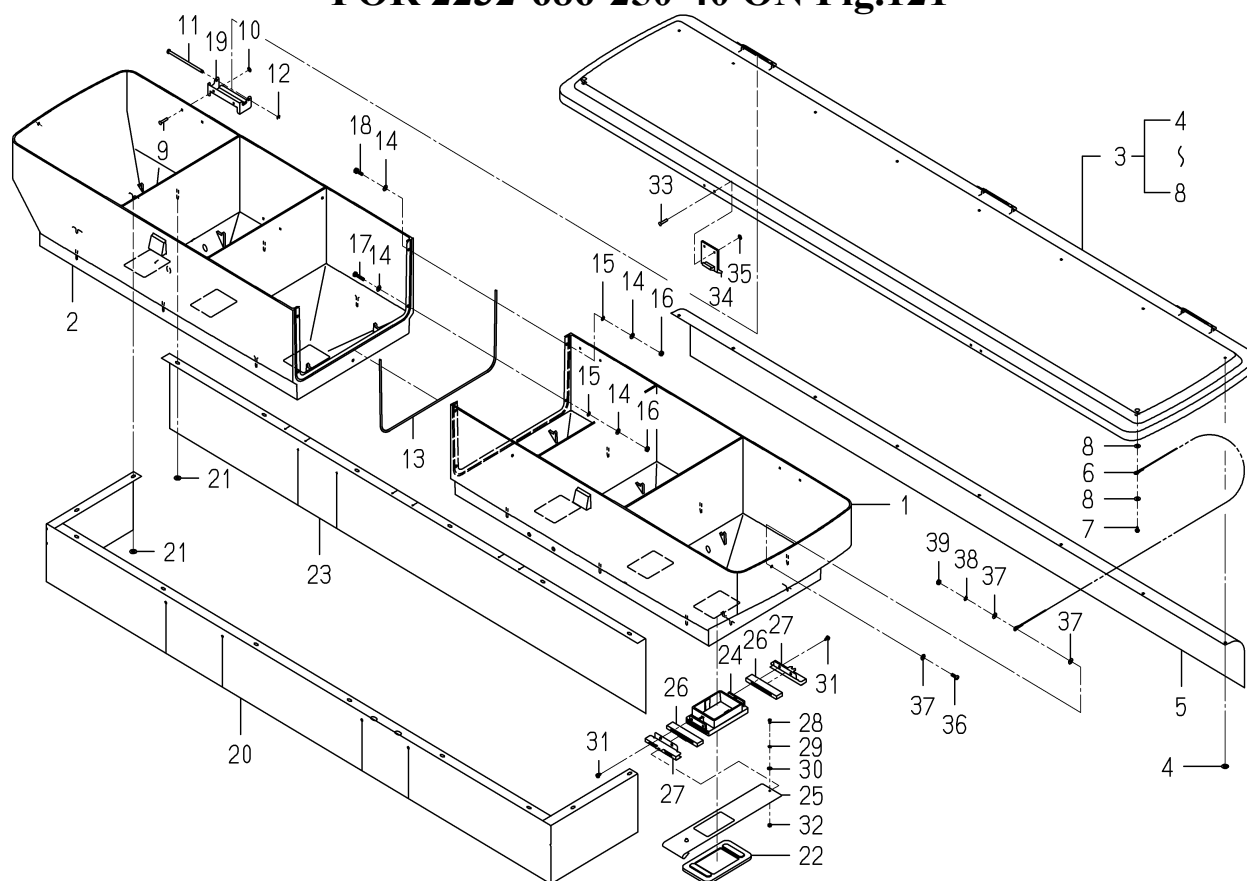
FIG.154 COMPONENT PARTS FOR 2232-686-250-40 ON Fig.121
