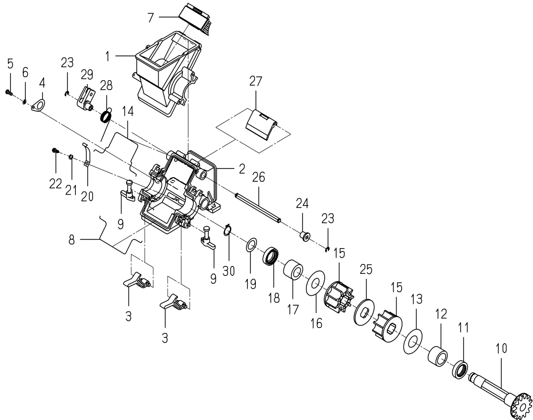
FIG.120 SEND OUT(FERTILIZER)SYSTEM(1/3)
