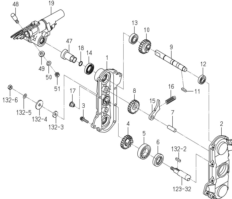
FIG.153 COMPONENT PARTS(1/2) FOR 2204-739-440-40 ON Fig.132
