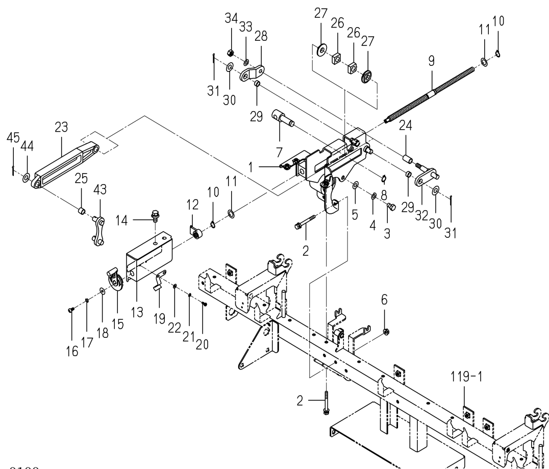
FIG.115 DRIVE(FERTILIZER)SYSTEM(G TYPE)(1/2)
