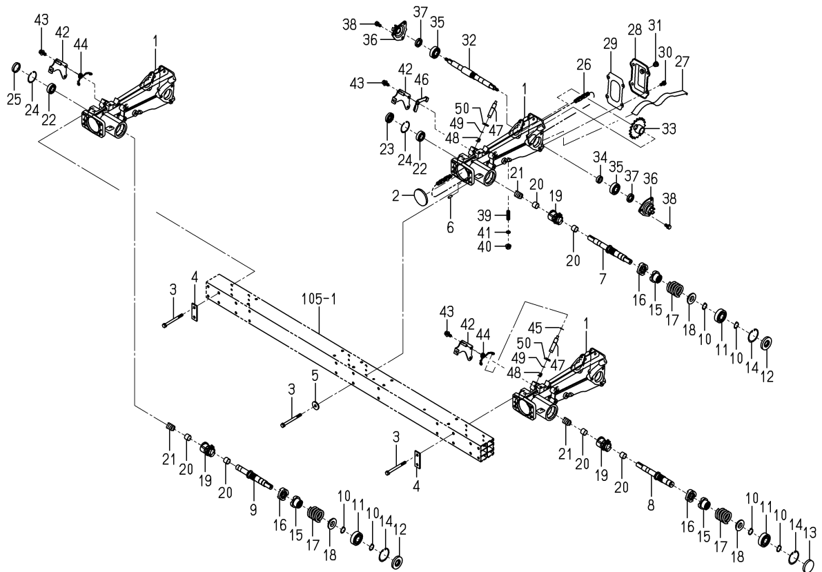
FIG.123 FRAME(SIDE)SYSTEM
