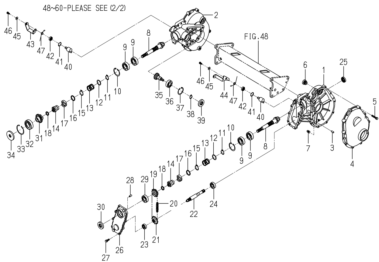
FIG. 55 CASE(REAR)SYSTEM(D TYPE)(1/2)
