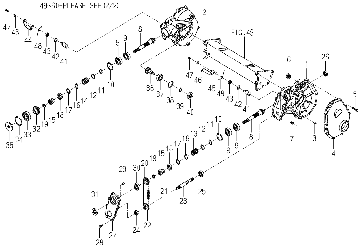
FIG. 54 CASE(REAR)SYSTEM(G TYPE)(1/2)
