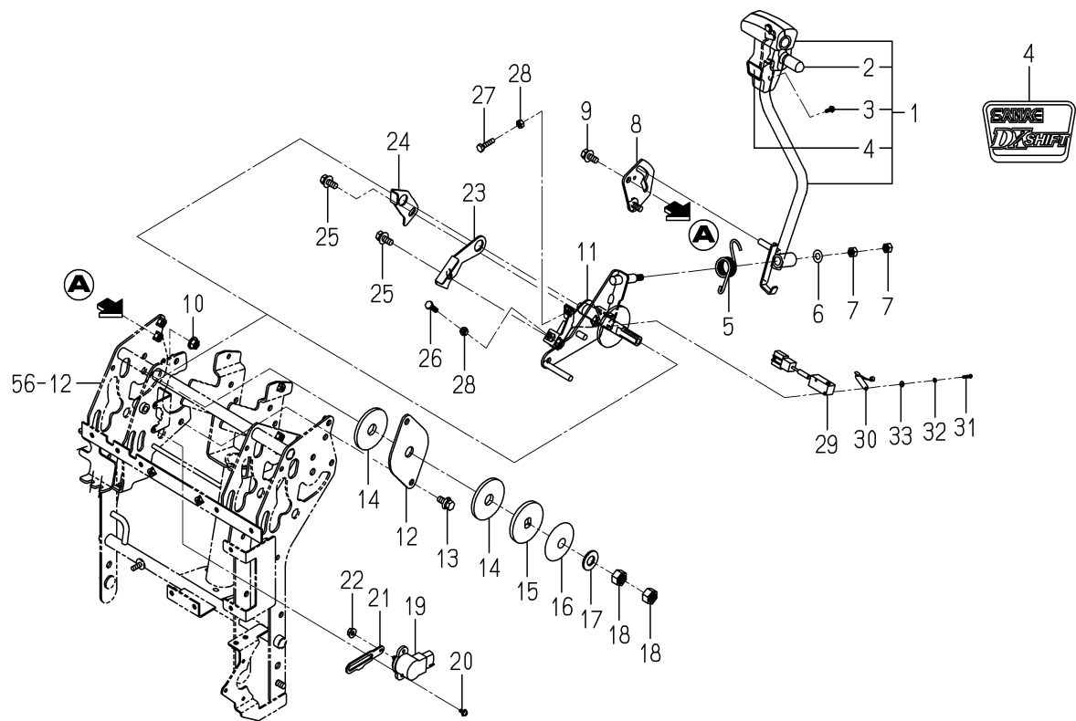
FIG. 13 LEVER(HST)SYSTEM(D TYPE)
