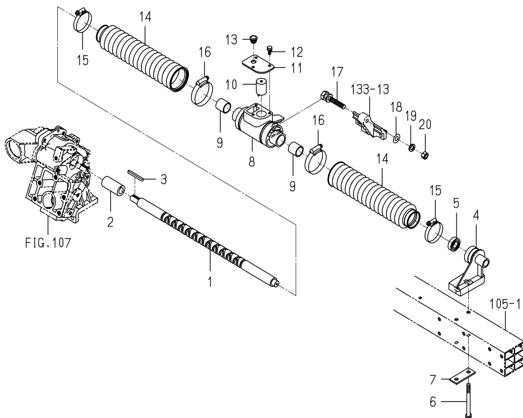
FIG.108 CAM(LEAD)SYSTEM
