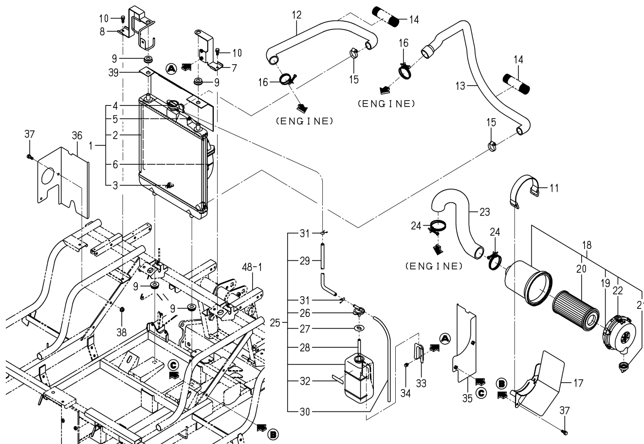
FIG. 4 RADIATOR SYSTEM(D TYPE)
