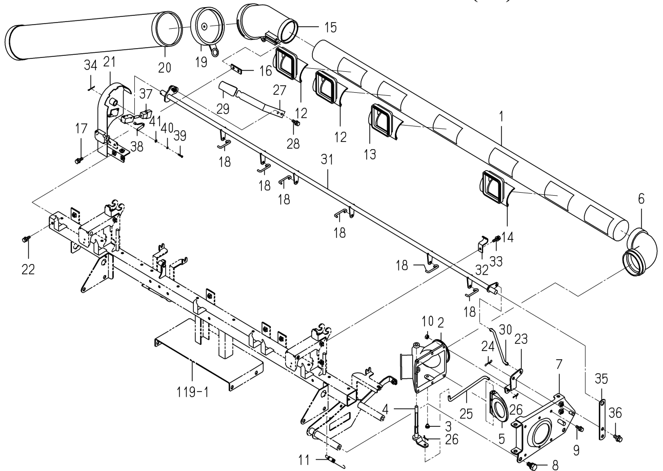
FIG.118 AIR CHAMBER SYSTEM(1/2)
