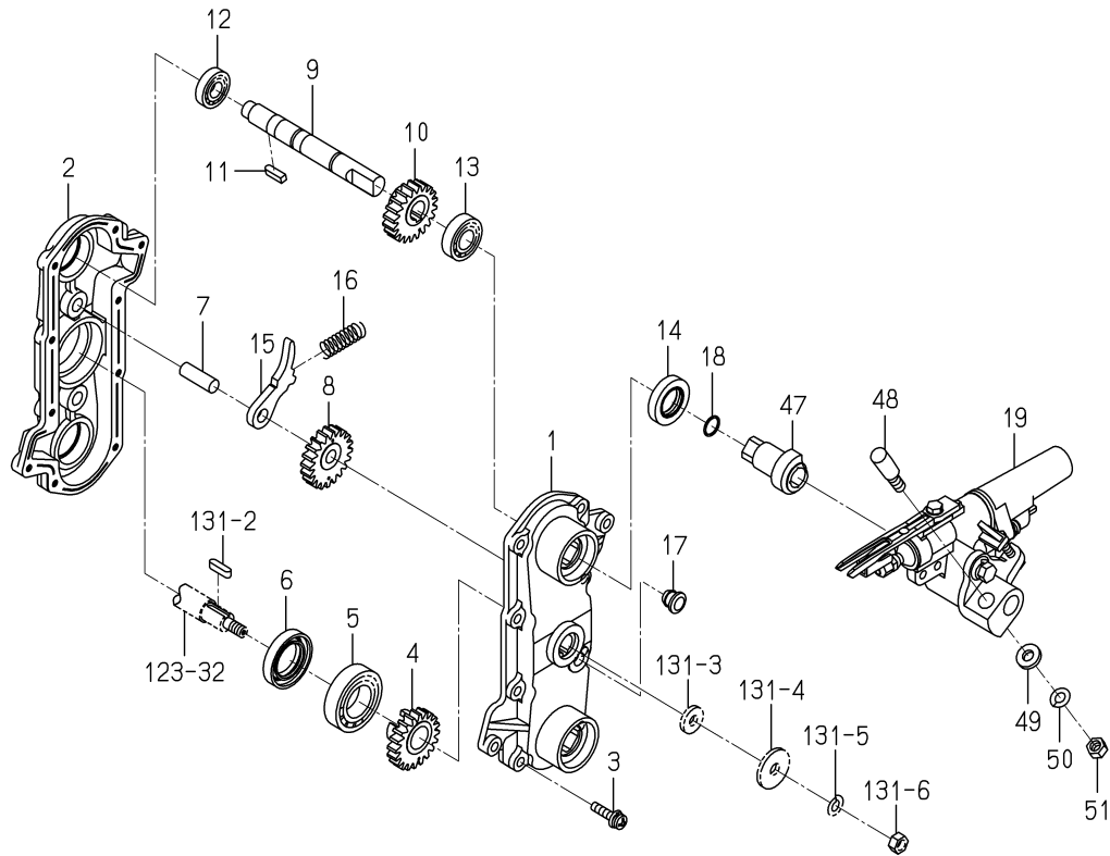
FIG.152 COMPONENT PARTS(1/2) FOR 2204-738-440-40 ON Fig.131
