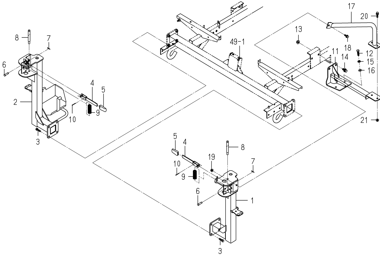
FIG. 82 STAY (FRAME/SEEDLING/SUB)SYSTEM(G TYPE)
