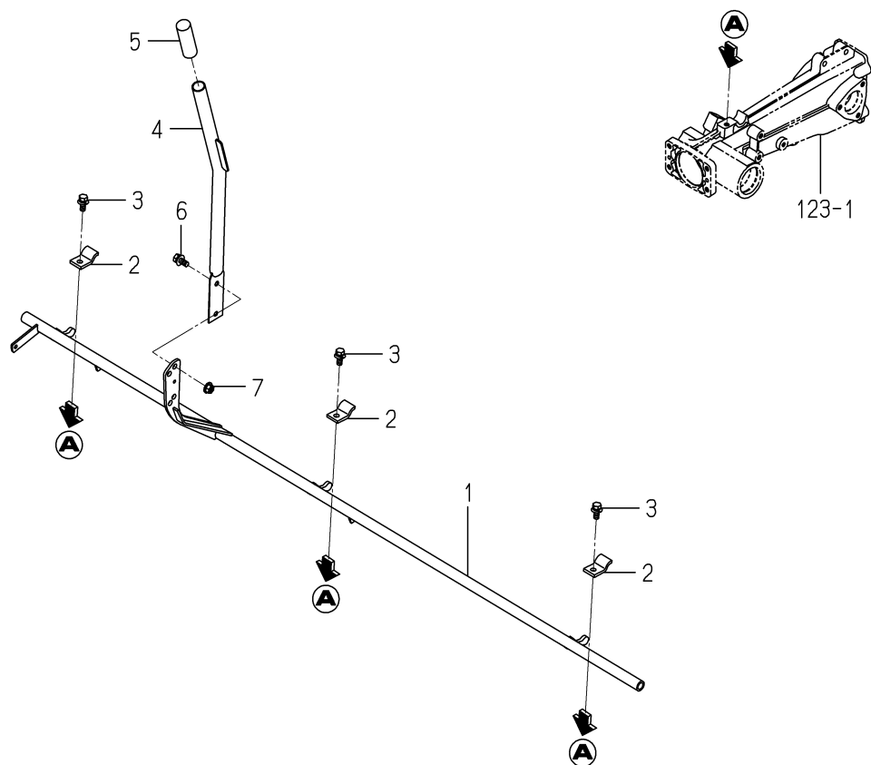
FIG.127 LEVER(PICKING/SEEDLING)SYSTEM
