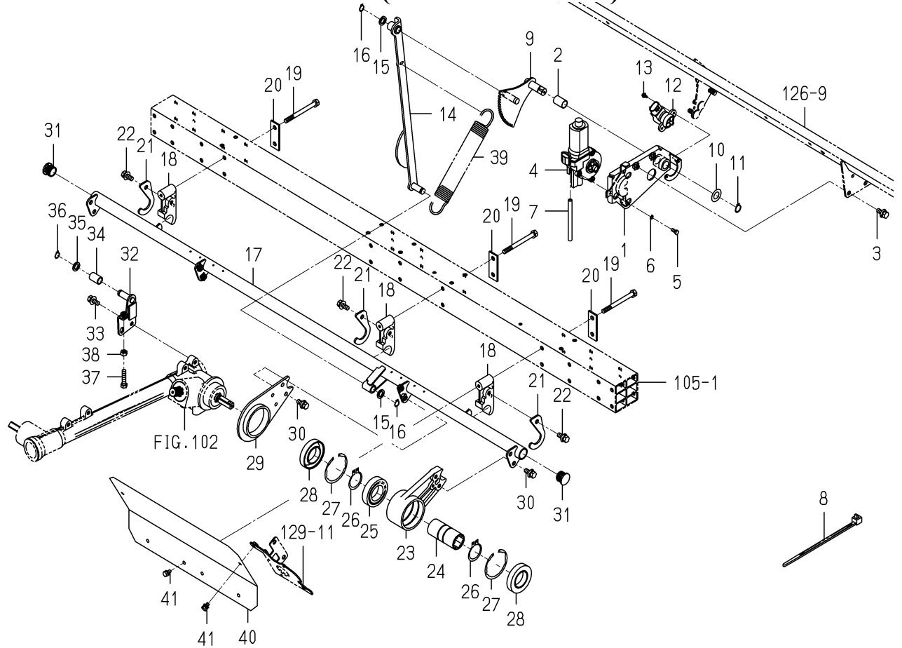
FIG.101 CONTROL(DEPTH/ROTOR)SYSTEM
