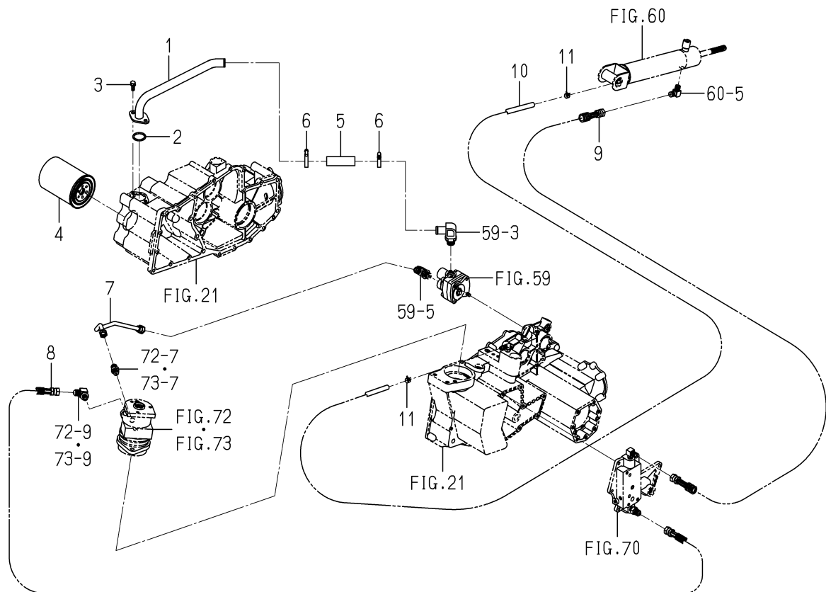
FIG. 61 PIPING SYSTEM
