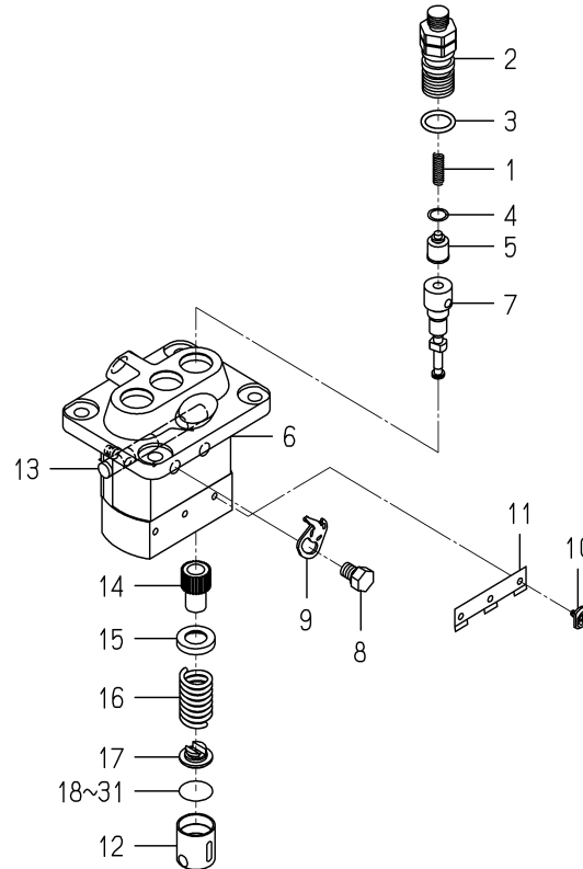
FIG. 27 COMPONENT PARTS FOR 6215-600-156-20 ON Fig.20
