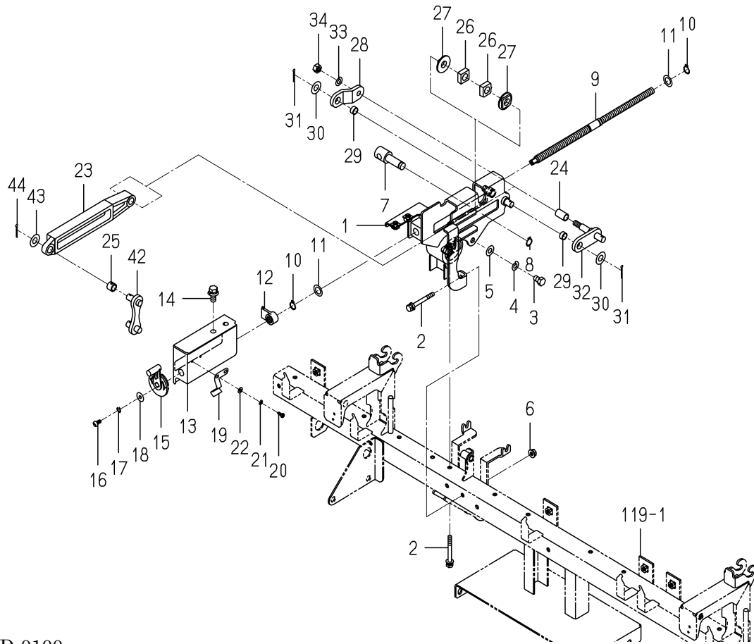
FIG.116 DRIVE(FERTILIZER)SYSTEM(D TYPE)(1/2)
