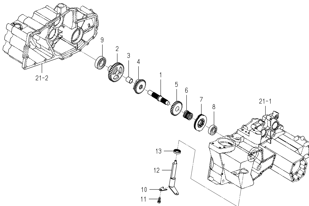
FIG. 27 SHAFT(CHANGE)SYSTEM(D TYPE)
