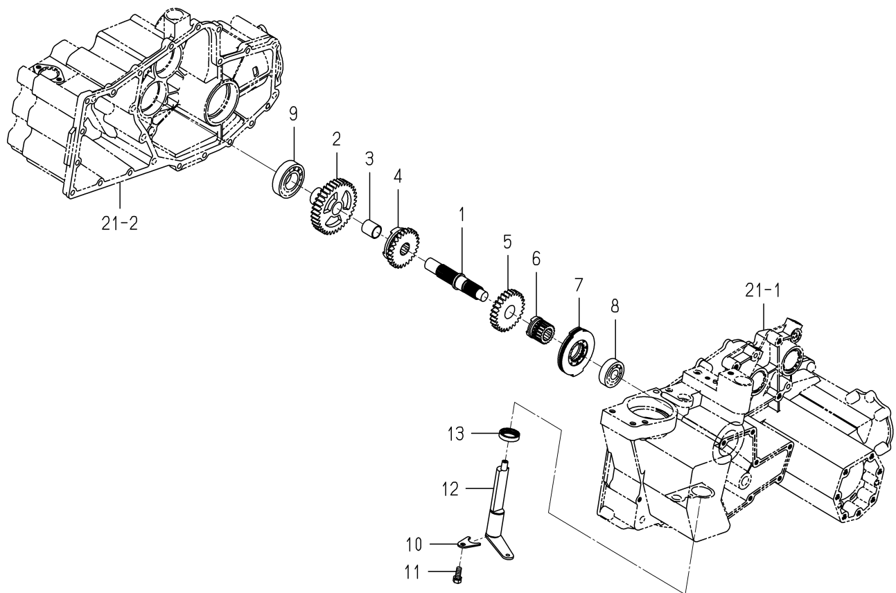
FIG. 26 SHAFT(CHANGE)SYSTEM(G TYPE)
