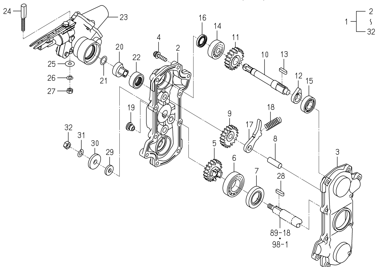
FIG.107 ROTARY PLANTER (RH) SYSTEM
