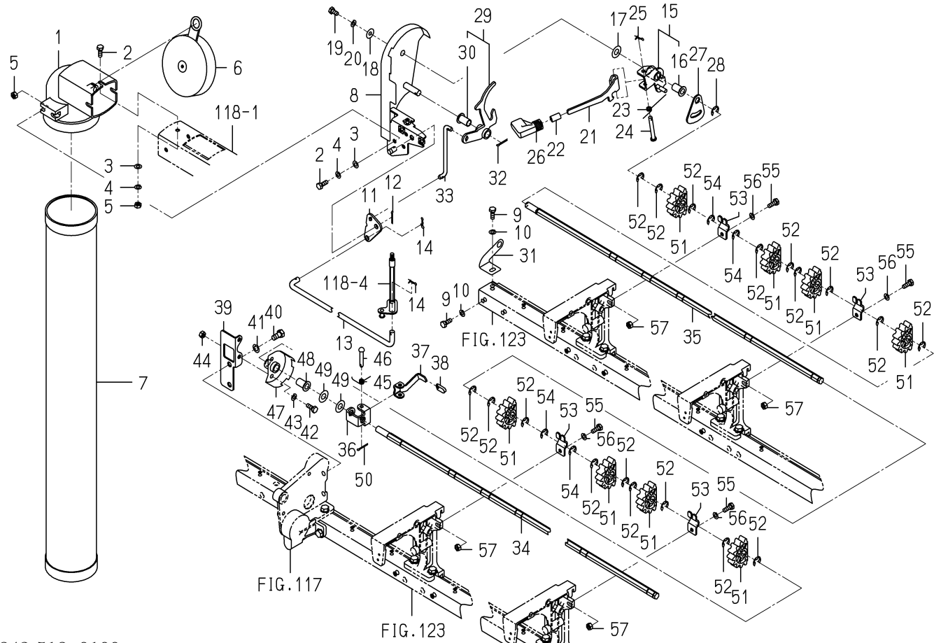
FIG.119 DUCT (BLOW) SYSTEM (F TYPE)
