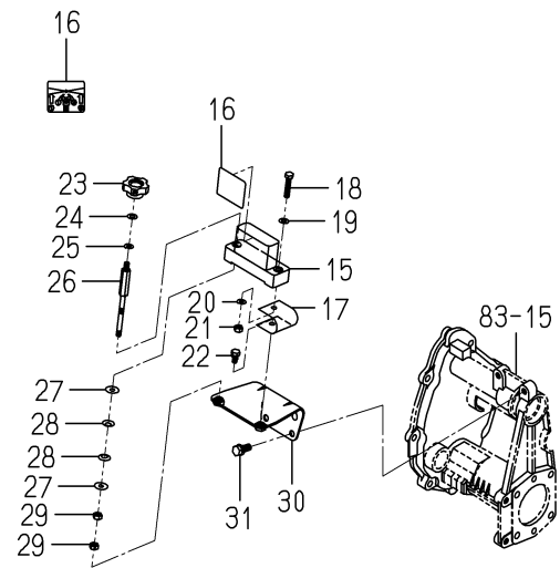
FIG. 80 CONTROLLER SYSTEM
