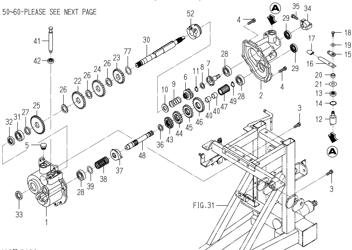
FIG. 47 CASE (FEEDING DRIVE) SYSTEM(1/2) (F TYPE)
