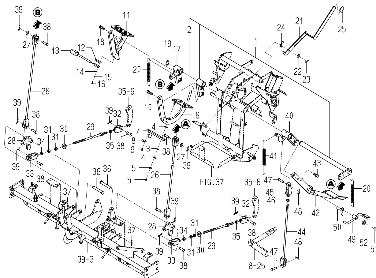
FIG. 38 PEDAL (BRAKE/CLUTCH) SYSTEM
