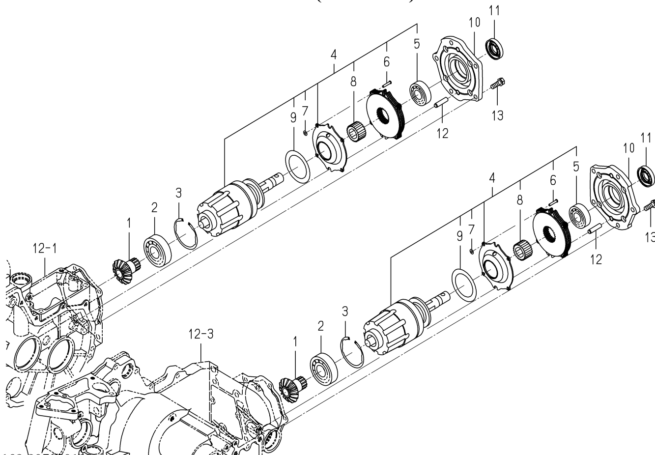
FIG. 16 SHAFT (OUTPUT) SYSTEM
