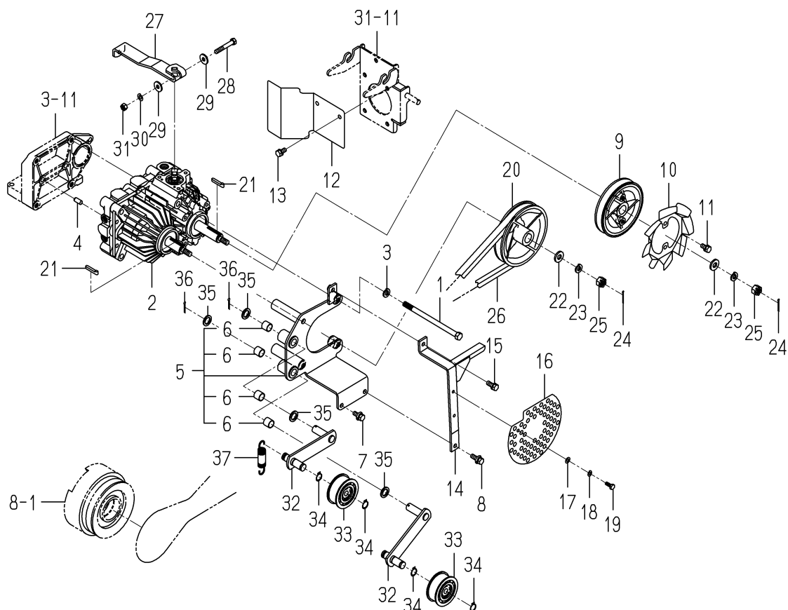
FIG. 9 HST SYSTEM
