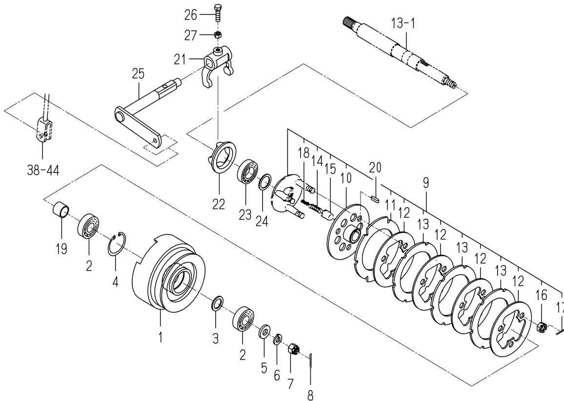
FIG. 8 CLUTCH SYSTEM
