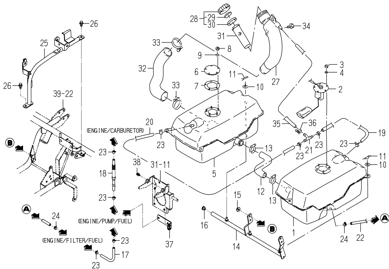
FIG. 4 FUEL TANK SYSTEM
