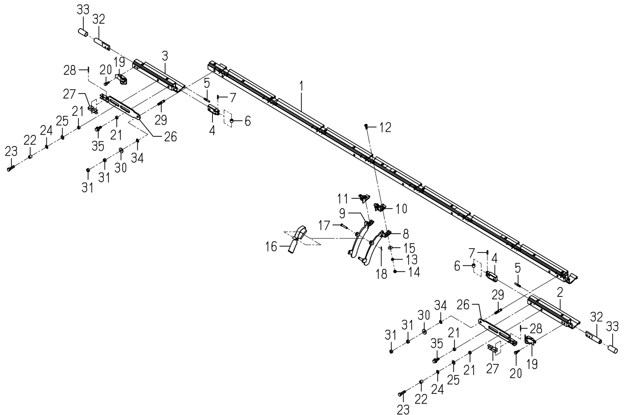
FIG.110 FRONT PLATE SYSTEM
