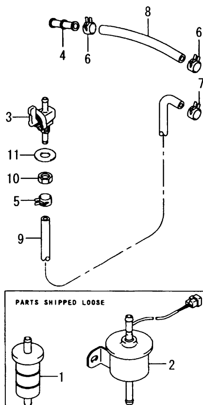
FIG. 10 FUEL-TANK/FUEL-VALVE
