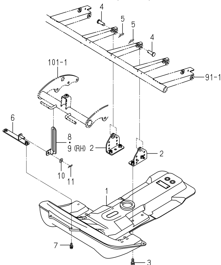
FIG.104 FLOAT (SIDE) SYSTEM
