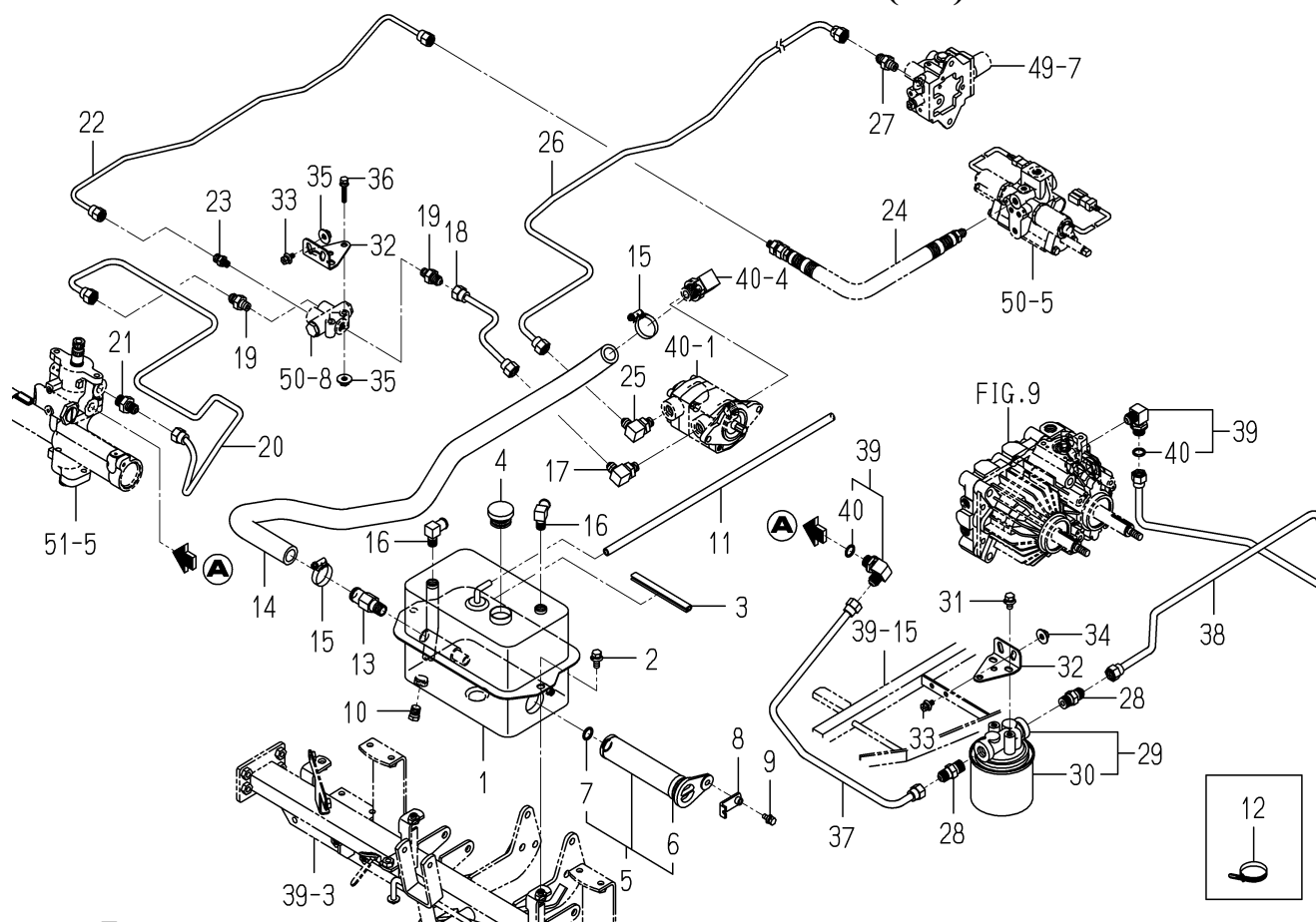
FIG. 42 PIPING SYSTEM(1/2)
