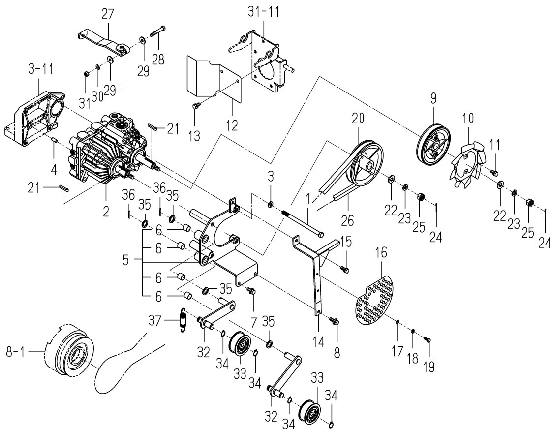
FIG. 9 HST SYSTEM
