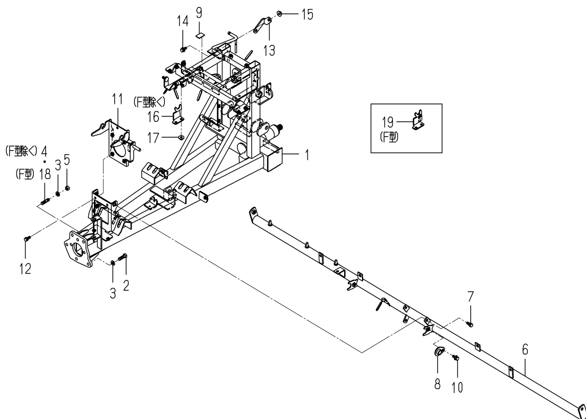
FIG. 31 FRAME SYSTEM
