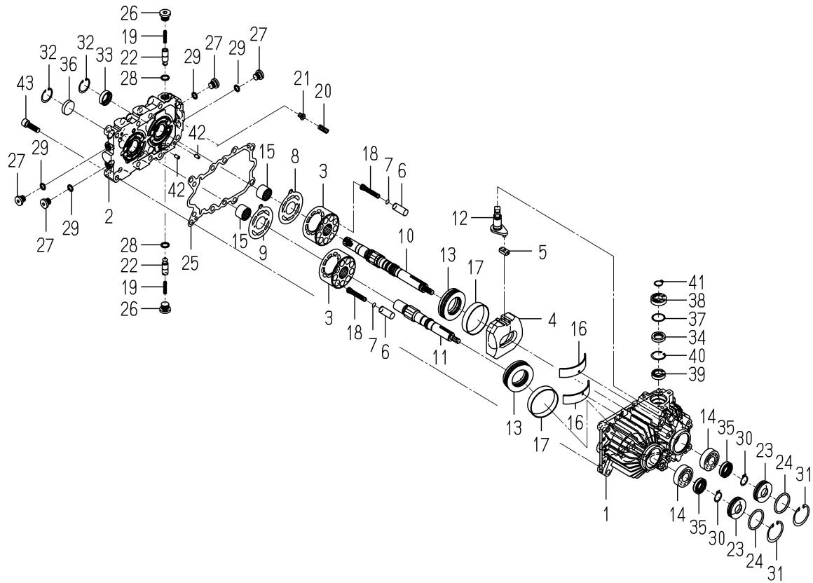
FIG.140 COMPONENT PARTS FOR K510-002-000-10 ON Fig.9
