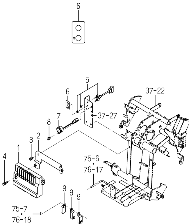
FIG. 80 CONTROLLER SYSTEM
