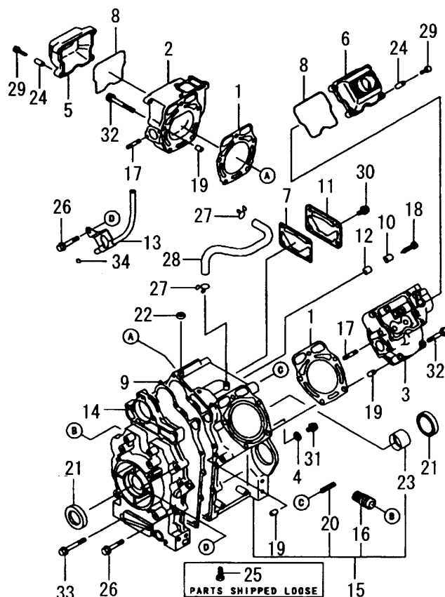
FIG. 1 CYLINDER/CRANKSHAFT
