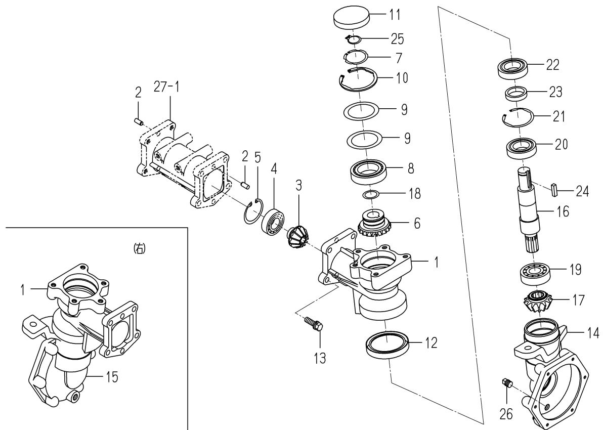
FIG. 28 CASE (FINAL) SYSTEM
