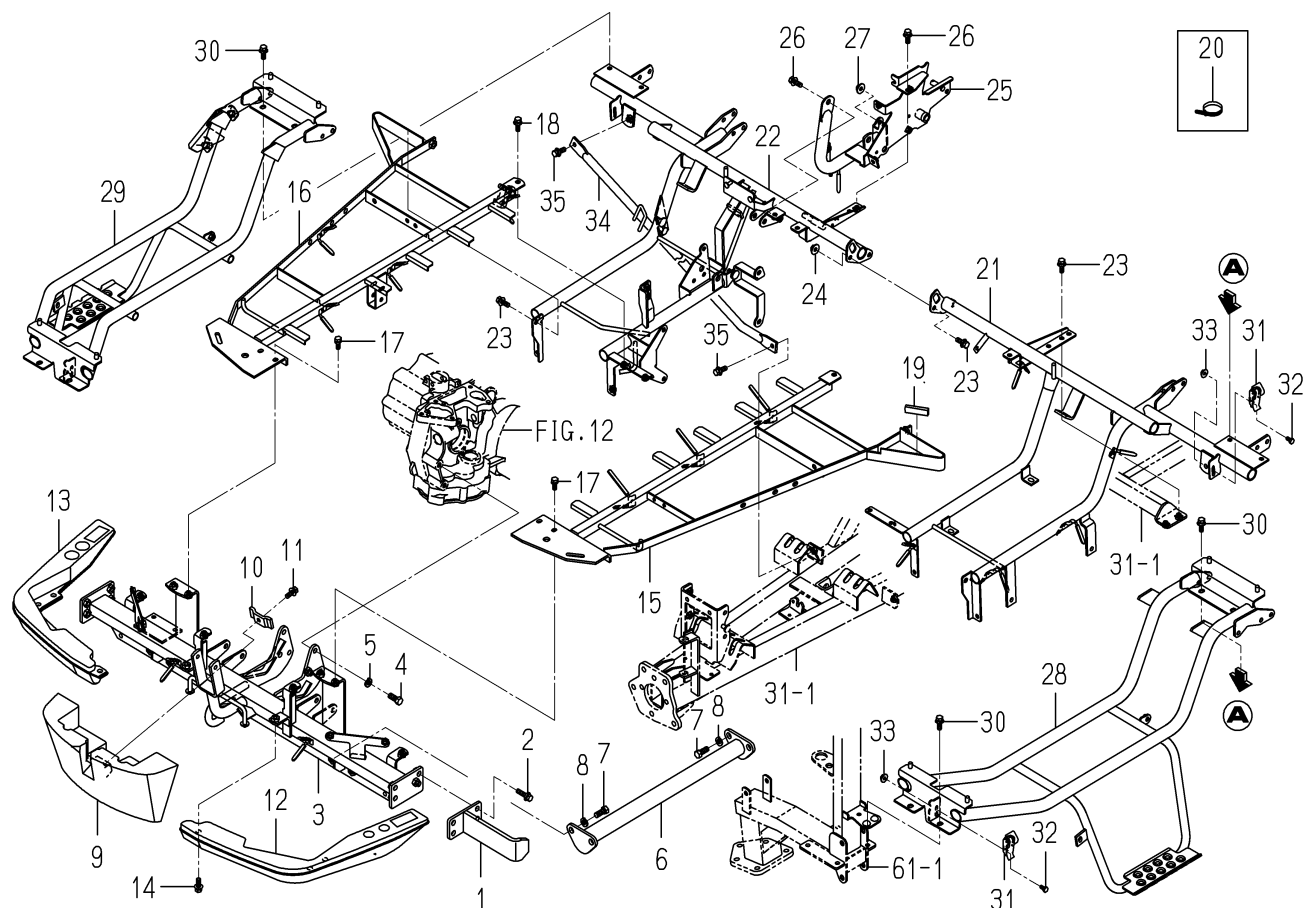
FIG. 39 BUMPER SIDE FRAME SYSTEM
