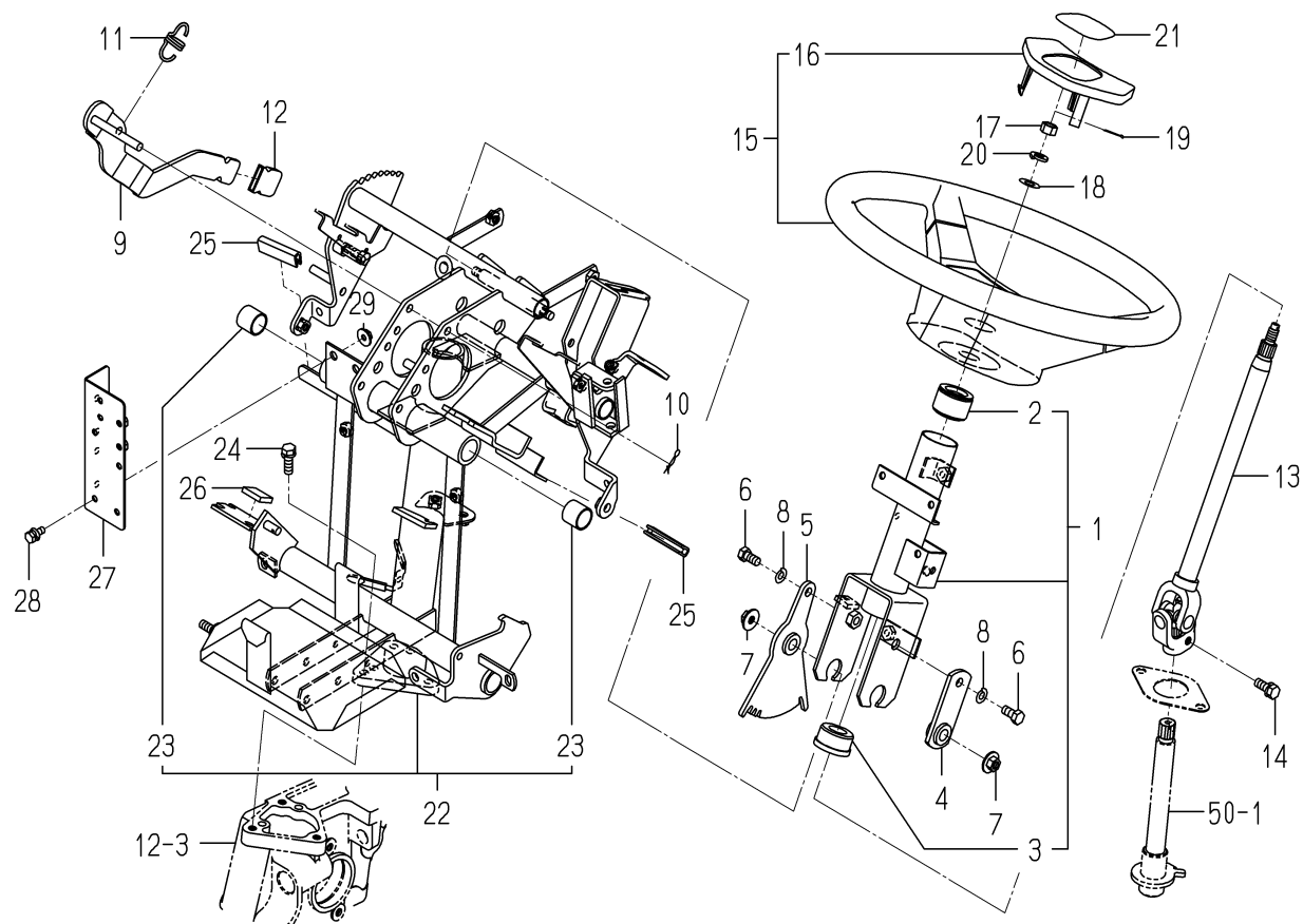
FIG. 37 STEERING SYSTEM
