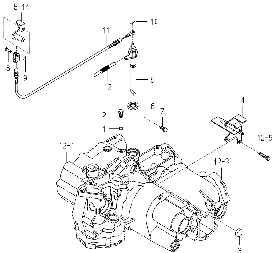
FIG. 21 SHIFTER (SEEDLING INTERVAL), SHAFT (DIFF-LOCK/REAR) SYSTEM
