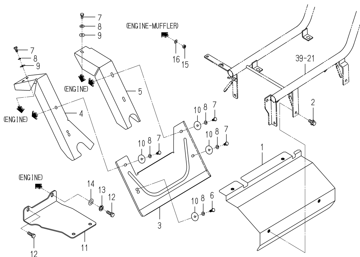
FIG. 5 MUFFLER COVER SYSTEM
