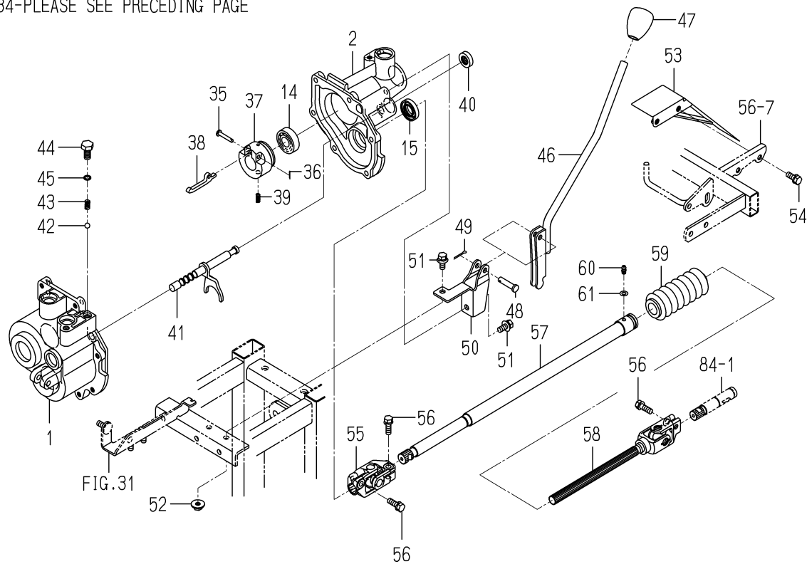
FIG. 48 CASE (FEEDING DRIVE) SYSTEM(2/2) (EXCEPT F TYPE)
