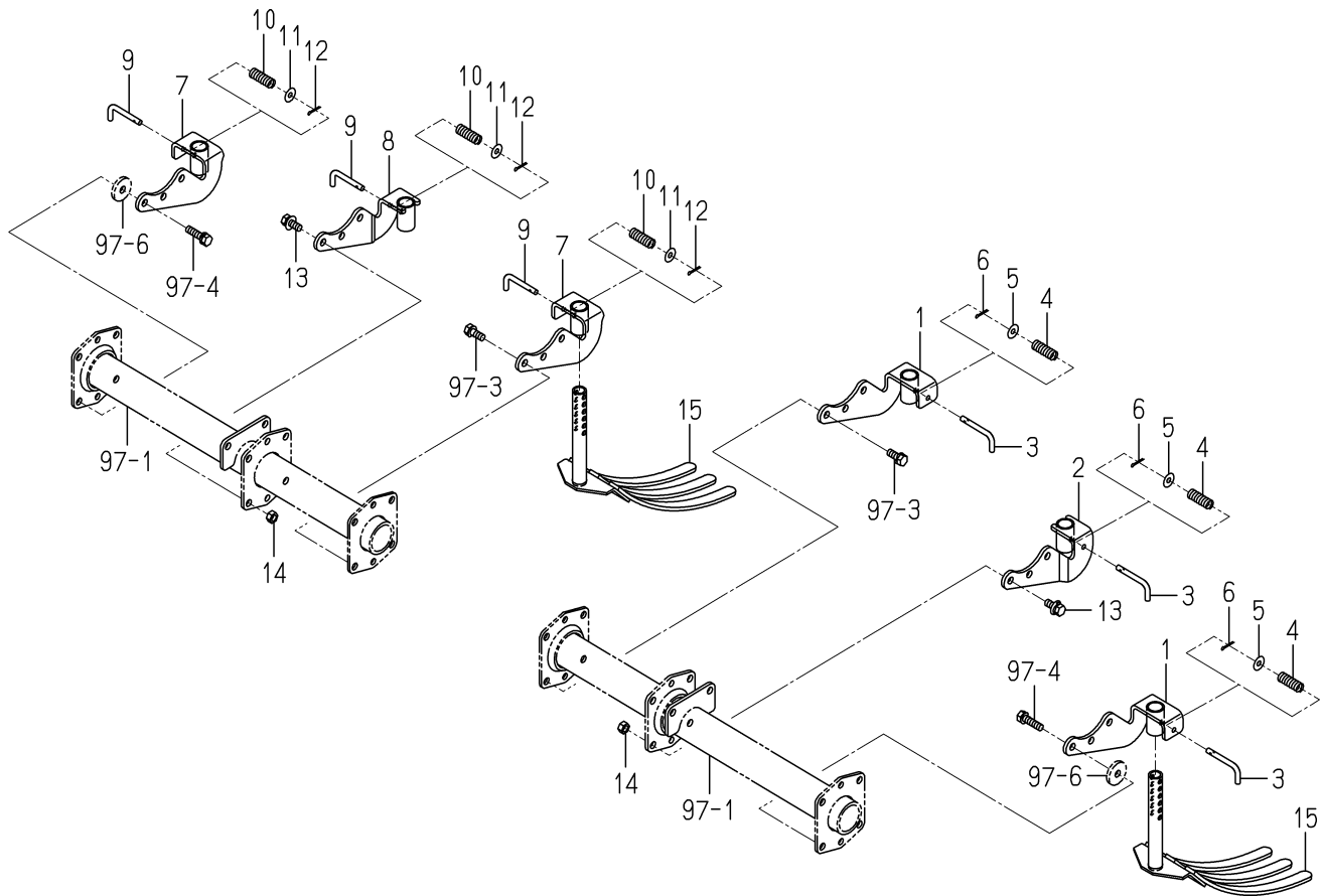
FIG. 95 RAKE SYSTEM
