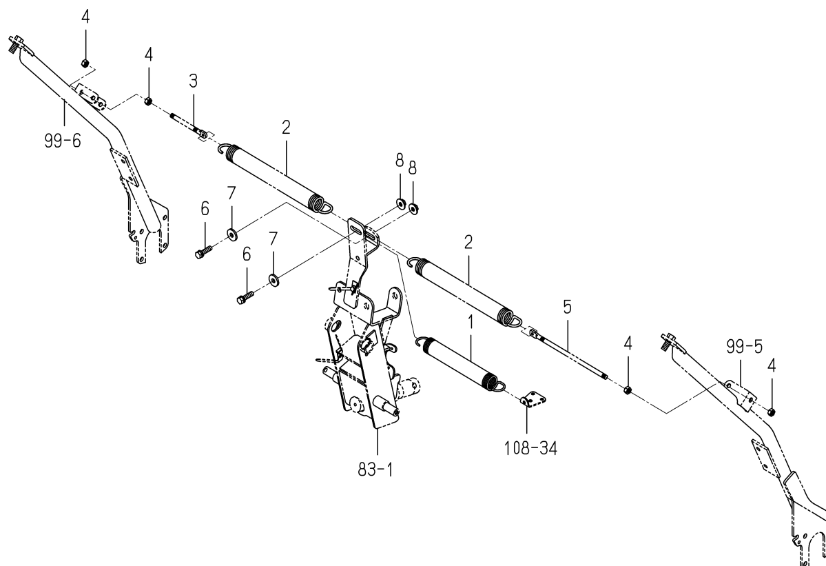
FIG. 94 BALANCE SPRING SYSTEM
