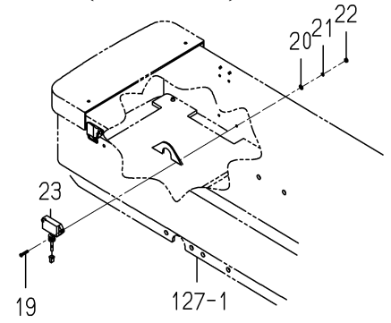
FIG.121 HARNESS SENSOR SYSTEM (F TYPE)
