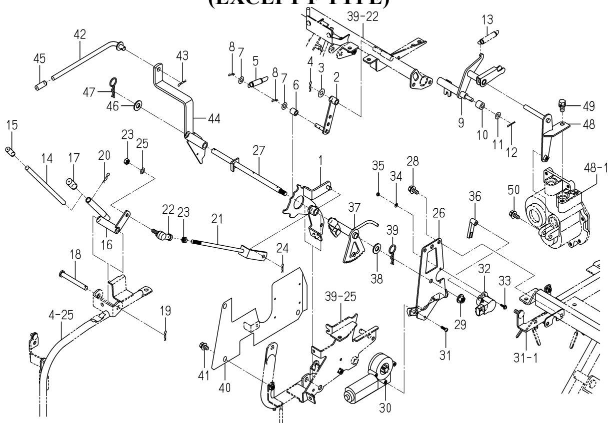
FIG. 70 OIL PRESSURE LEVER SYSTEM (EXCEPT F TYPE)
