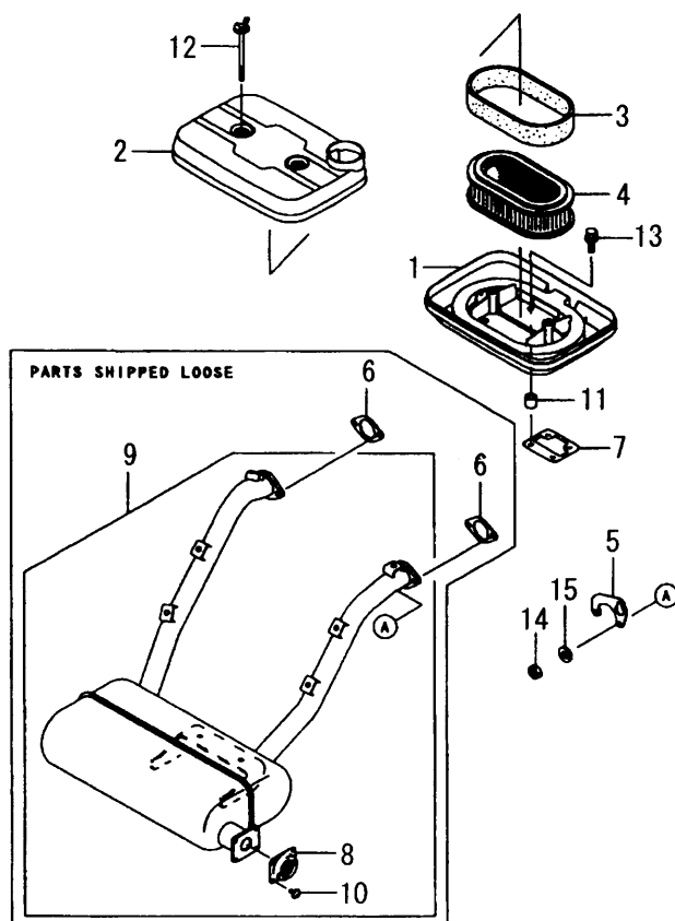
FIG. 9 AIR-FILTER/MUFFLER
