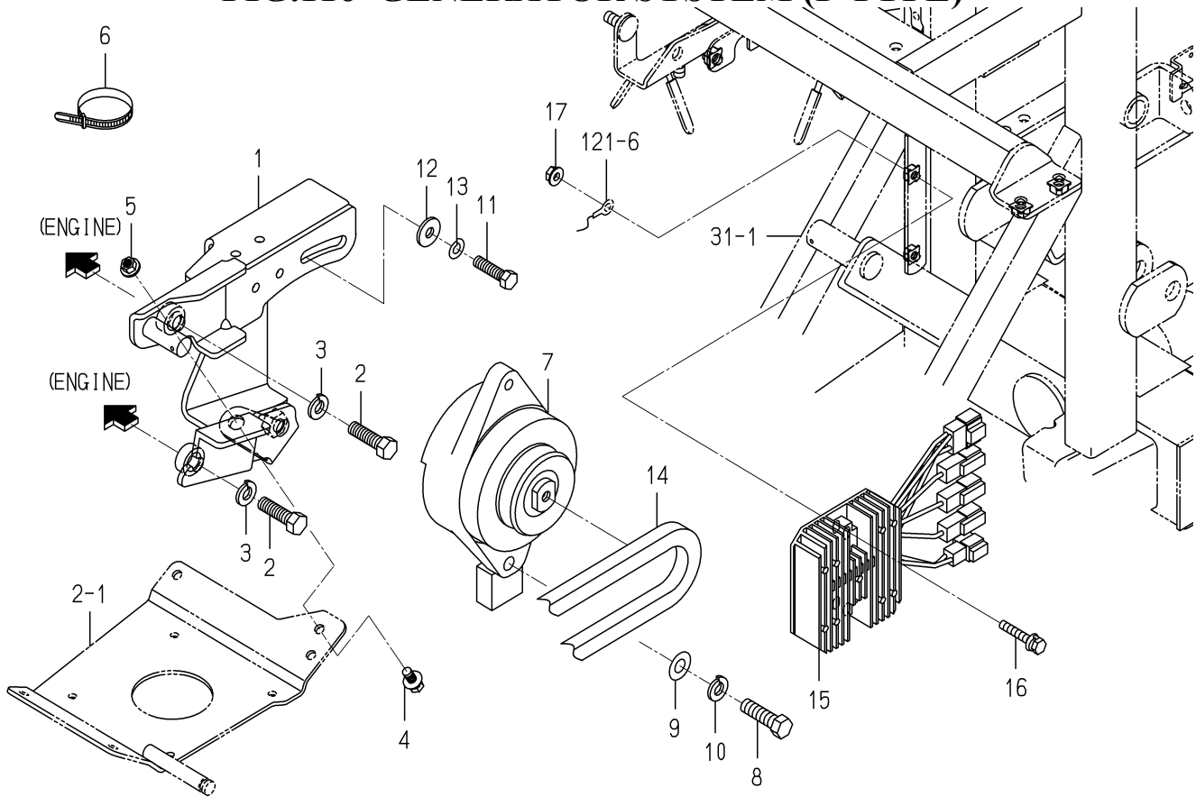
FIG.116 GENERATOR SYSTEM (F TYPE)
