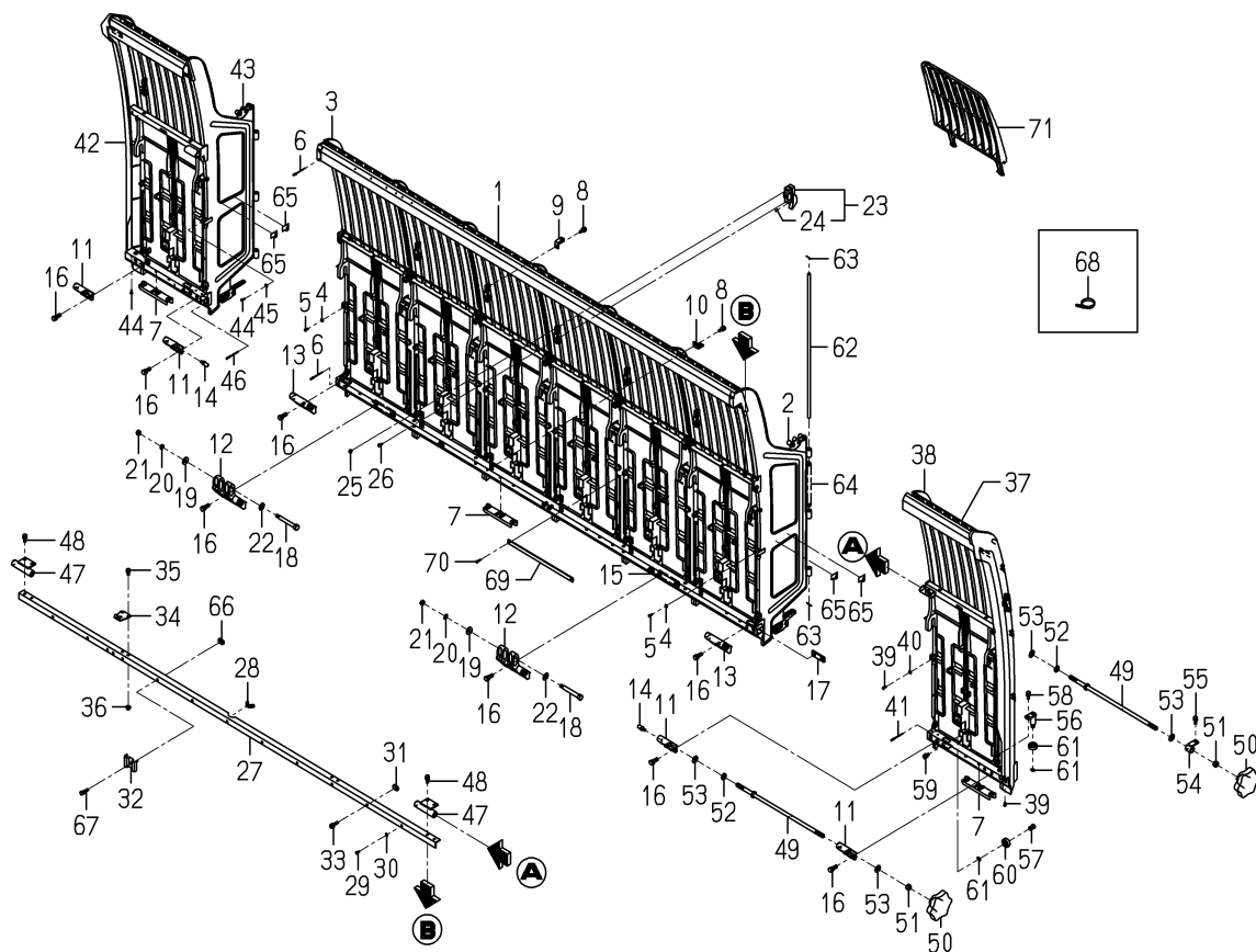
FIG.108 SEEDLING TANK SYSTEM
