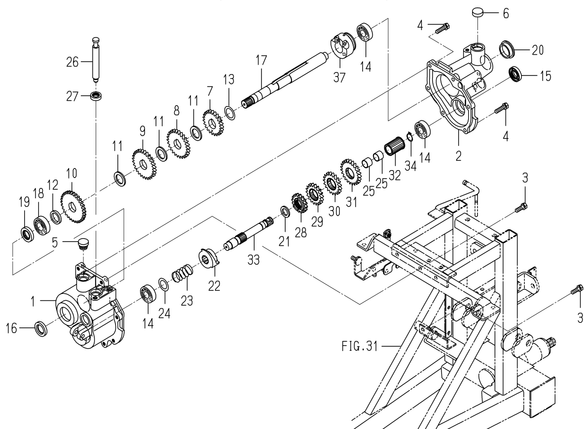
FIG. 48 CASE (FEEDING DRIVE) SYSTEM(1/2) (EXCEPT F TYPE)
