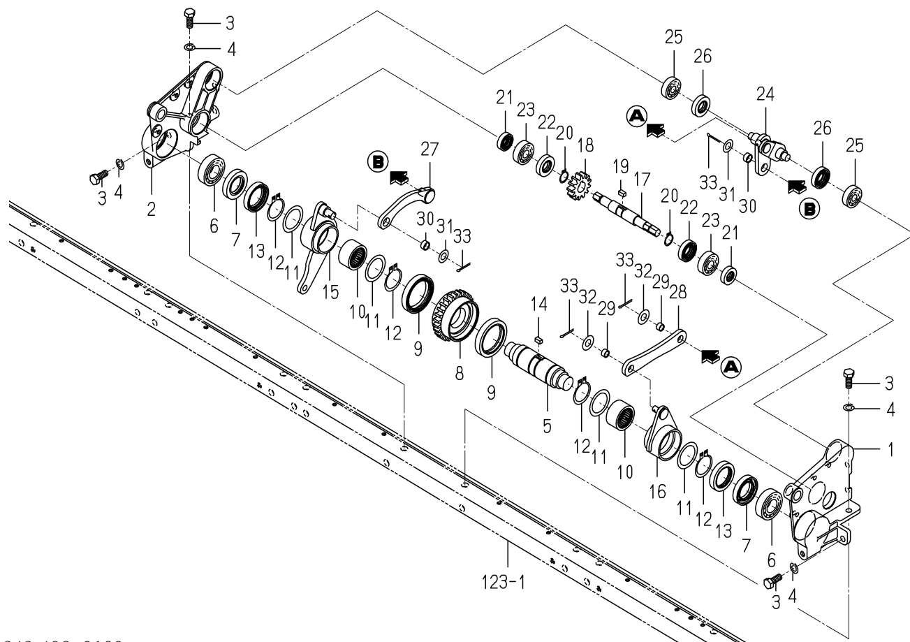
FIG.117 DRIVE SYSTEM (F TYPE)(1/3)
