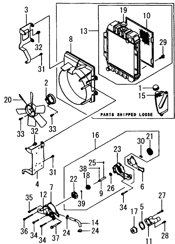
FIG. 5 COOLING-EQUIPMENT
