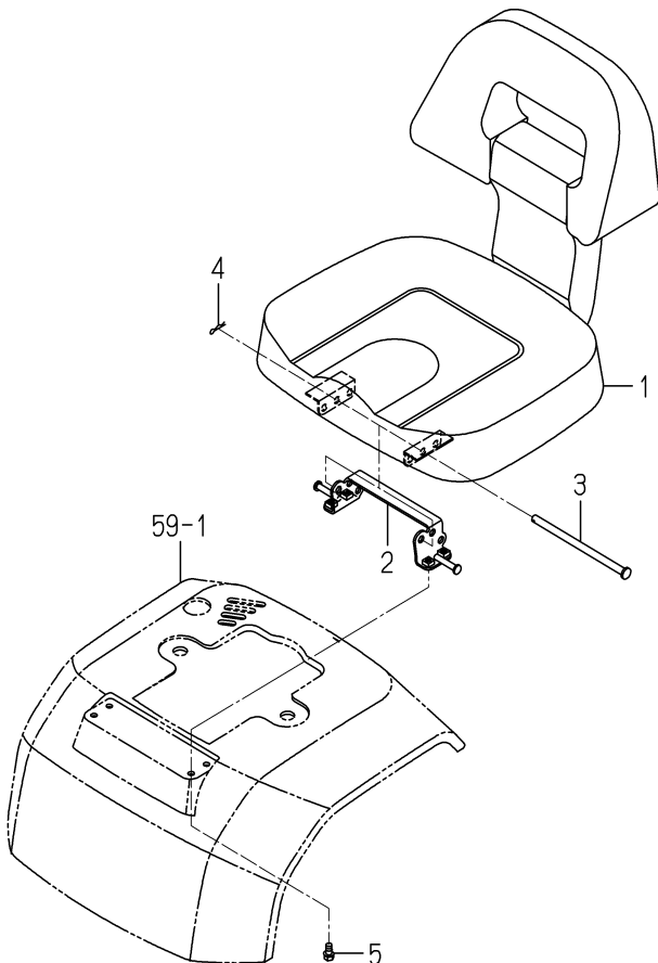
FIG. 63 SEAT SYSTEM
