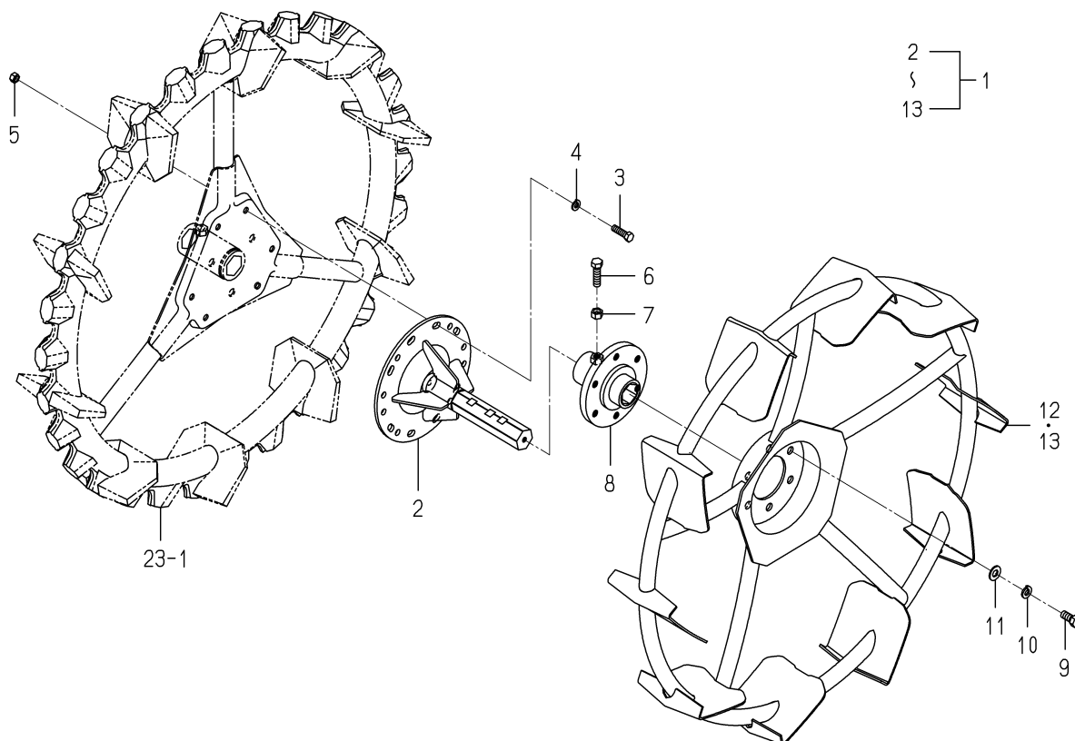
FIG.134 SUB WHEEL (850K/PG/OUT) SET (F TYPE-OPTION)
