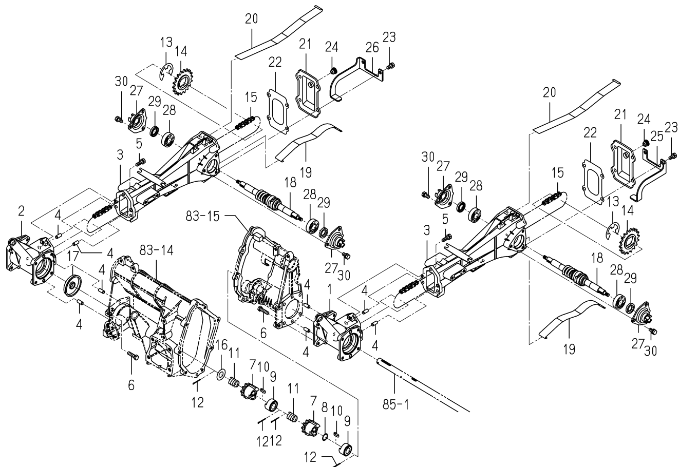
FIG. 89 SHAFT (PLANTING/CENTER) SYSTEM
