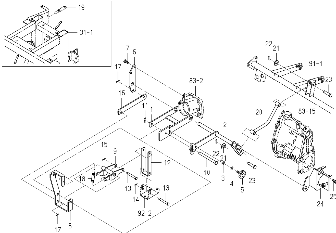
FIG. 93 FLOAT LINK SYSTEM
