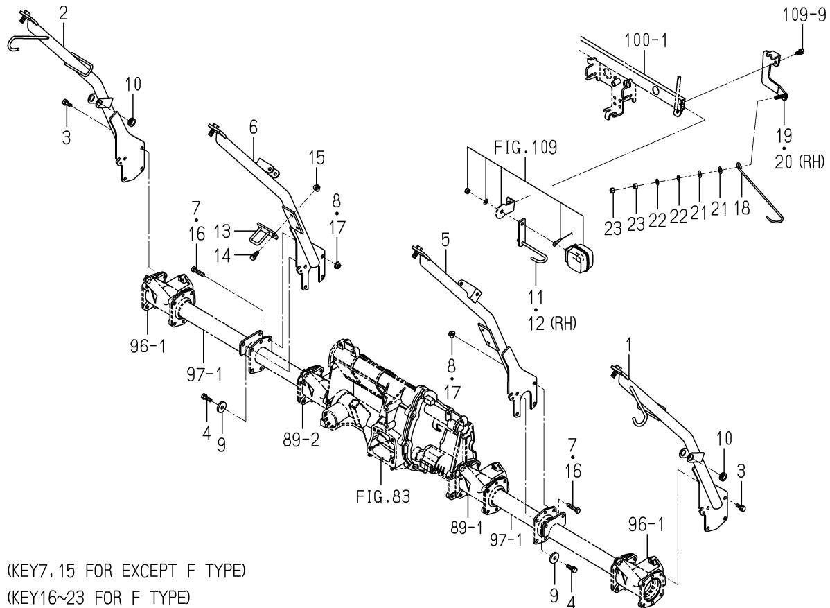
FIG. 99 SUPPORT PIPE SYSTEM
