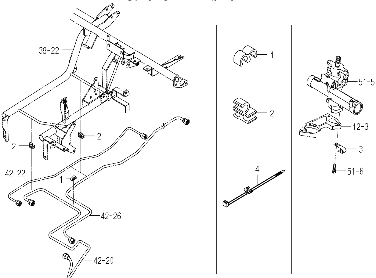
FIG. 43 CLAMP SYSTEM
