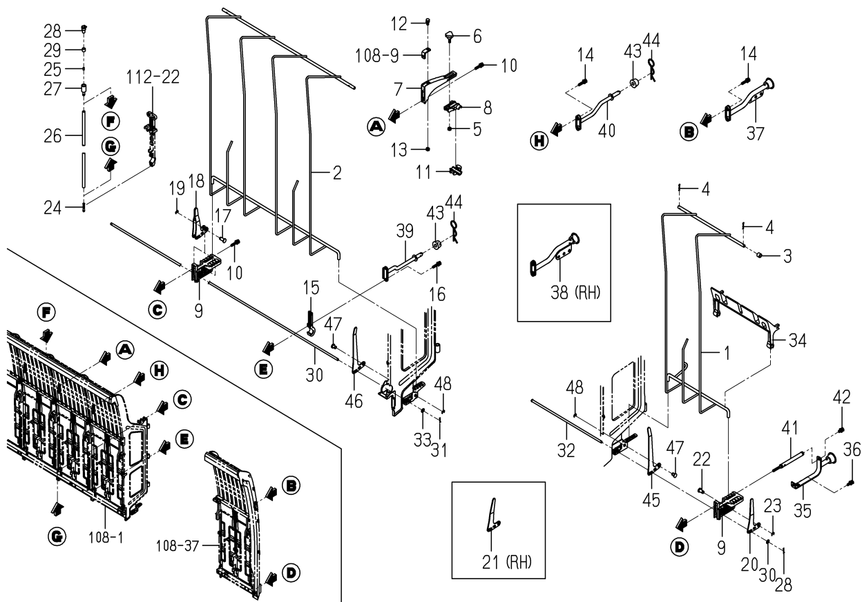
FIG.111 SEEDLING HOLD SYSTEM
