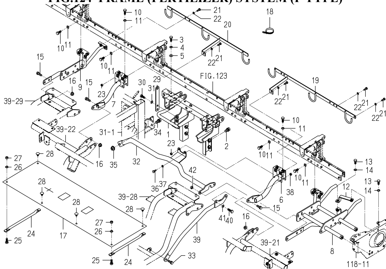
FIG.124 FRAME (FERTILIZER) SYSTEM (F TYPE)
