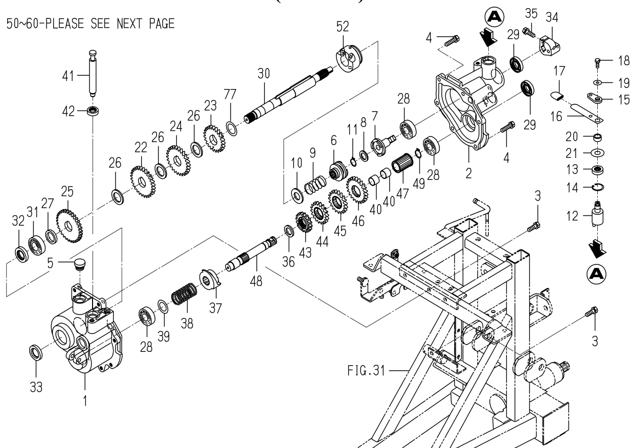
FIG. 47 CASE (FEEDING DRIVE) SYSTEM(1/2) (F TYPE)
