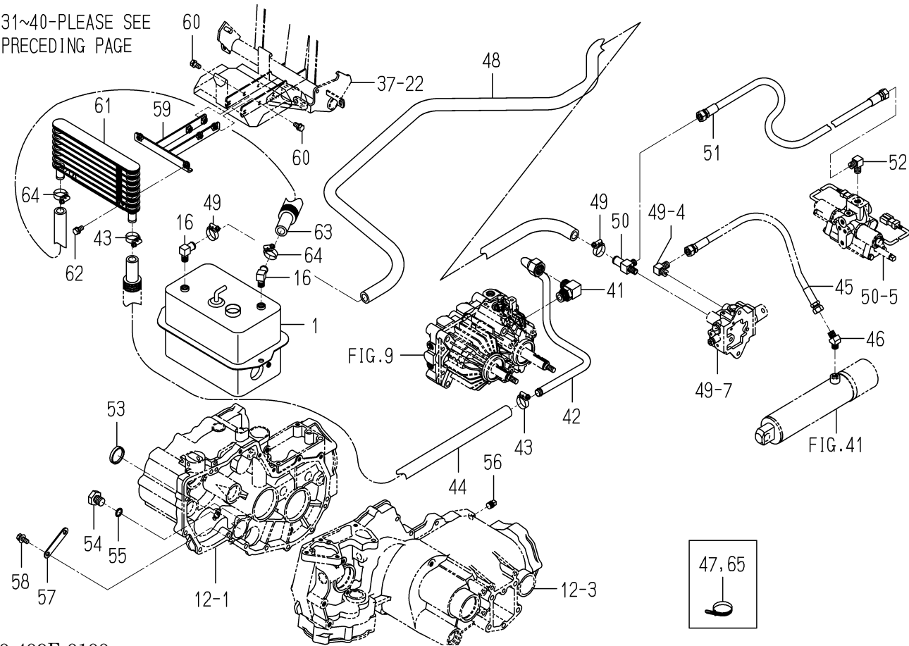
FIG. 42 PIPING SYSTEM(2/2)
