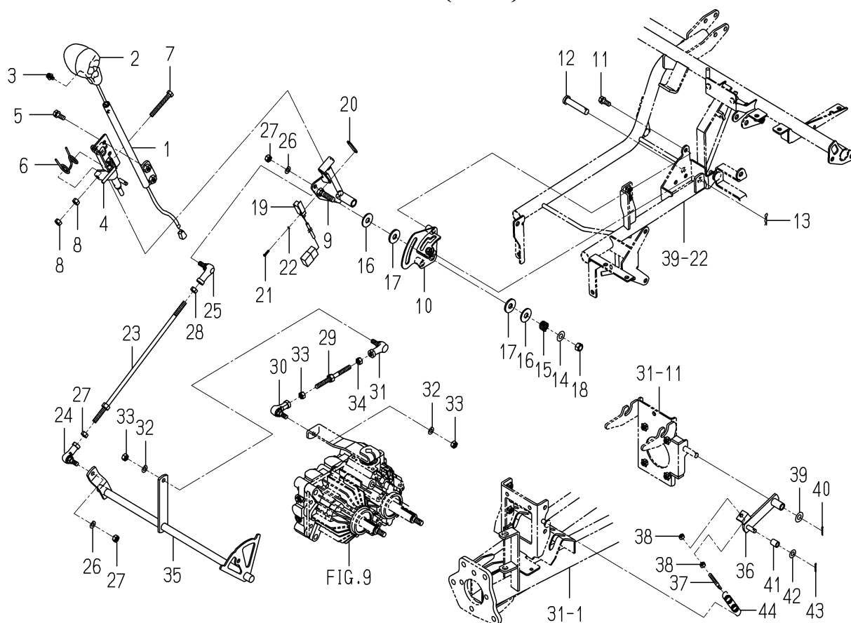
FIG. 7 LEVER (HST) SYSTEM
