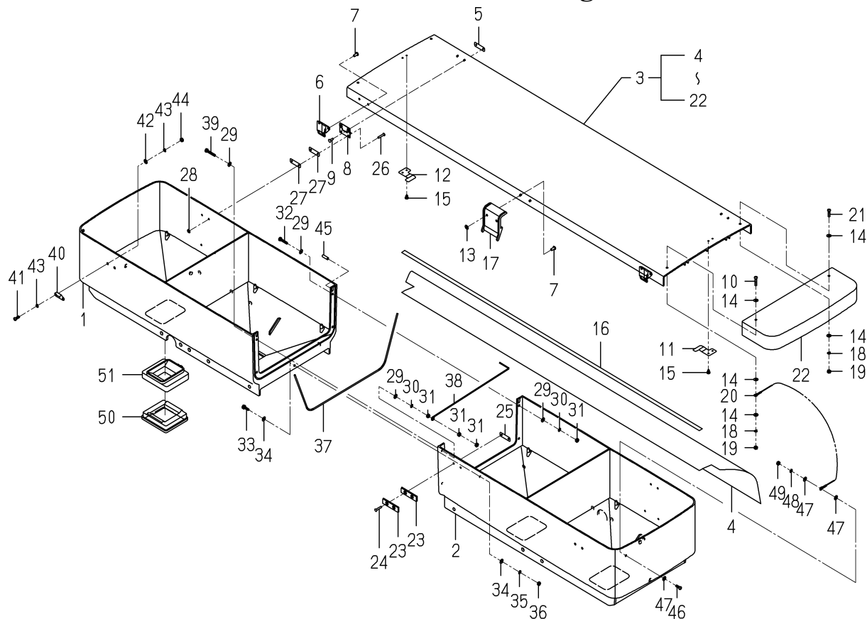
FIG.145 COMPONENT PARTS FOR 8842-718-350-10 ON Fig.127
