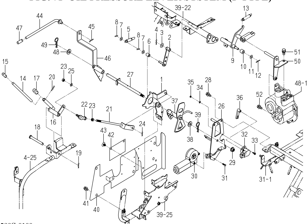
FIG. 71 OIL PRESSURE LEVER SYSTEM (F TYPE)
