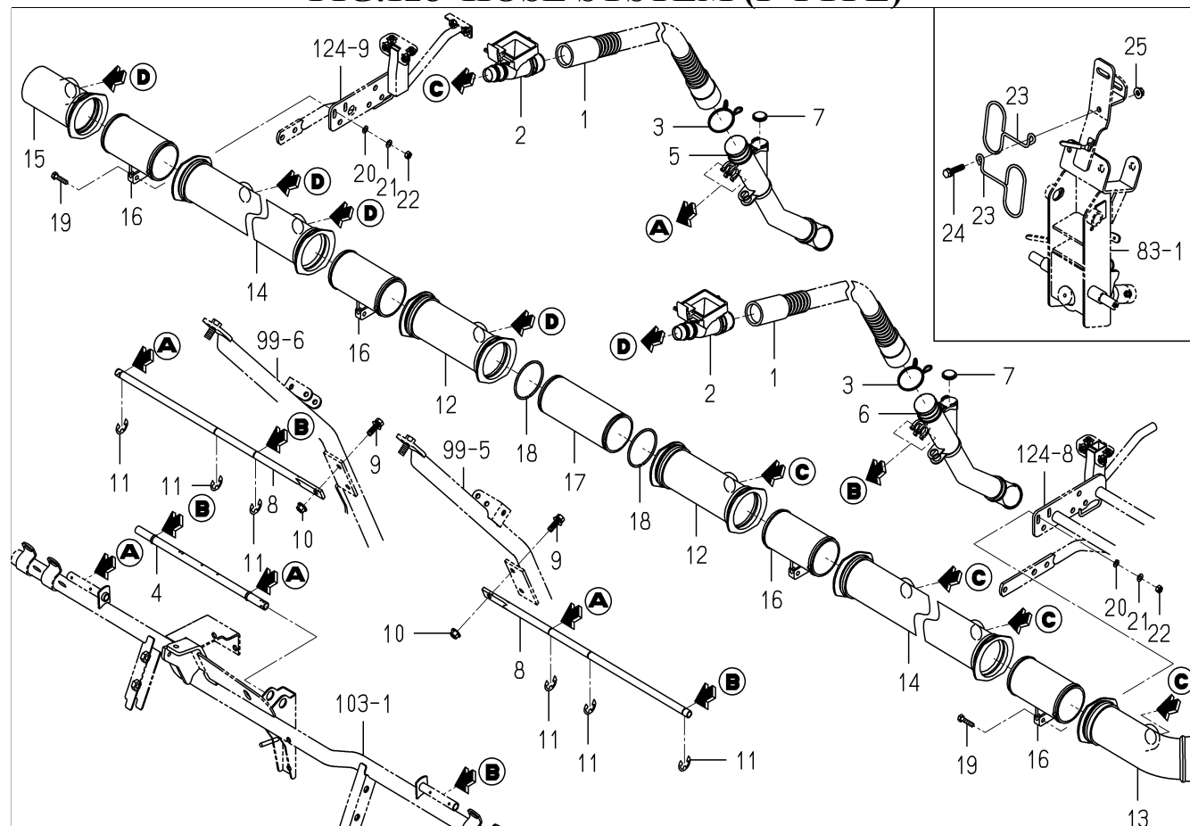
FIG.128 HOSE SYSTEM (F TYPE)
