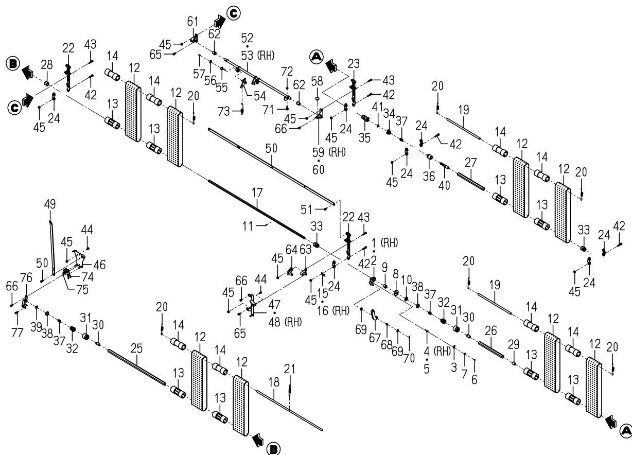
FIG.112 SEEDLING FEED SYSTEM
