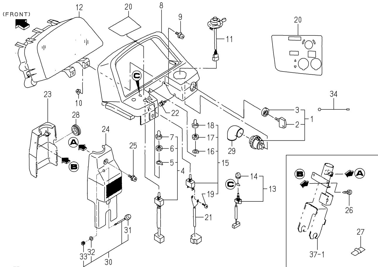
FIG. 74 METER PANEL SYSTEM
