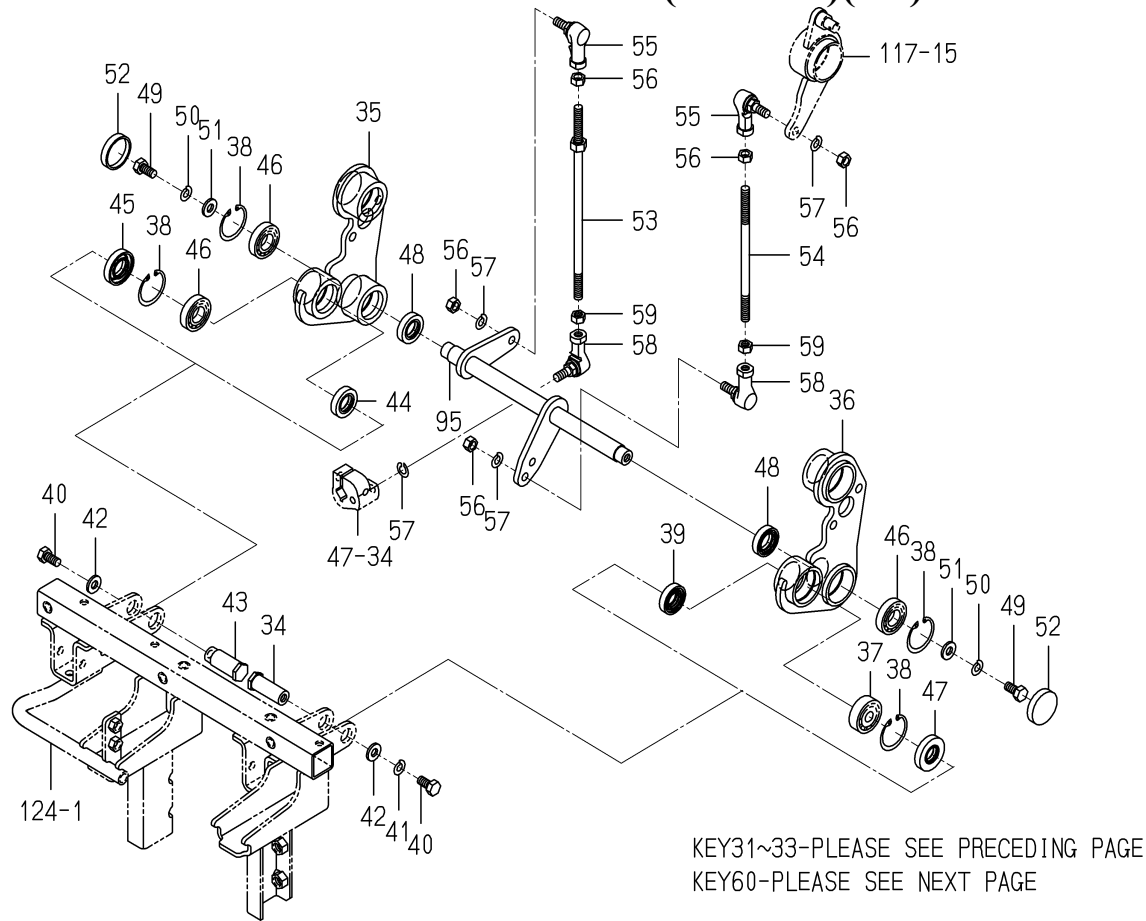
FIG.117 DRIVE SYSTEM (F TYPE)(2/3)
