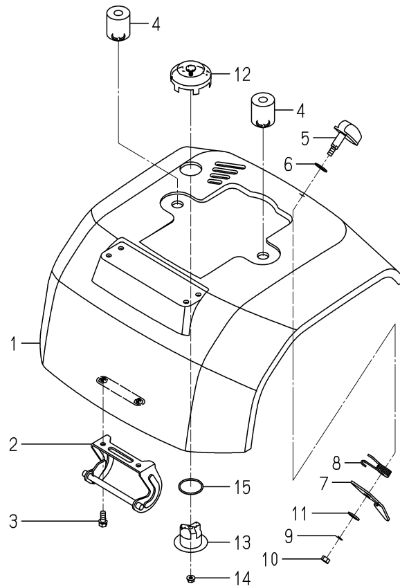
FIG. 59 ENGINE COVER SYSTEM
