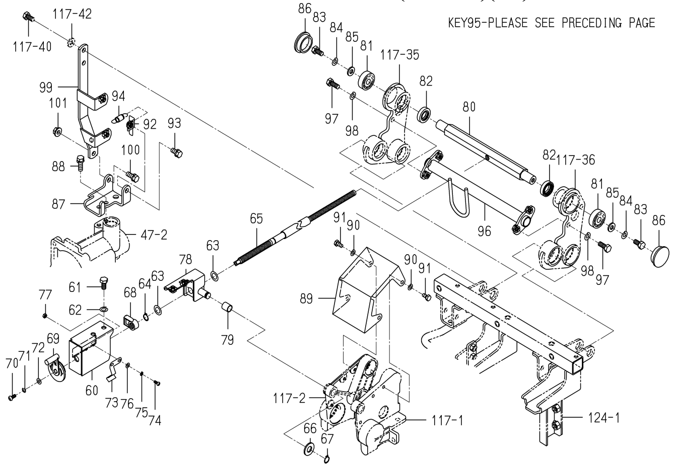
FIG.117 DRIVE SYSTEM (F TYPE)(3/3)
