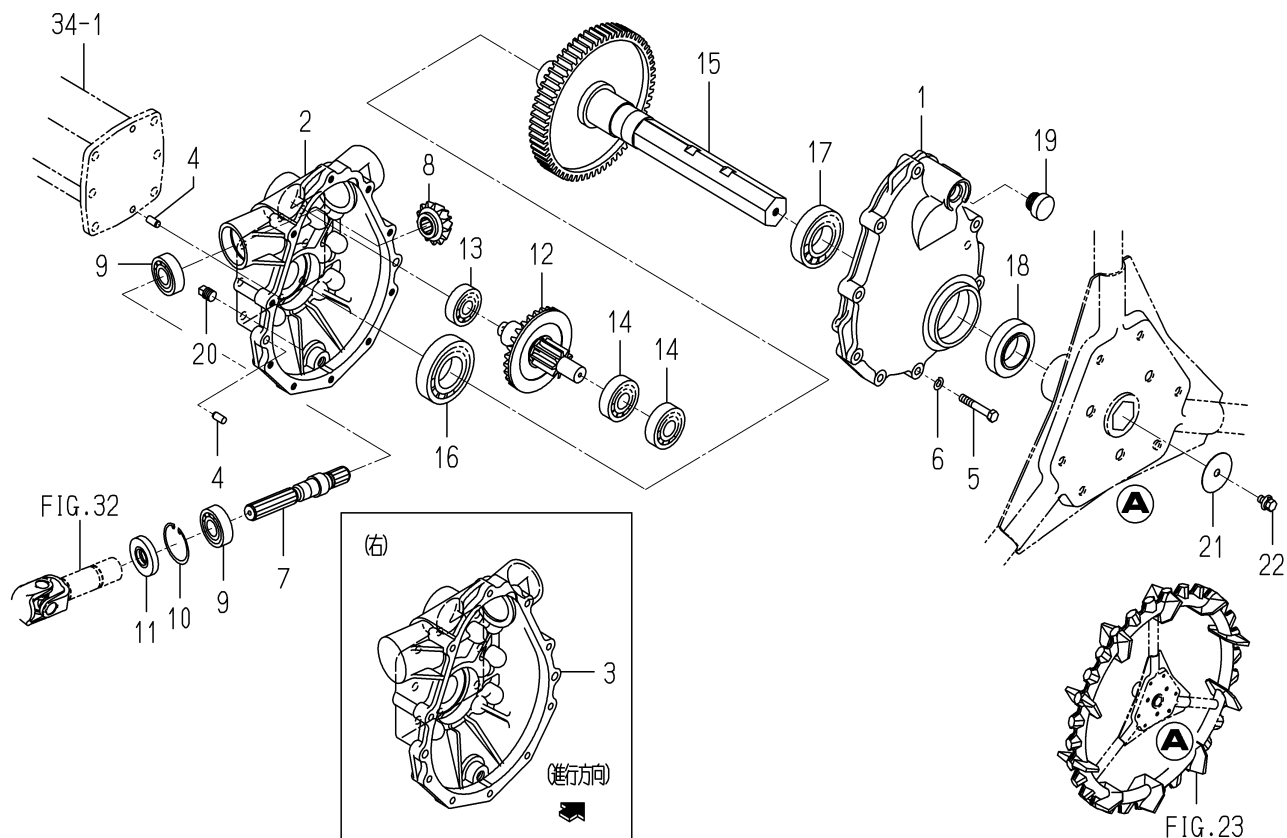
FIG. 36 CASE (REAR) SYSTEM
