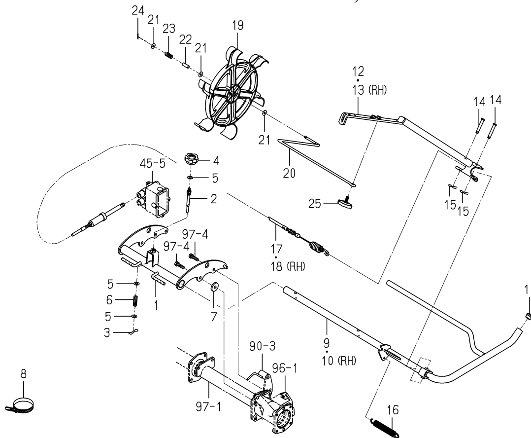
FIG.101 FRONT PLATE GUARD,MARKER SYSTEM
