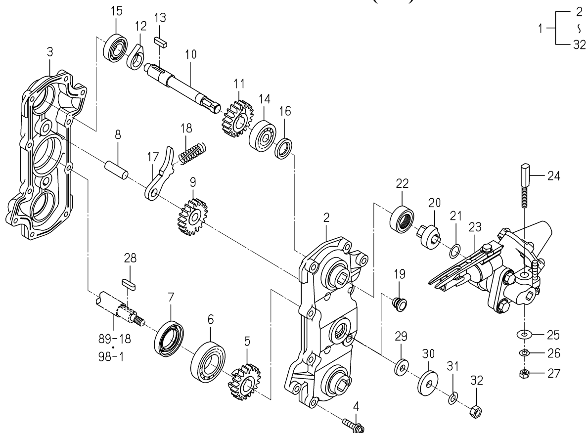
FIG.106 ROTARY PLANTER (LH) SYSTEM
