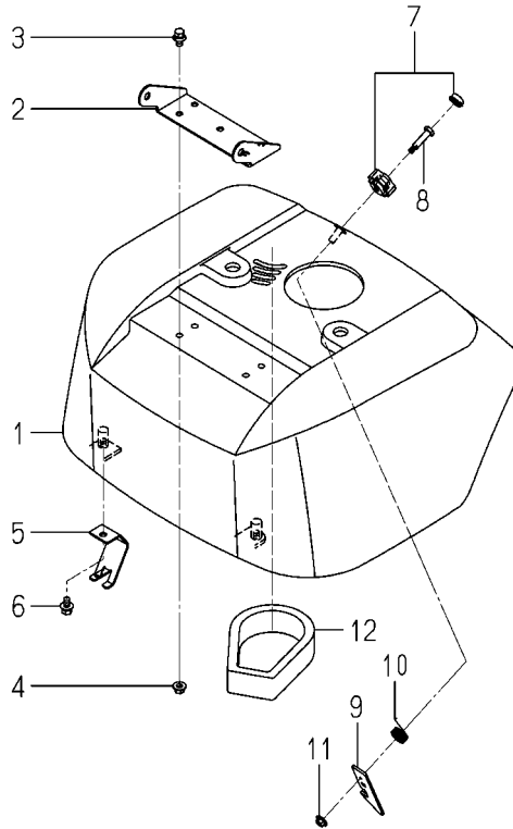
FIG.505 COVER(ENGINE)SYSTEM
