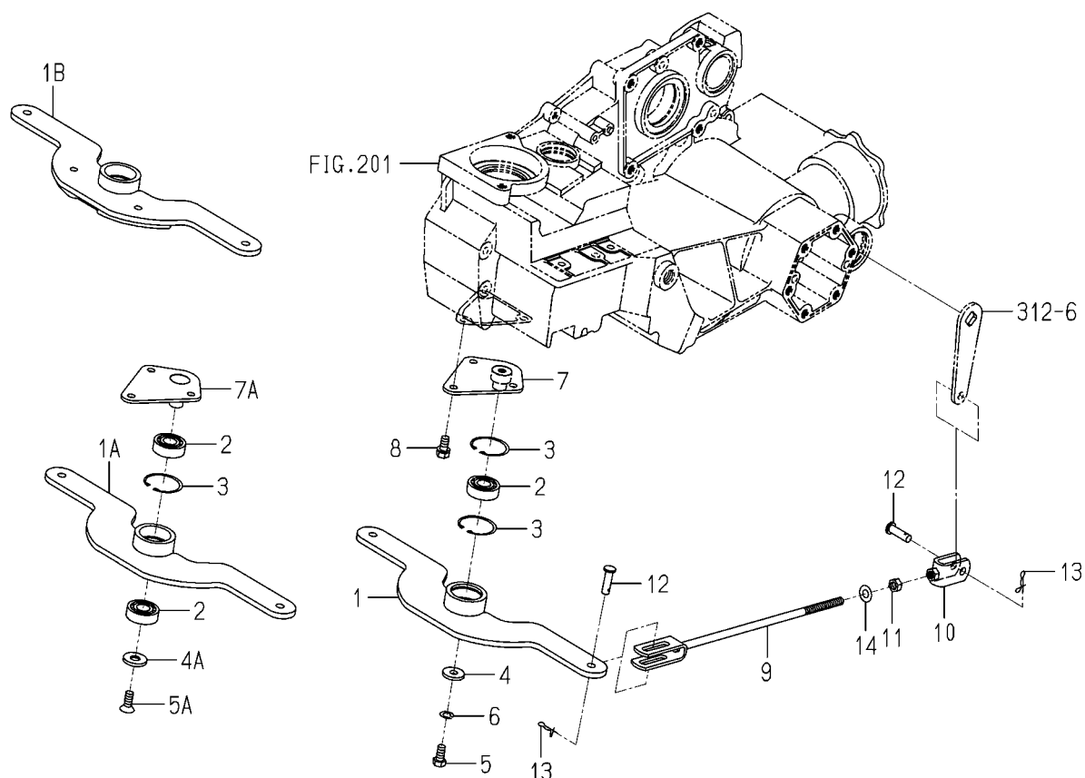
FIG.303 TURN SYSTEM
