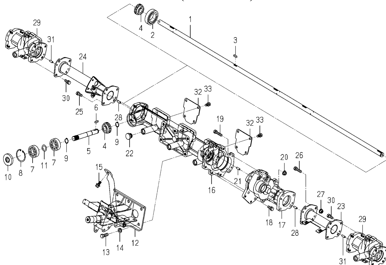
FIG.603 FRAME(PLANTING)SYSTEM
