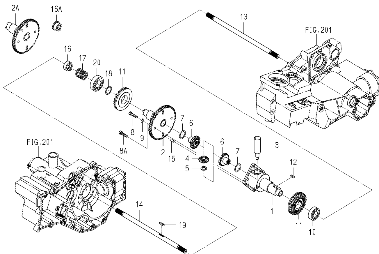
FIG.206 SHAFT(DRIVE/FRONT)SYSTEM
