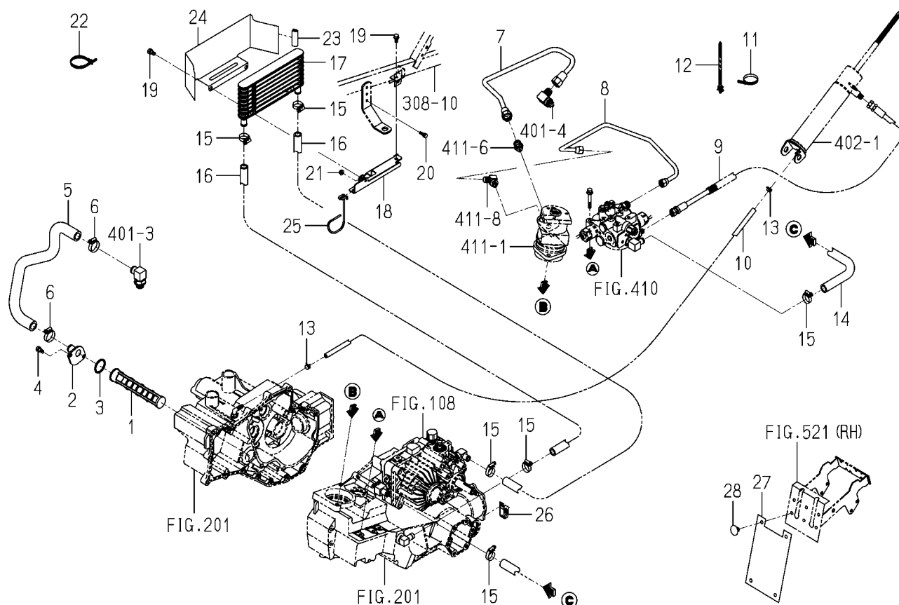
FIG.403 PIPING SYSTEM
