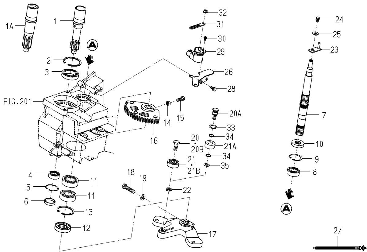
FIG.301 STEERING SYSTEM
