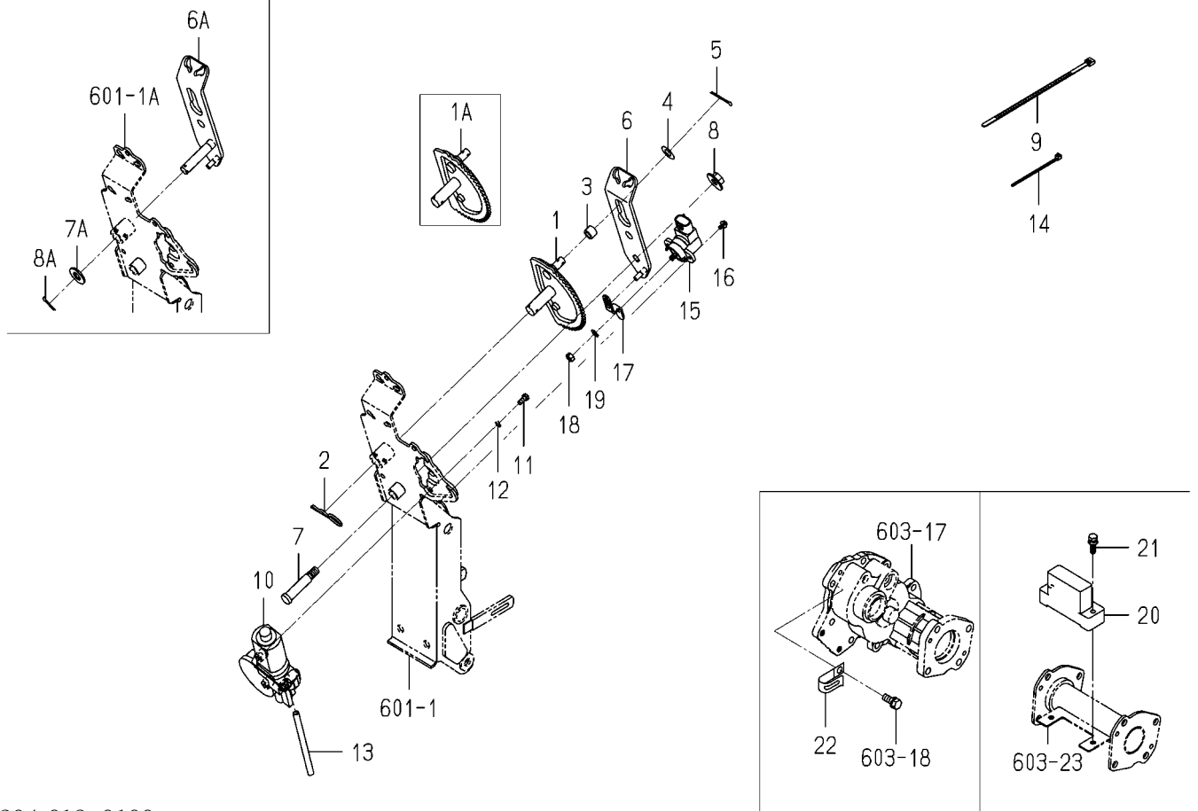
FIG.611 AUTOMATIC(ROLLING)SYSTEM
