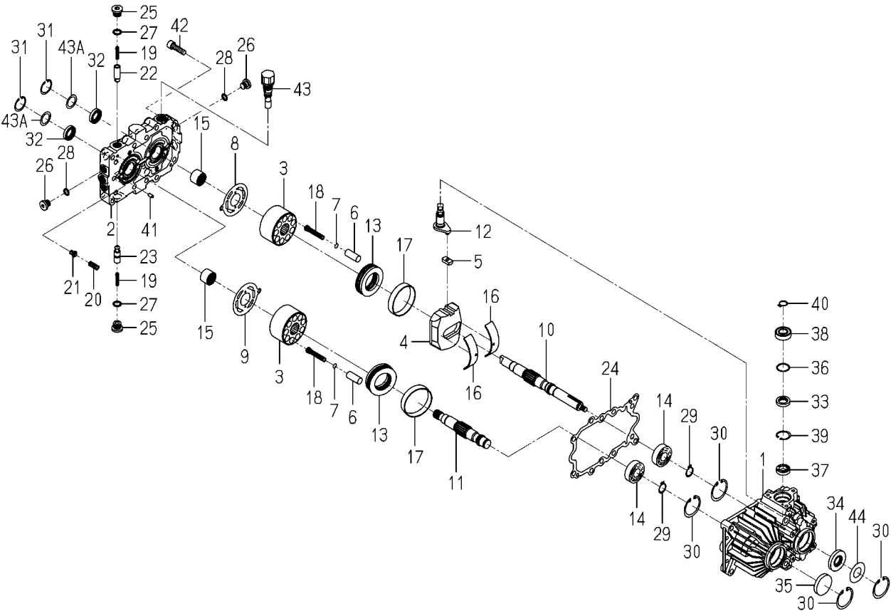
FIG.S02 COMPONENT PARTS FOR K510-013-000-40 ON Fig.108
