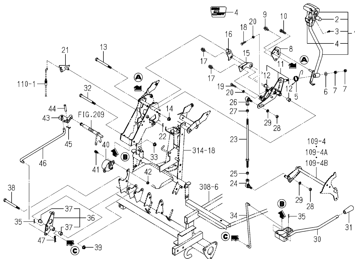
FIG.107 LEVER(HST)SYSTEM
