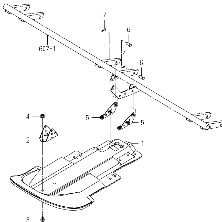
FIG.608 FLOAT(CENTER)SYSTEM(F TYPE)
