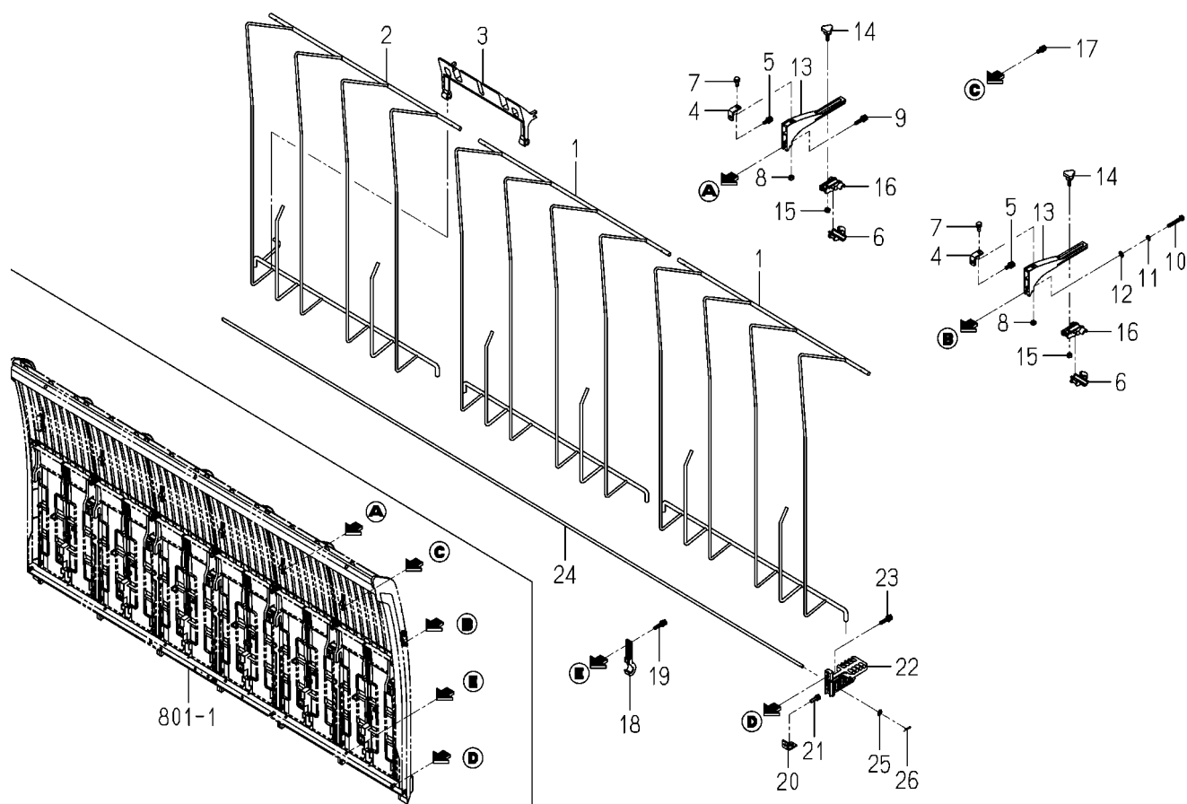
FIG.804 HOLDER(SEEDLING)SYSTEM
