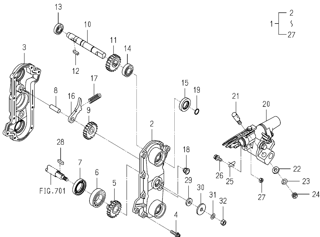
FIG.708 PLANTER(LH)SYSTEM
