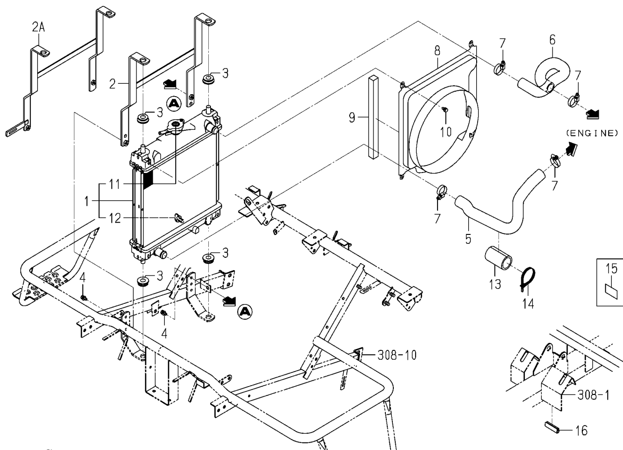
FIG.102 RADIATOR&CLEANER(AIR)SYSTEM
