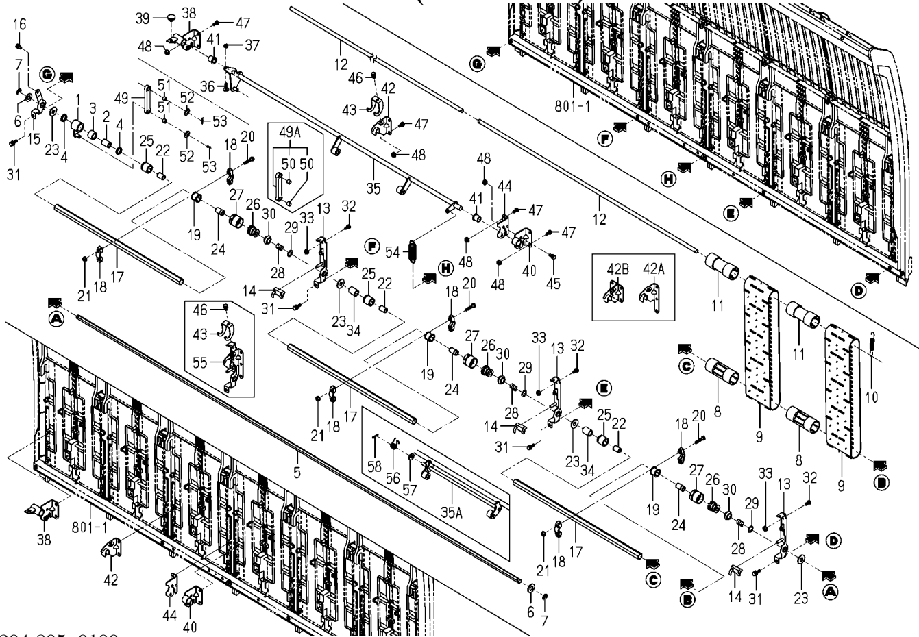
FIG.805 FEED(SEEDLING)SYSTEM
