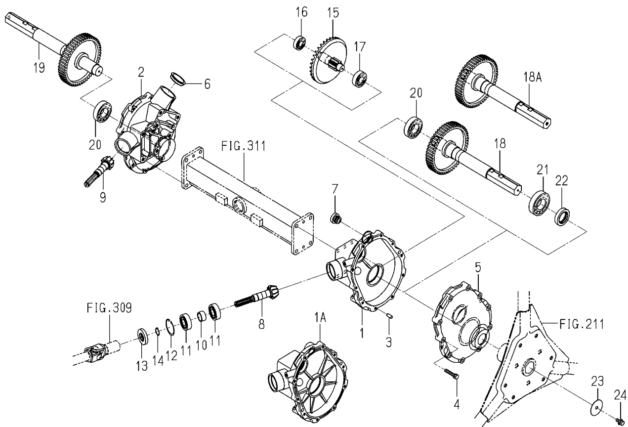
FIG.313 CASE(REAR)SYSTEM
