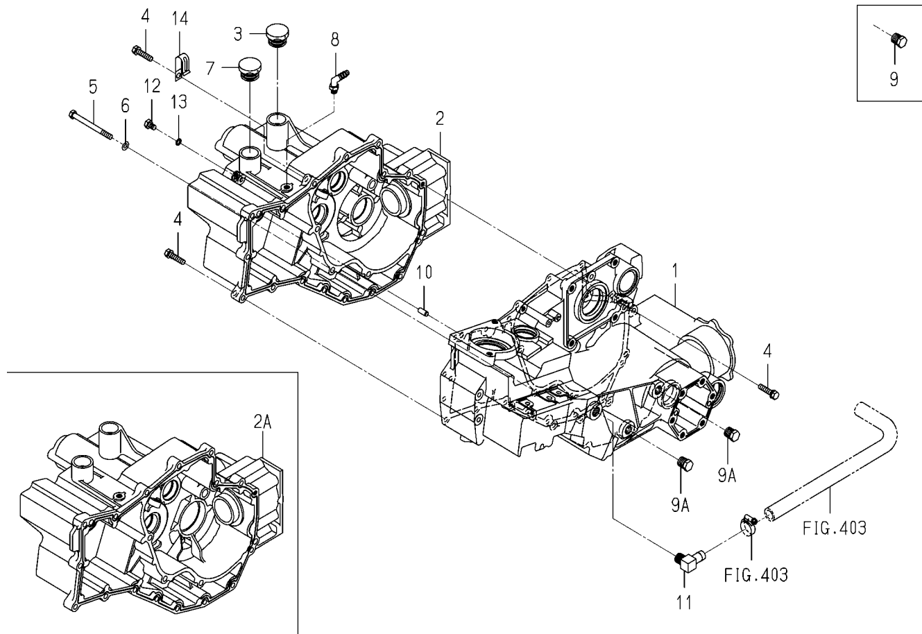
FIG.201 CASE(TRANSMISSION)SYSTEM
