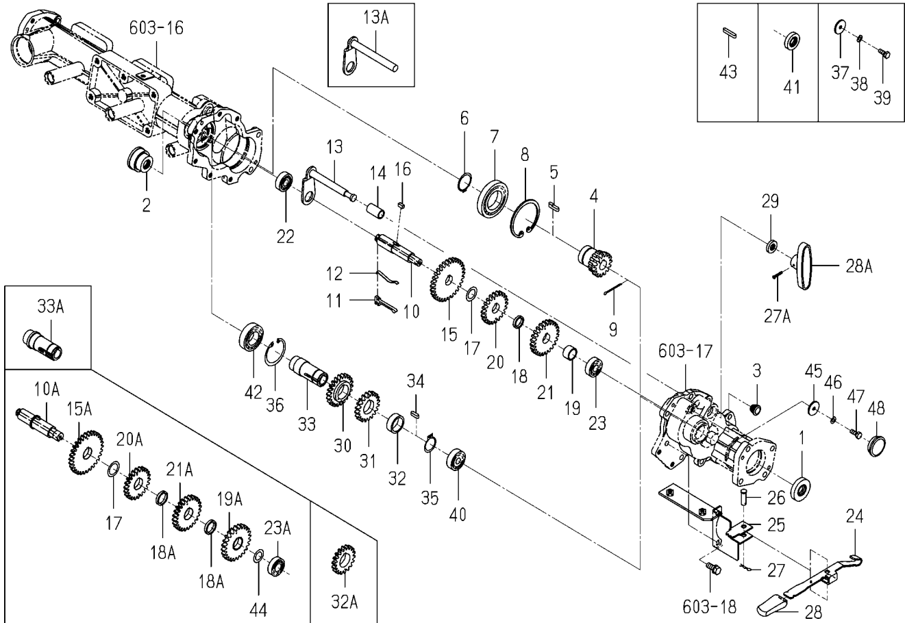
FIG.605 SLIDE SYSTEM
