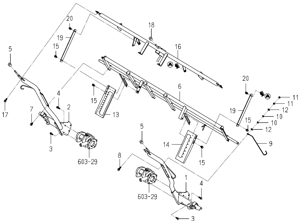
FIG.707 FRAME(TANK/SEEDLING)SYSTEM
