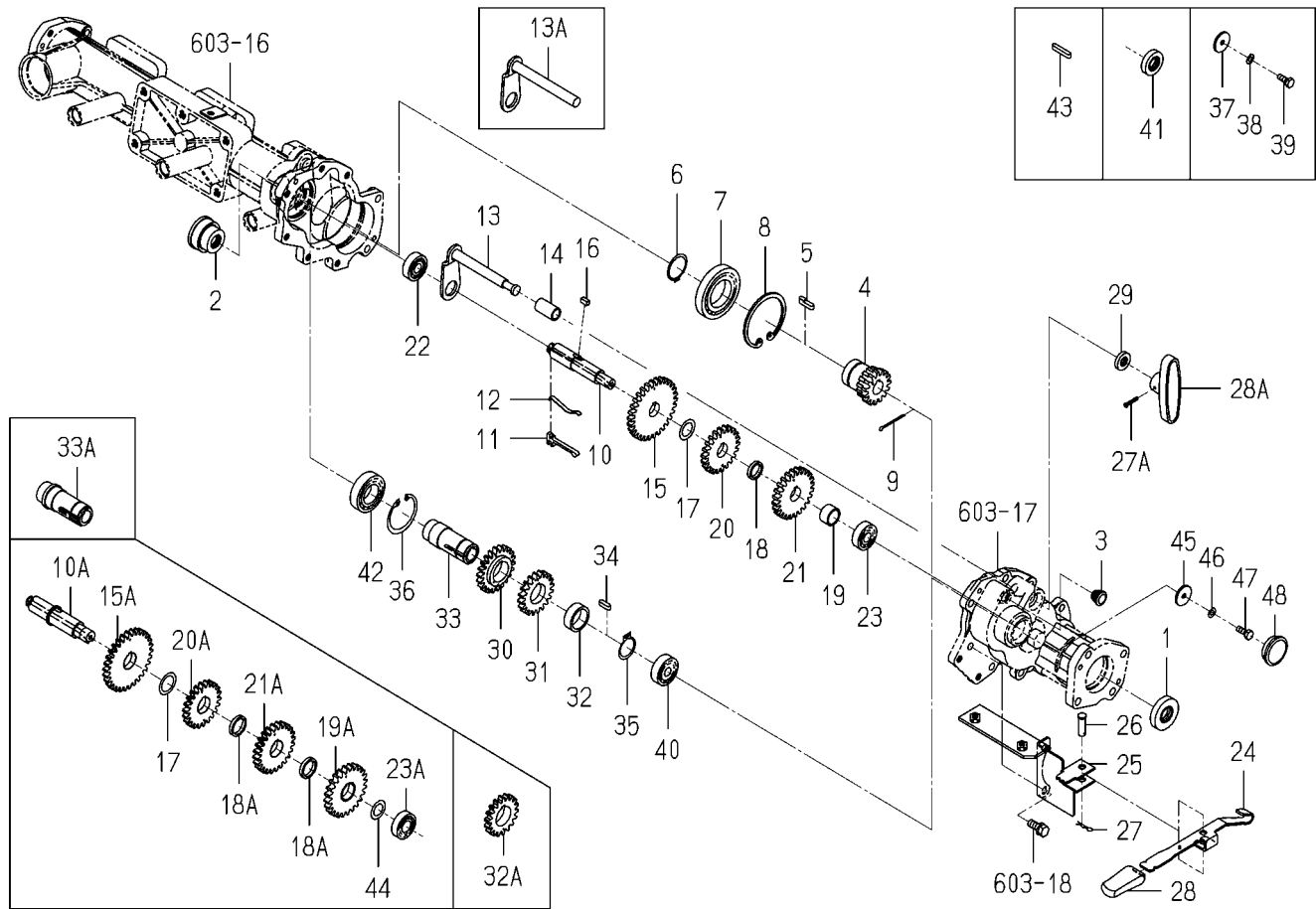
FIG.605 SLIDE SYSTEM
