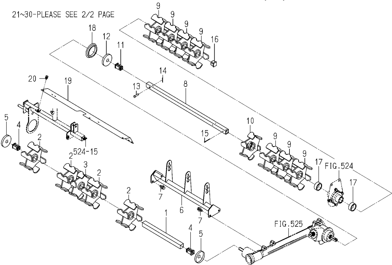
FIG.523 ROTOR SYSTEM(1/2)
