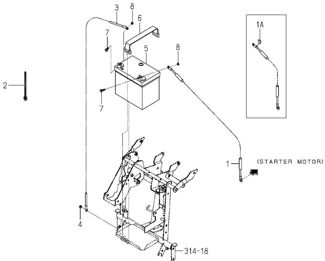
FIG.518 BATTERY SYSTEM
