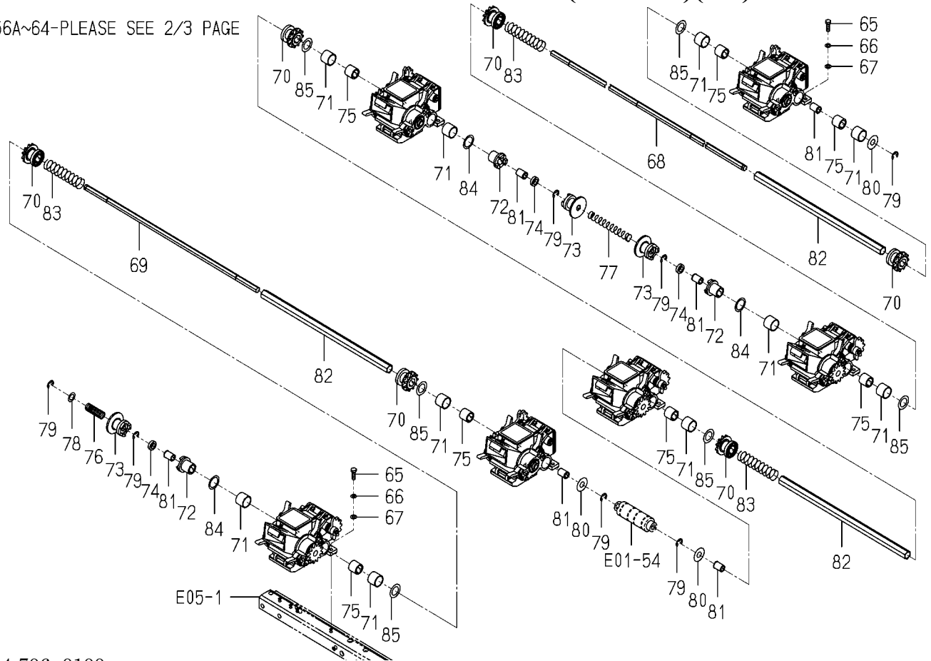
FIG.E08 OUT PUT SYSTEM(F TYPE)(3/3)
