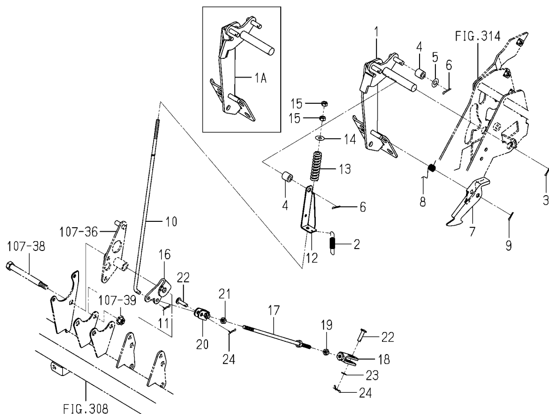
FIG.315 PEDAL SYSTEM
