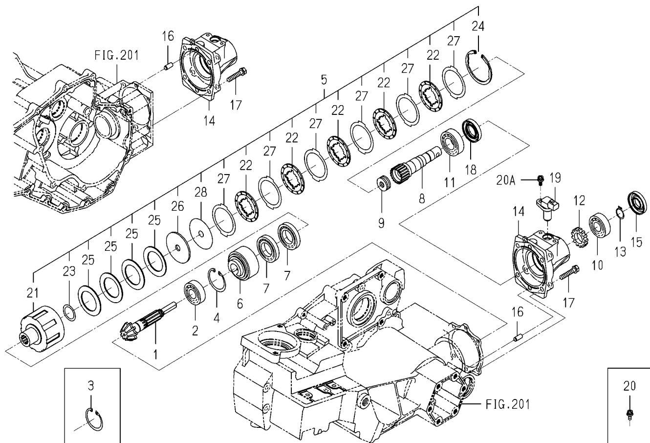
FIG.205 SHAFT(OUT PUT)SYSTEM
