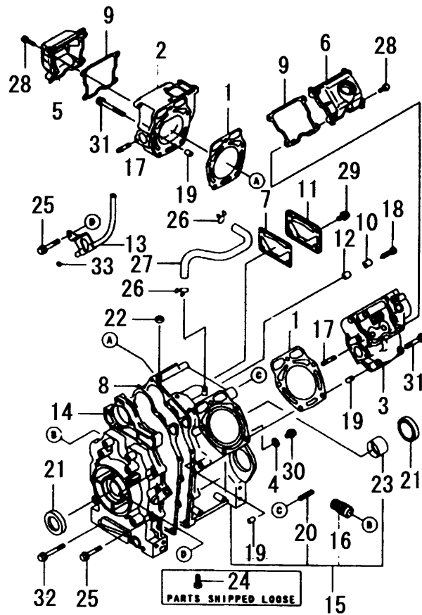
FIG. 1 CYLINDER/CRANKCASE
