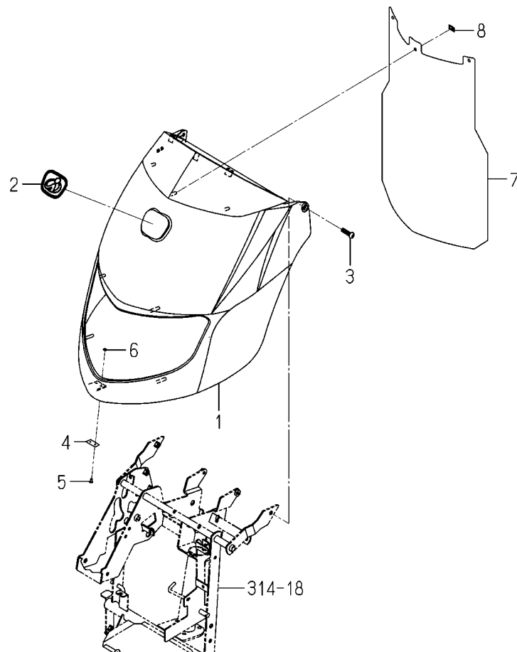
FIG.501 HOOD SYSTEM
