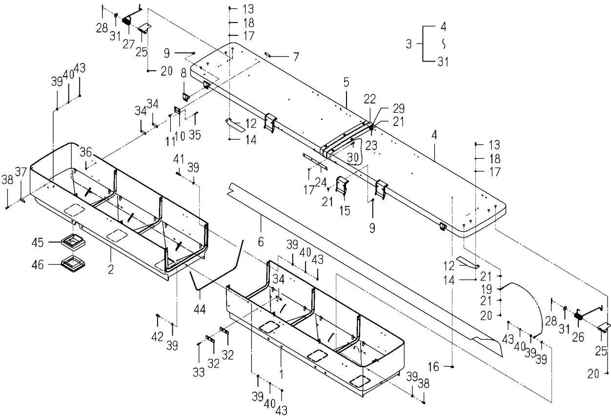
FIG.S05 COMPONENT PARTS FOR 8844-716-260-40 ON Fig.E09
