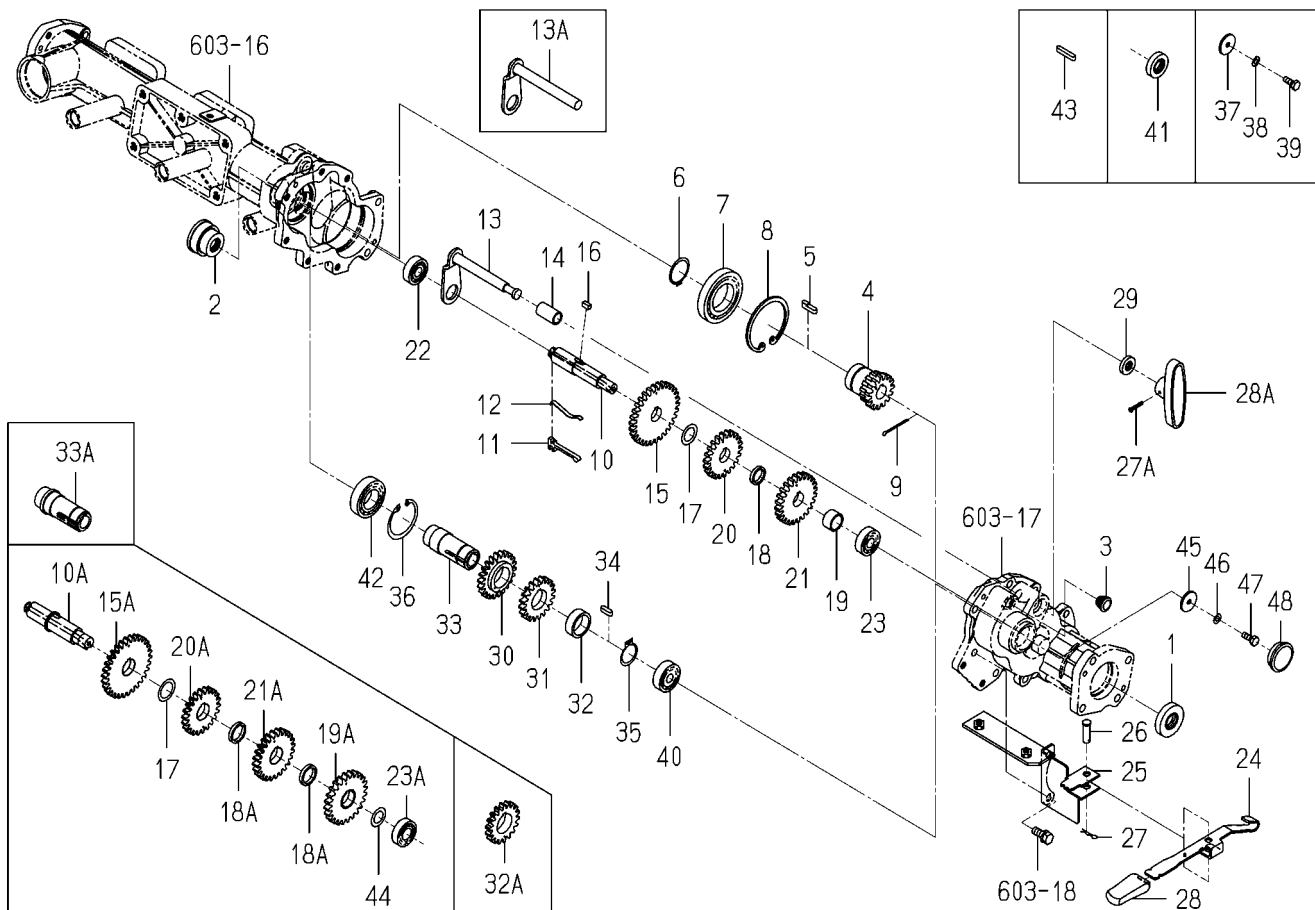
FIG.605 SLIDE SYSTEM
