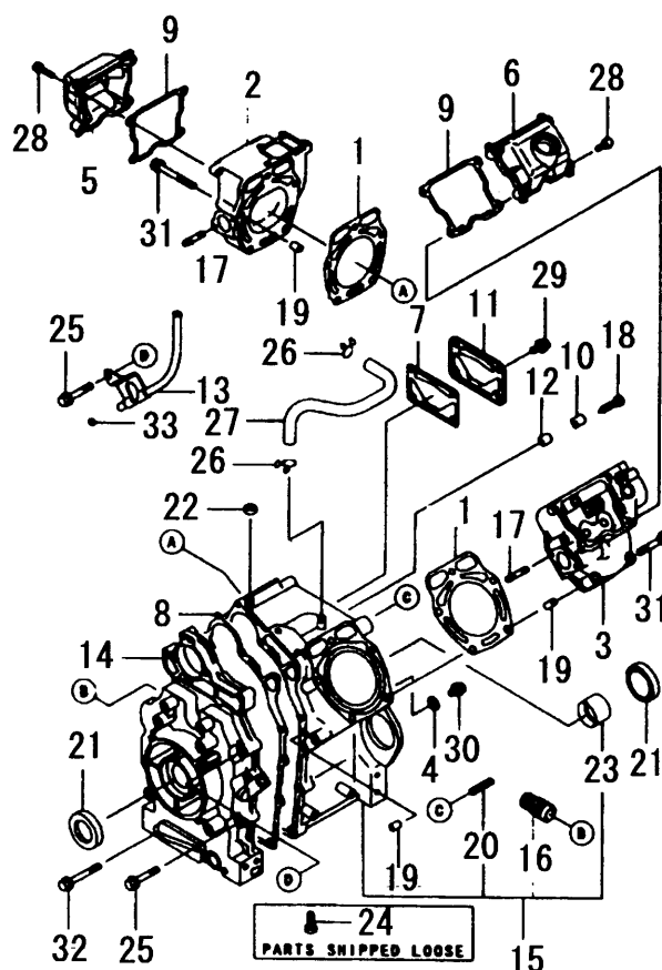
FIG. 1 CYLINDER/CRANKCASE
