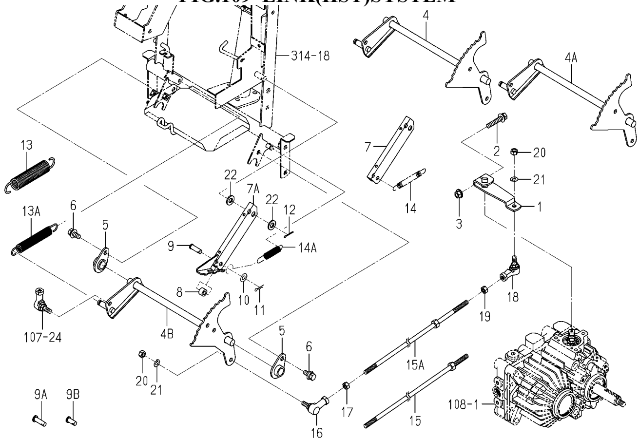
FIG.109 LINK(HST)SYSTEM
