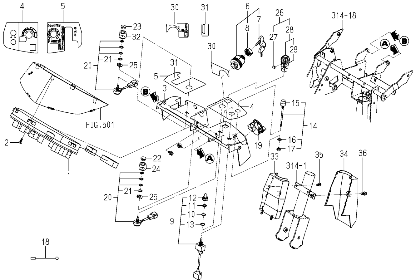
FIG.514 PANEL(MONITOR)SYSTEM
