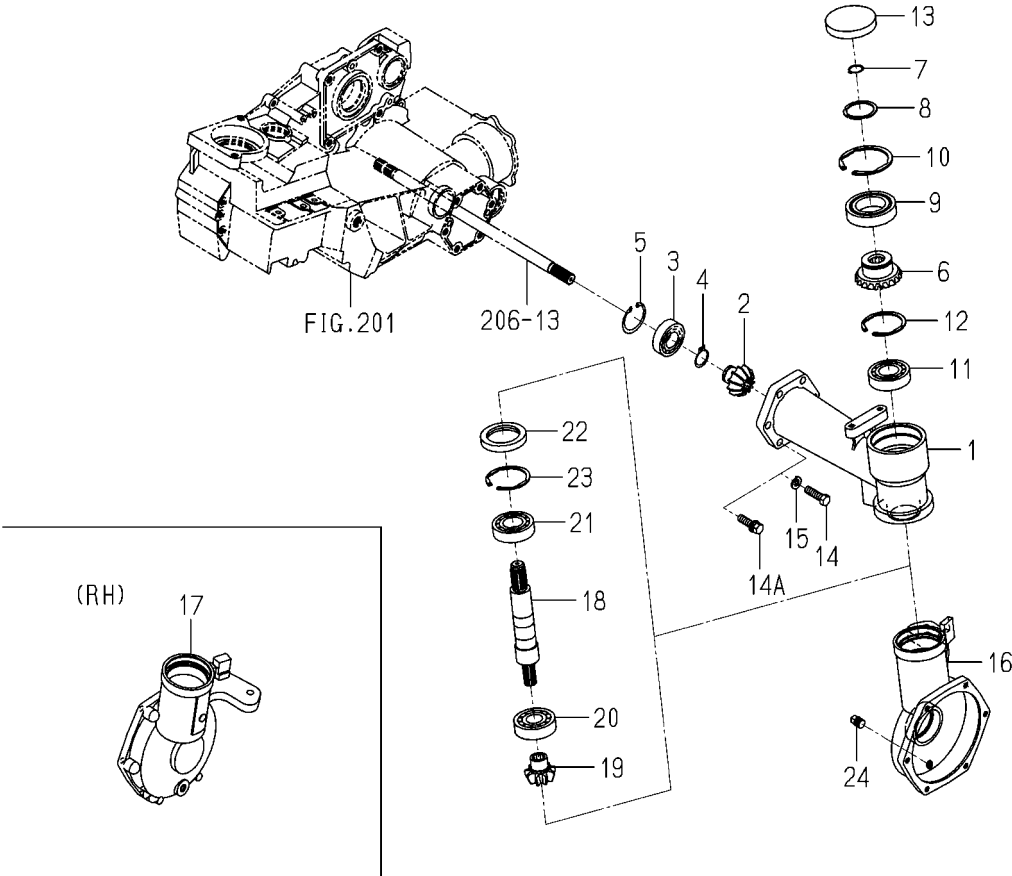
FIG.304 CASE(FINAL)SYSTEM
