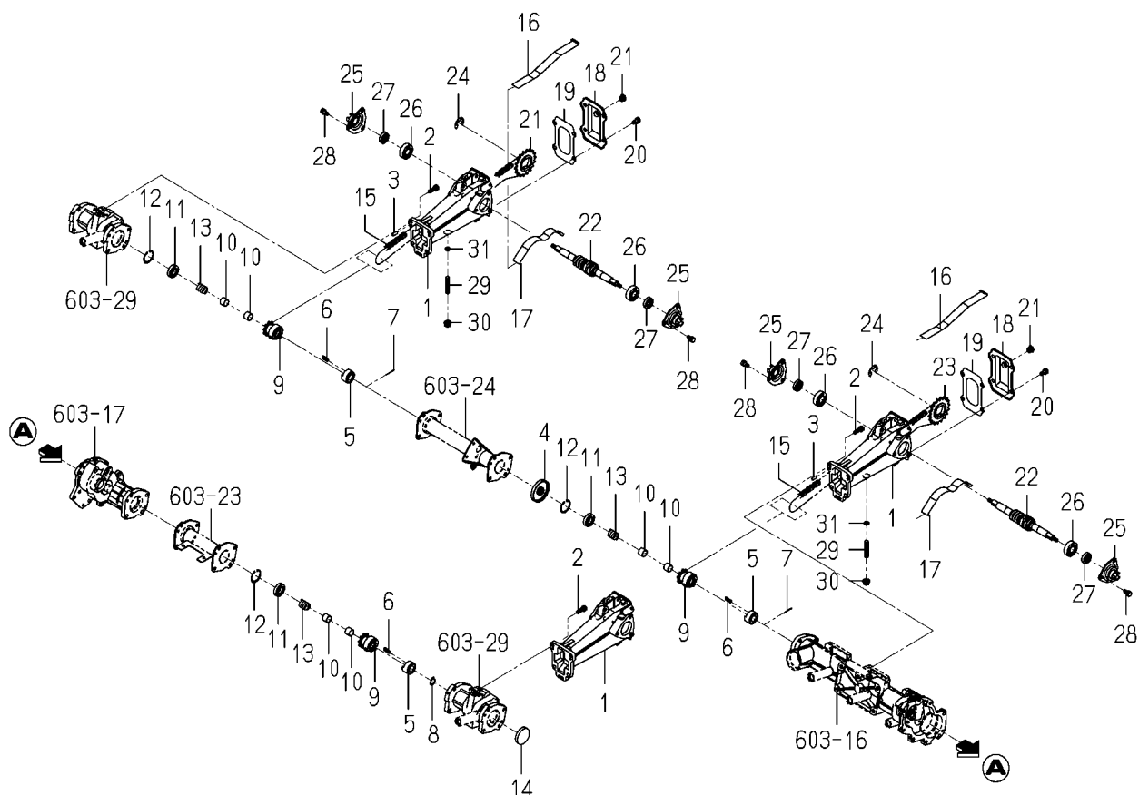
FIG.701 FRAME(SIDE)SYSTEM
