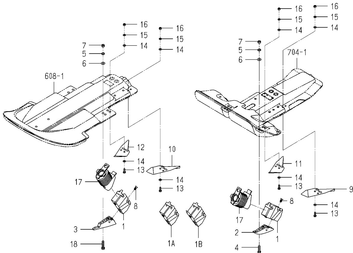
FIG.E12 DITCHER SYSTEM(F TYPE)
