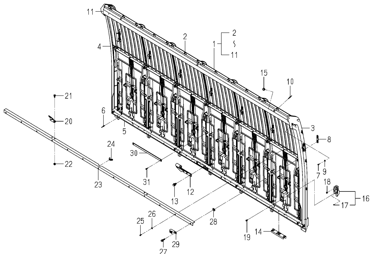
FIG.801 TANK(SEEDLING)SYSTEM
