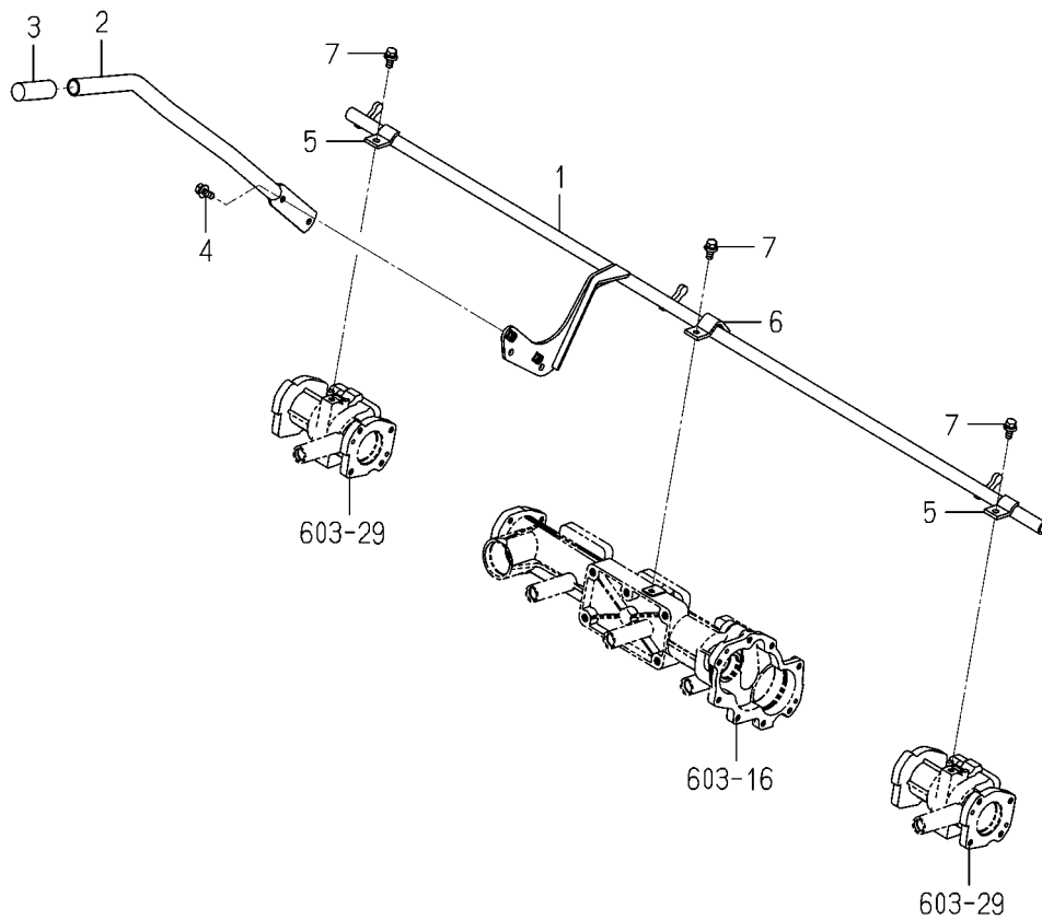
FIG.703 LEVER(PICKING/SEEDLING)SYSTEM
