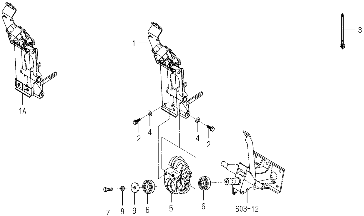
FIG.601 LIFT SYSTEM
