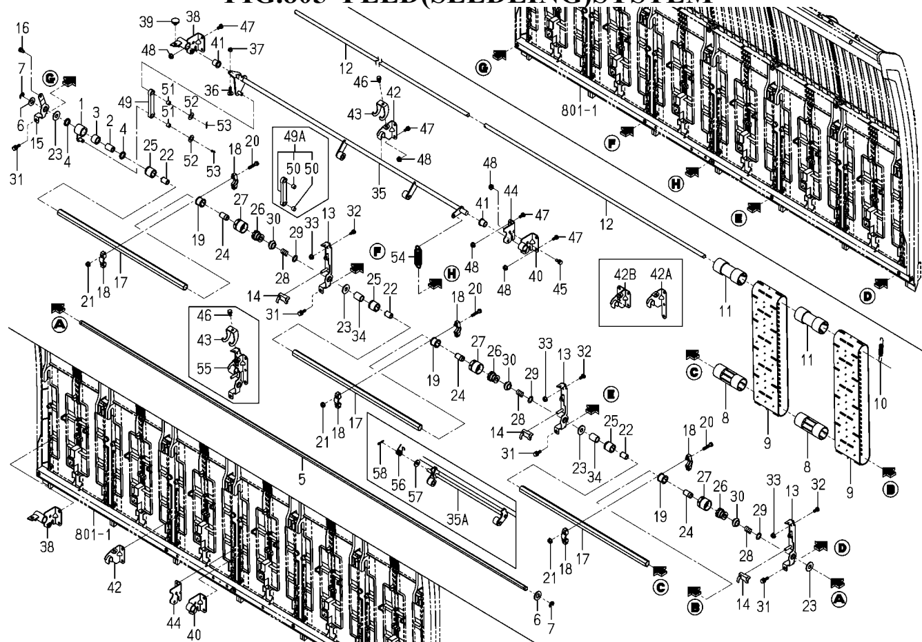
FIG.805 FEED(SEEDLING)SYSTEM
