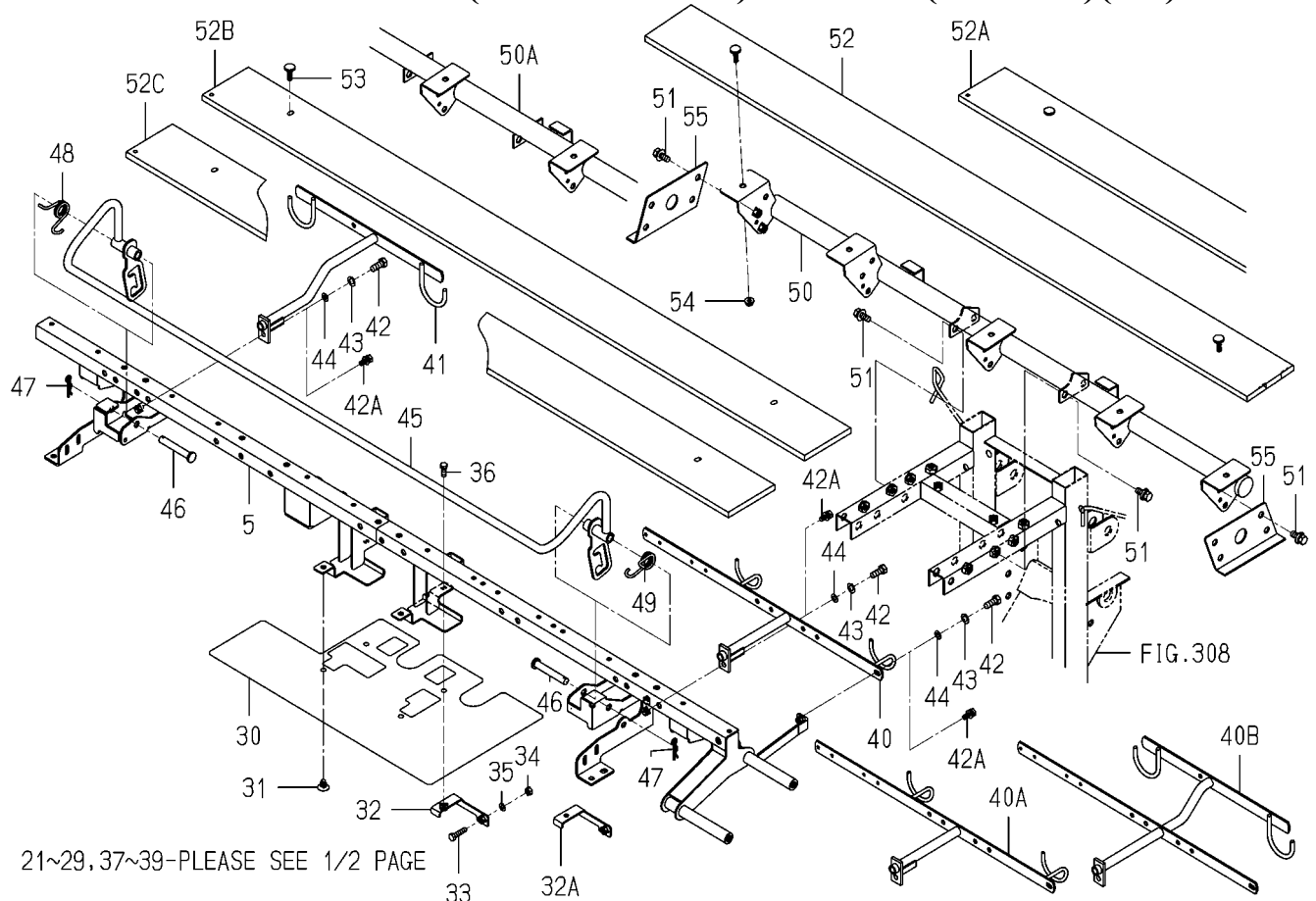
FIG.E06 FRAME(FERTILIZER)SYSTEM(F TYPE)(2/2)
