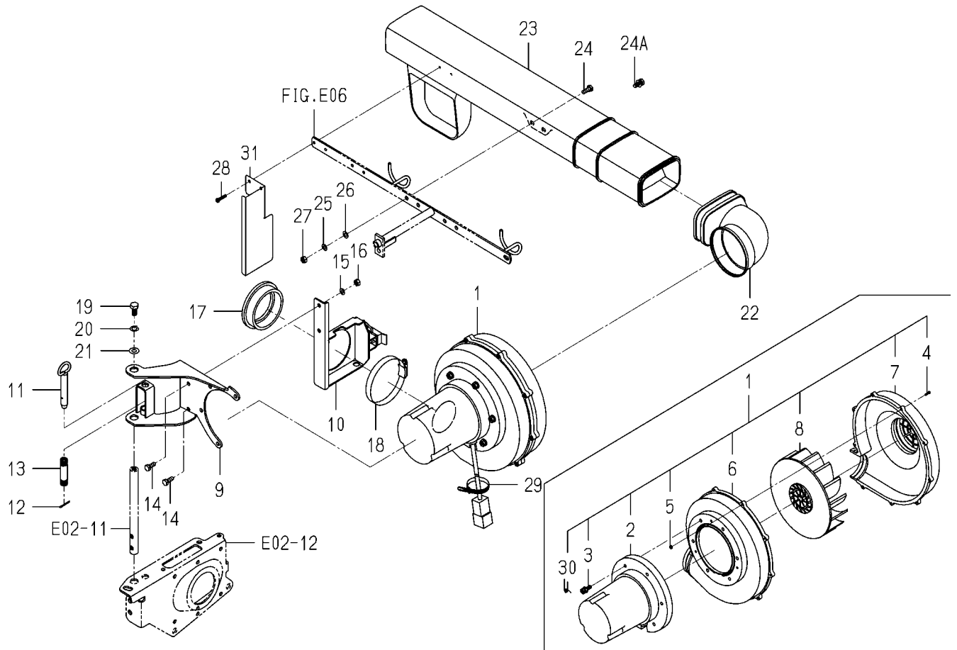
FIG.E07 BLOWER SYSTEM(F TYPE)
