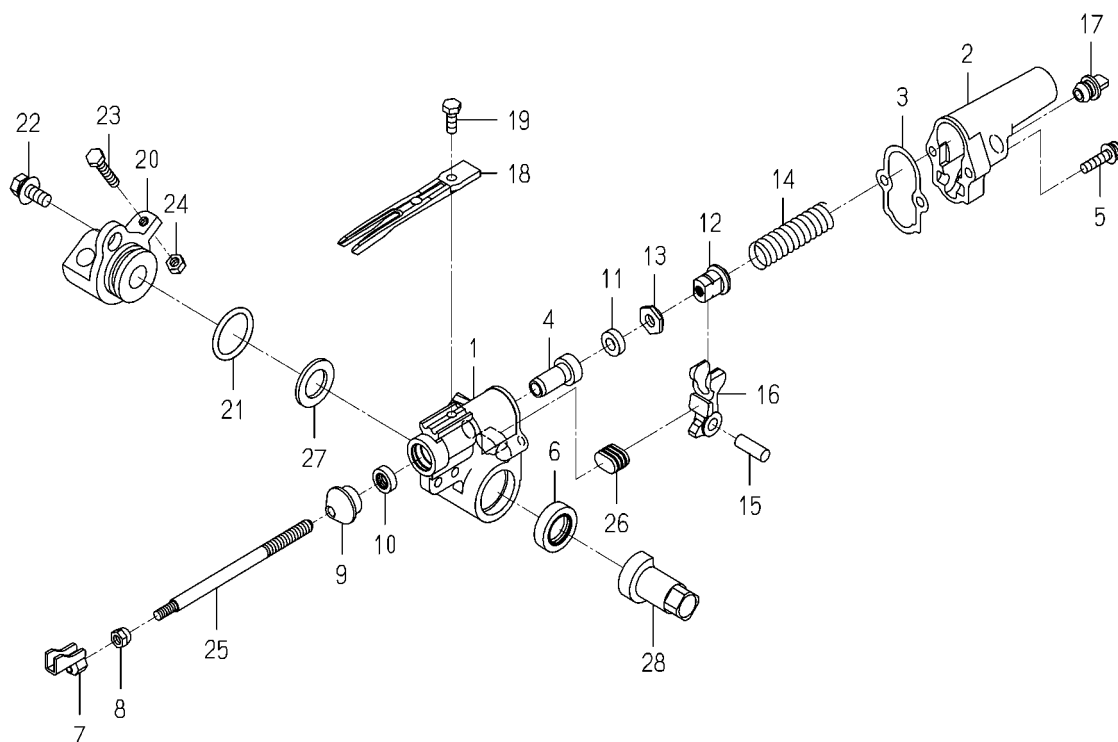
FIG.S04 COMPONENT PARTS FOR 2204-739-410-70 ON Fig.709
