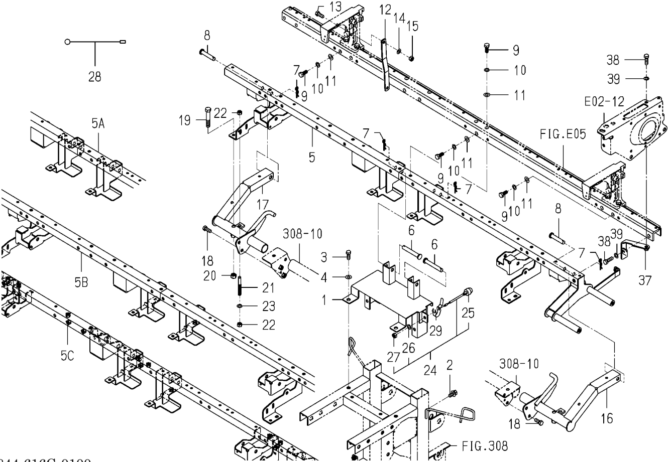
FIG.E06 FRAME(FERTILIZER)SYSTEM(F TYPE)(1/2)
