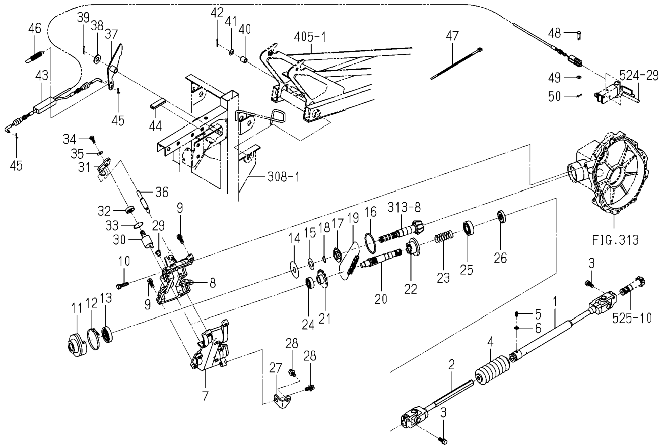
FIG.522 DRIVE(ROTOR)SYSTEM
