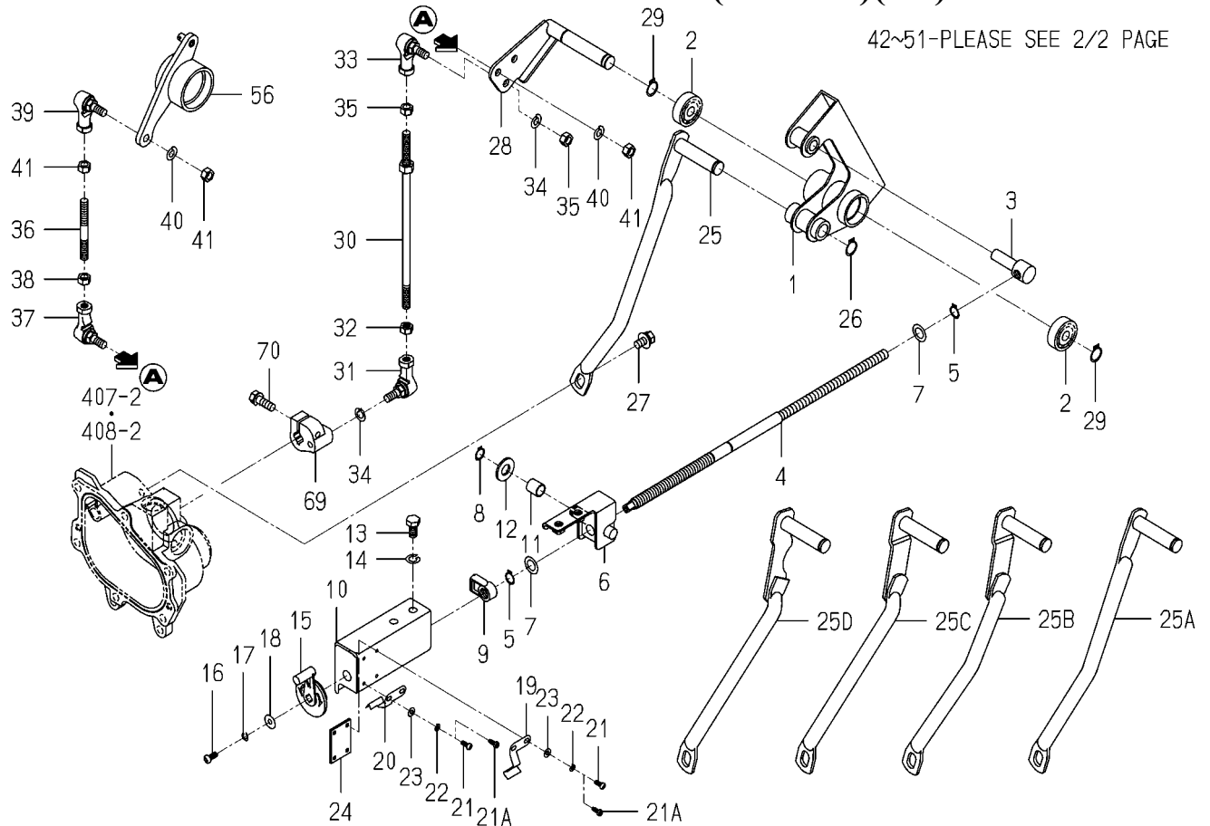
FIG.E01 DRIVE SYSTEM(F TYPE)(1/2)
