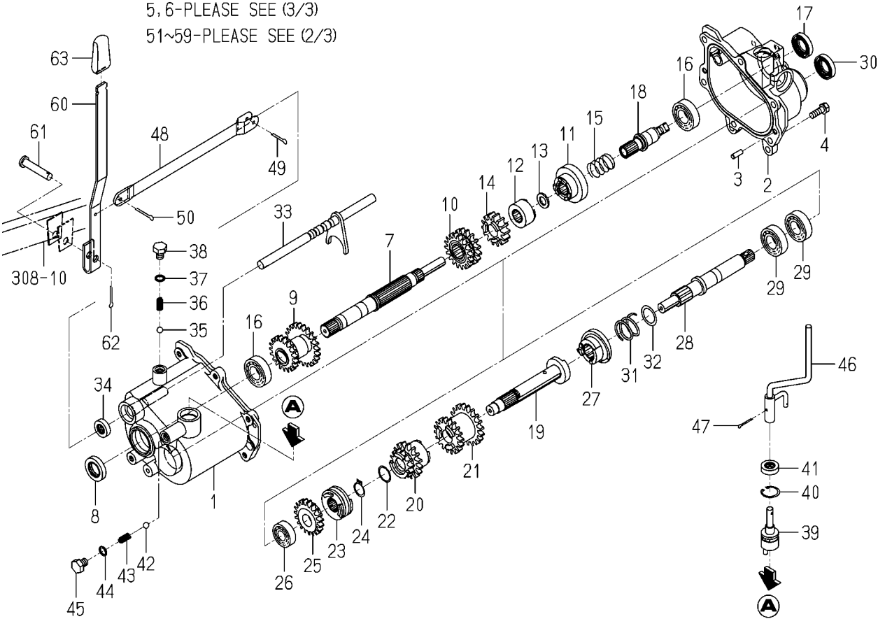
FIG.407 CASE(PLANTING)SYSTEM(F TYPE)(1/3)
