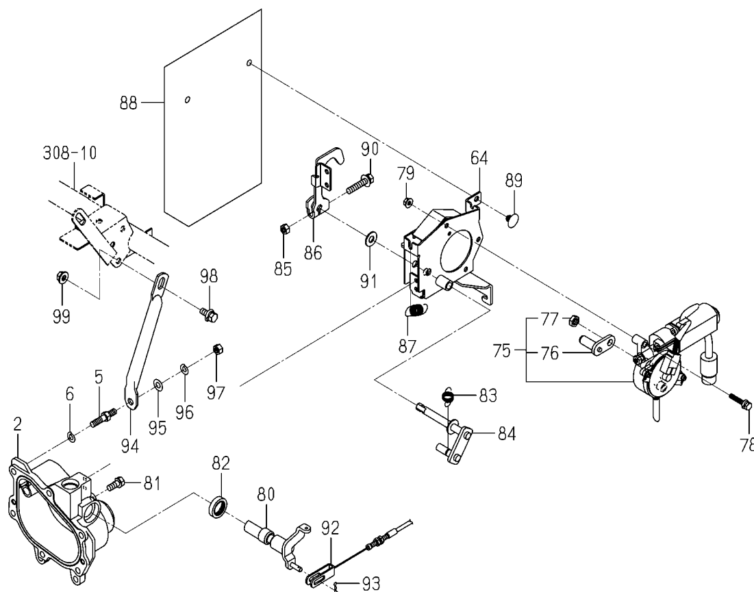
FIG.407 CASE(PLANTING)SYSTEM(F TYPE)(3/3)
