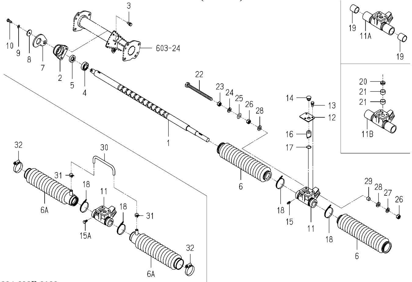
FIG.606 CAM(LEAD)SYSTEM
