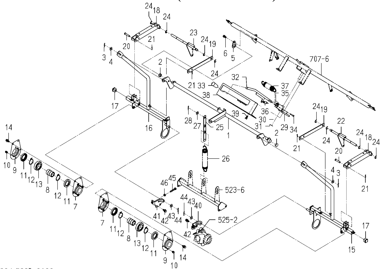
FIG.524 CONTROL(DEPTH/ROTOR)SYSTEM
