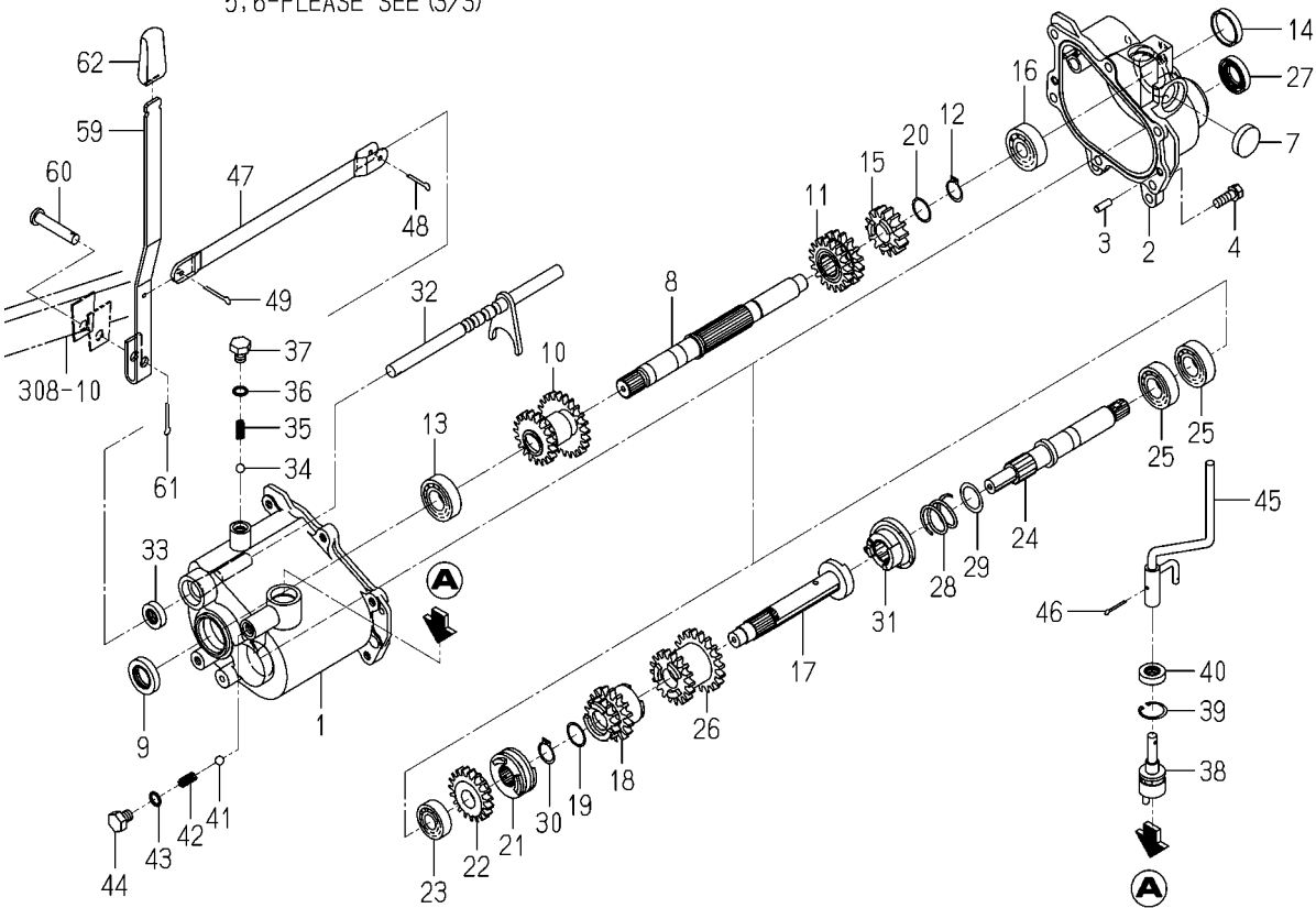
FIG.408 CASE(PLANTING)SYSTEM(1/3) (EXCEPT F TYPE)
