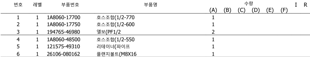
(A)=YT490AY,KR (B)=YT5101AY,KR (C)=YT5113AY,KR
