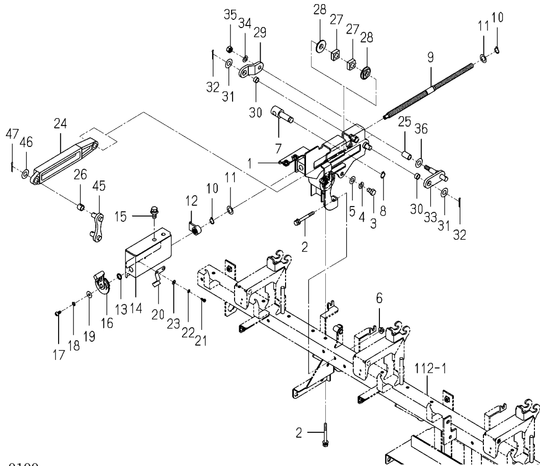
FIG.108 DRIVE(FERTILIZER)SYSTEM(F TYPE)(1/2)
