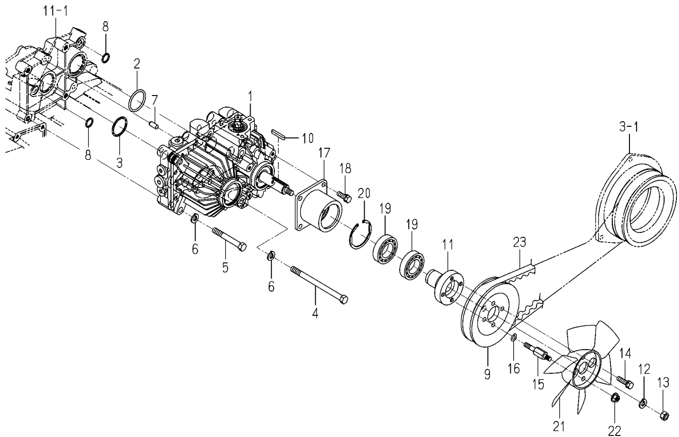
FIG. 8 HST SYSTEM
