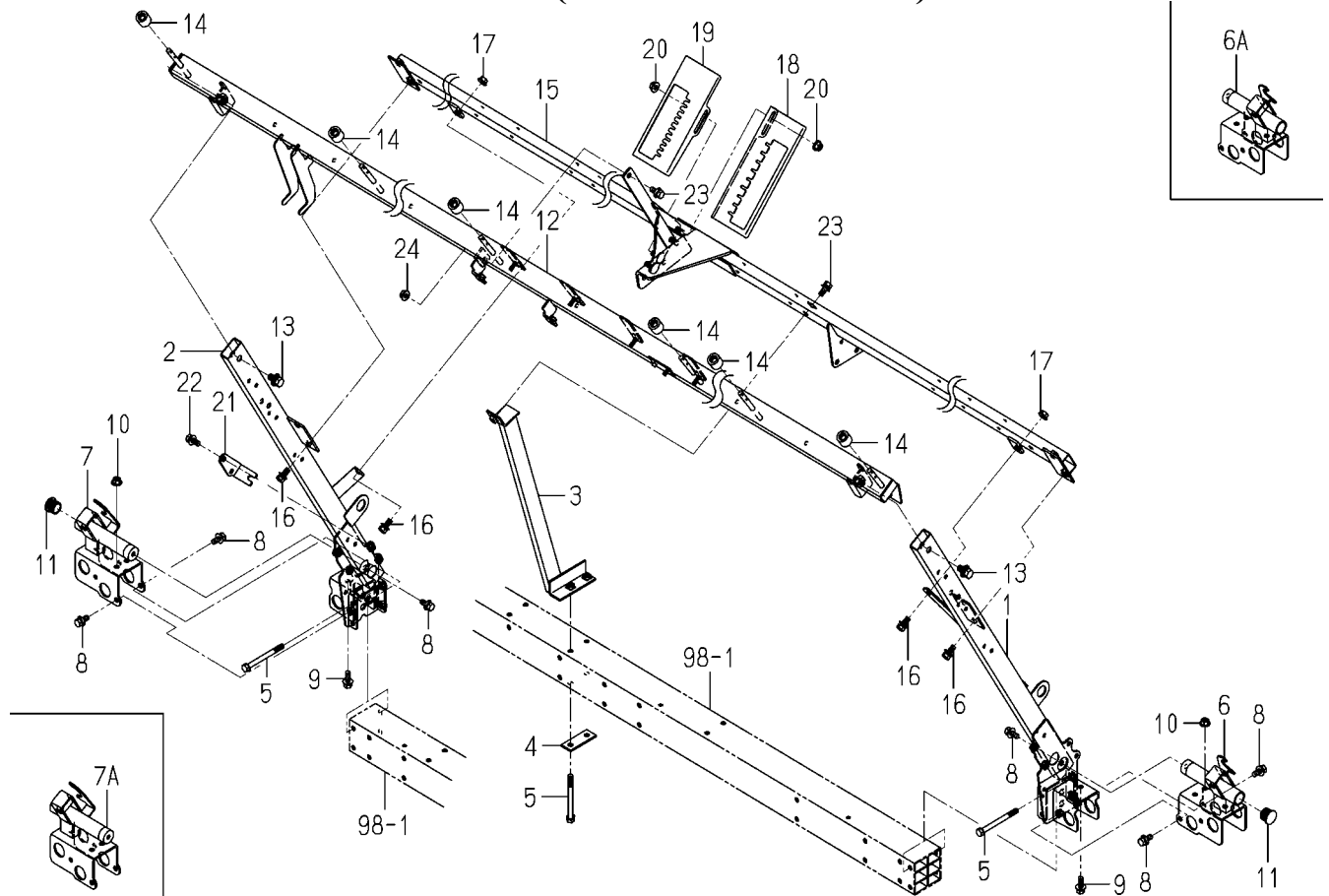
FIG.119 FRAME(TANK/SEEDLING)SYSTEM
