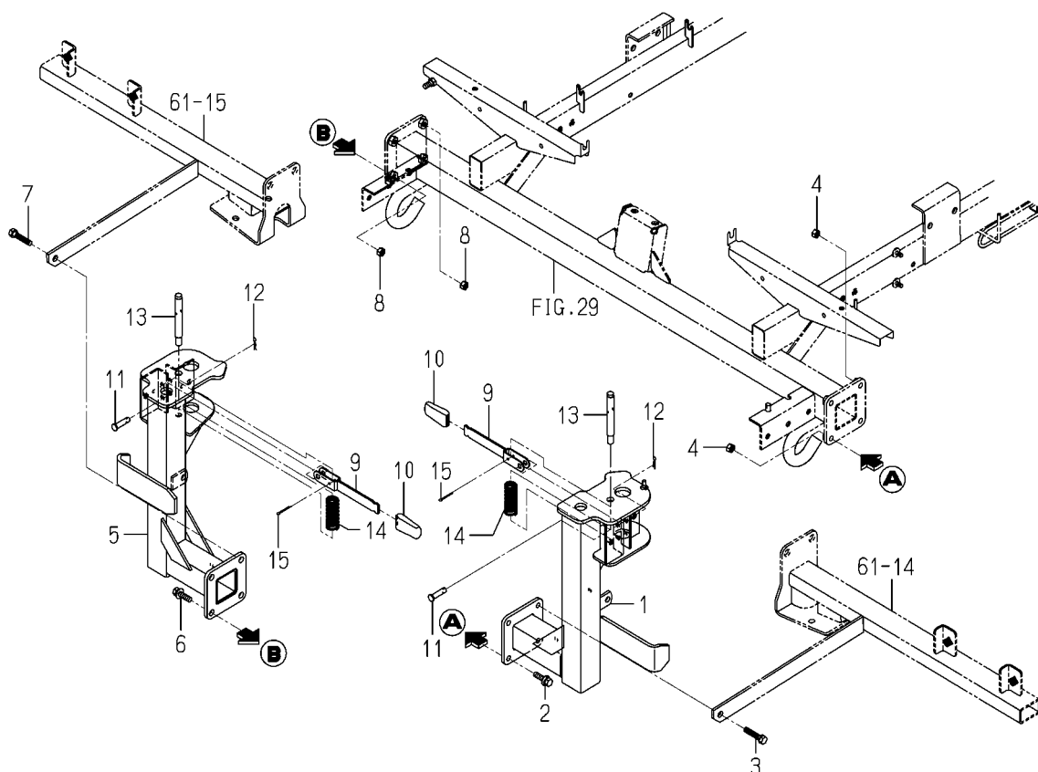
FIG. 71 STAY(FRAME/SEEDLING/SUB)SYSTEM (ZRF TYPE)
