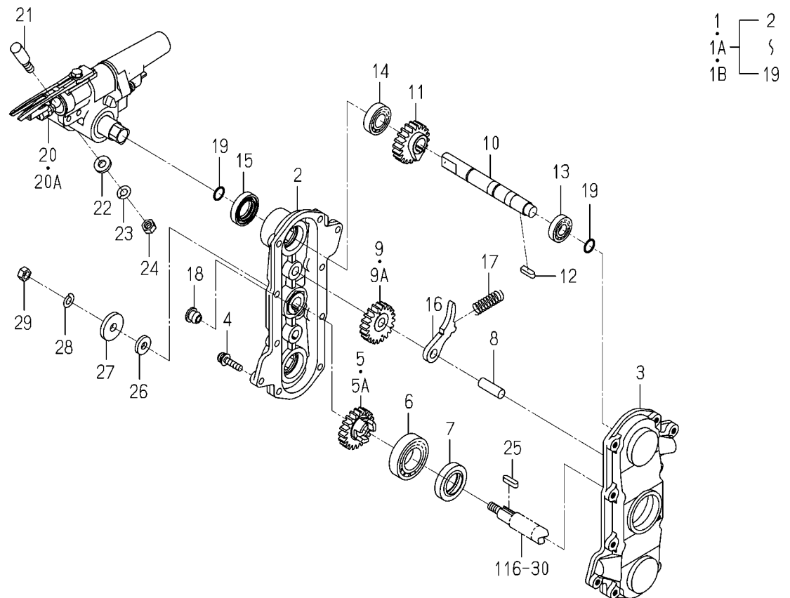
FIG.125 PLANTER(RH)SYSTEM
