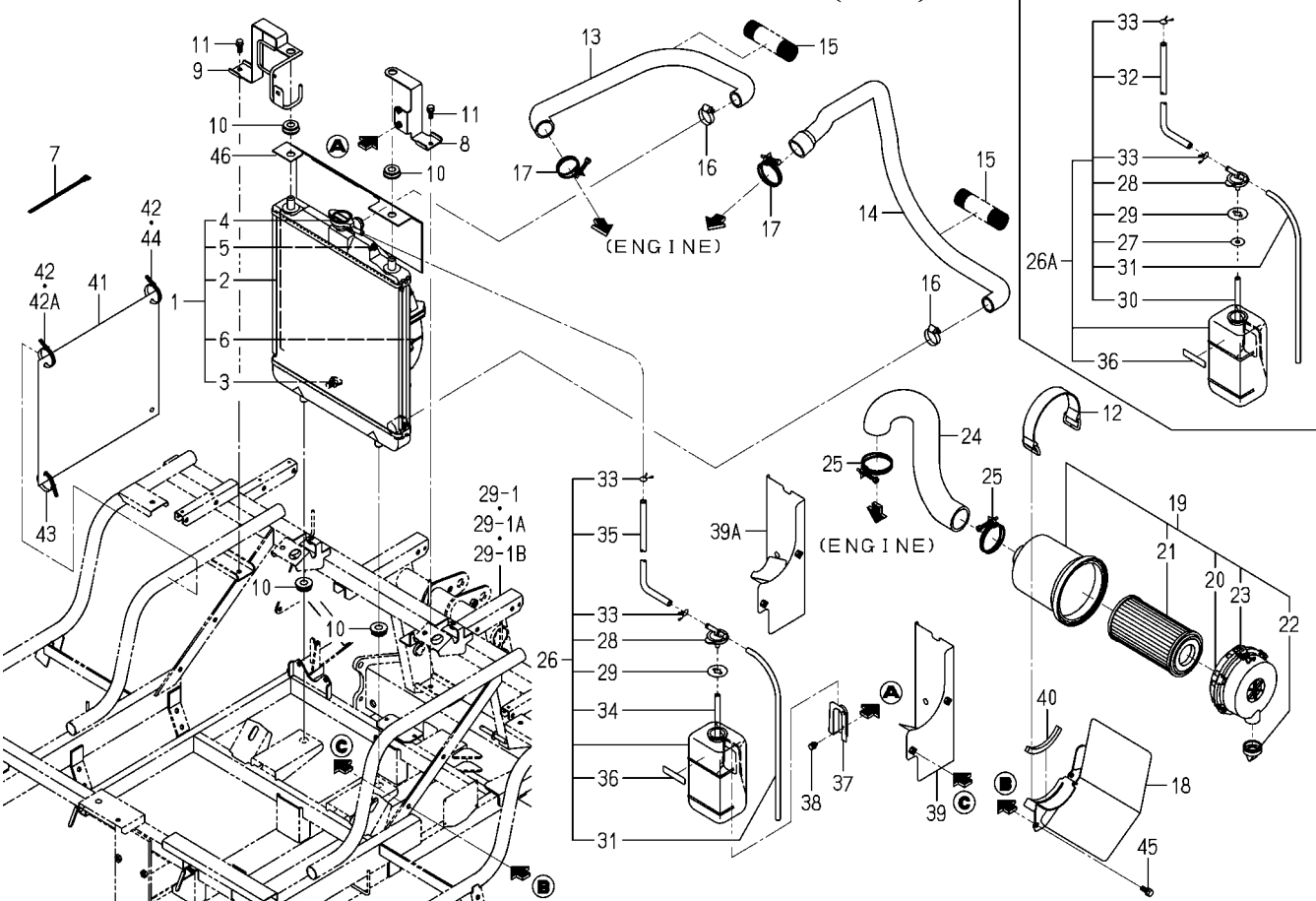
FIG. 2 RADIATOR&CLEANER(AIR)SYSTEM
