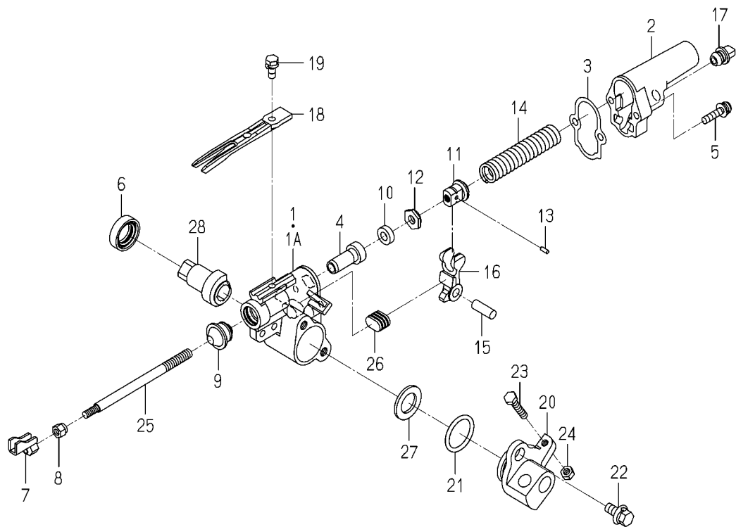
FIG.154 COMPONENT PARTS FOR 2204-738-450-30 ON Fig.124
