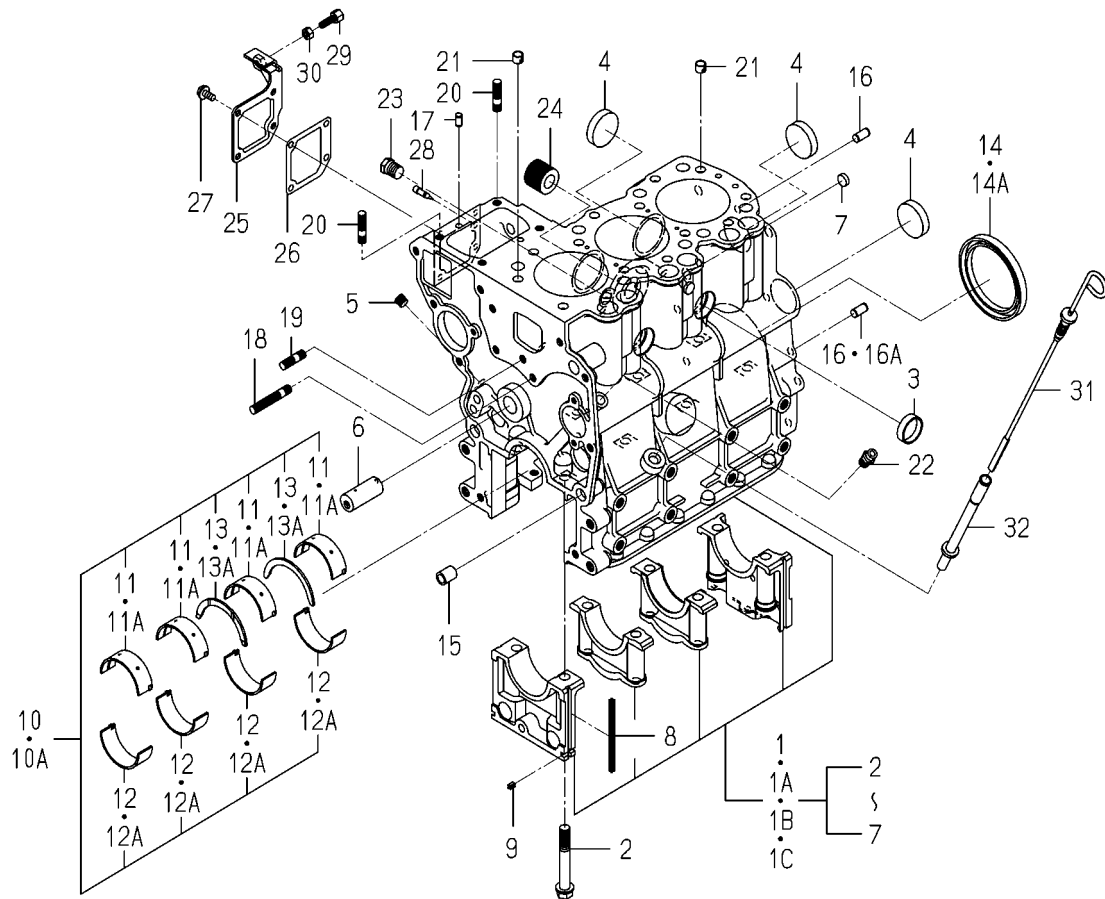
FIG. 5 CYLINDER BLOCK
