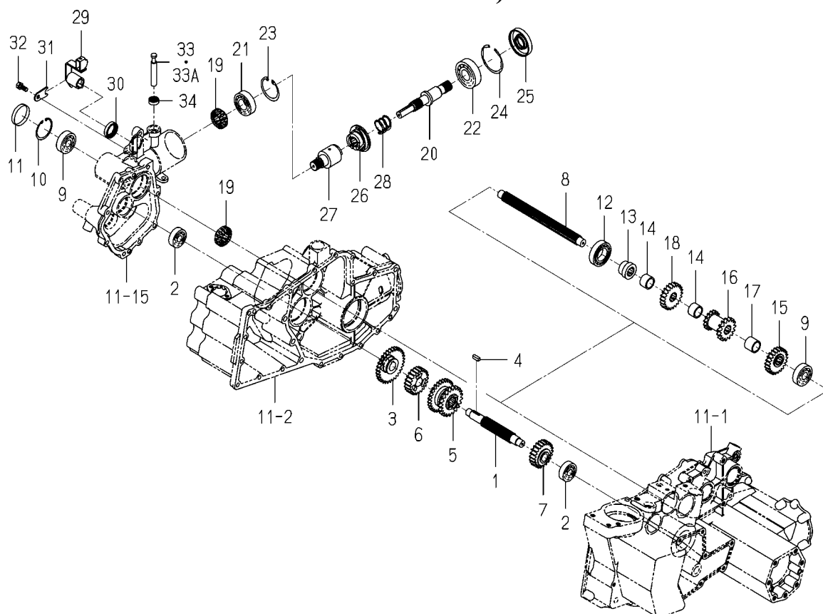
FIG. 18 SHAFT(PLANTING INTERVAL, PLANTING/OUTPUT)SYSTEM
