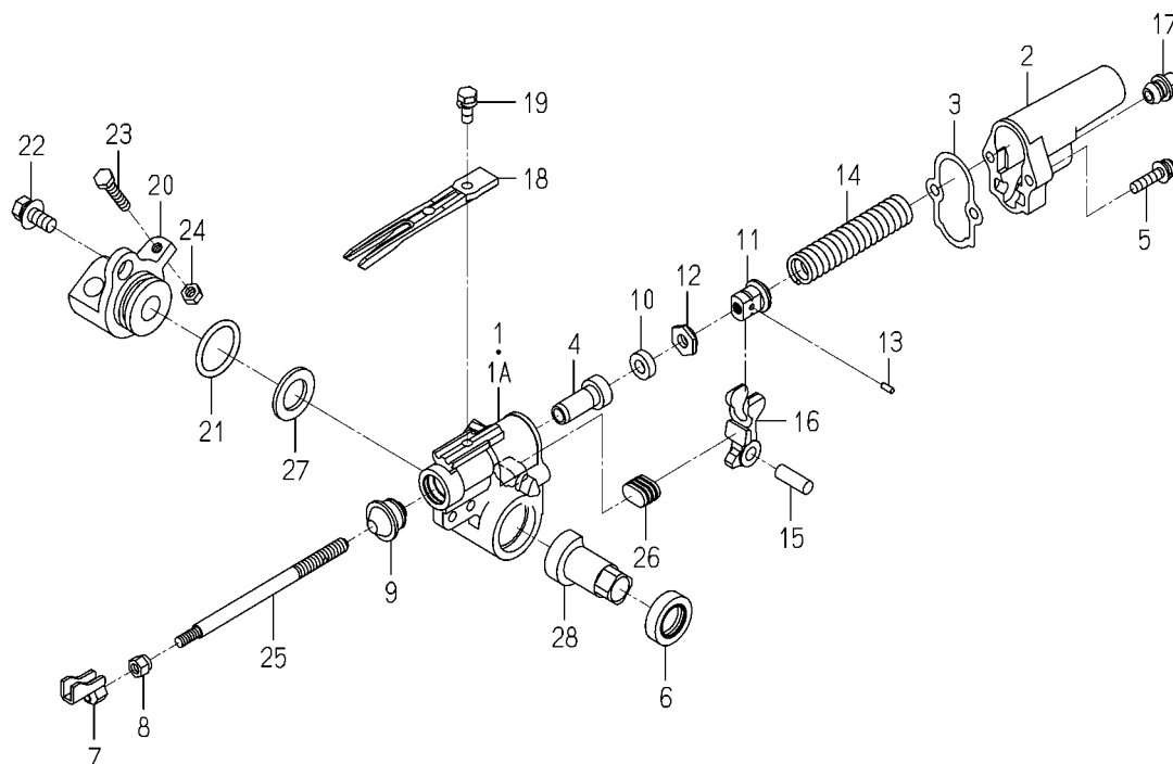
FIG.155 COMPONENT PARTS FOR 2204-739-450-30 ON Fig.125
