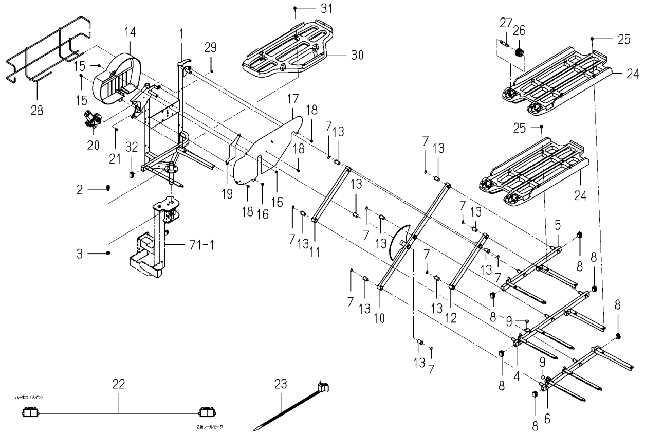
FIG. 67 TRAY(SEEDLING/SUB)SYSTEM(1/3) (RF TYPE EXCEPT Z)
