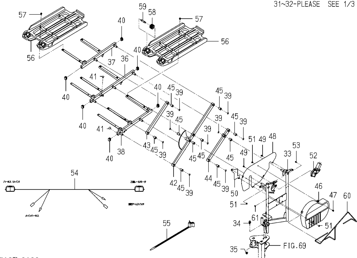
FIG. 67 TRAY(SEEDLING/SUB)SYSTEM(2/3) (RF TYPE EXCEPT Z)
