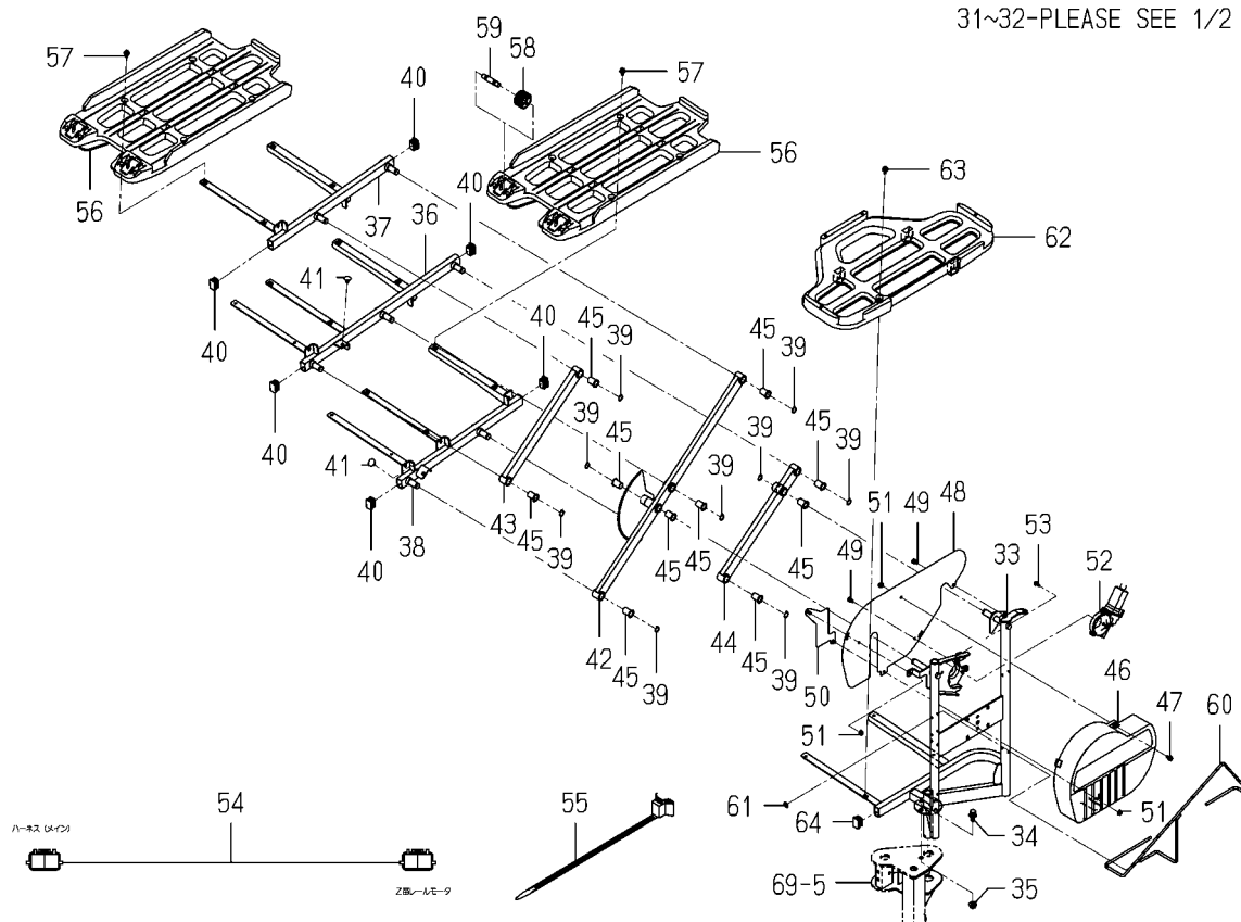
FIG. 64 TRAY(SEEDLING/SUB)SYSTEM(2/2) (R TYPE EXCEPT F)
