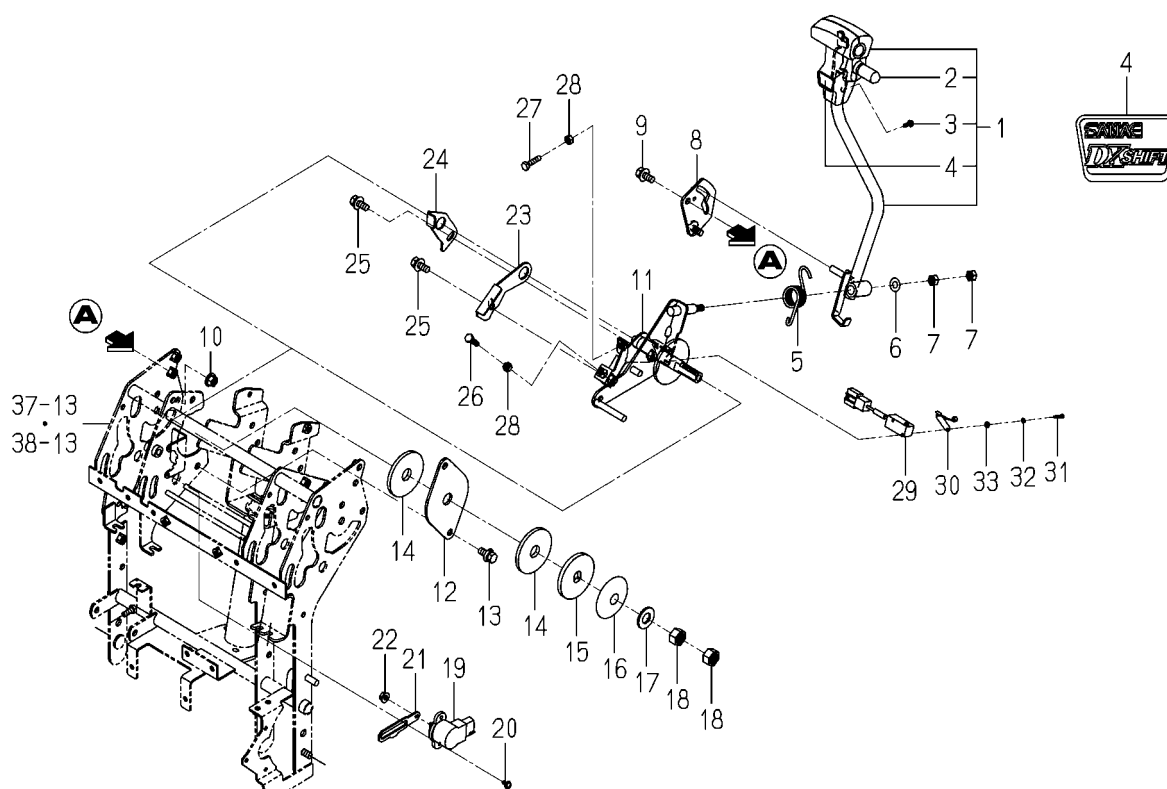
FIG. 6 LEVER(MAIN)SYSTEM
