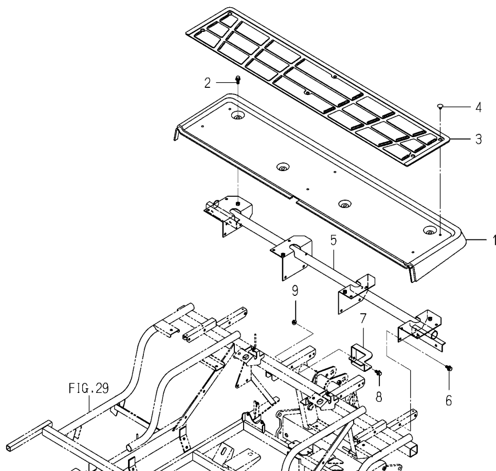
FIG. 62 STEP( REAR)SYSTEM( EXCEPT F TYPE)
