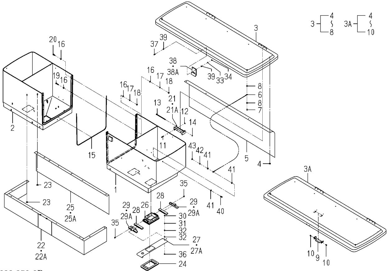
FIG.157 COMPONENT PARTS FOR 2233-688-250-90 ON Fig.114
