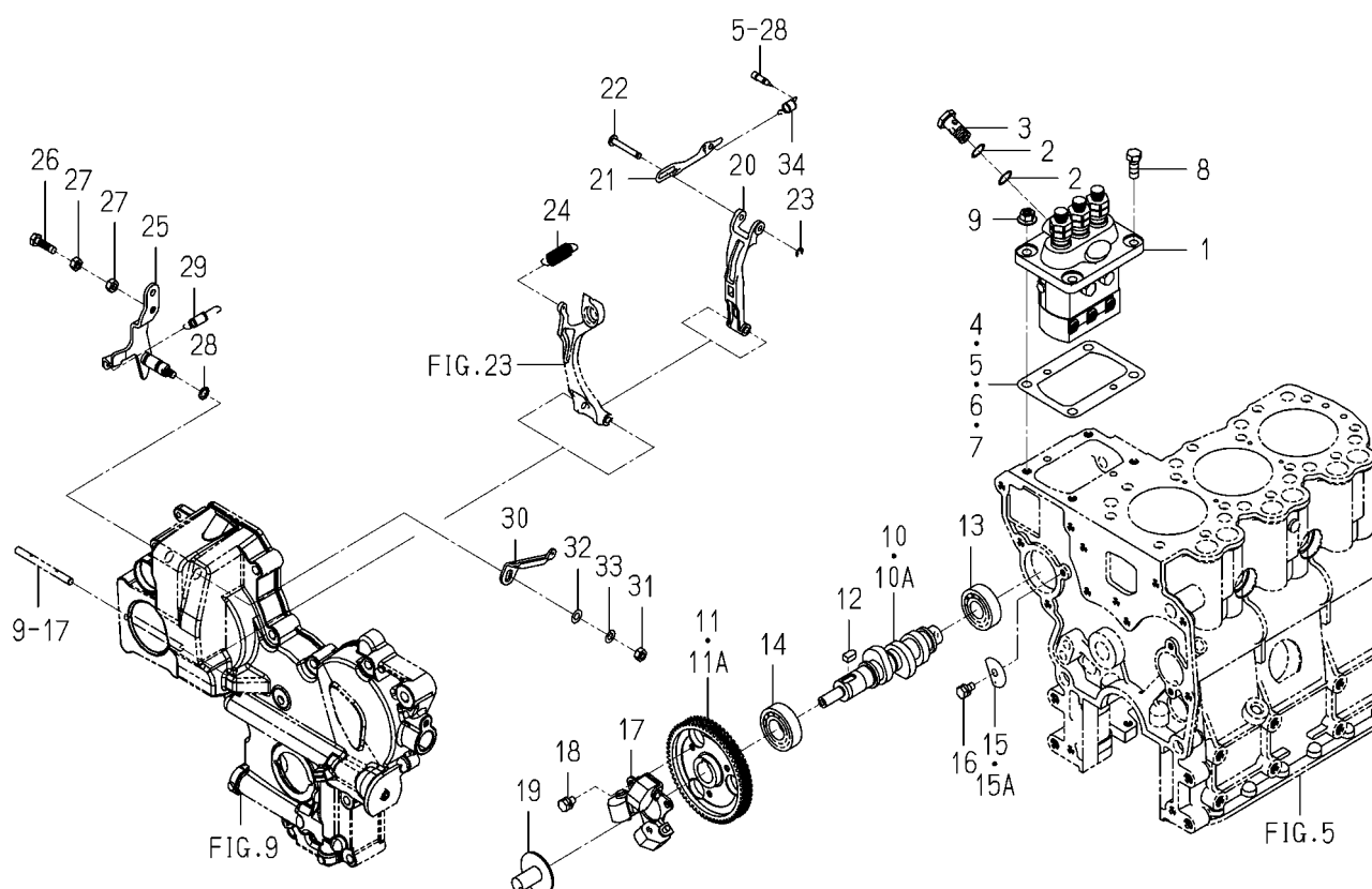
FIG. 21 INJECTION PUMP
