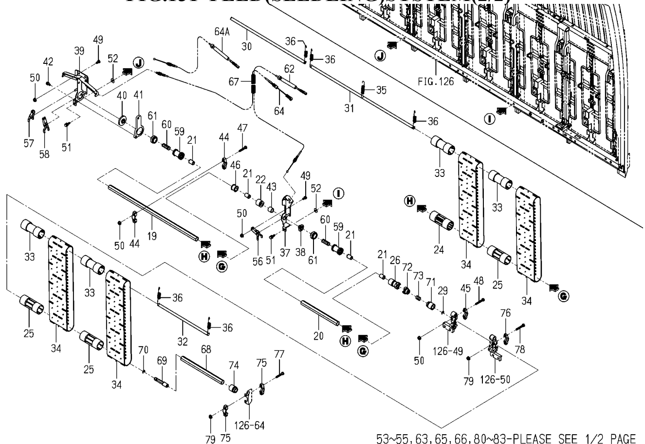
FIG.131 FEED(SEEDLING)SYSTEM(2/2)
