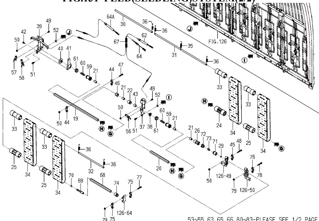
FIG.131 FEED(SEEDLING)SYSTEM(2/2)
