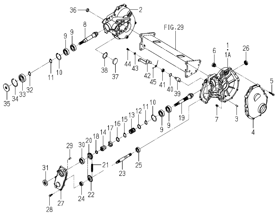
FIG. 36 CASE(REAR)SYSTEM(EXCEPT Z,F TYPE)(1/2)
