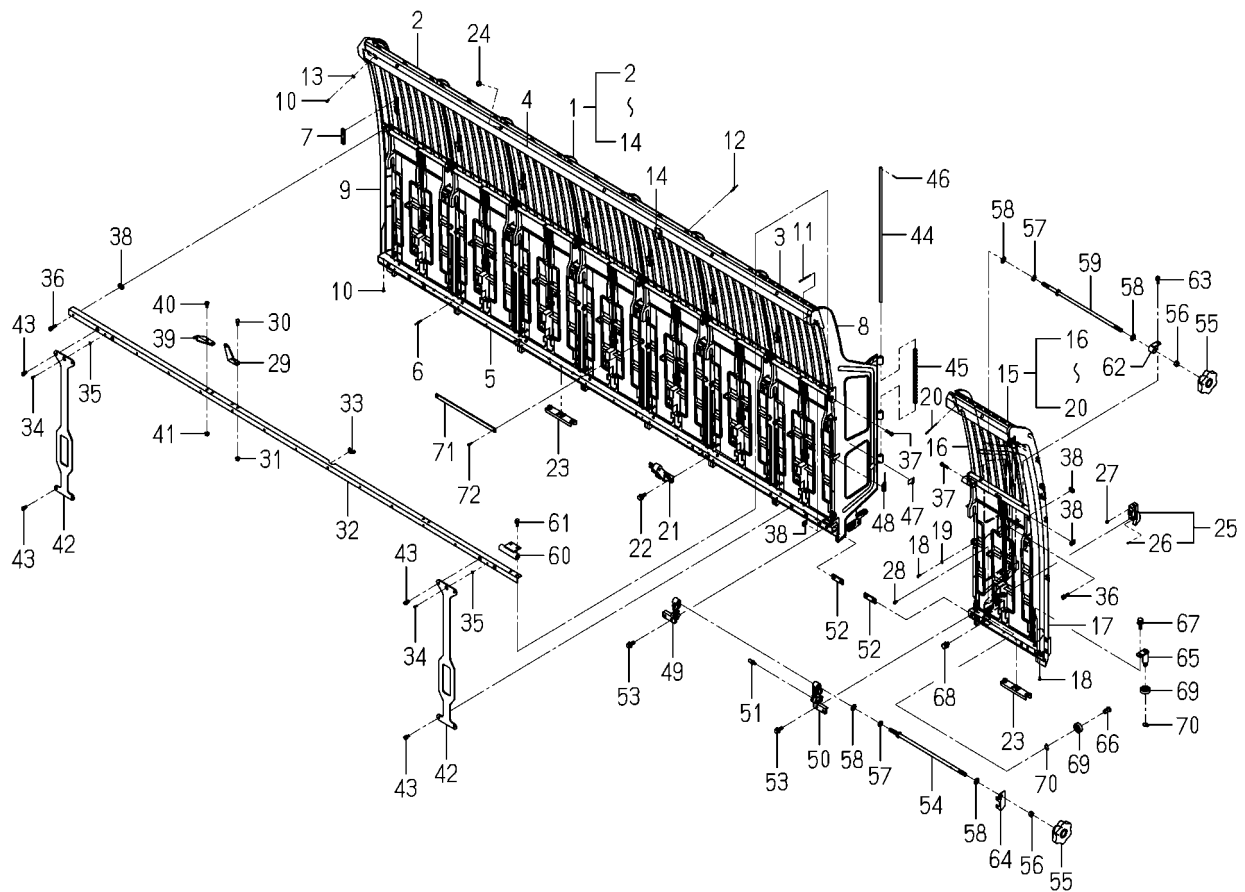
FIG.126 TANK(SEEDLING)SYSTEM
