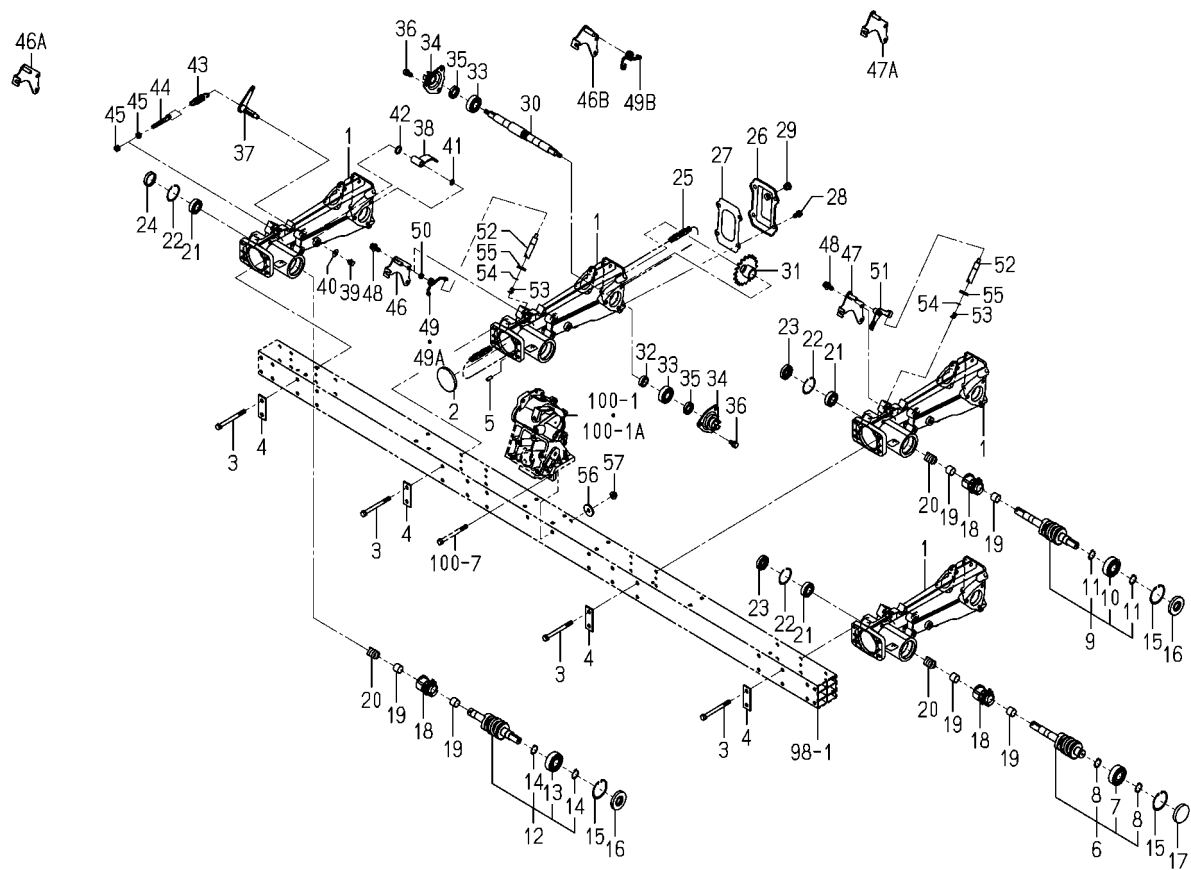
FIG.116 FRAME(SIDE)SYSTEM
