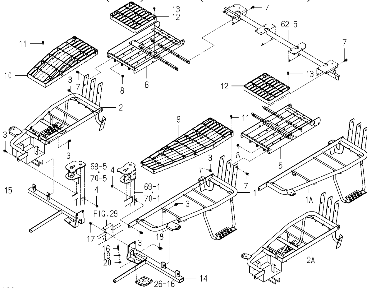
FIG. 60 STEP(SIDE)SYSTEM(EXCEPT F TYPE)
