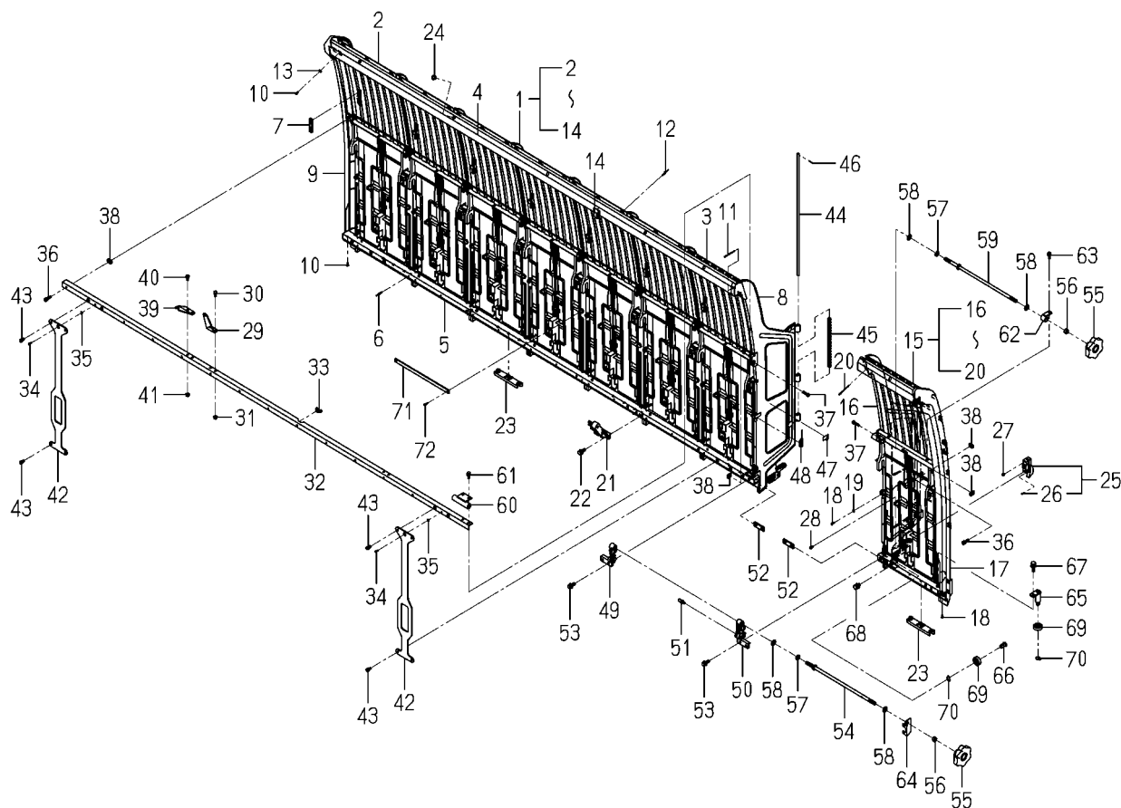
FIG.126 TANK(SEEDLING)SYSTEM
