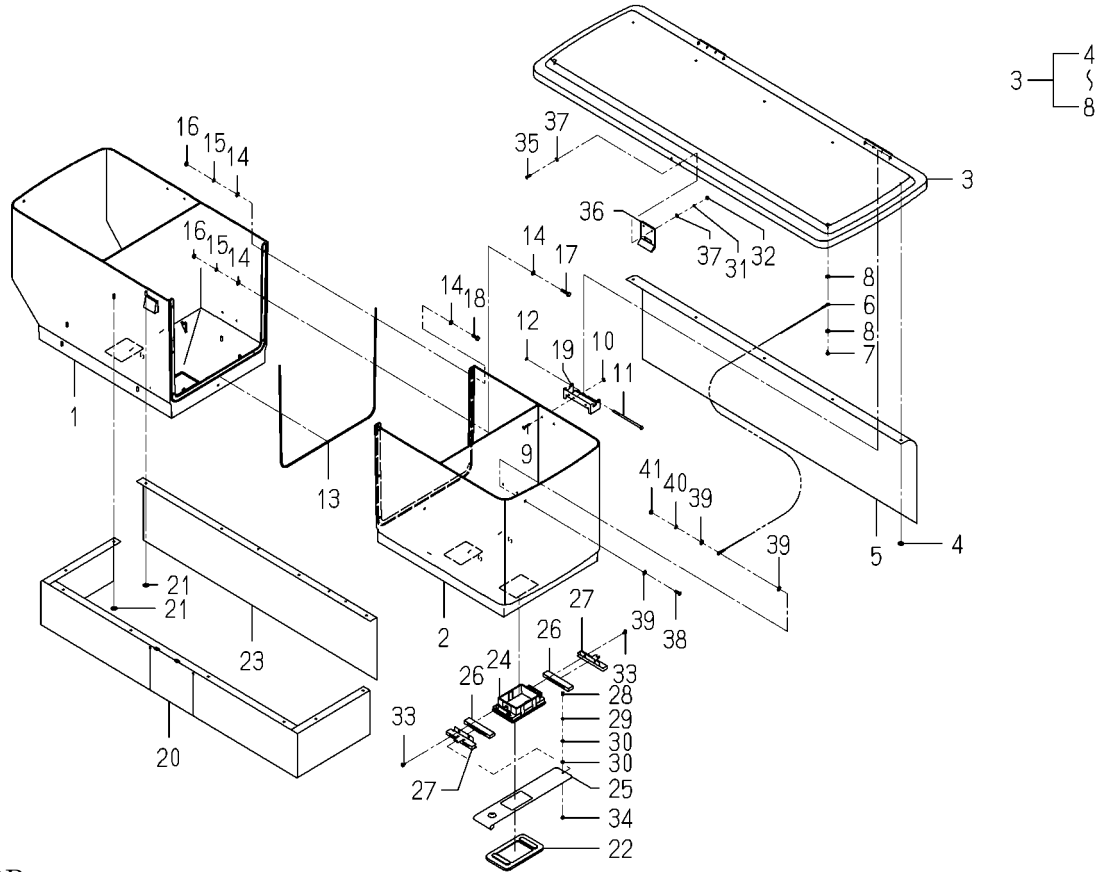
FIG.160 COMPONENT PARTS FOR 2233-688-320-00 ON Fig.114
