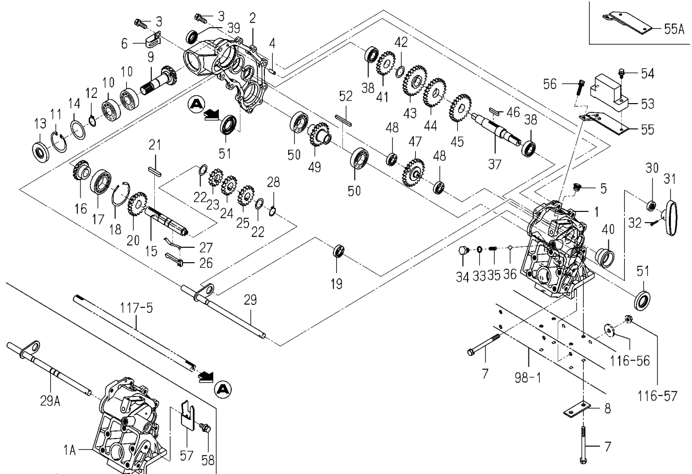
FIG.100 SLIDE SYSTEM
