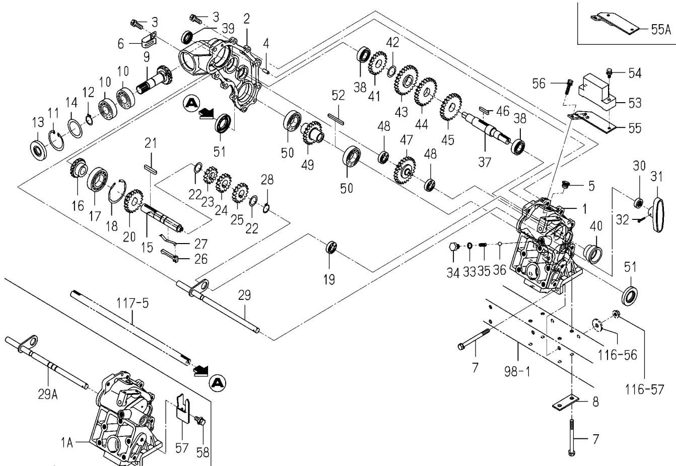
FIG.100 SLIDE SYSTEM
