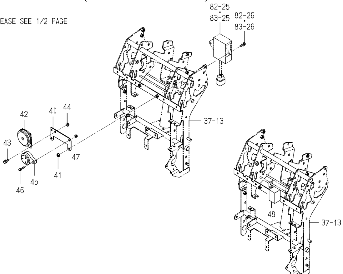
FIG. 81 PANEL(INSTRUMENT)SYSTEM(2/2) (R TYPE EXCEPT Z)
