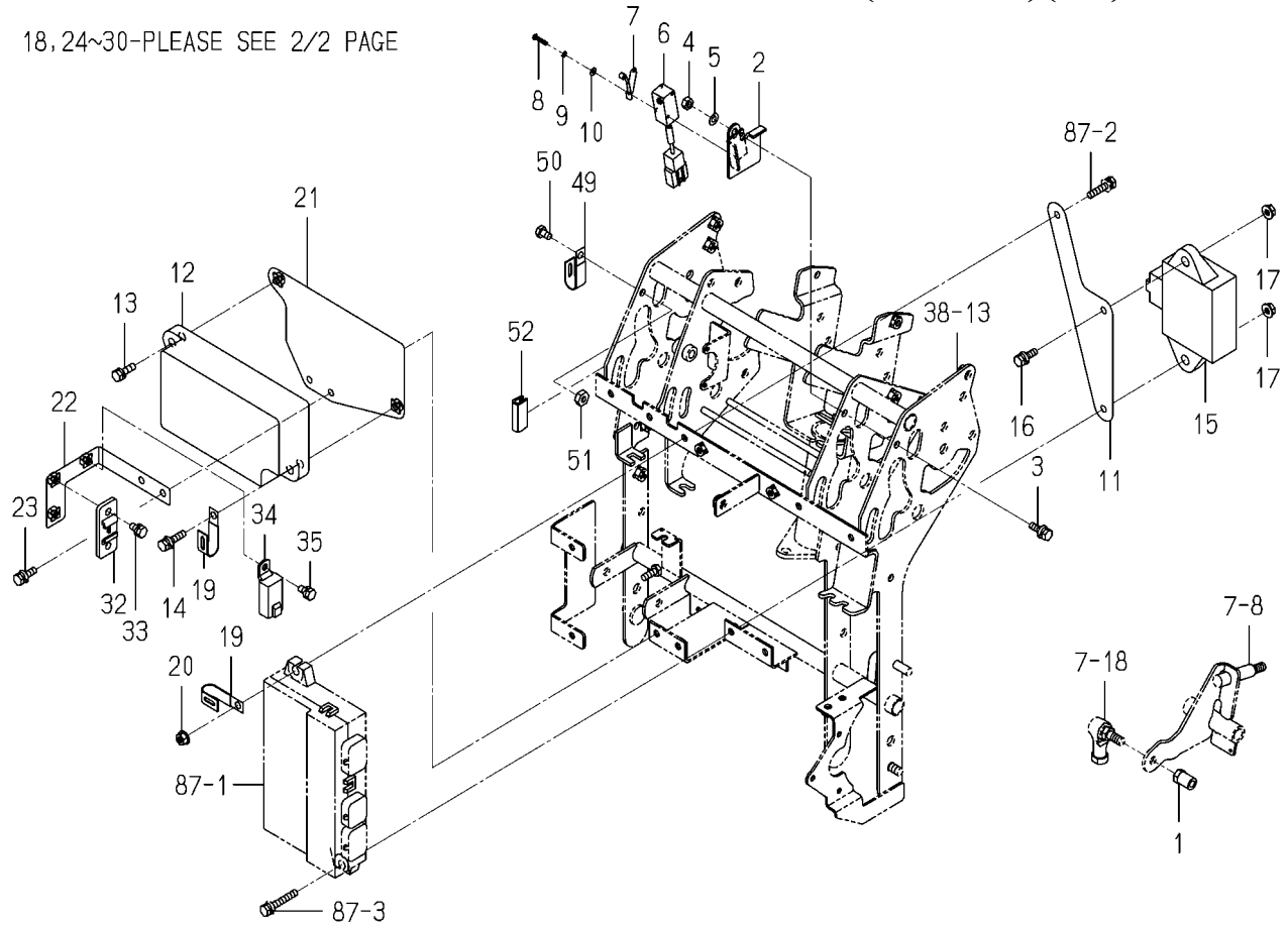
FIG. 90 CONTROLLER SYSTEM(Z TYPE)(1/2)
