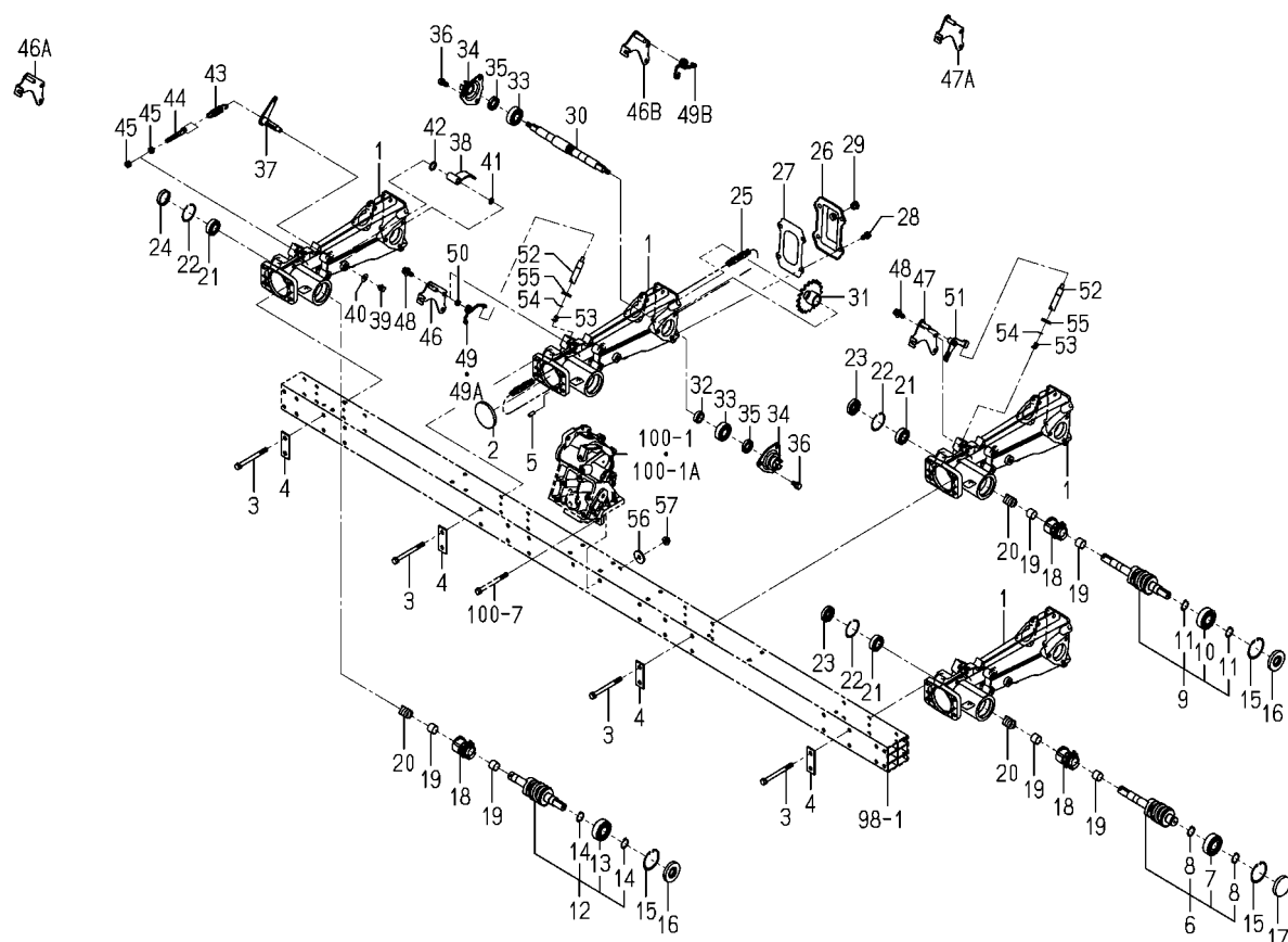
FIG.116 FRAME(SIDE)SYSTEM
