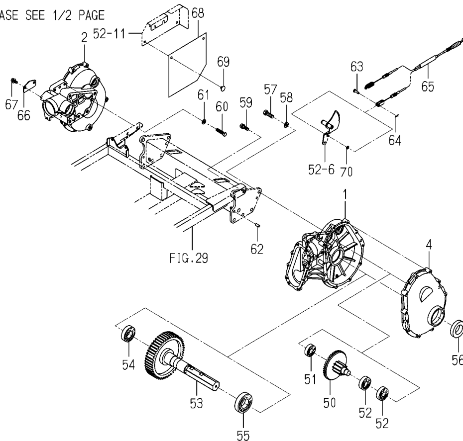
FIG. 33 CASE(REAR)SYSTEM(ZRF TYPE)(2/2)
