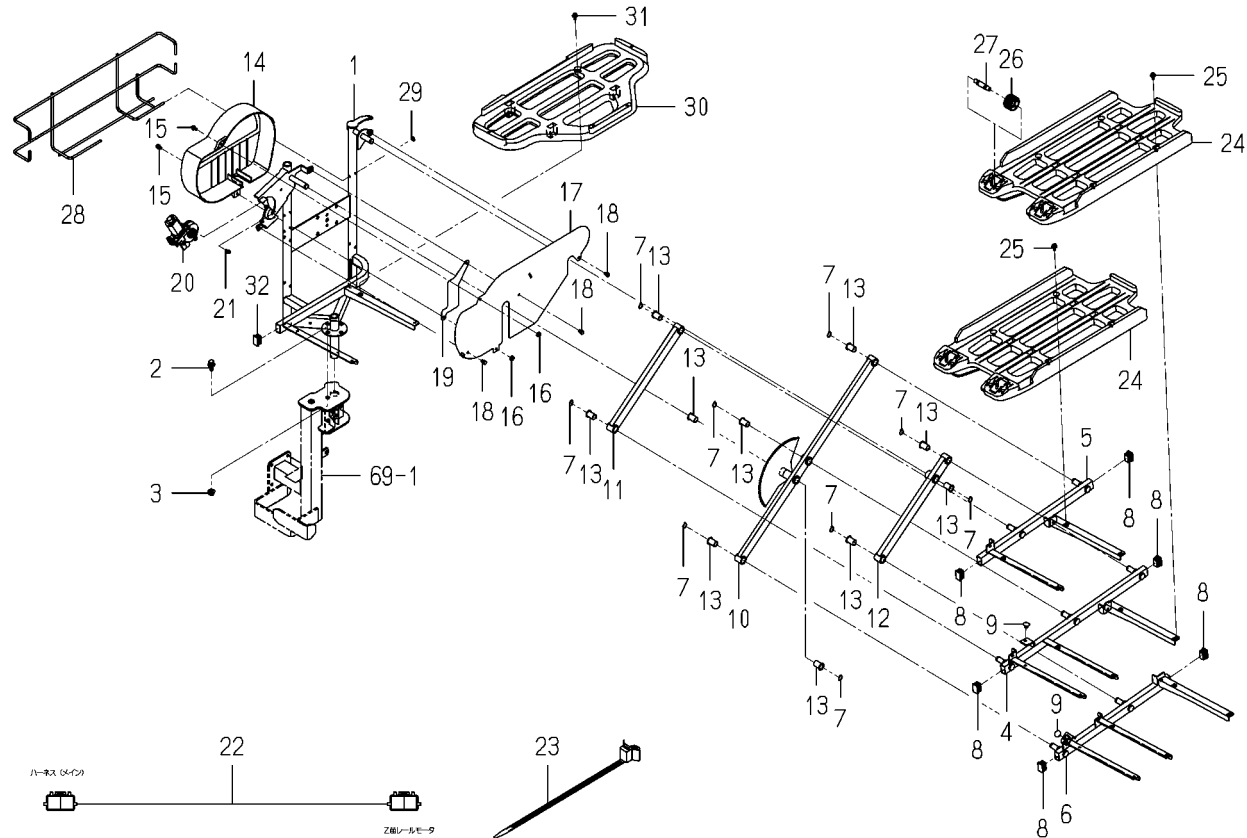
FIG. 64 TRAY(SEEDLING/SUB)SYSTEM(1/2) (R TYPE EXCEPT F)
