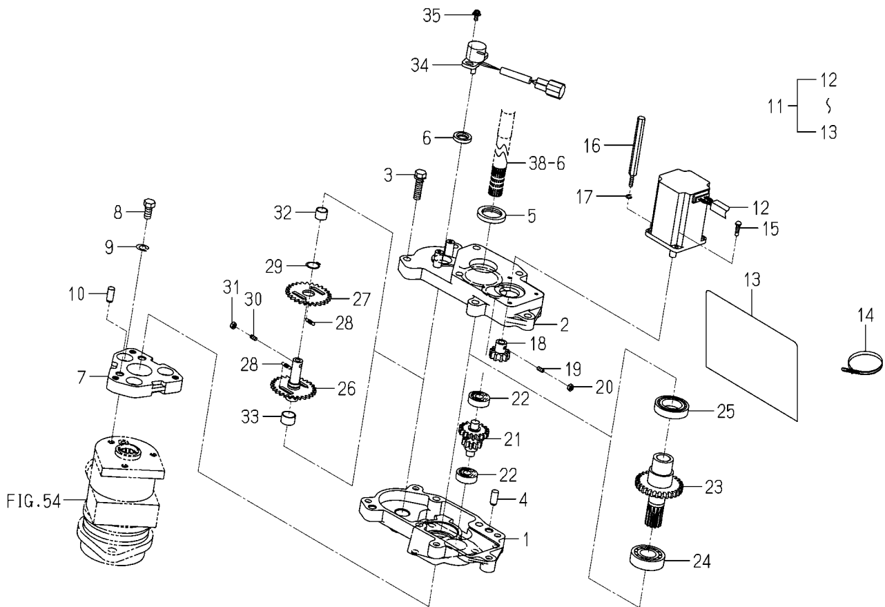
FIG. 44 MOTOR(DRIVE/UNIT)SYSTEM(Z TYPE)
