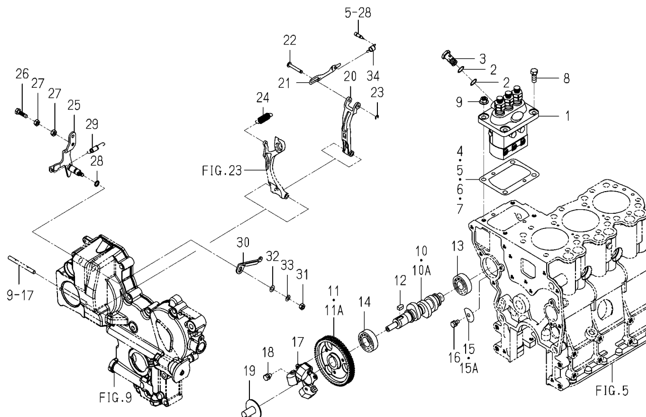
FIG. 21 INJECTION PUMP
