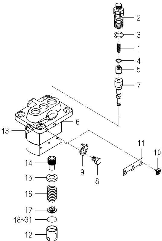
FIG. 28 COMPONENT PARTS FOR 6215-600-156-20 ON Fig.021
