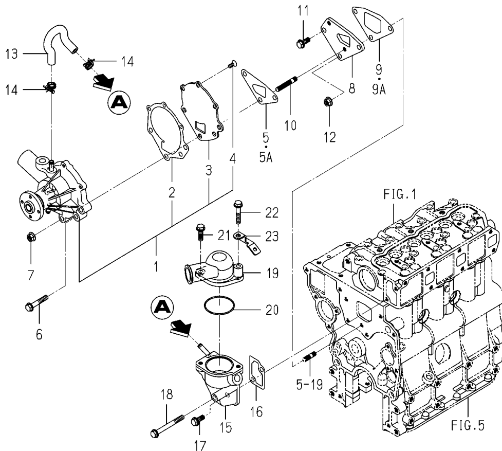
FIG. 18 WATER PUMP
