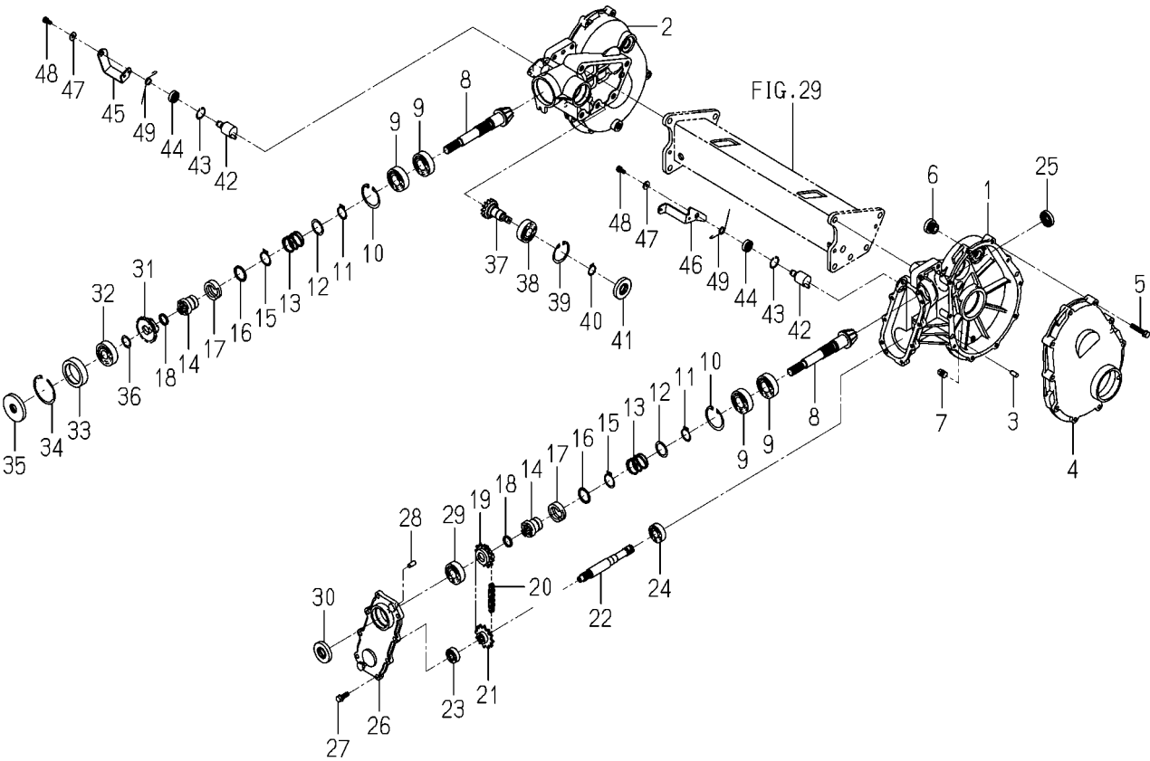
FIG. 33 CASE(REAR)SYSTEM(ZRF TYPE)(1/2)
