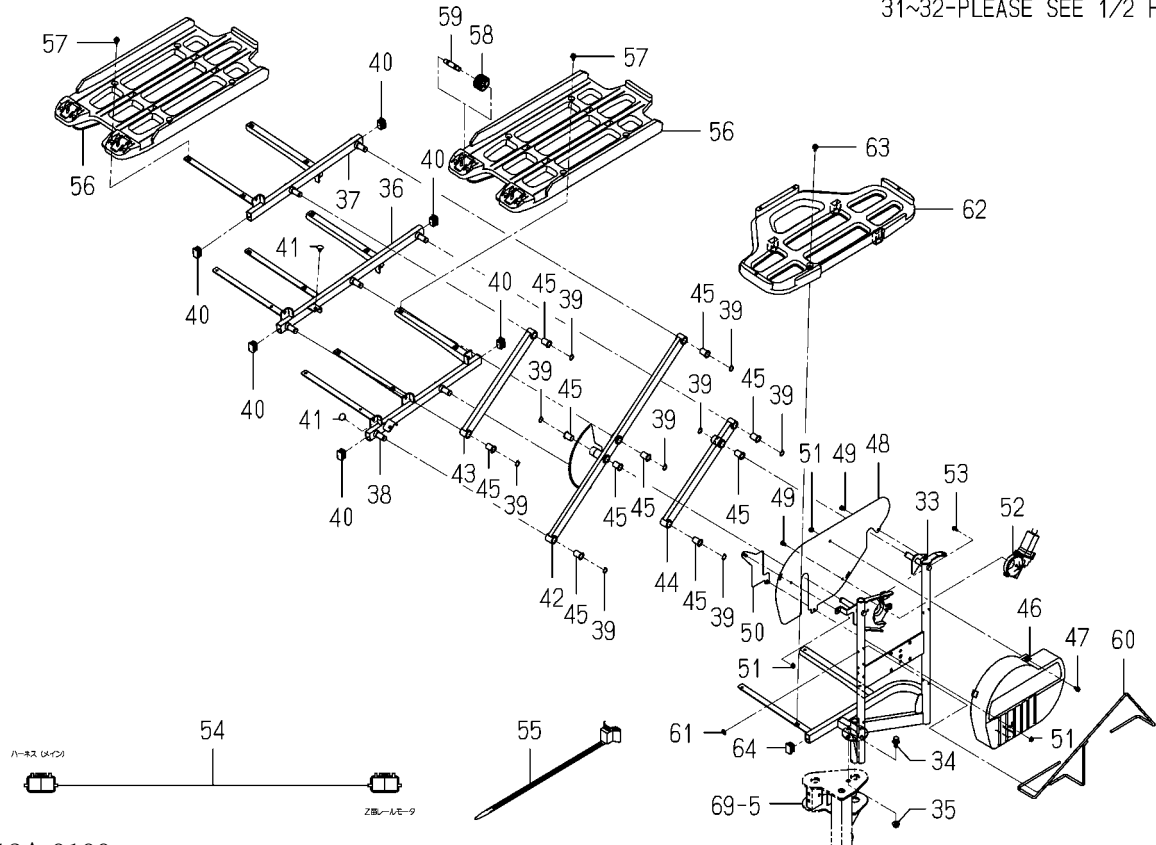
FIG. 64 TRAY(SEEDLING/SUB)SYSTEM(2/2) (R TYPE EXCEPT F)
