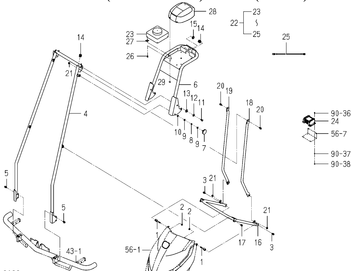
FIG. 89 STAY(GPS/ANTENNA)SYSTEM(Z TYPE)
