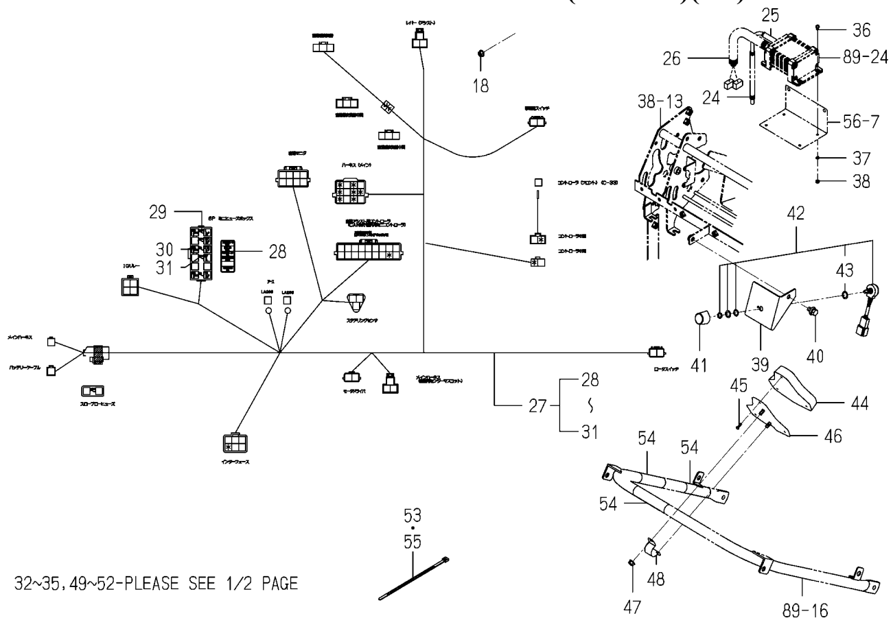
FIG. 90 CONTROLLER SYSTEM(Z TYPE)(2/2)
