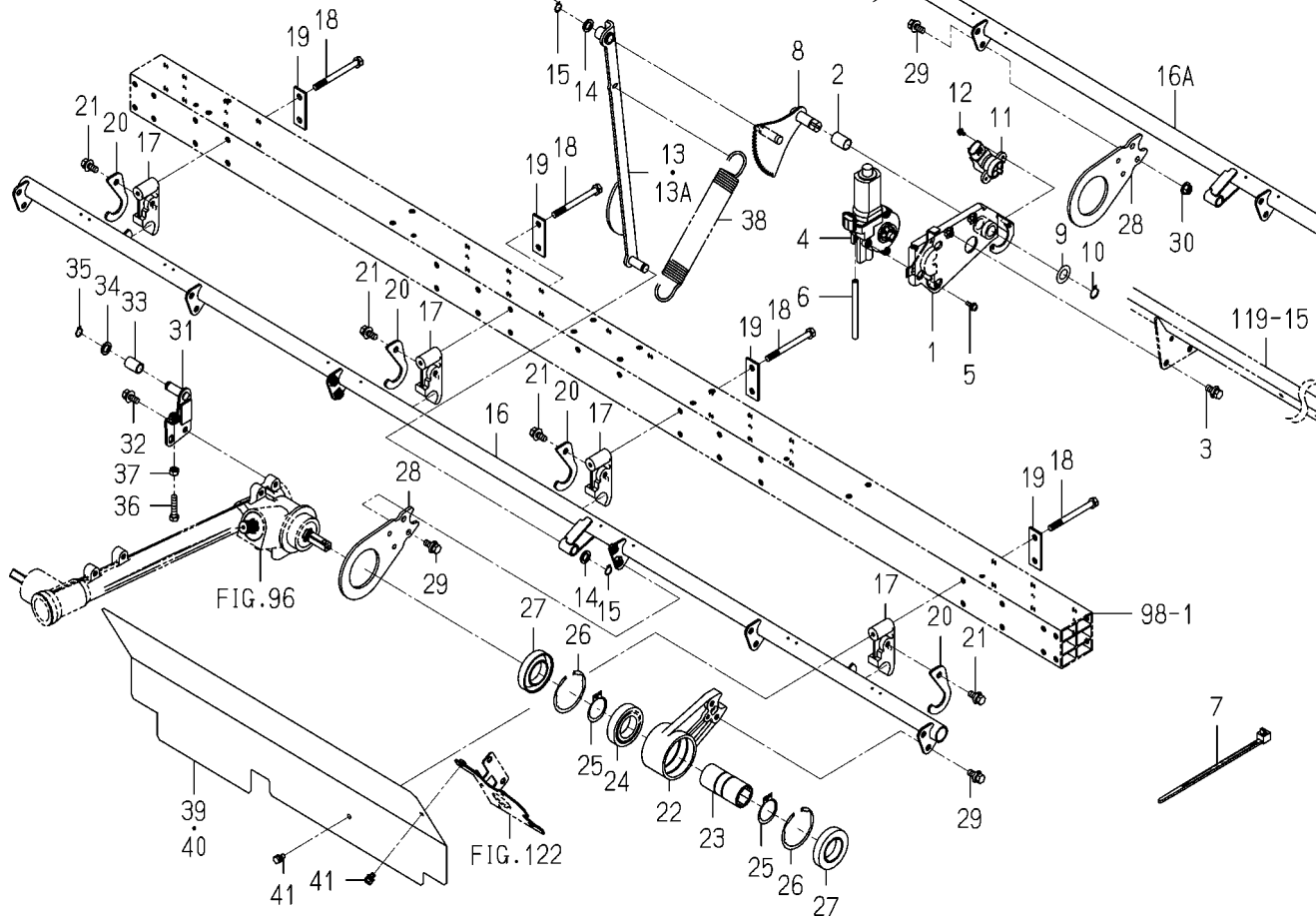
FIG. 95 LEVER(DEPTH/ROTOR)SYSTEM
