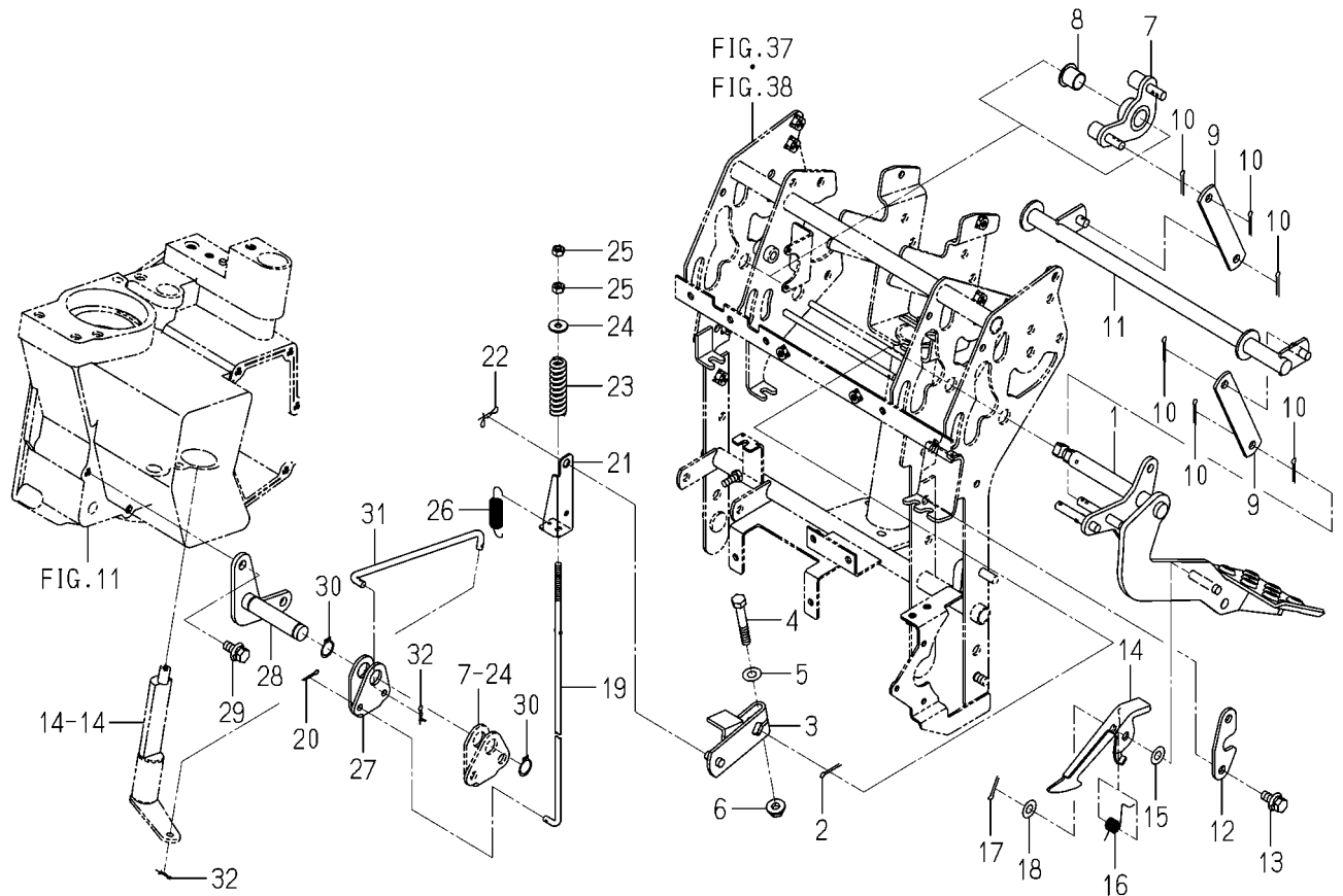
FIG. 39 PEDAL(BRAKE/PARKING)SYSTEM
