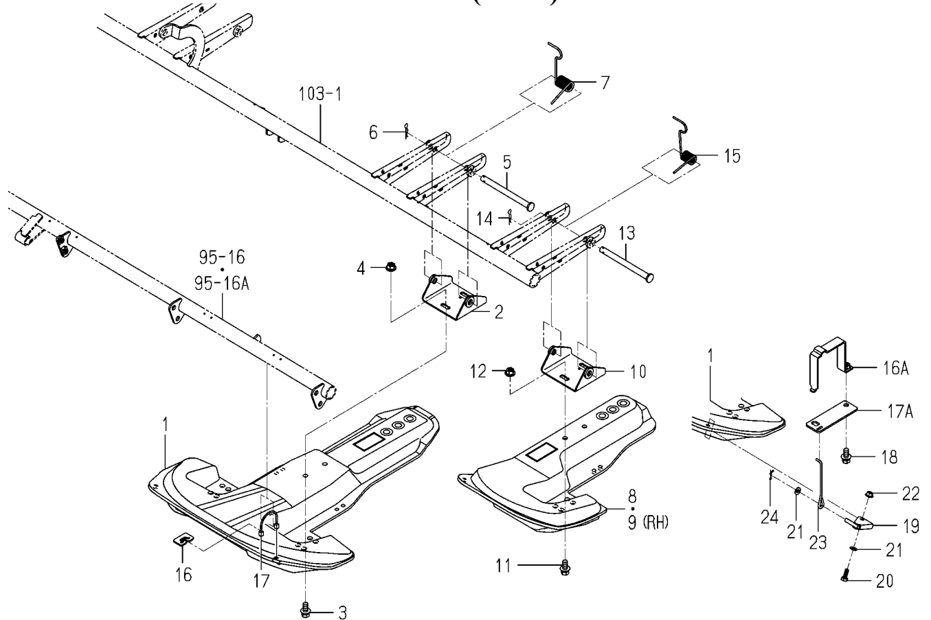
FIG.121 FLOAT(SIDE)SYSTEM
