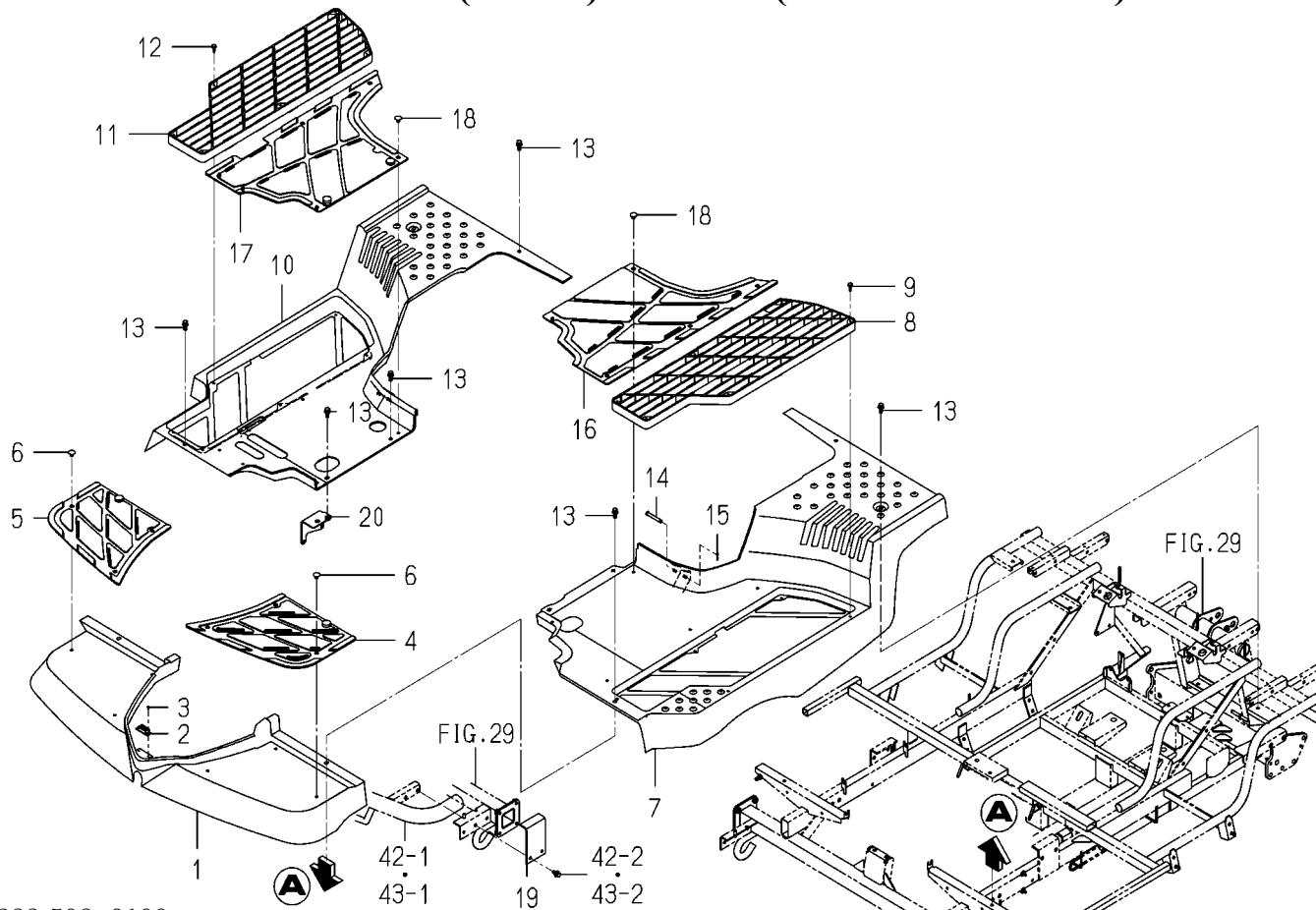
FIG. 58 STEP(MAIN)SYSTEM(EXCEPT F TYPE)
