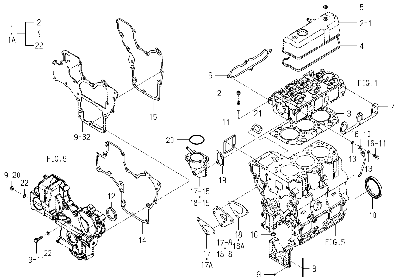
FIG. 26 REPAIR PARTS(OPTION)
