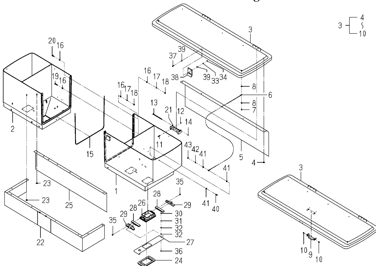
FIG.159 COMPONENT PARTS FOR 2233-688-310-00 ON Fig.114
