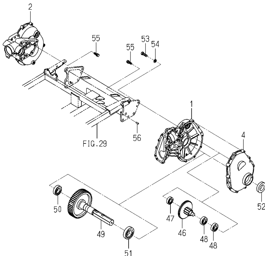
FIG. 34 CASE(REAR)SYSTEM(ZR TYPE EXCEPT F)(2/2)
