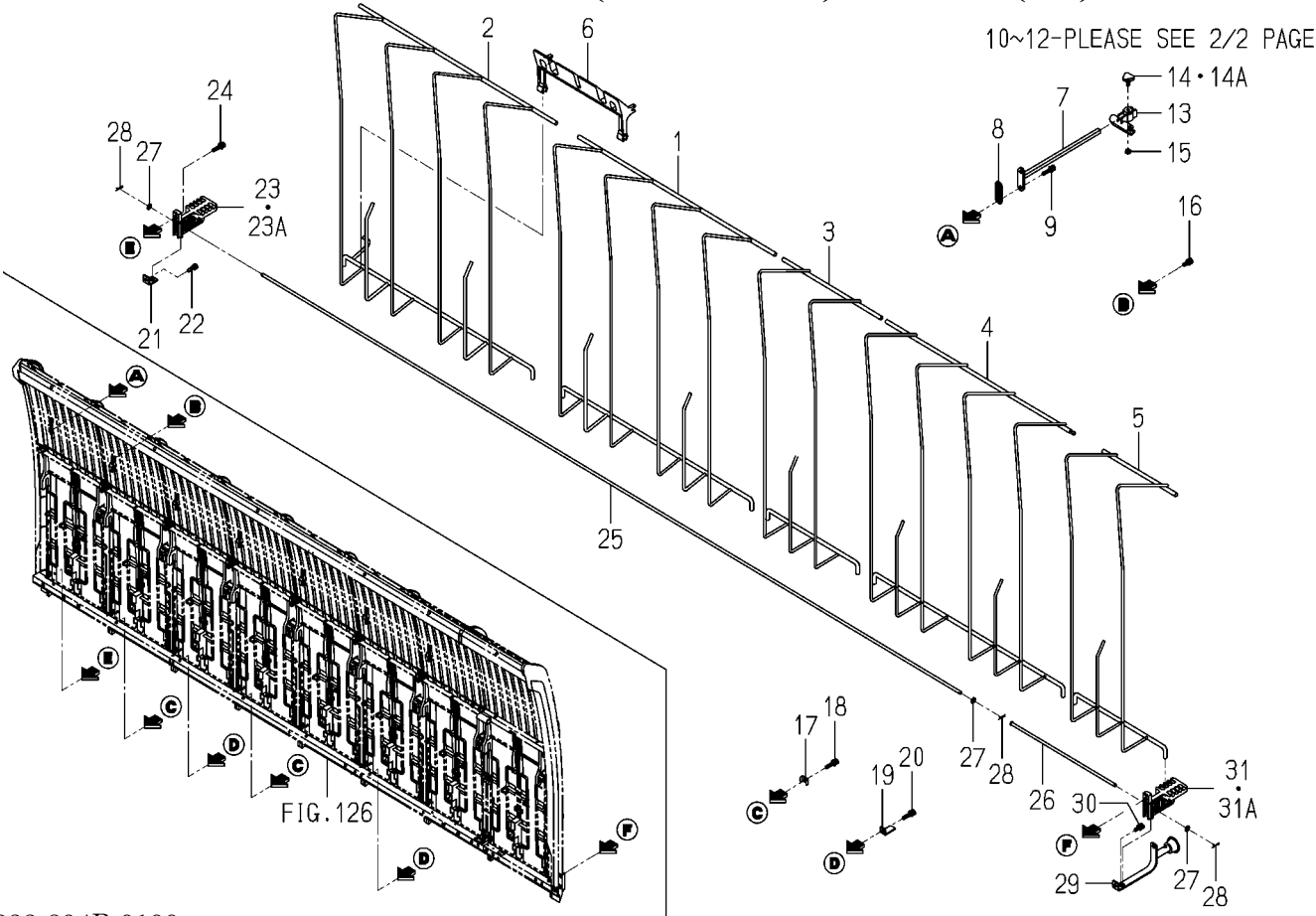
FIG.130 HOLDER(SEEDLING)SYSTEM(1/2)
