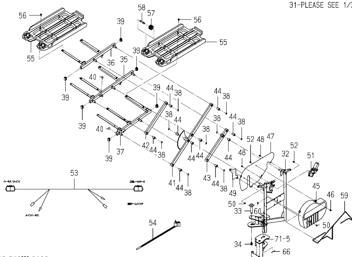
FIG. 68 TRAY(SEEDLING/SUB)SYSTEM(ZRF TYPE)(2/3)
