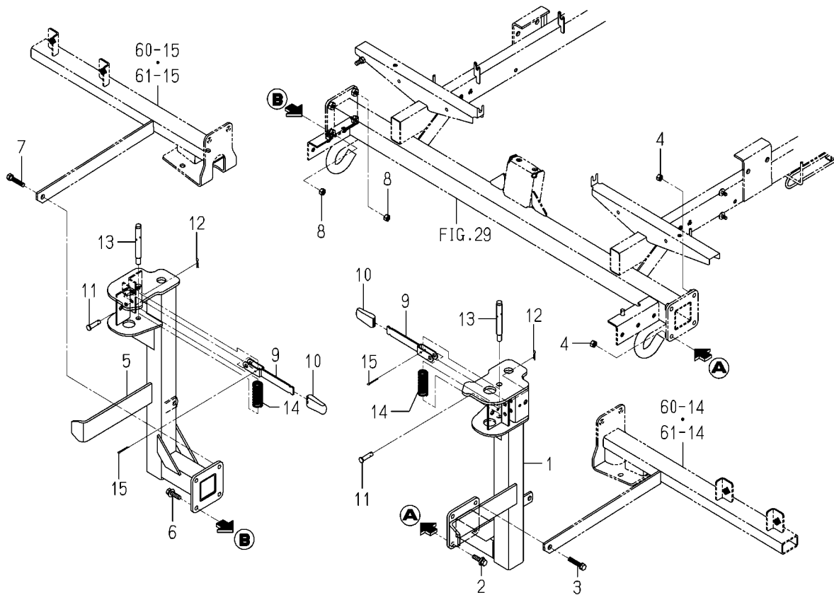
FIG. 70 STAY(FRAME/SEEDLING/SUB)SYSTEM (EXCEPT R TYPE)
