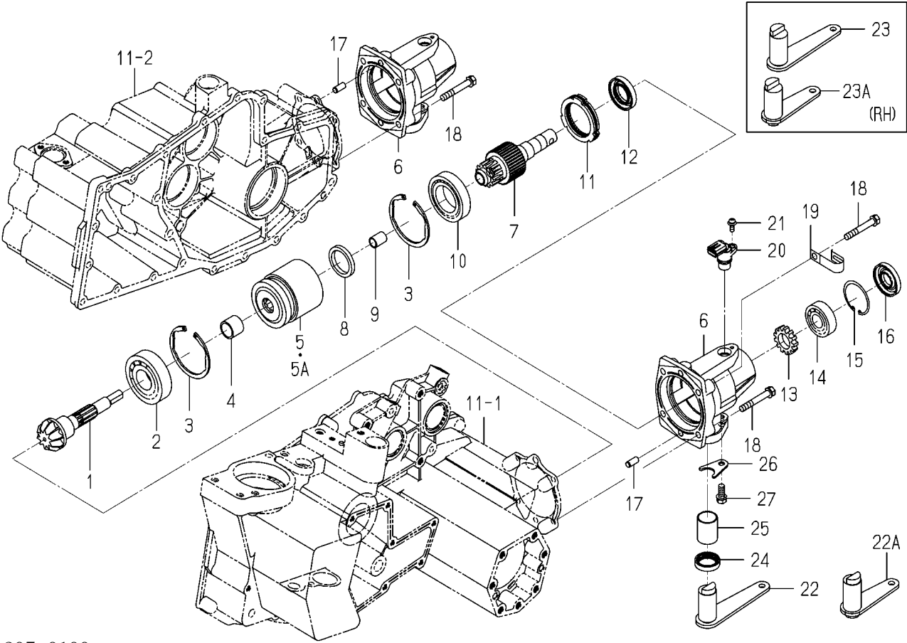
FIG. 15 SHAFT(REAR),CLUTCH&BRAKE SYSTEM
