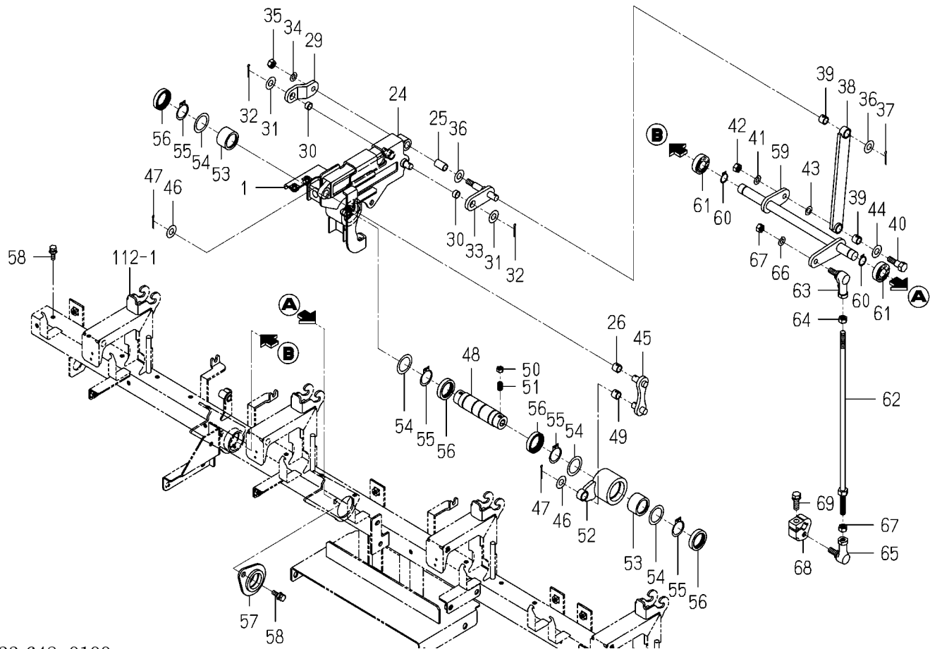
FIG.108 DRIVE(FERTILIZER)SYSTEM(F TYPE)(2/2)
