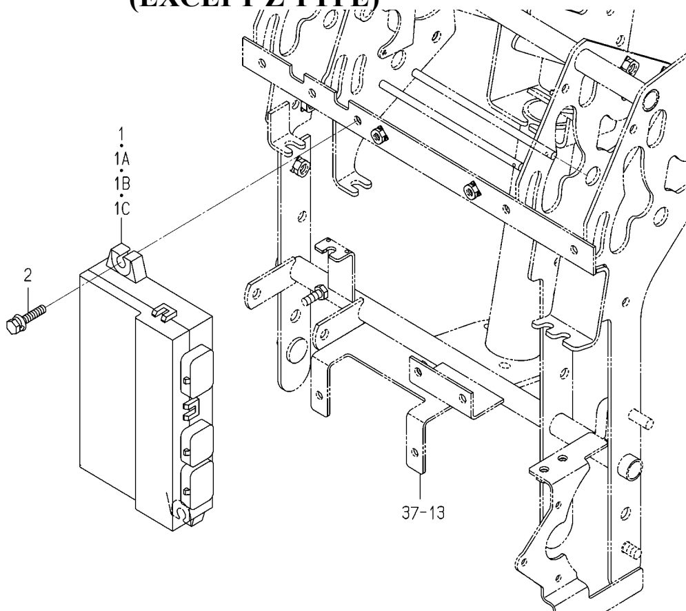
FIG. 86 CONTROLLER(FRONT)SYSTEM (EXCEPT Z TYPE)
