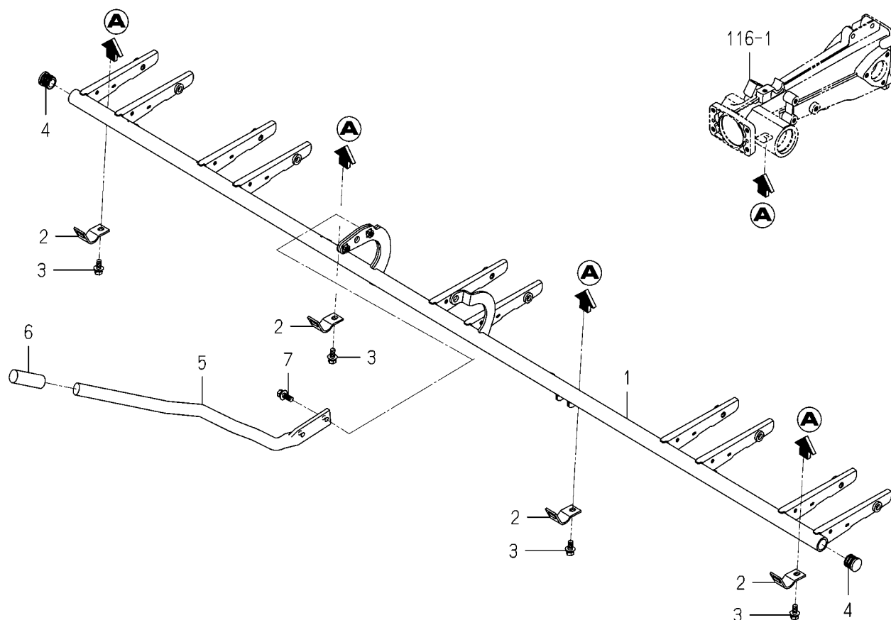
FIG.103 LEVER(DEPTH/PLANTING)SYSTEM
