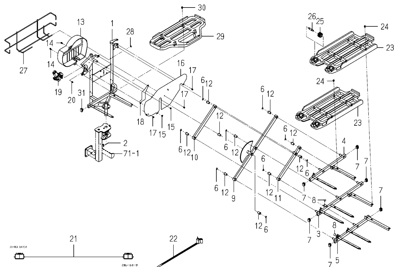
FIG. 68 TRAY(SEEDLING/SUB)SYSTEM(ZRF TYPE)(1/3)
