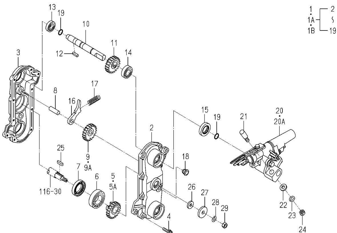
FIG.124 PLANTER(LH)SYSTEM
