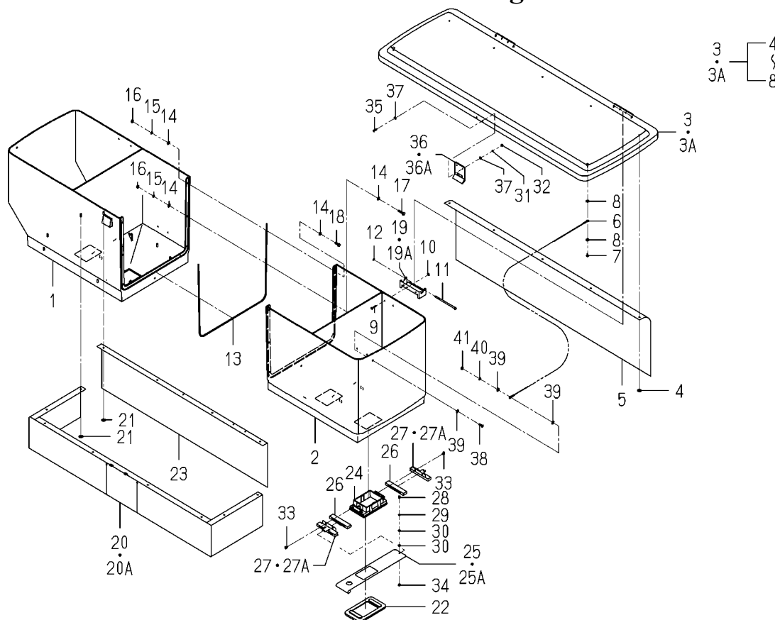
FIG.158 COMPONENT PARTS FOR 2233-688-270-90 ON Fig.114
