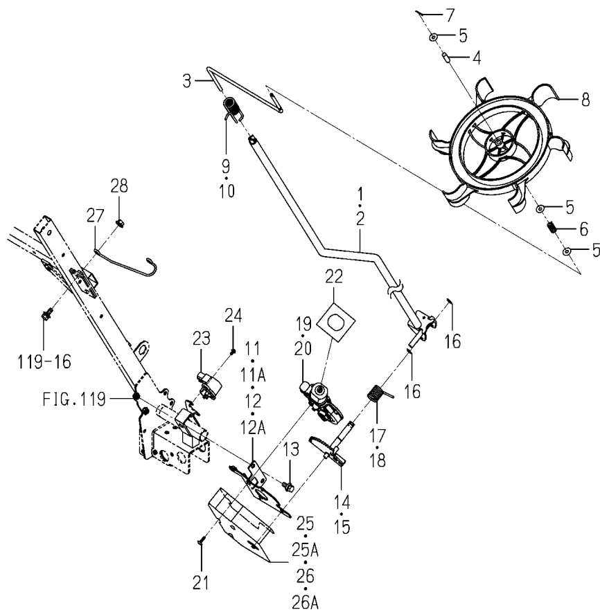
FIG.122 MARKER SYSTEM
