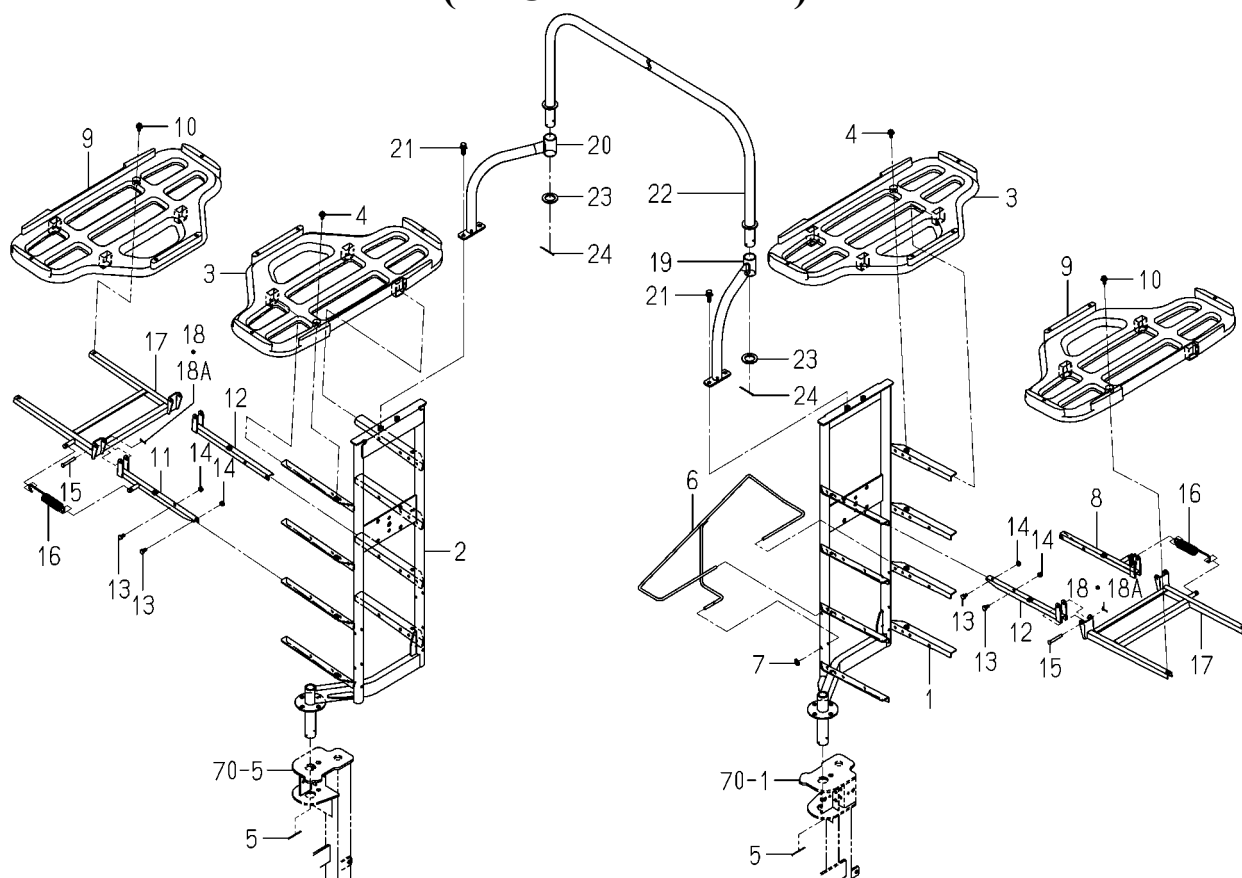
FIG. 65 TRAY(SEEDLING/SUB)SYSTEM (EXCEPT R TYPE)
