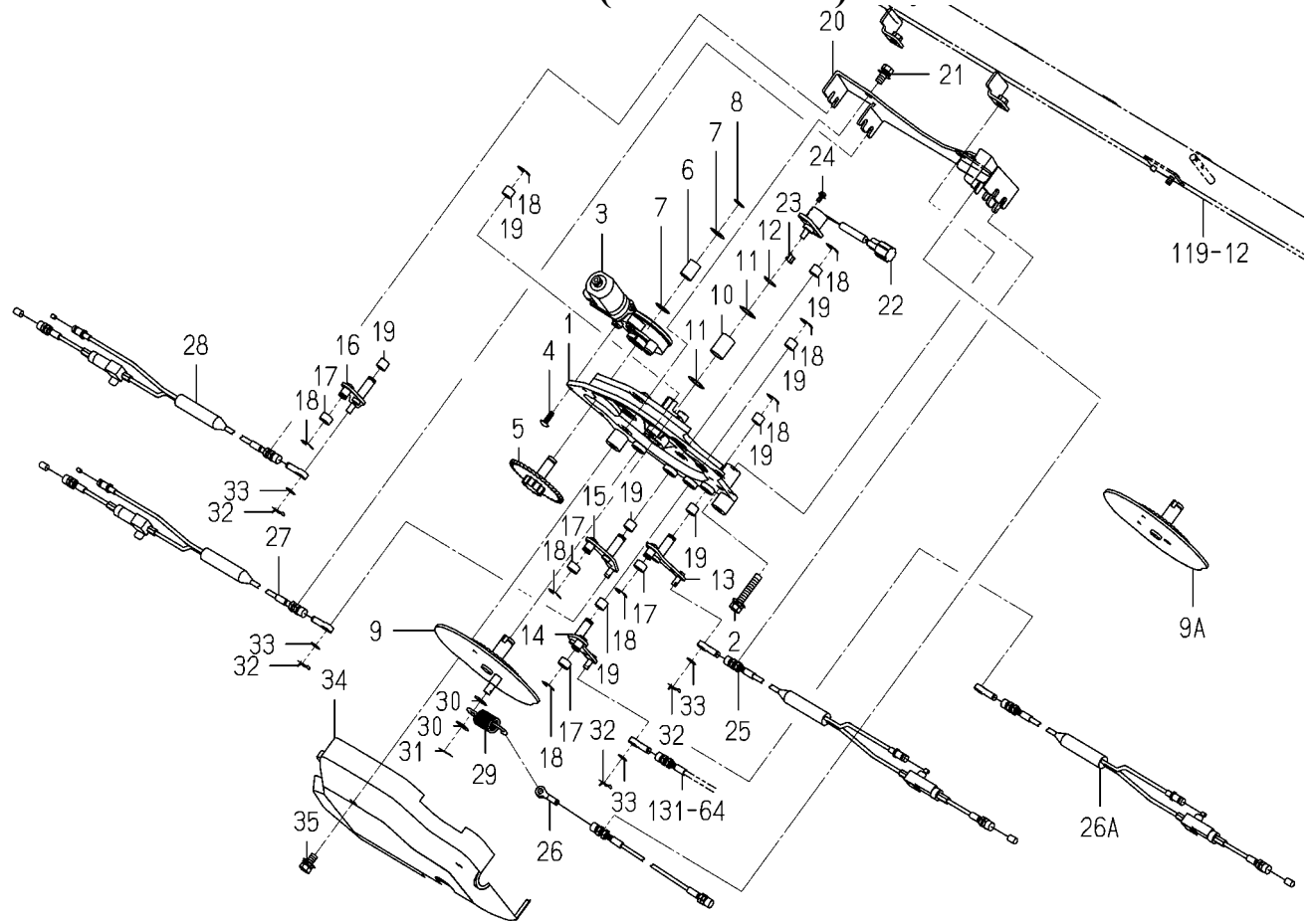
FIG. 91 CLUTCH(PLANTING)SYSTEM
