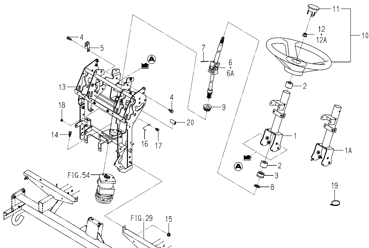
FIG. 37 WHEEL(STEERING)SYSTEM (EXCEPT Z TYPE)
