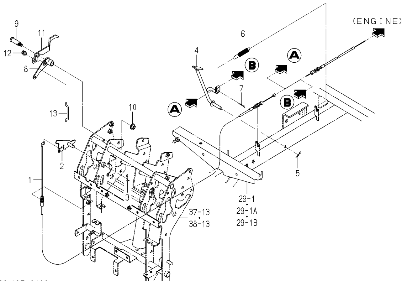
FIG. 10 PEDAL(ACCELERATOR)SYSTEM
