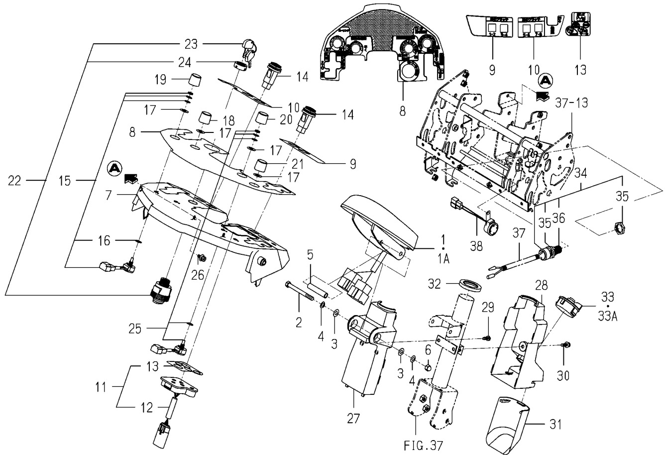
FIG. 80 PANEL(INSTRUMENT)SYSTEM(1/2)
