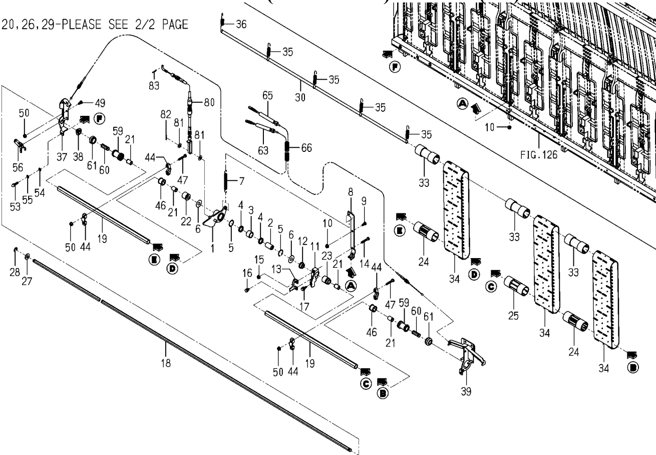
FIG.131 FEED(SEEDLING)SYSTEM(1/2)
