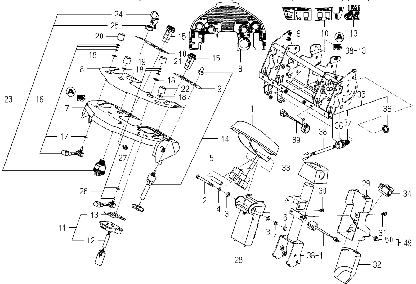
FIG. 79 PANEL(INSTRUMENT)SYSTEM(Z TYPE)(1/2)
