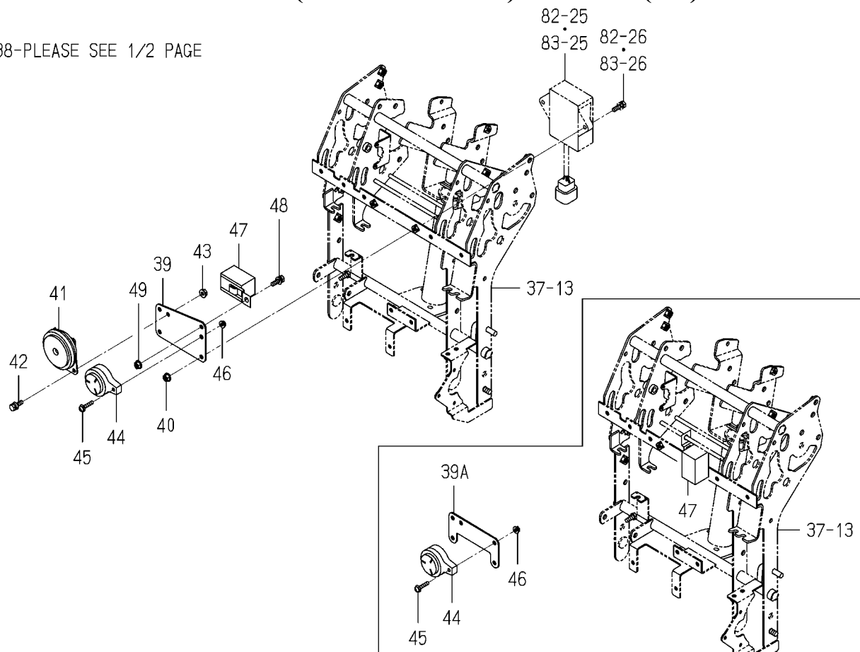
FIG. 80 PANEL(INSTRUMENT)SYSTEM(2/2)
