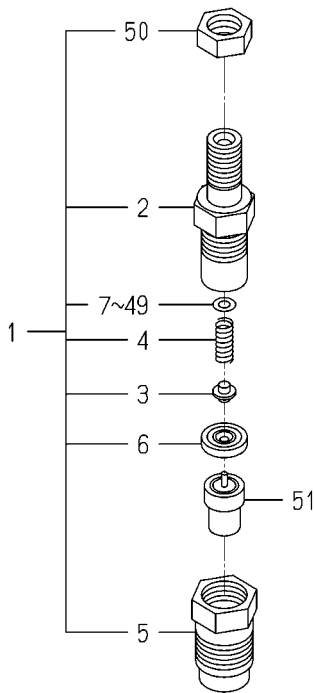
FIG. 27 COMPONENT PARTS FOR 6215-300-036-10 ON Fig.020
