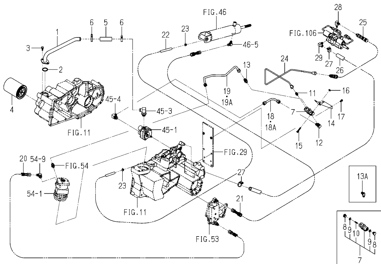
FIG. 47 PIPING SYSTEM(1/2)
