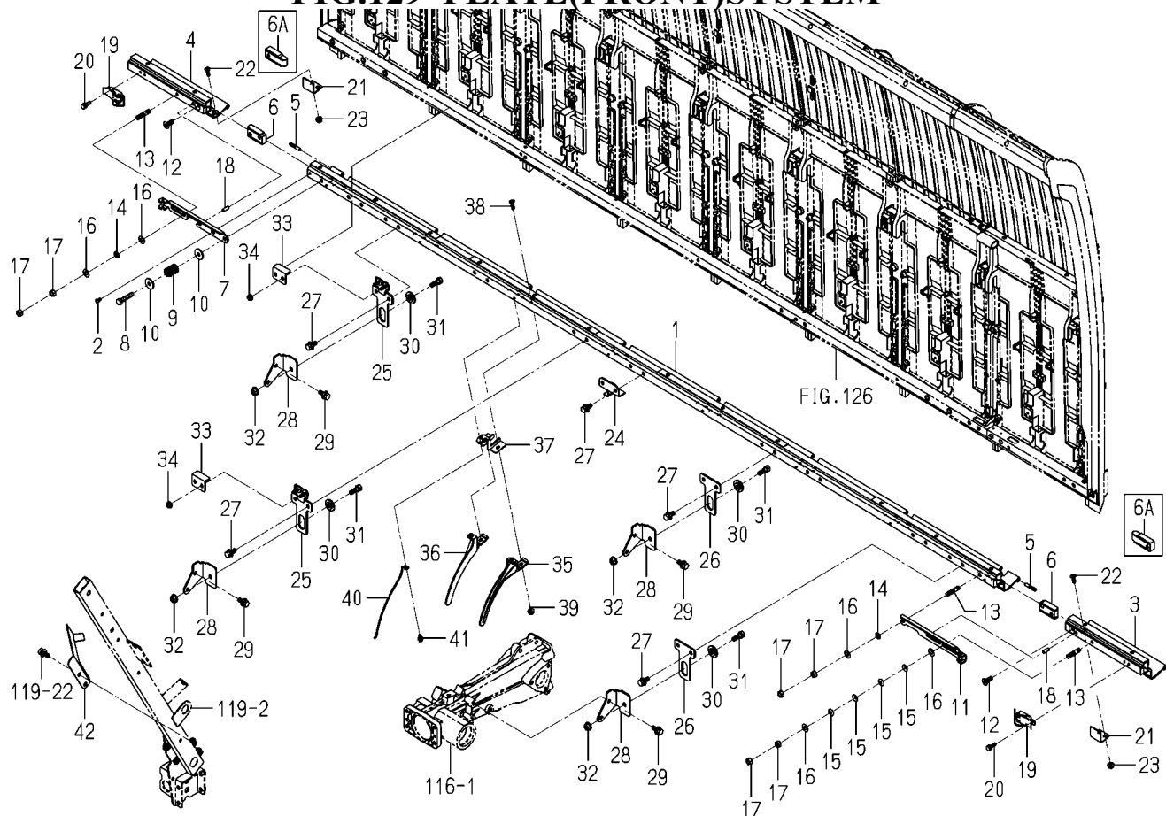
FIG.129 PLATE(FRONT)SYSTEM
