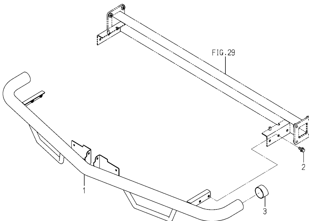
FIG. 42 BUMPER SYSTEM(EXCEPT Z TYPE)
