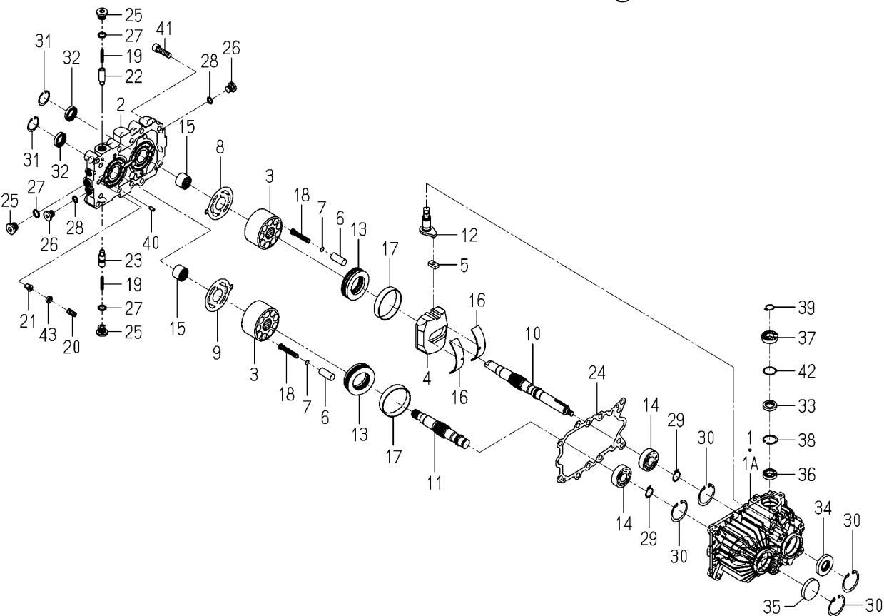
FIG.153 COMPONENT PARTS FOR K510-022-000-00 ON Fig.8
