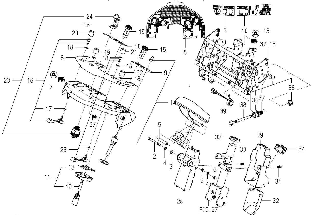
FIG. 81 PANEL(INSTRUMENT)SYSTEM(1/2) (R TYPE EXCEPT Z)
