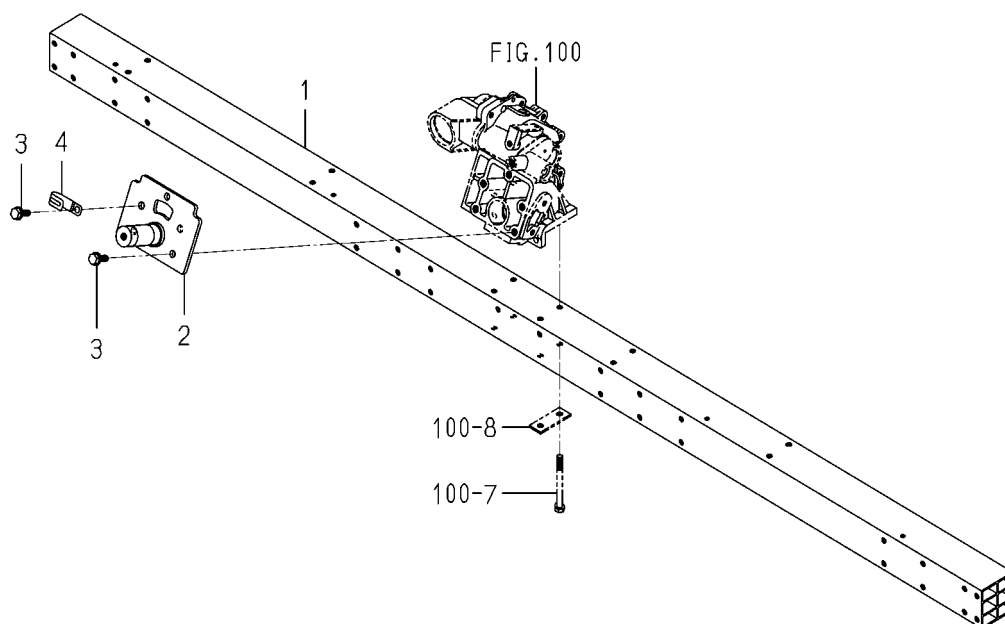
FIG. 98 RAIL(PLANTING)SYSTEM
