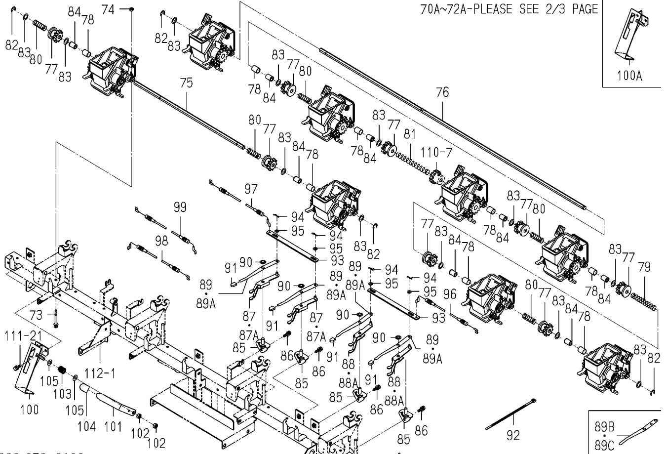
FIG.113 SEND OUT(FERTILIZER)SYSTEM(F TYPE)(3/3)
