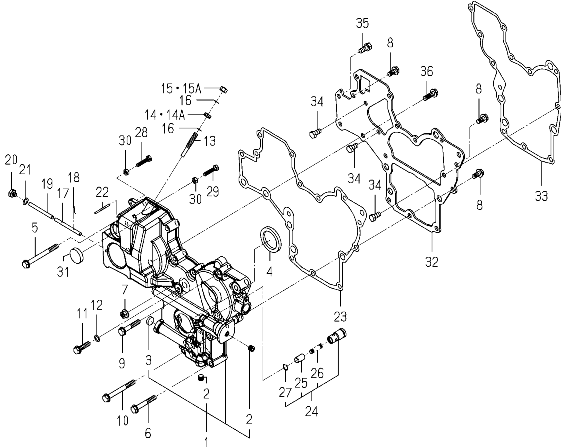
FIG. 9 TIMING GEAR CASE
