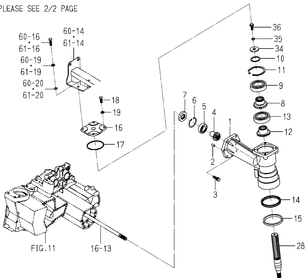
FIG. 26 CASE(GEAR/FINAL)SYSTEM(1/2)
