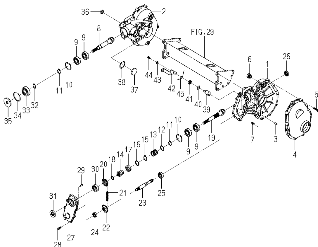
FIG. 34 CASE(REAR)SYSTEM(ZR TYPE EXCEPT F)(1/2)
