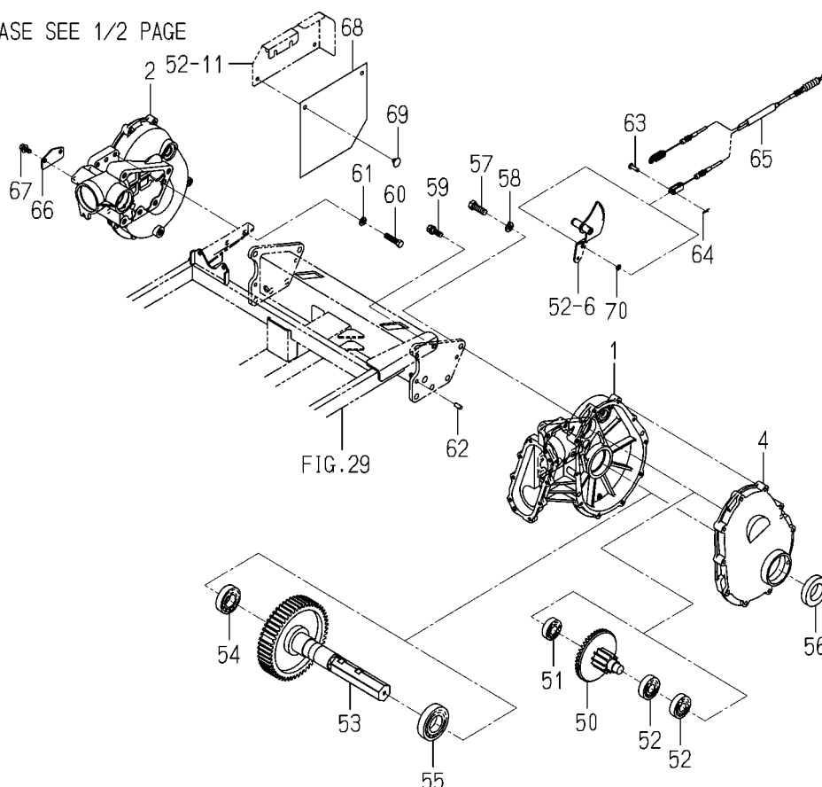
FIG. 33 CASE(REAR)SYSTEM(ZRF TYPE)(2/2)
