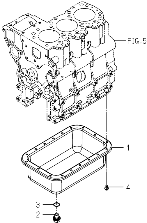
FIG. 7 OIL PAN
