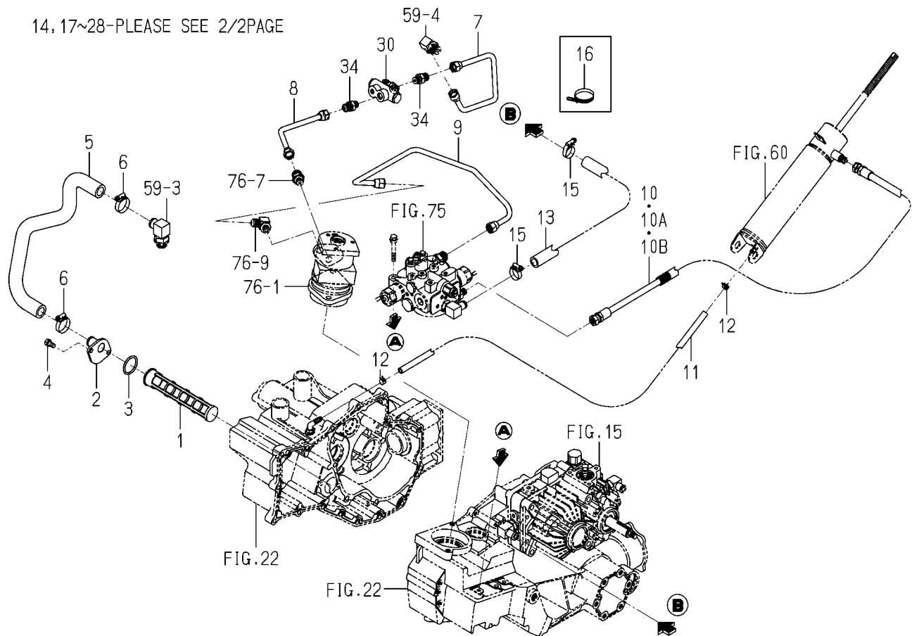
FIG. 61 PIPING SYSTEM(D TYPE)(1/2)
