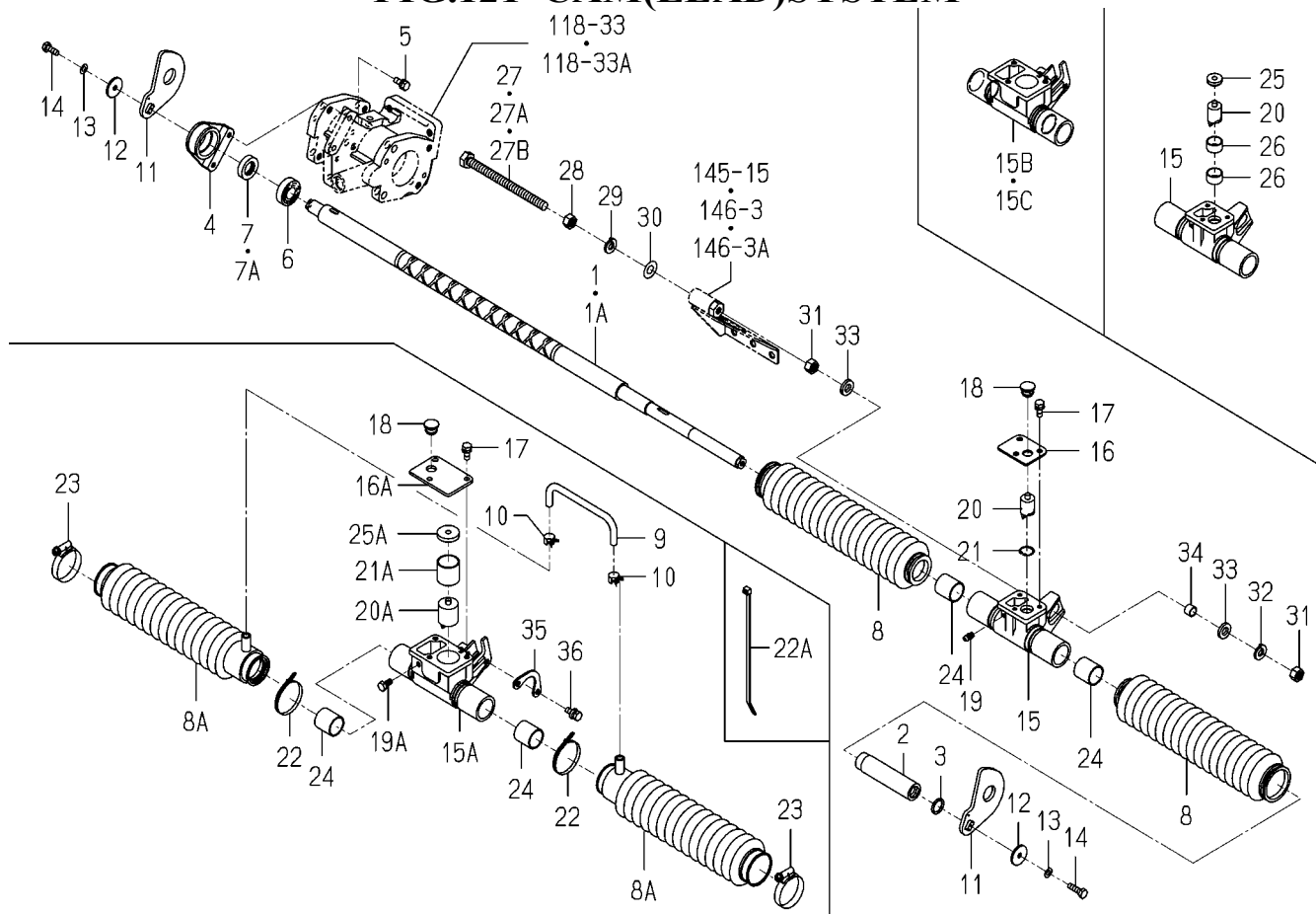
FIG.121 CAM(LEAD)SYSTEM
