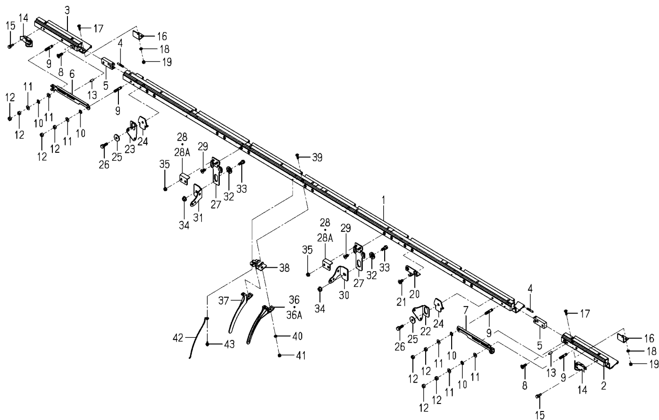
FIG.149 PLATE(FRONT)SYSTEM(NO.101650-)
