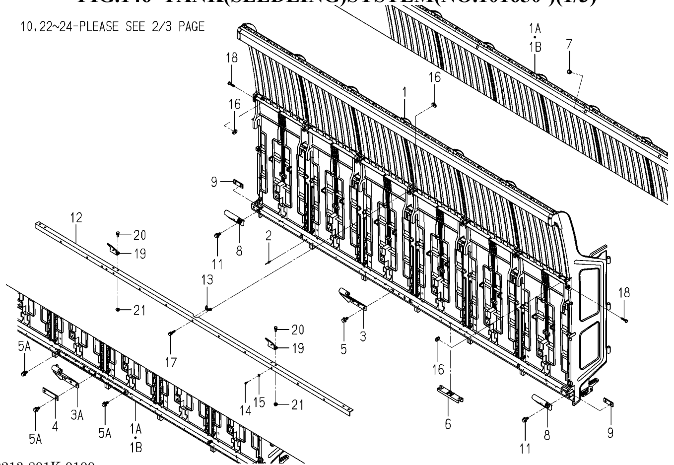
FIG.146 TANK(SEEDLING)SYSTEM(NO.101650-)(1/3)
