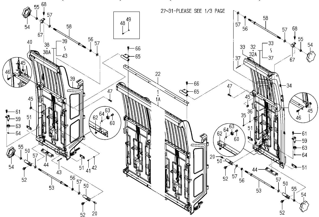
FIG.145 TANK(2/3) (SEEDLING)SYSTEM(NO.100001-101649)
