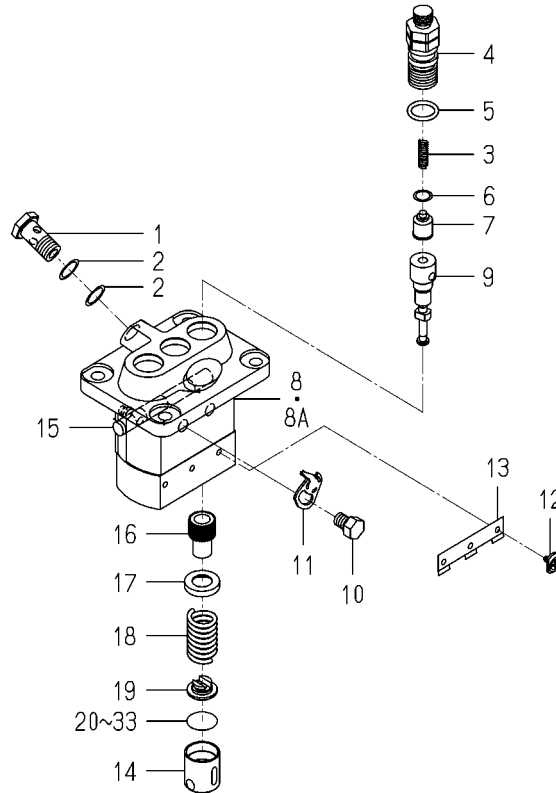
FIG. 27 COMPONENT PARTS FOR 6215-600-103-30 ON Fig.020
