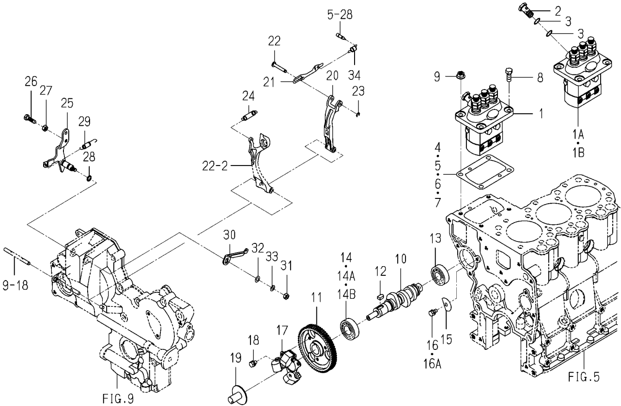
FIG. 20 INJECTION PUMP
