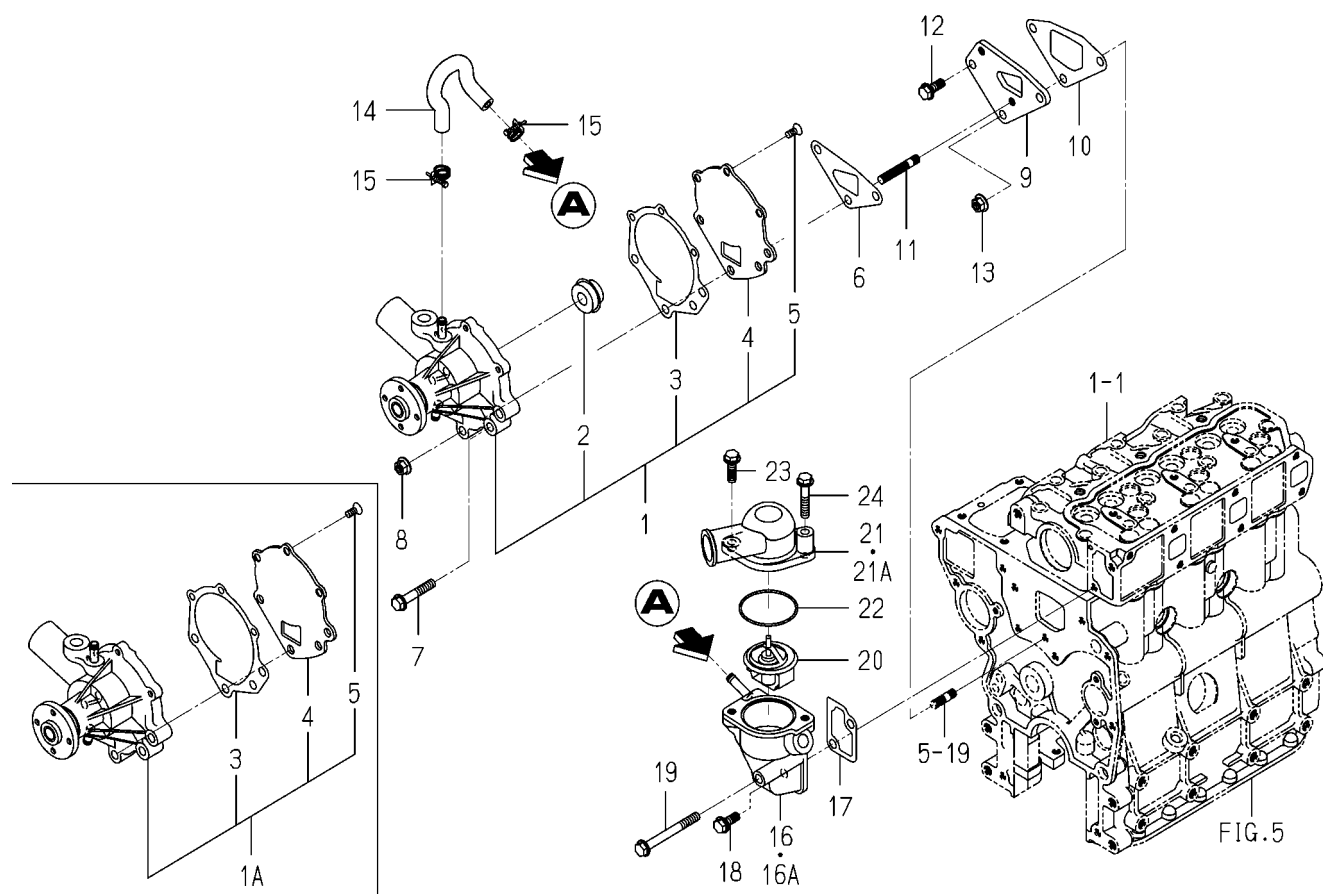
FIG. 17 WATER PUMP
