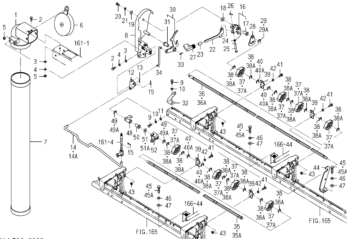
FIG.162 DISCHARGE SYSTEM(F TYPE)
