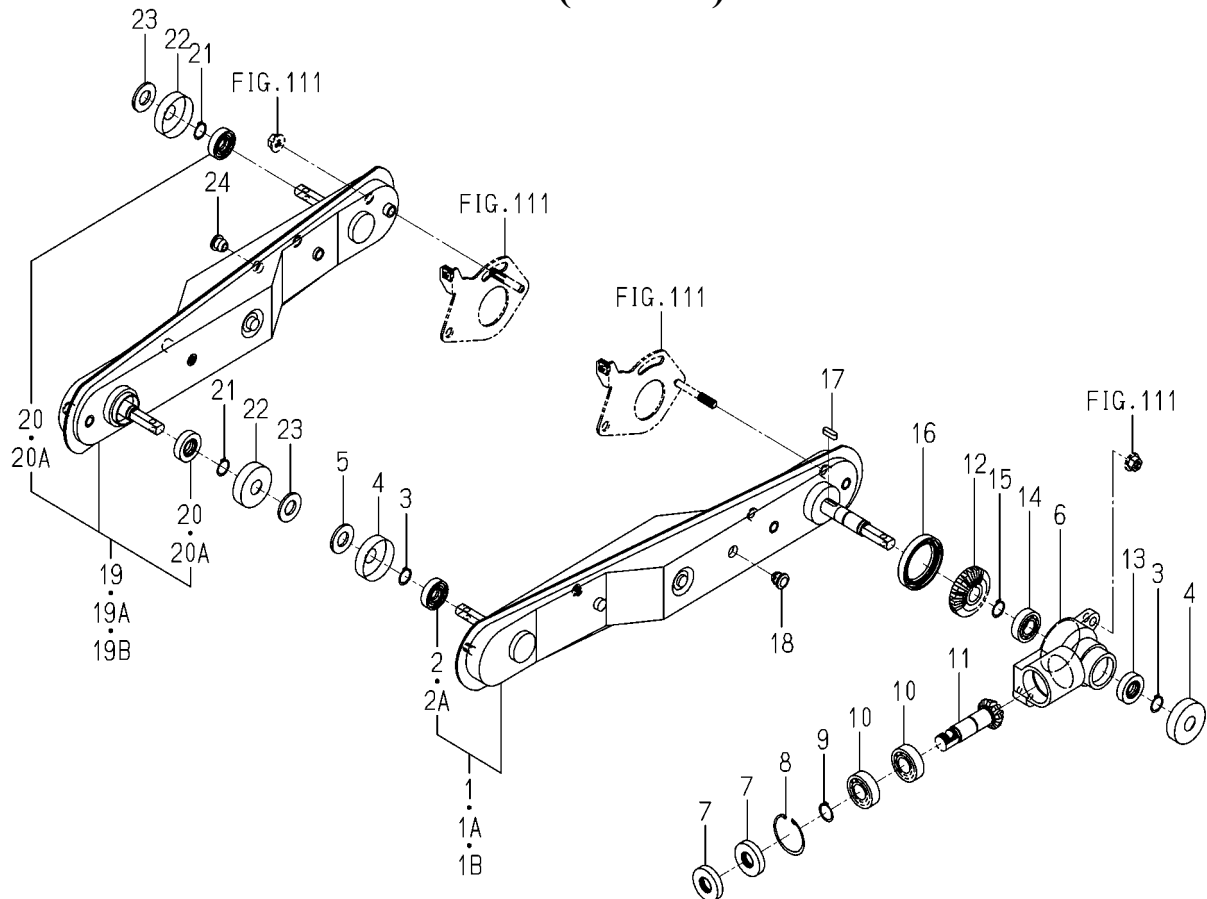
FIG.114 CASE(CHAIN)SYSTEM
