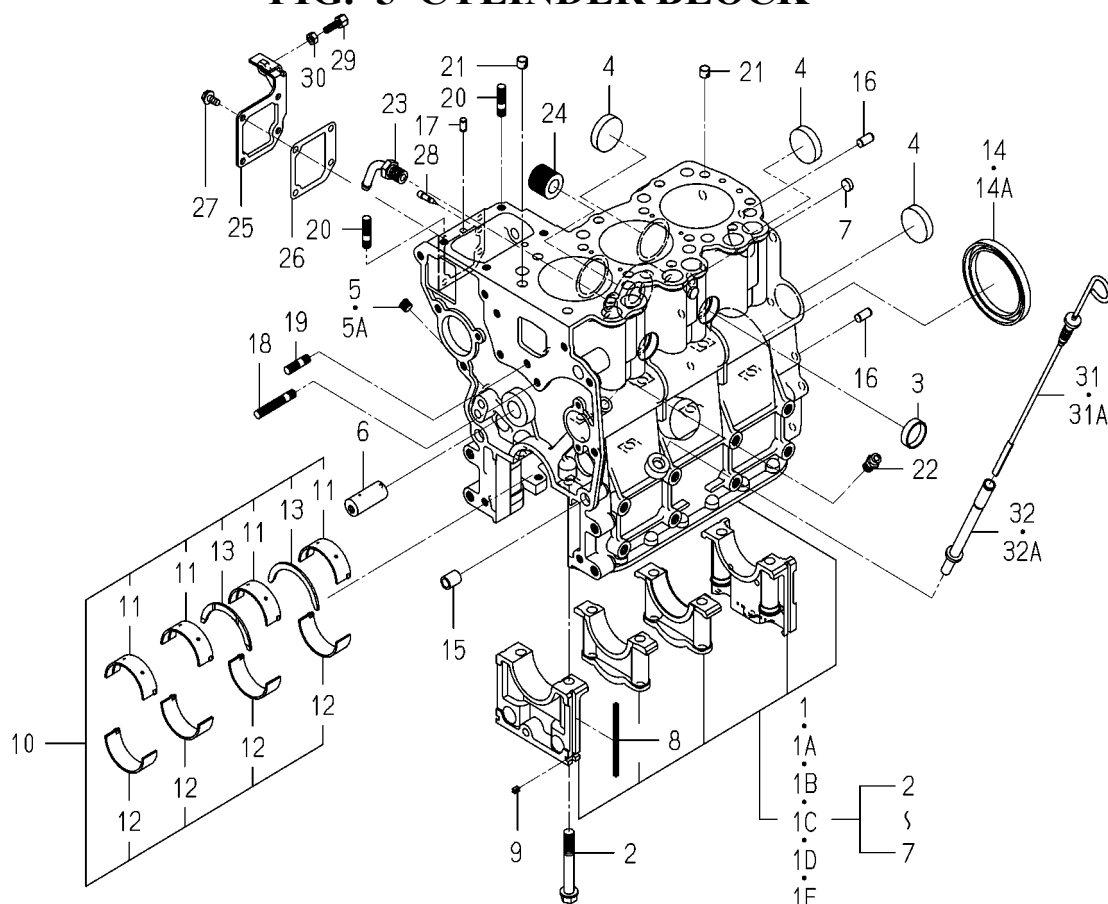
FIG. 5 CYLINDER BLOCK
