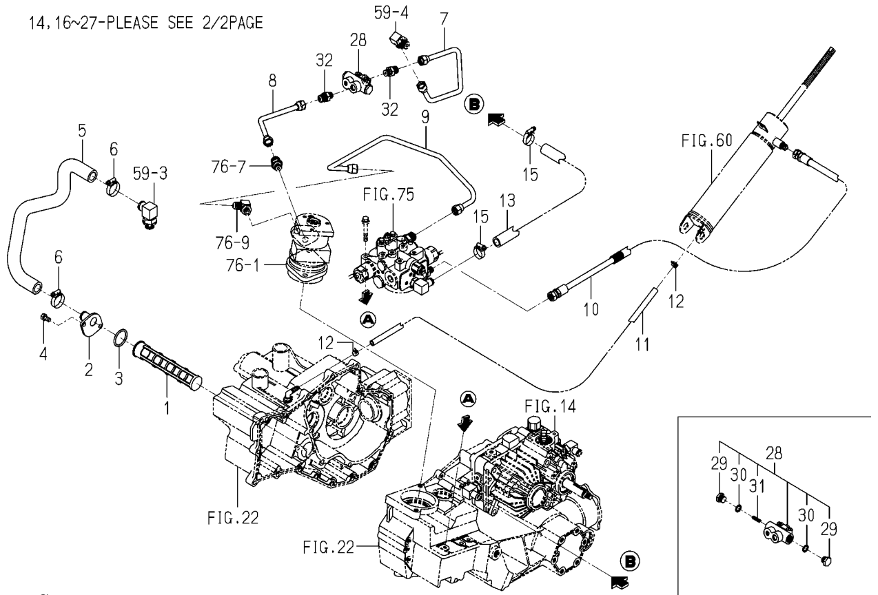
FIG. 62 PIPING SYSTEM(G TYPE)(1/2) (NO.100001-101046)
