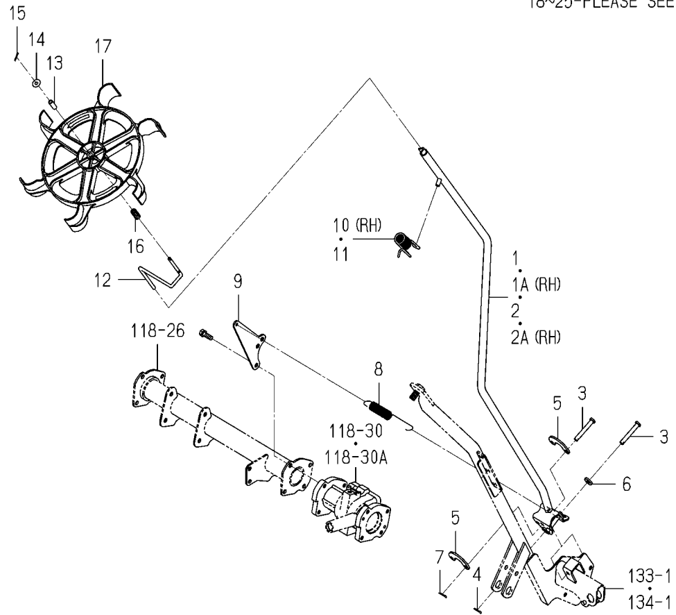
FIG.141 MARKER SYSTEM(1/2)
