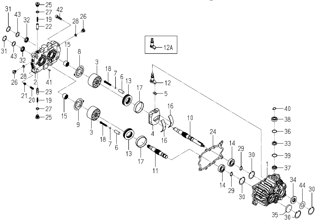
FIG.192 COMPONENT PARTS FOR K510-019-000-20 ON Fig.14□15
