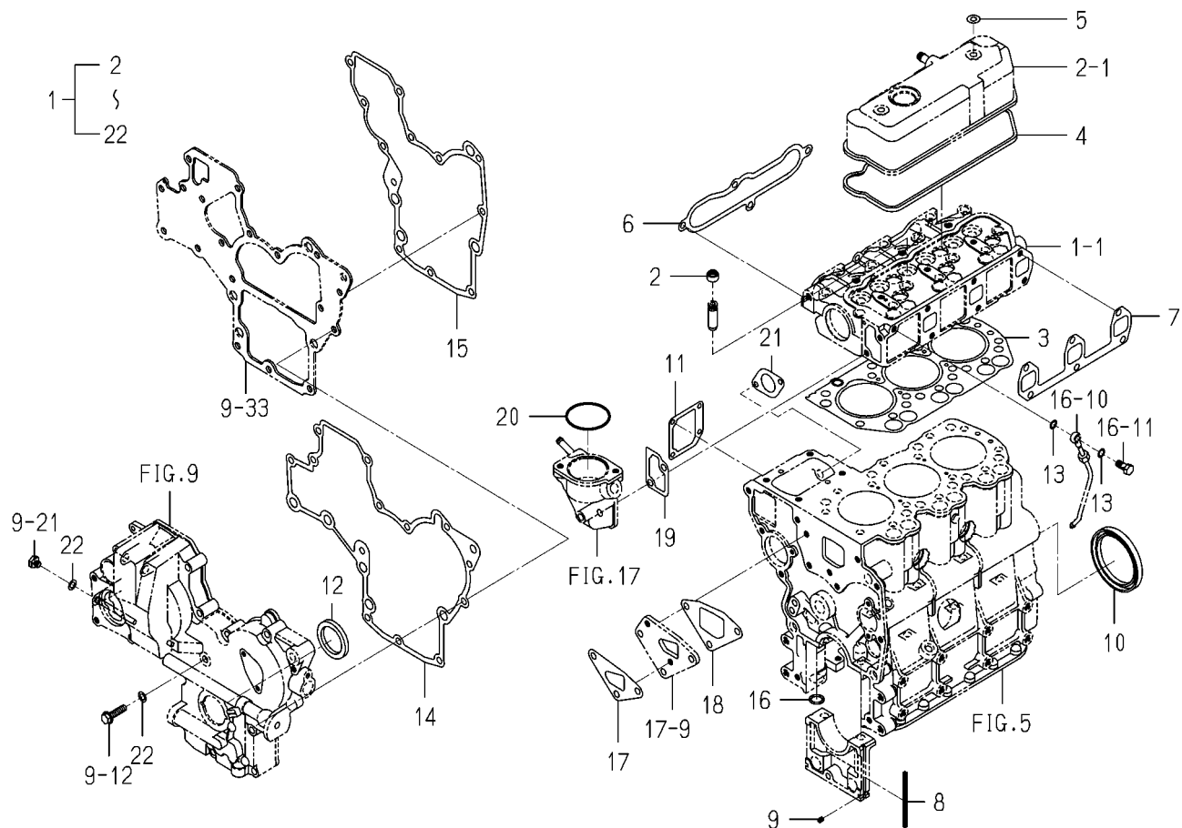
FIG. 25 REPAIR PARTS(OPTION)
