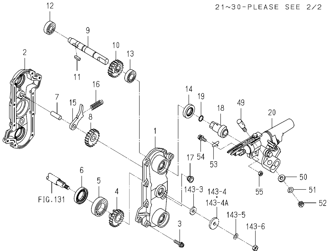
FIG.194 COMPONENT PARTS(1/2) FOR 2204-738-440-10 ON Fig.143
