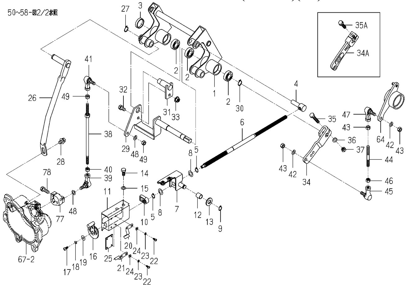
FIG.160 DRIVE SYSTEM(F TYPE)(1/2)
