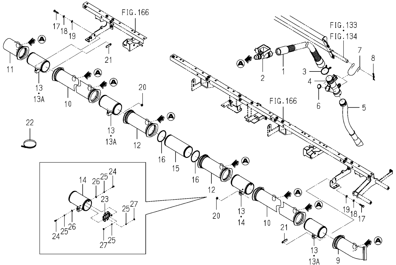
FIG.172 PIPING(FERTILIZER)SYSTEM(F TYPE)
