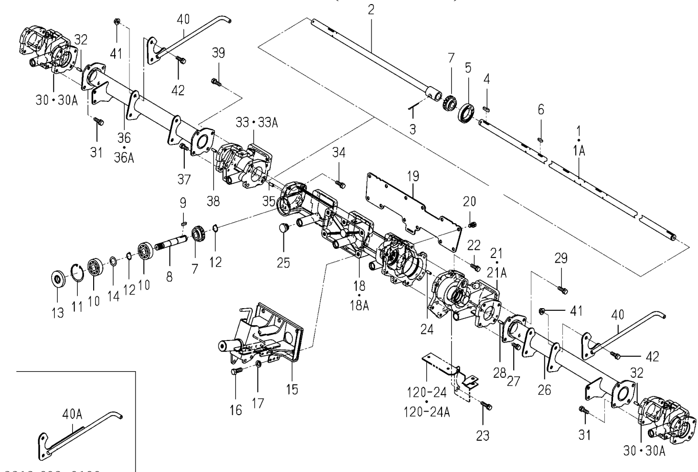
FIG.118 FRAME(PLANTING)SYSTEM
