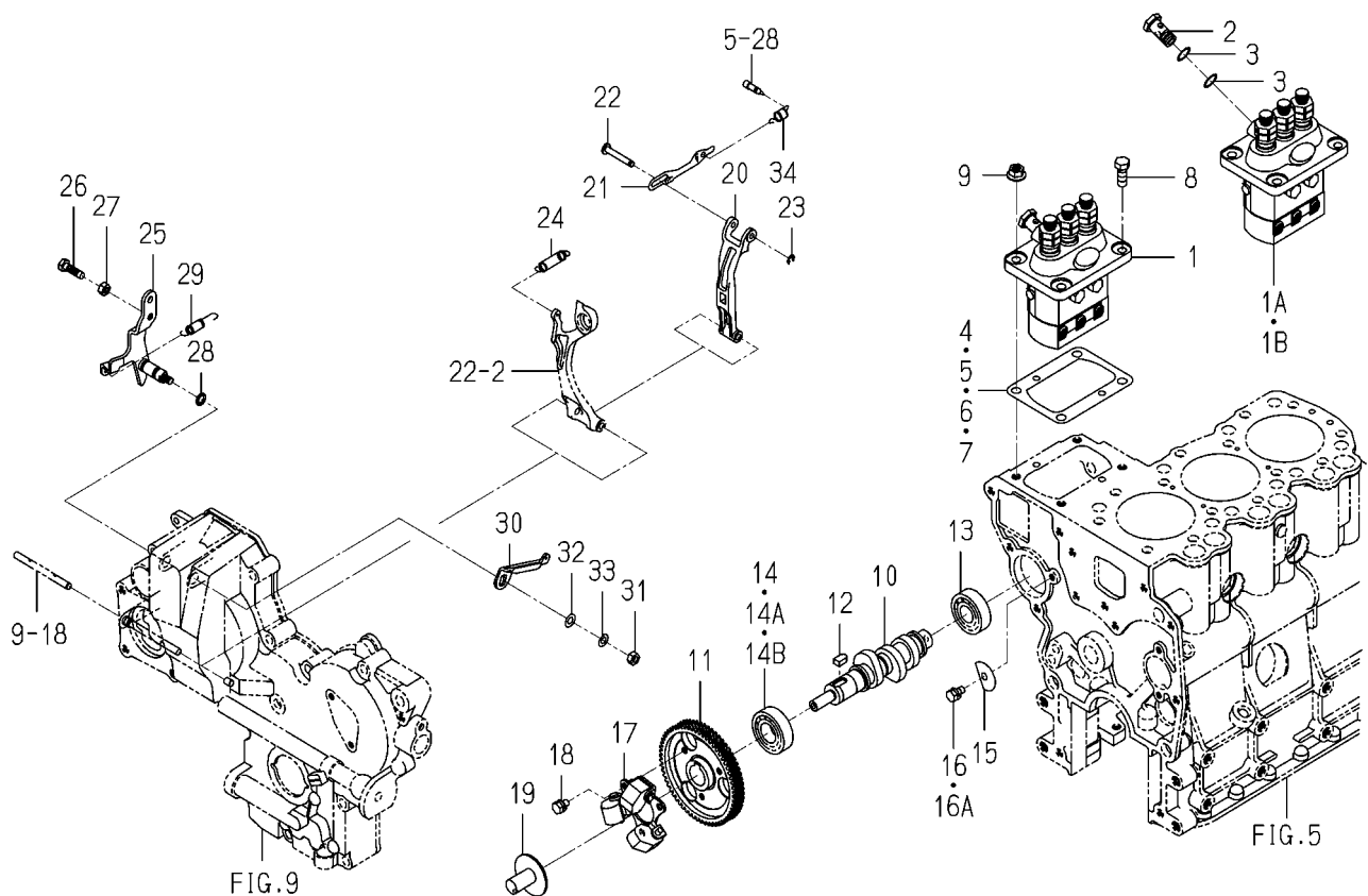
FIG. 20 INJECTION PUMP
