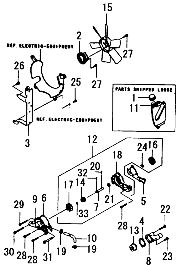
FIG. 5 COOLING-EQUIPMENT
