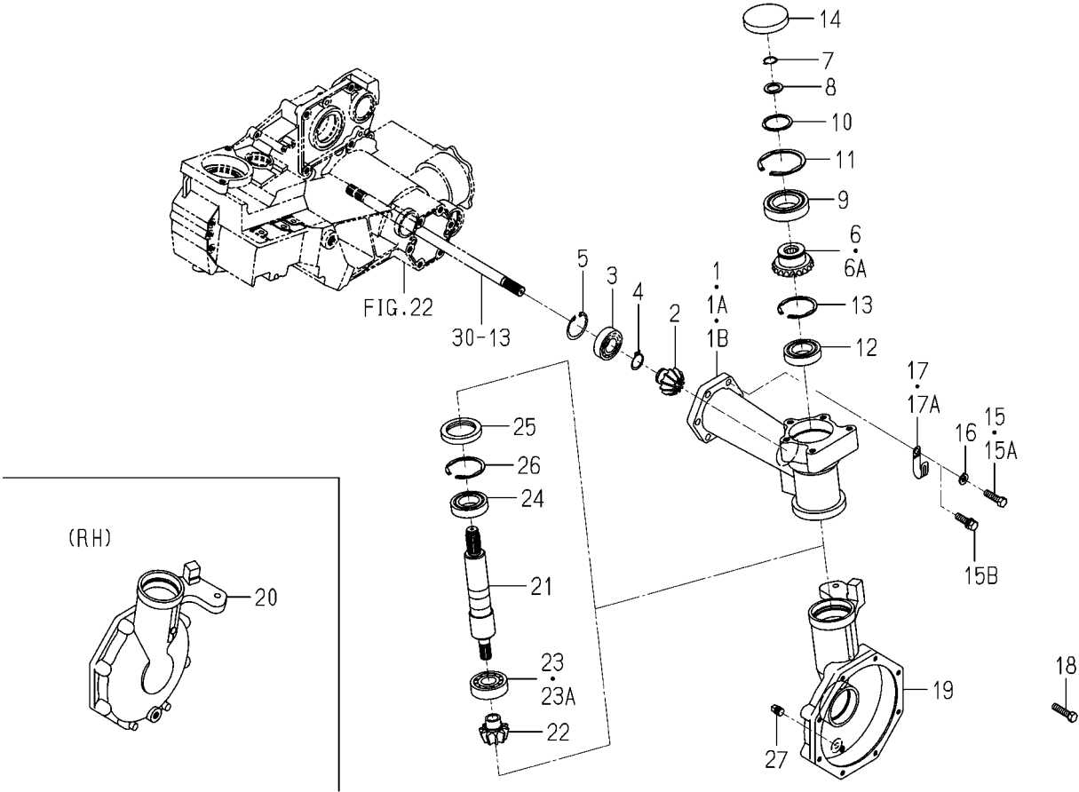
FIG. 41 CASE(FINAL)SYSTEM(D TYPE)
