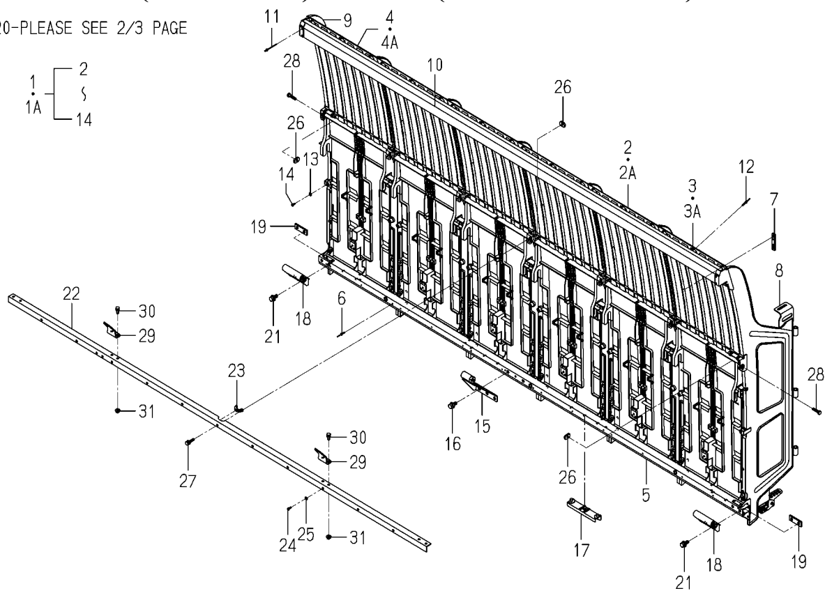
FIG.145 TANK(1/3) (SEEDLING)SYSTEM(NO.100001-101649)
