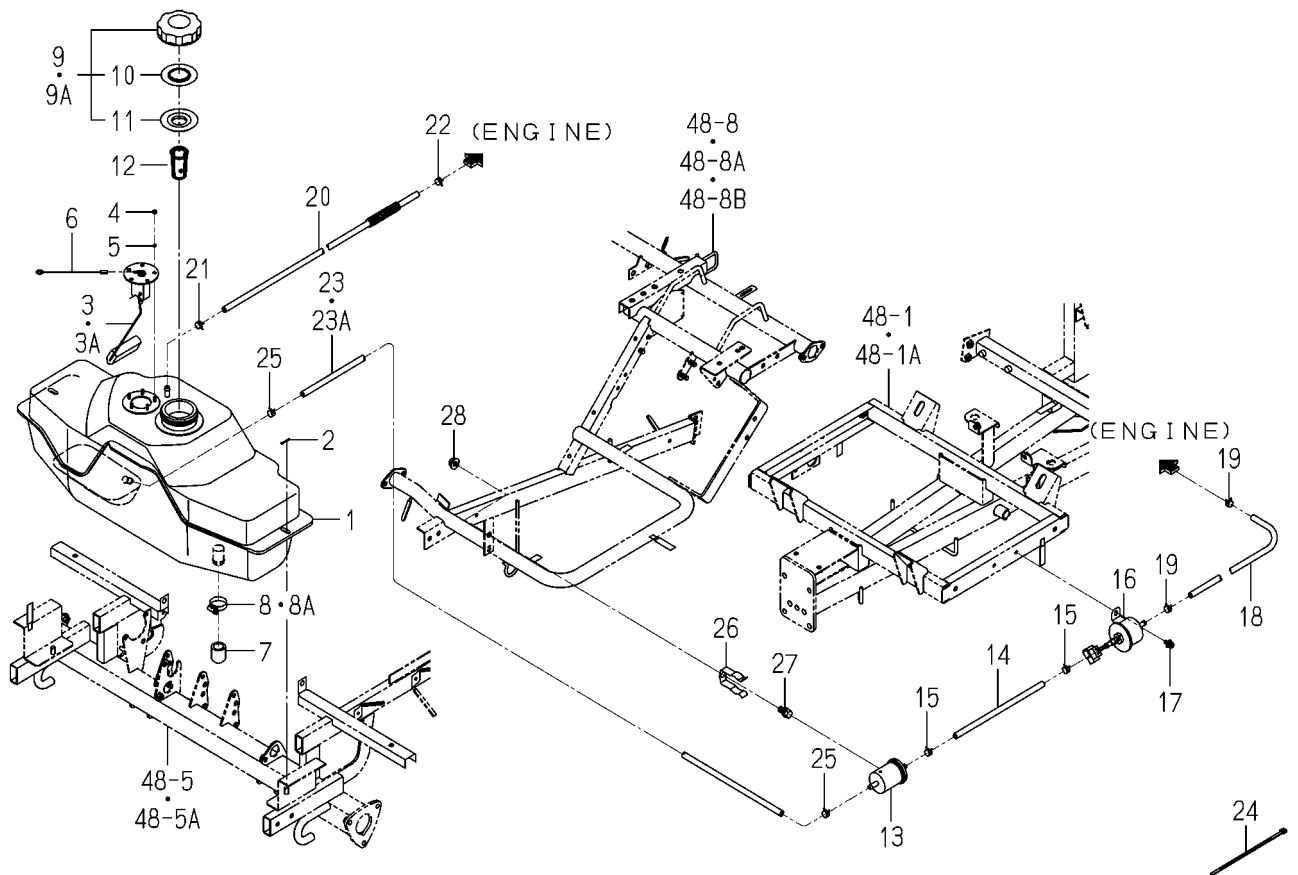
FIG. 11 TANK(FUEL)SYSTEM(D TYPE)
