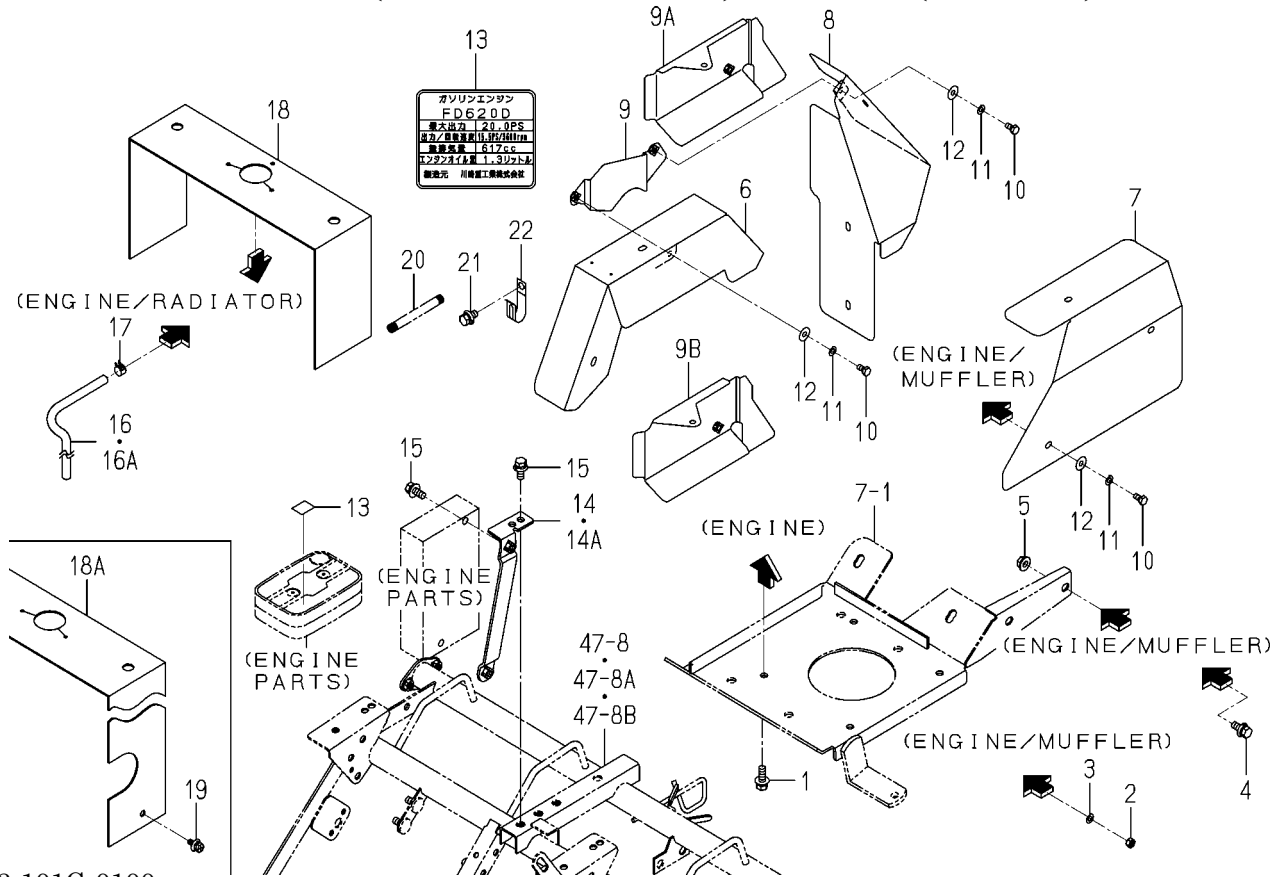
FIG. 4 BOLT(SET)⇔COVER(MUFFLER⇔RADIATOR) & LABEL(MODEL/ENGINE)SYSTEM(G TYPE)
