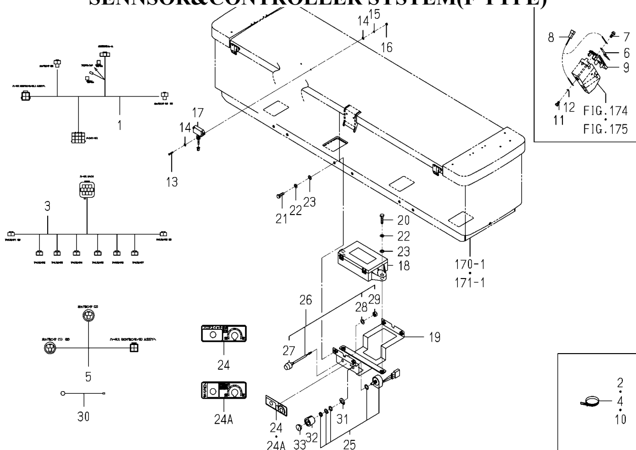
FIG.163 HARNESS, SENNSOR&CONTROLLER SYSTEM(F TYPE)
