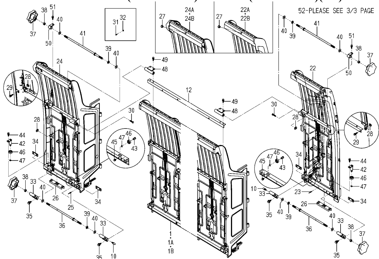
FIG.146 TANK(SEEDLING)SYSTEM(NO.101650-)(2/3)
