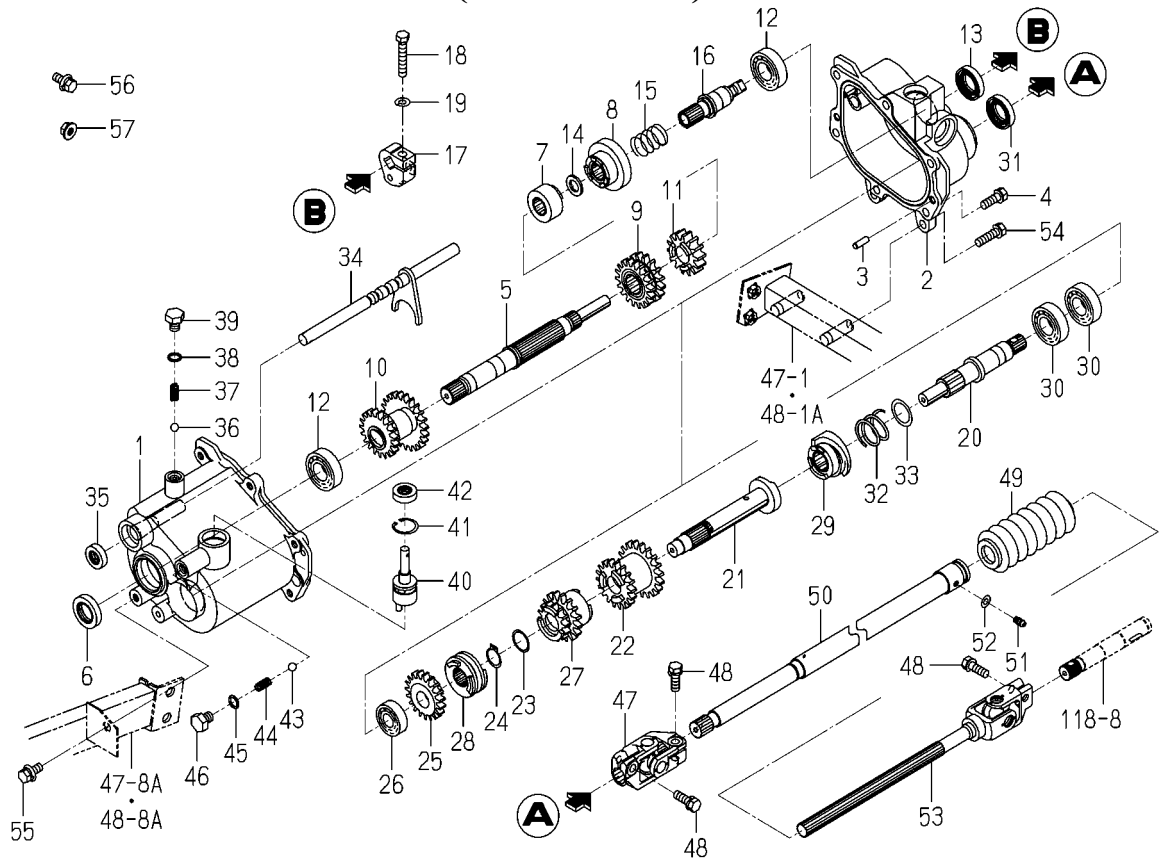
FIG. 69 (F TYPE)(NO.101047-) CASE(PLANTING)SYSTEM
