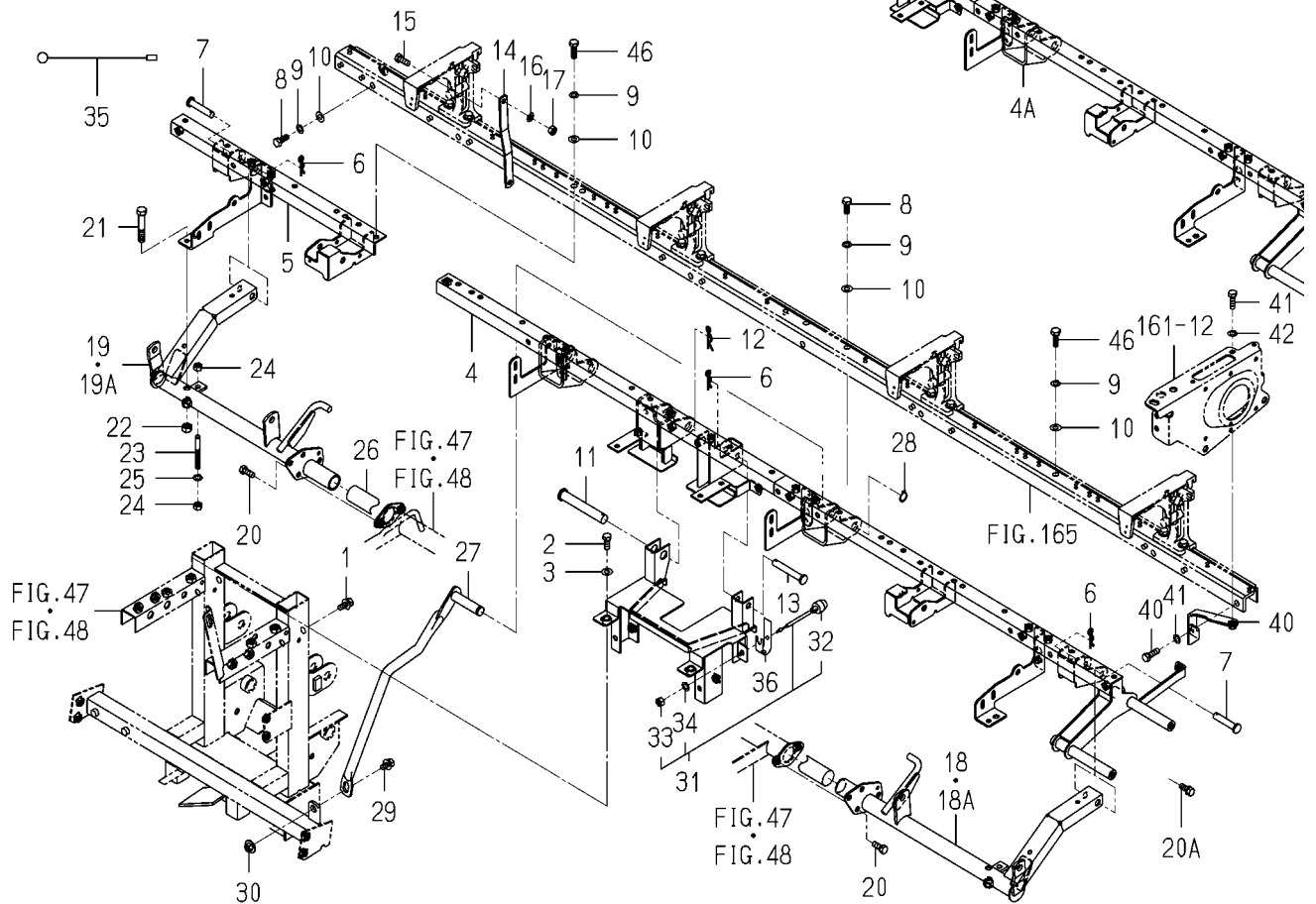
FIG.166 FRAME(FERTILIZER)SYSTEM(F TYPE)(1/2)
