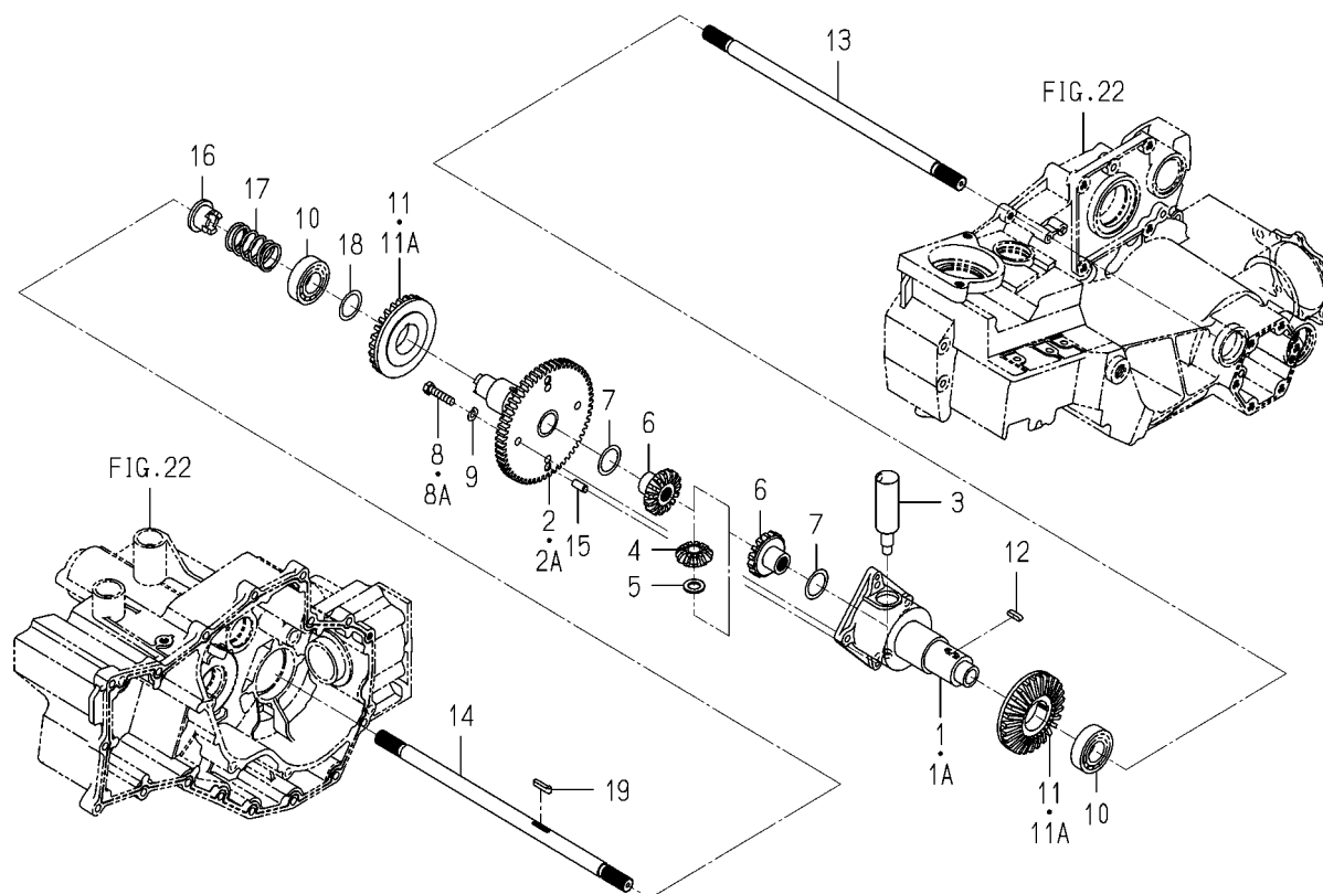
FIG. 29 SHAFT(DRIVE/FRONT)SYSTEM (NO.100001-102349)
