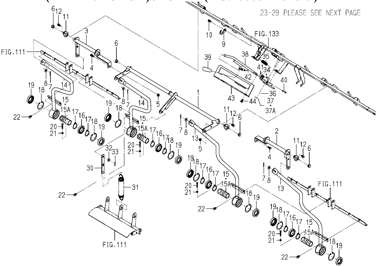
FIG.113 LEVER(1/2) (DEPTH/ROTOR)SYSTEM(NO.100001-101649)
