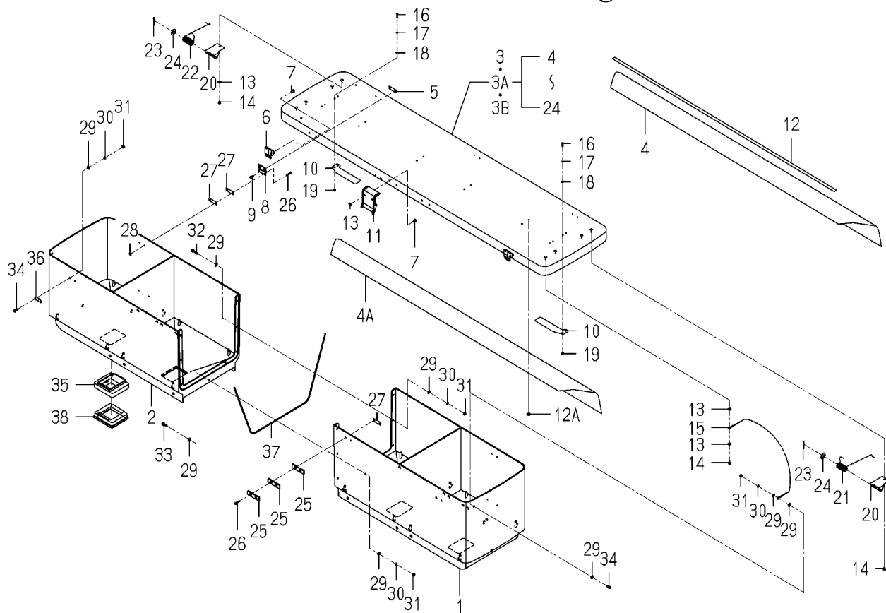
FIG.198 COMPONENT PARTS FOR 8844-718-310-40 ON Fig.171
