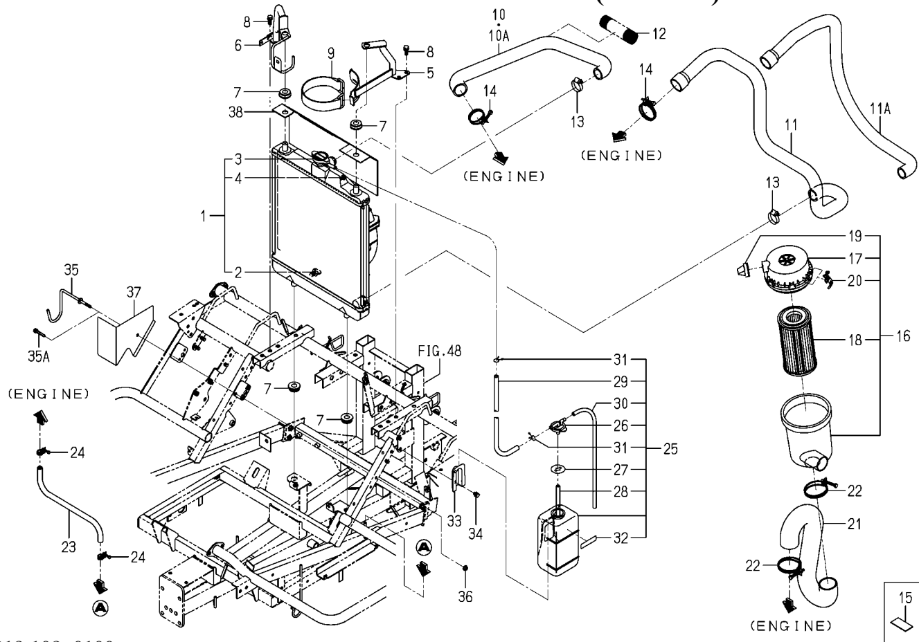
FIG. 5 RADIATOR SYSTEM(D TYPE)
