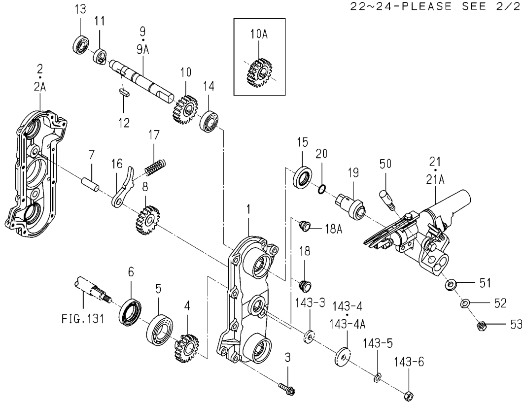
FIG.193 COMPONENT PARTS(1/2) FOR 2204-738-400-90 ON Fig.143
