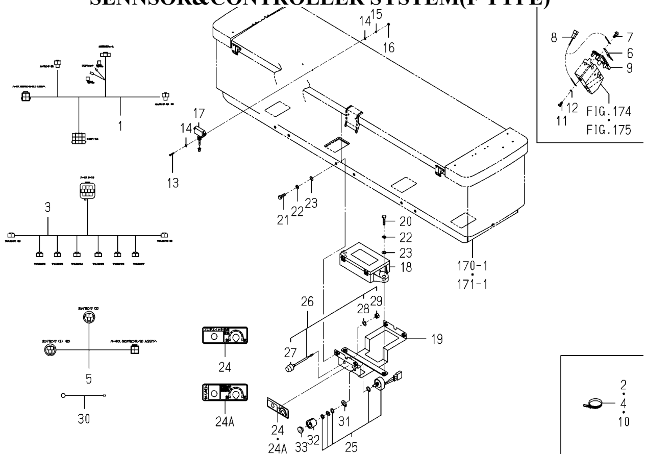
FIG.163 HARNESS, SENNOR&CONTROLLER SYSTEM(F TYPE)
