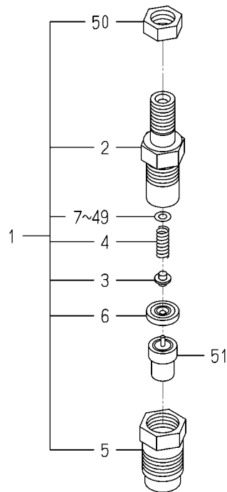
FIG. 26 COMPONENT PARTS FOR 6215-300-036-10 ON Fig.019
