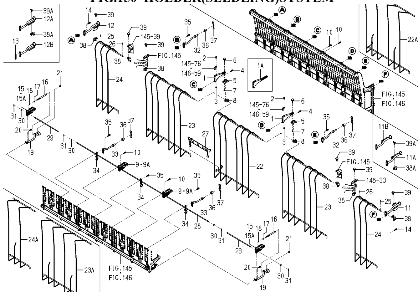
FIG.150 HOLDER(SEEDLING)SYSTEM
