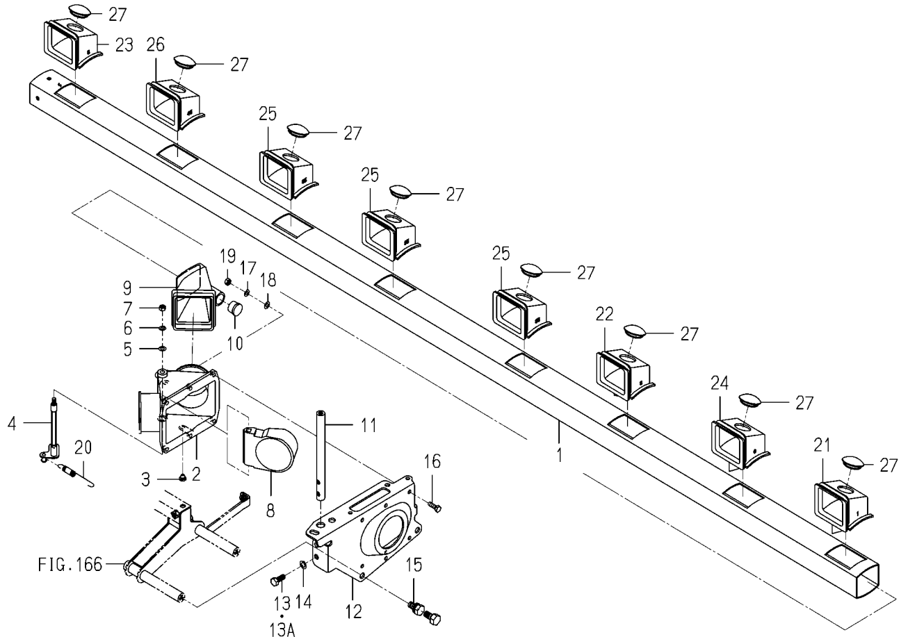
FIG.161 AIR CHAMBER SYSTEM(F TYPE)
