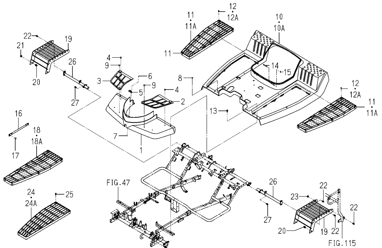
FIG. 80 STEP(MAIN)SYSTEM(G-F TYPE)
