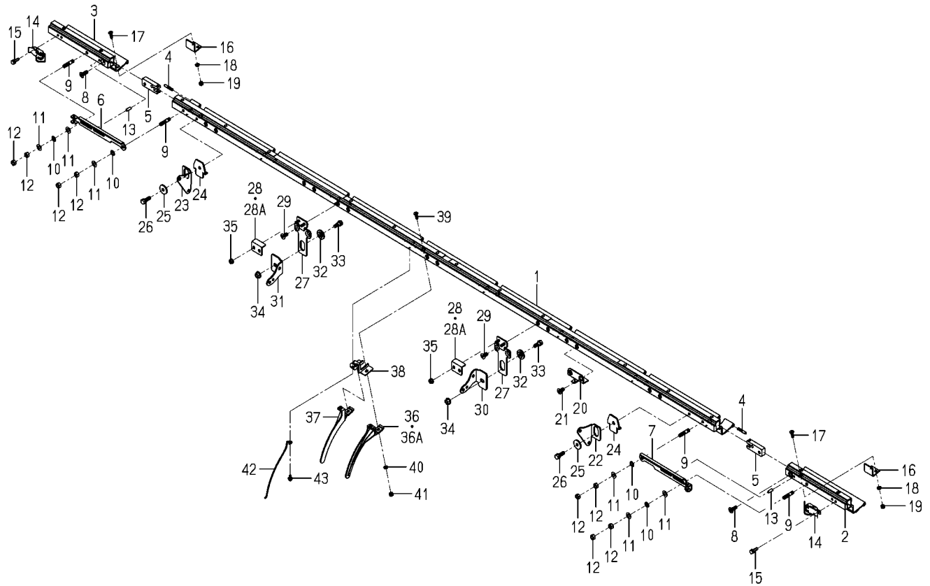
FIG.149 PLATE(FRONT)SYSTEM(NO.101650-)
