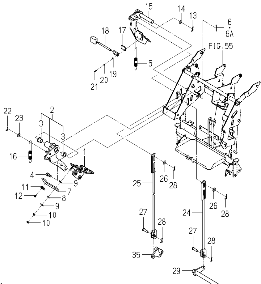
FIG. 56 PEDAL(BRAKE)SYSTEM(1/3)
