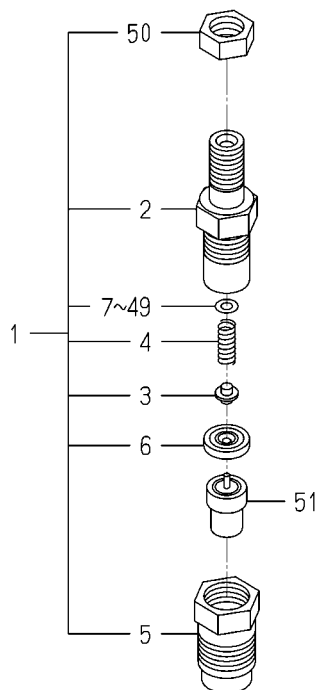
FIG. 26 COMPONENT PARTS FOR 6215-300-036-10 ON Fig.019
