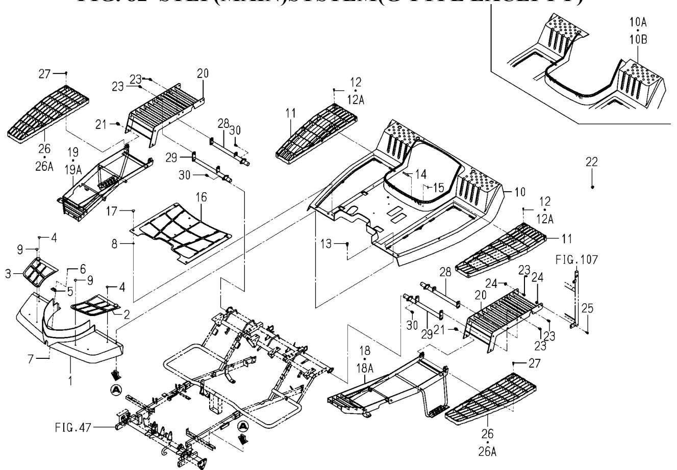
FIG. 82 STEP(MAIN)SYSTEM(G TYPE EXCEPT F)
