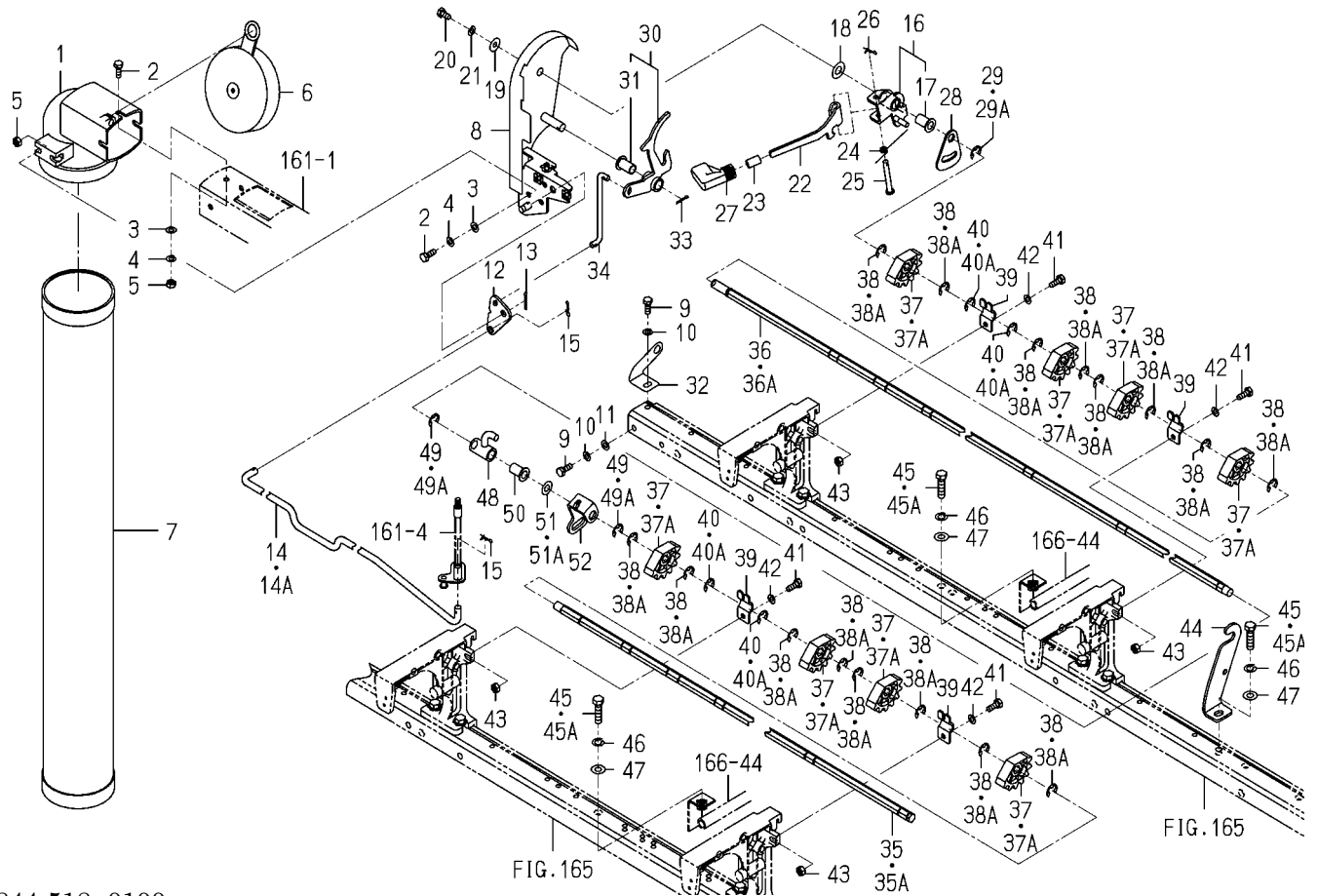
FIG.162 DISCHARGE SYSTEM(F TYPE)
