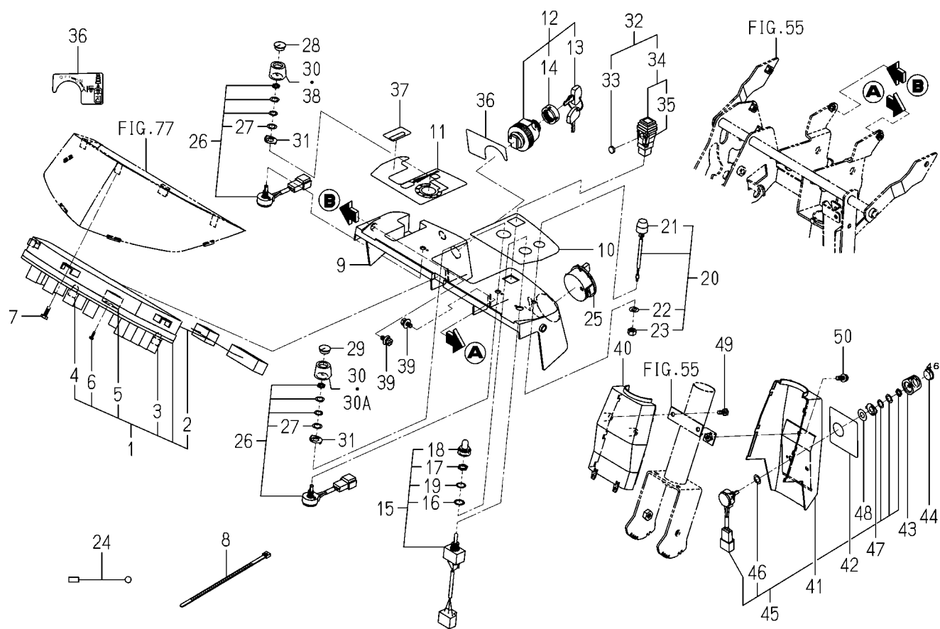
FIG. 96 PANEL(INSTRUMENT)SYSTEM(G TYPE)
