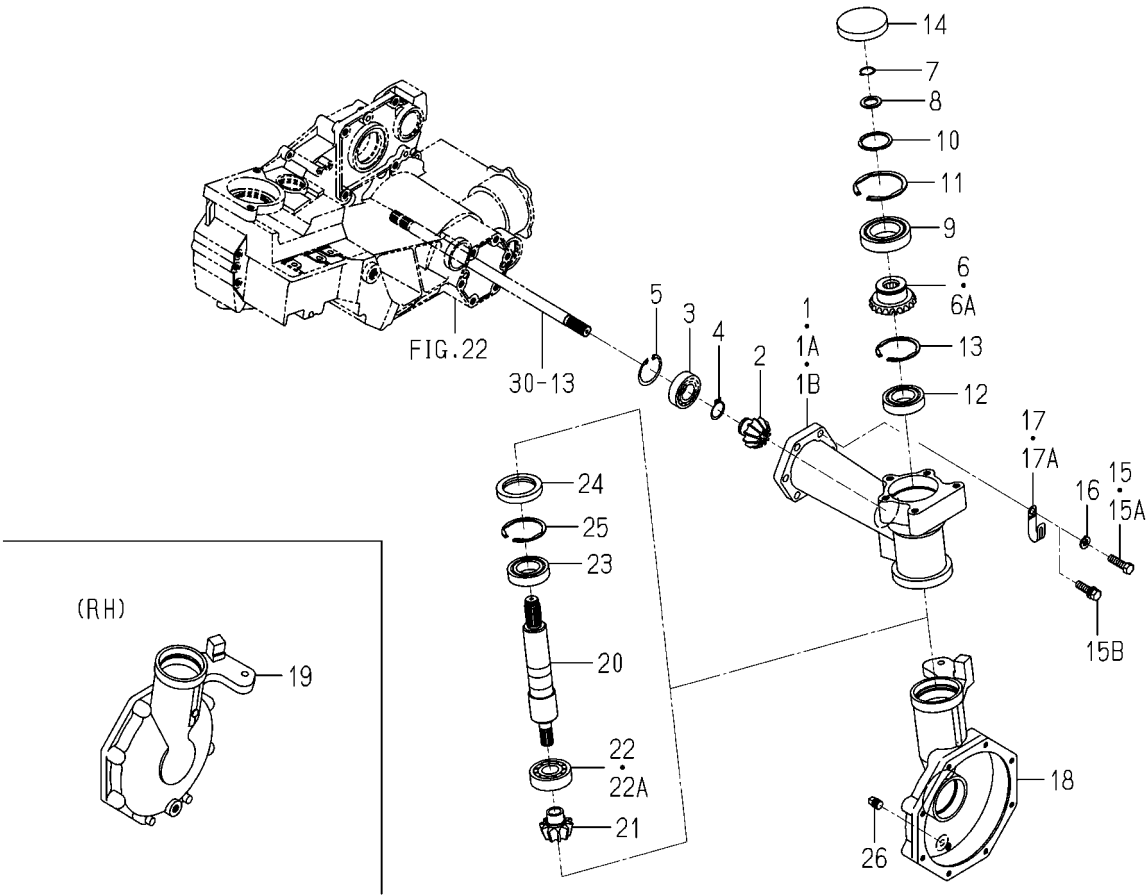
FIG. 42 CASE(FINAL)SYSTEM(G TYPE)
