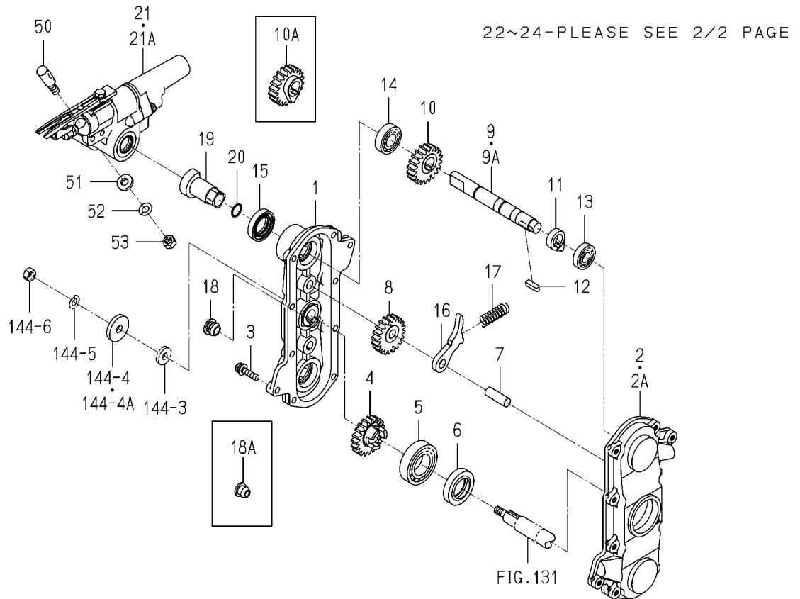
FIG.195 COMPONENT PARTS(1/2) FOR 2204-739-400-90 ON Fig.144
