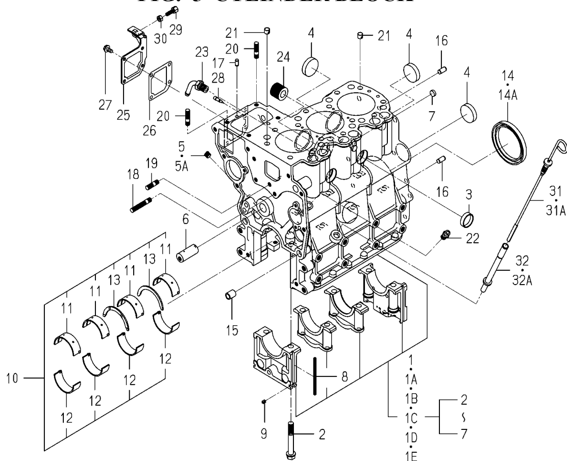
FIG. 5 CYLINDER BLOCK
