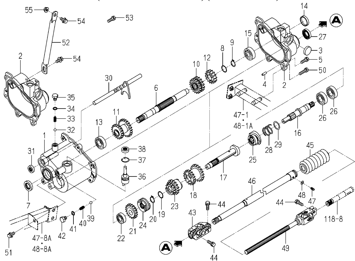
FIG. 70 CASE(PLANTING)SYSTEM (EXCEPT F TYPE)(NO.101047-)
