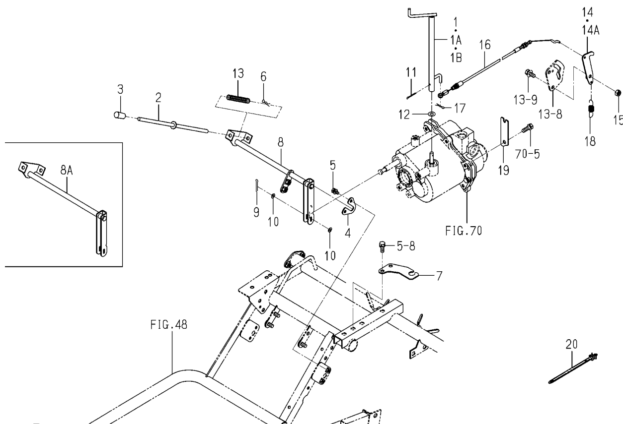
FIG. 73 LEVER (PLANTING INTERVAL)SYSTEM(D TYPE)
