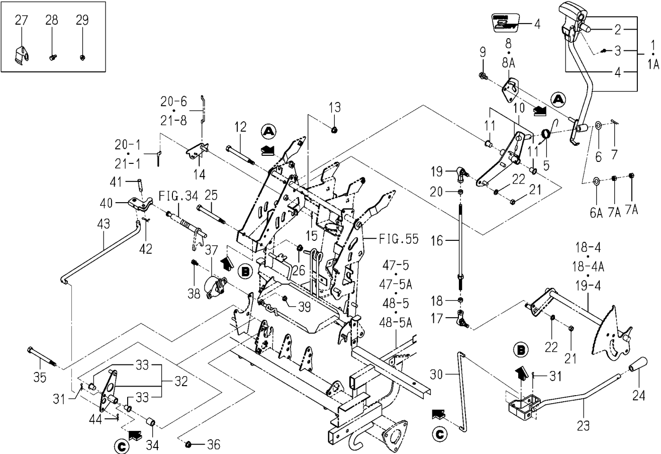
FIG. 13 LEVER(HST)SYSTEM
