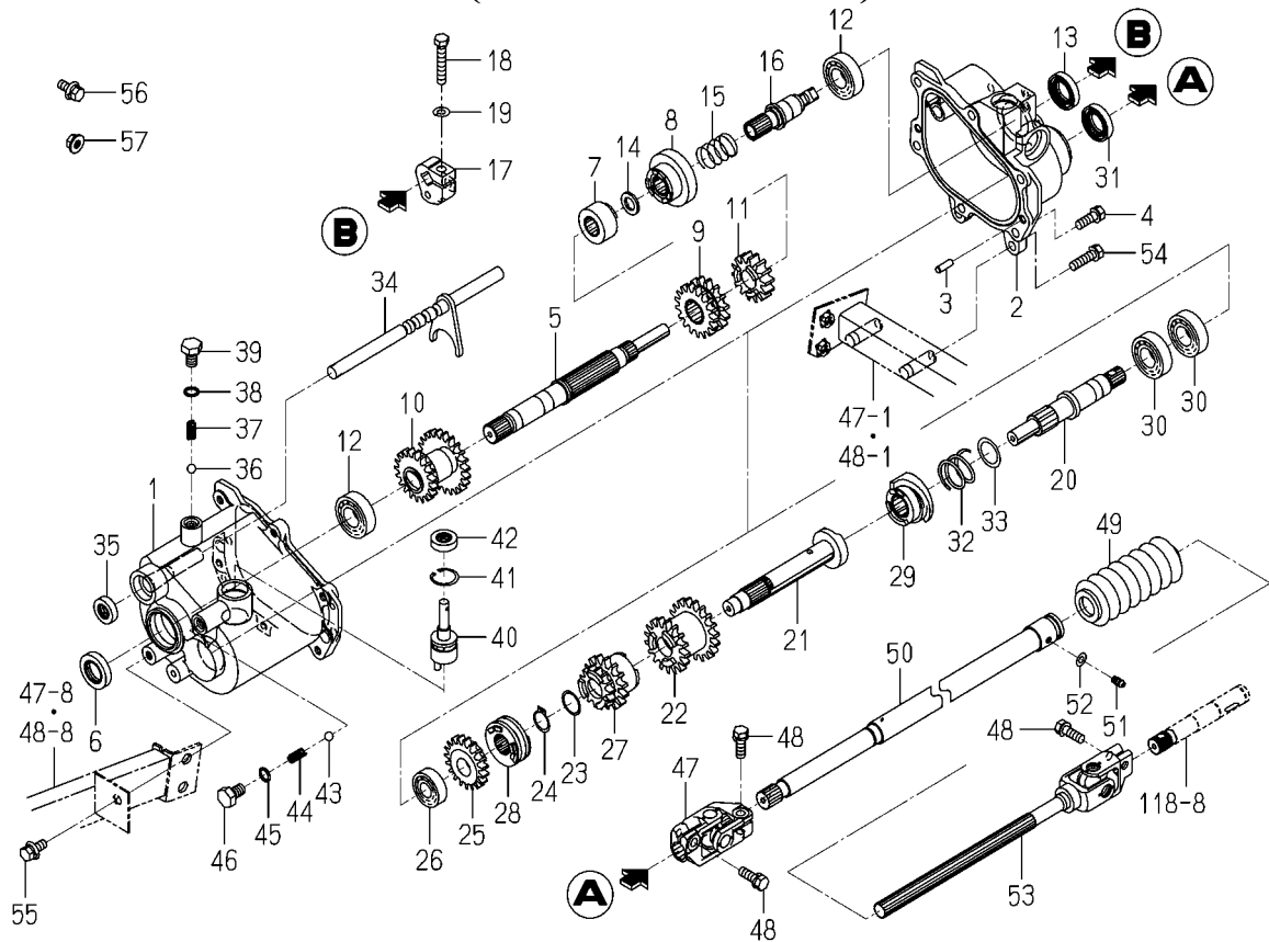
FIG. 67 CASE(PLANTING)SYSTEM(F TYPE) (NO.100001-101046)
