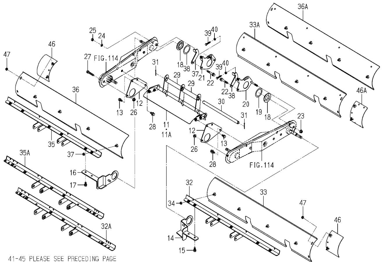
FIG.111 ROTOR SYSTEM(2/2)
