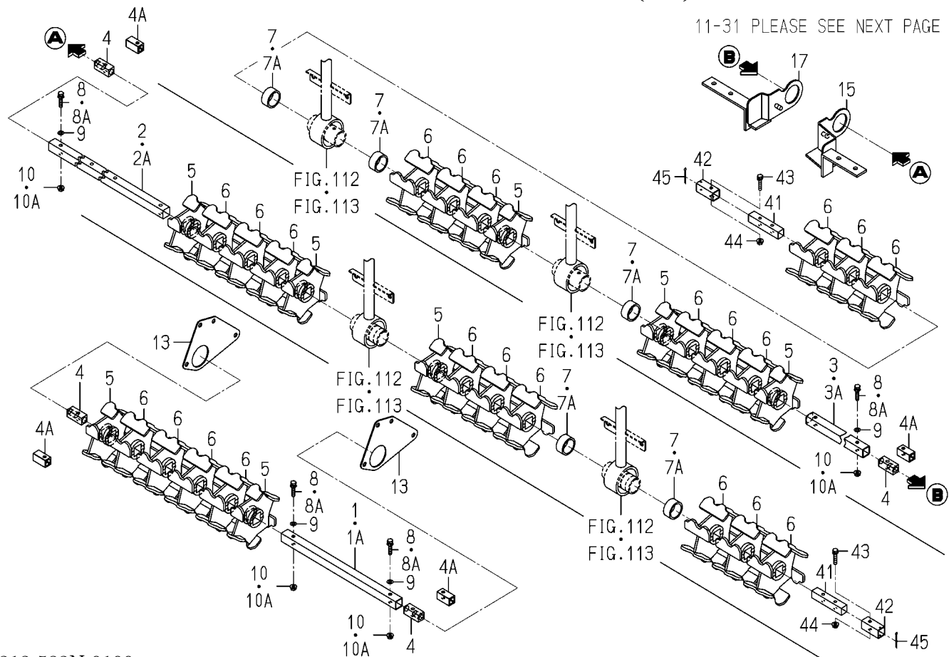
FIG.111 ROTOR SYSTEM(1/2)
