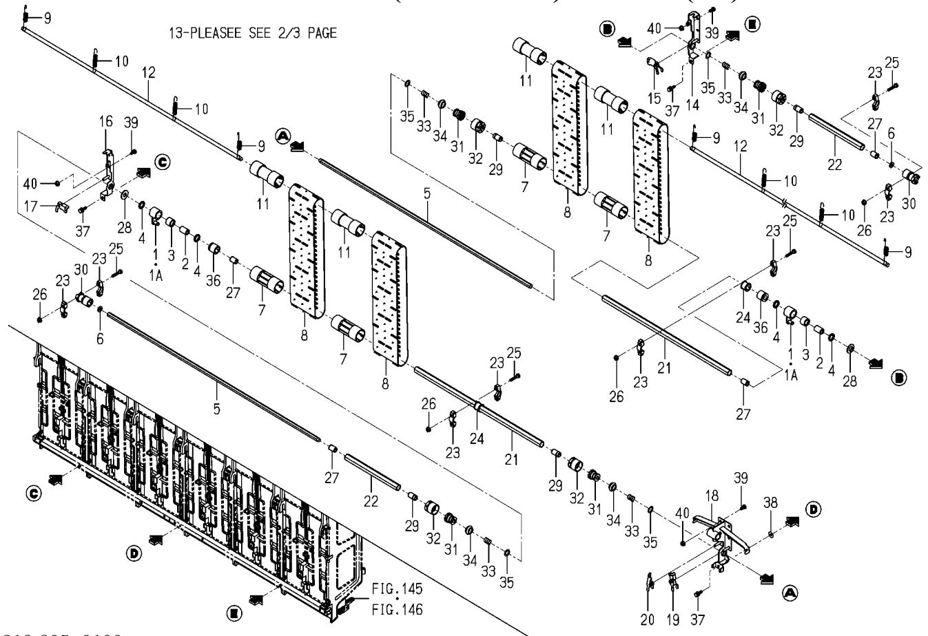
FIG.151 FEED(SEEDLING)SYSTEM(1/3)
