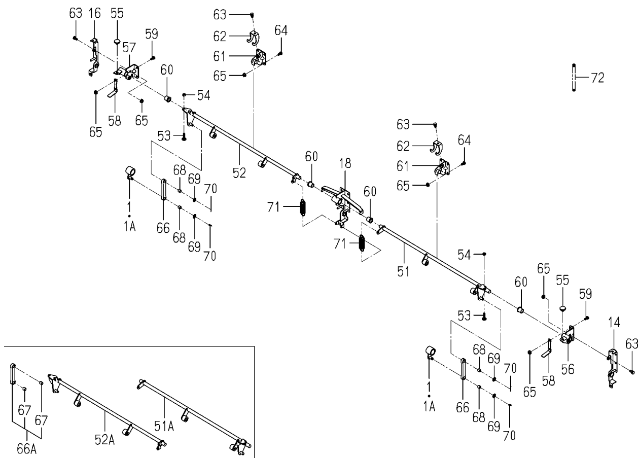
FIG.151 FEED(SEEDLING)SYSTEM(3/3)
