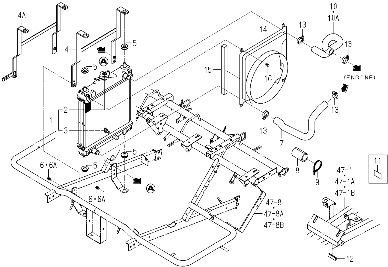
FIG. 6 RADIATOR SYSTEM(G TYPE)
