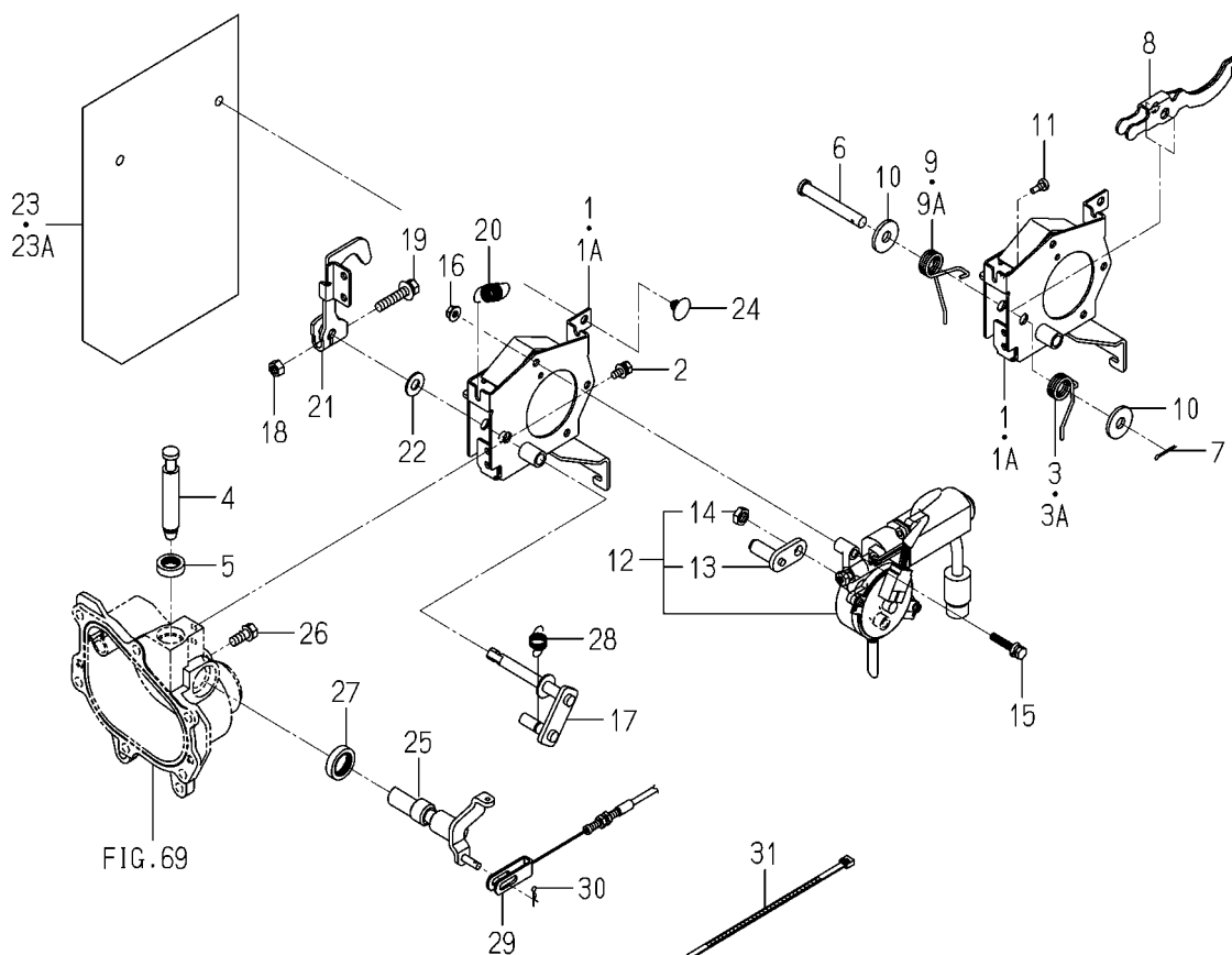
FIG. 72 MOTOR(PLANTING)SYSTEM(F TYPE)
