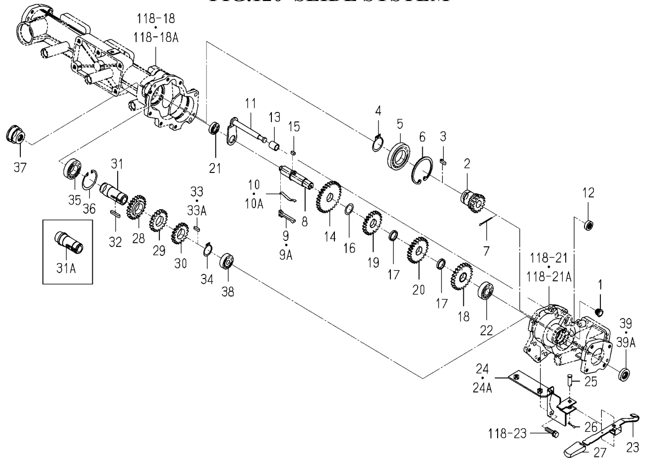
FIG.120 SLIDE SYSTEM
