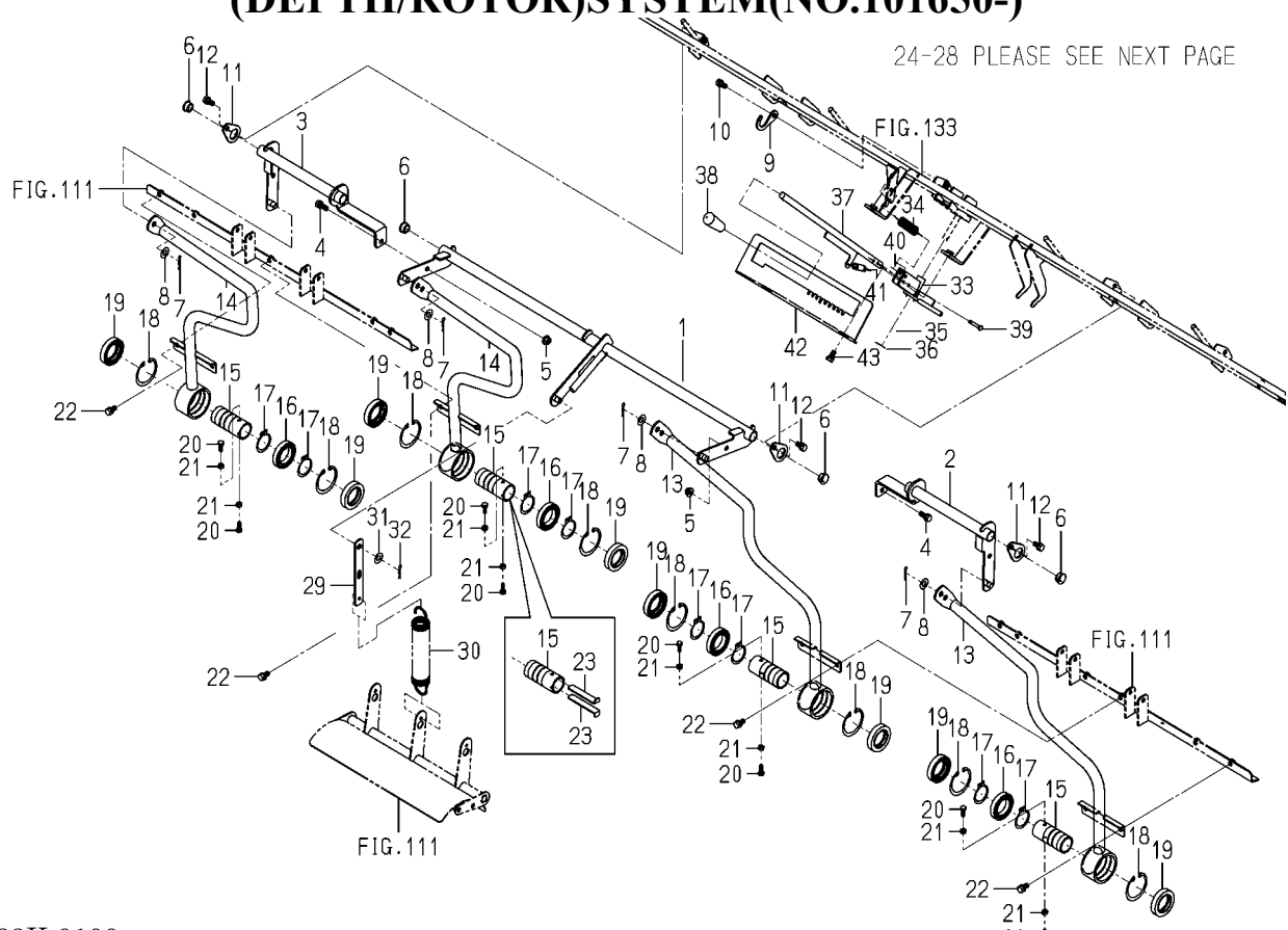
FIG.112 LEVER(1/2) (DEPTH/ROTOR)SYSTEM(NO.101650-)
