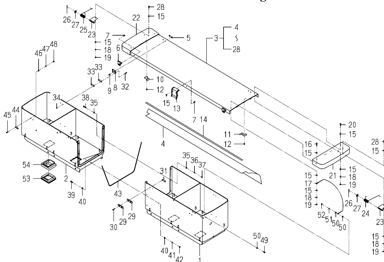
FIG.197 COMPONENT PARTS FOR 8844-718-200-10 ON Fig.170
