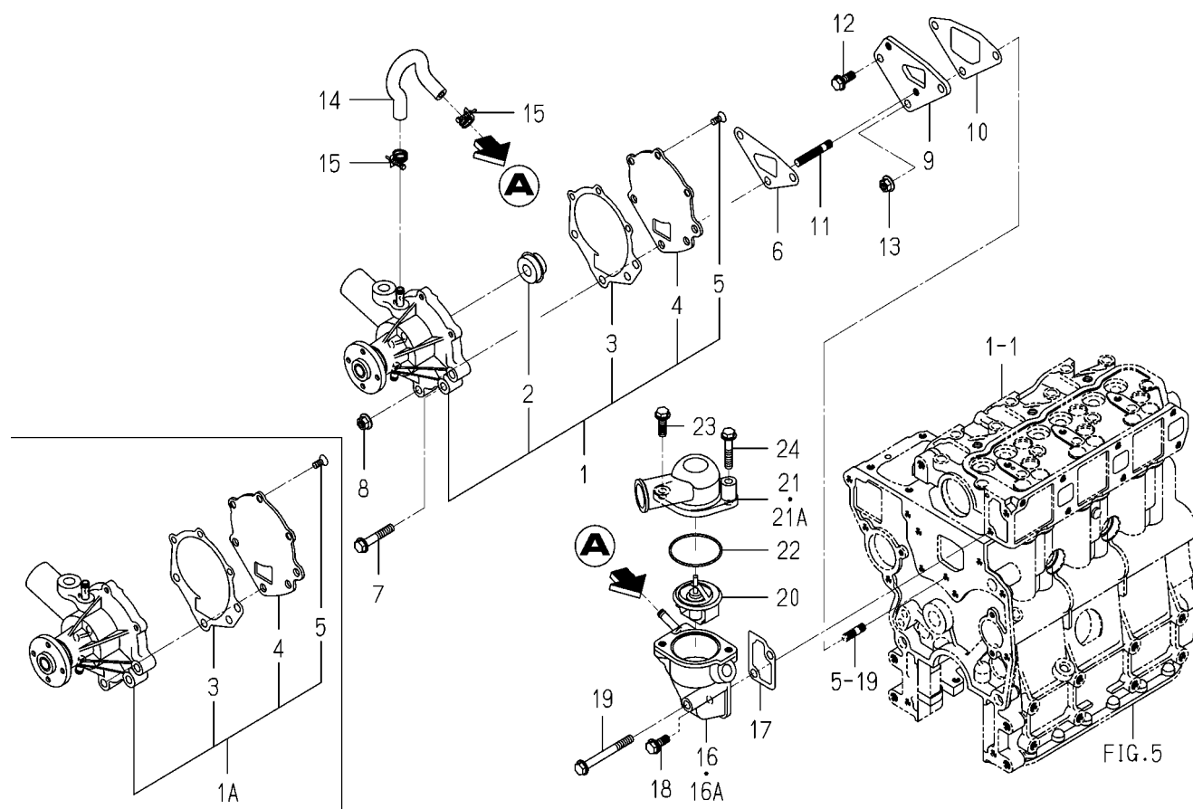
FIG. 17 WATER PUMP
