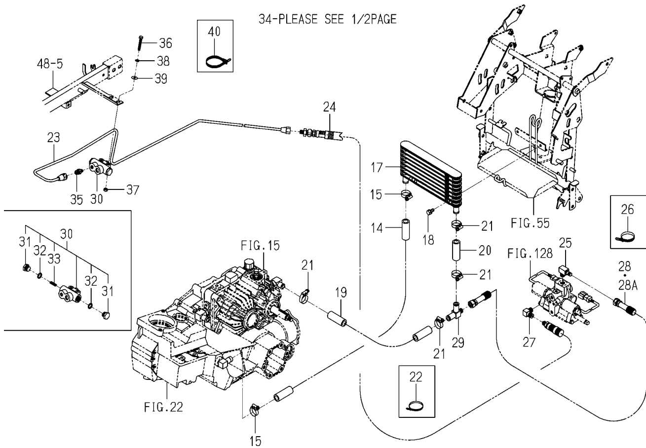
FIG. 61 PIPING SYSTEM(D TYPE)(2/2)
