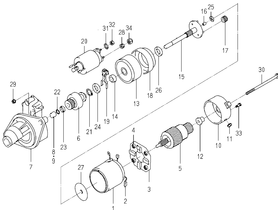
FIG. 28 COMPONENT PARTS FOR 6281-100-014-00 ON Fig.023
