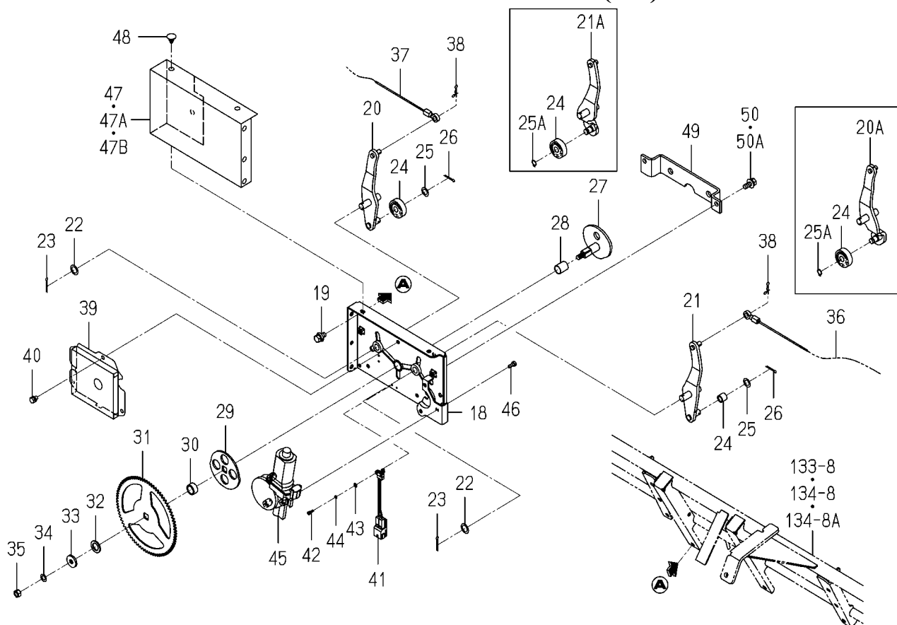
FIG.141 MARKER SYSTEM(2/2)
