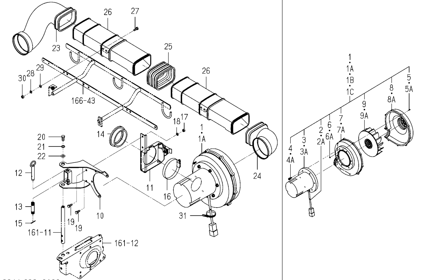
FIG.167 BLOWER SYSTEM(F TYPE)
