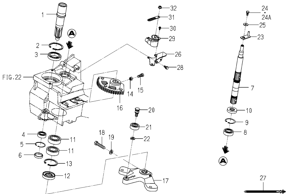
FIG. 38 STEERING SYSTEM
