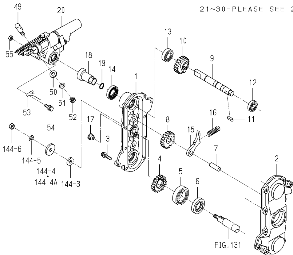
FIG.196 COMPONENT PARTS(1/2) FOR 2204-739-440-10 ON Fig.144
