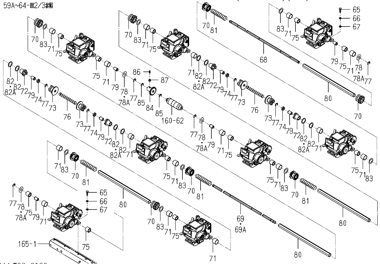
FIG.169 SEND OUT SYSTEM(F TYPE)(3/3)
