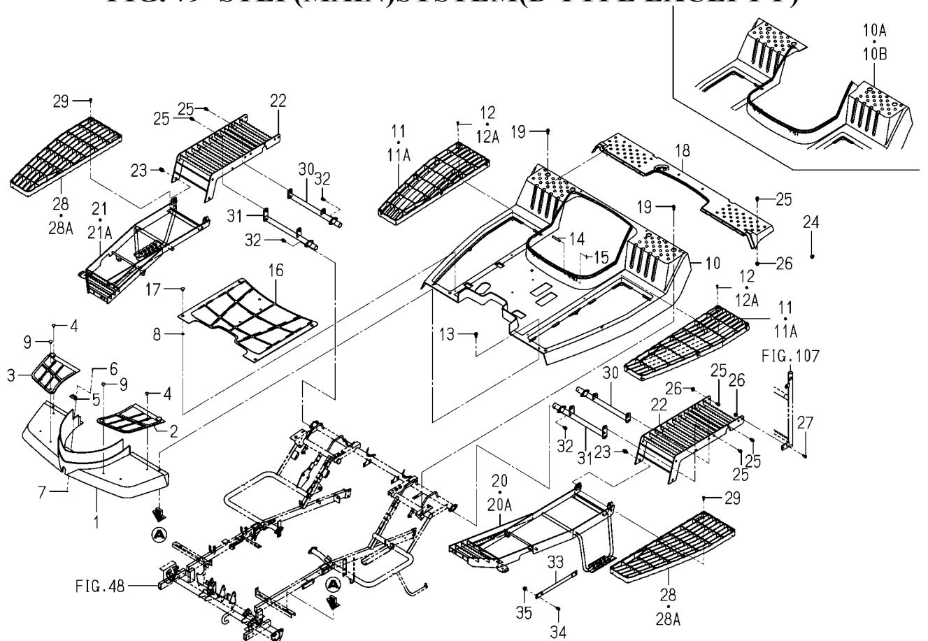
FIG. 79 STEP(MAIN)SYSTEM(D TYPE EXCEPT F)
