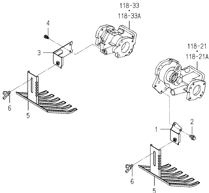
FIG.129 RAKE SYSTEM
