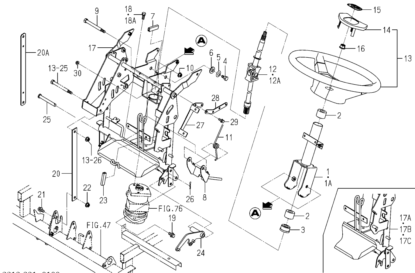
FIG. 55 WHEEL(STEERING)SYSTEM
