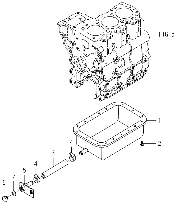
FIG. 7 OIL PAN
