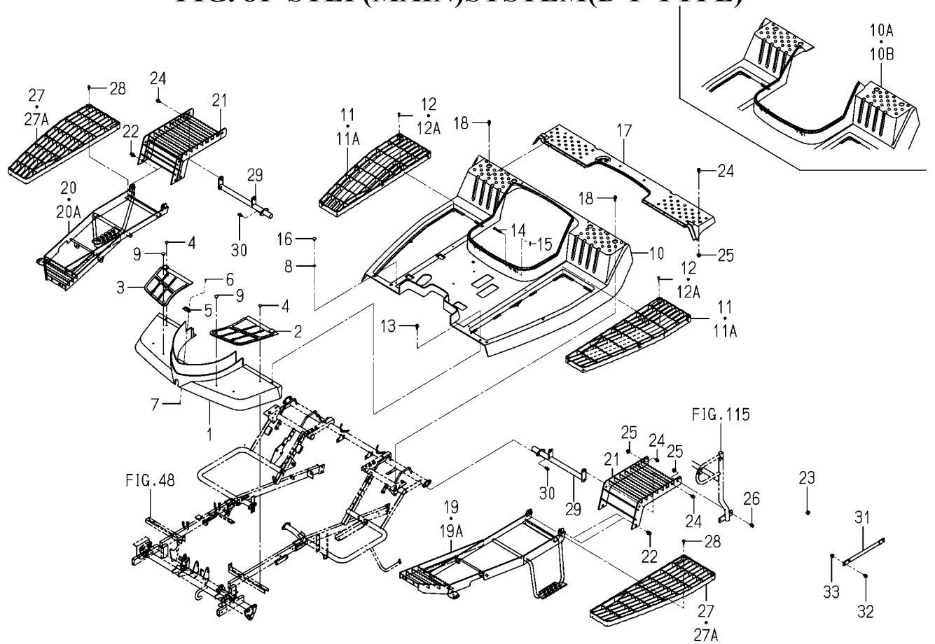
FIG. 81 STEP(MAIN)SYSTEM(D-F TYPE)
