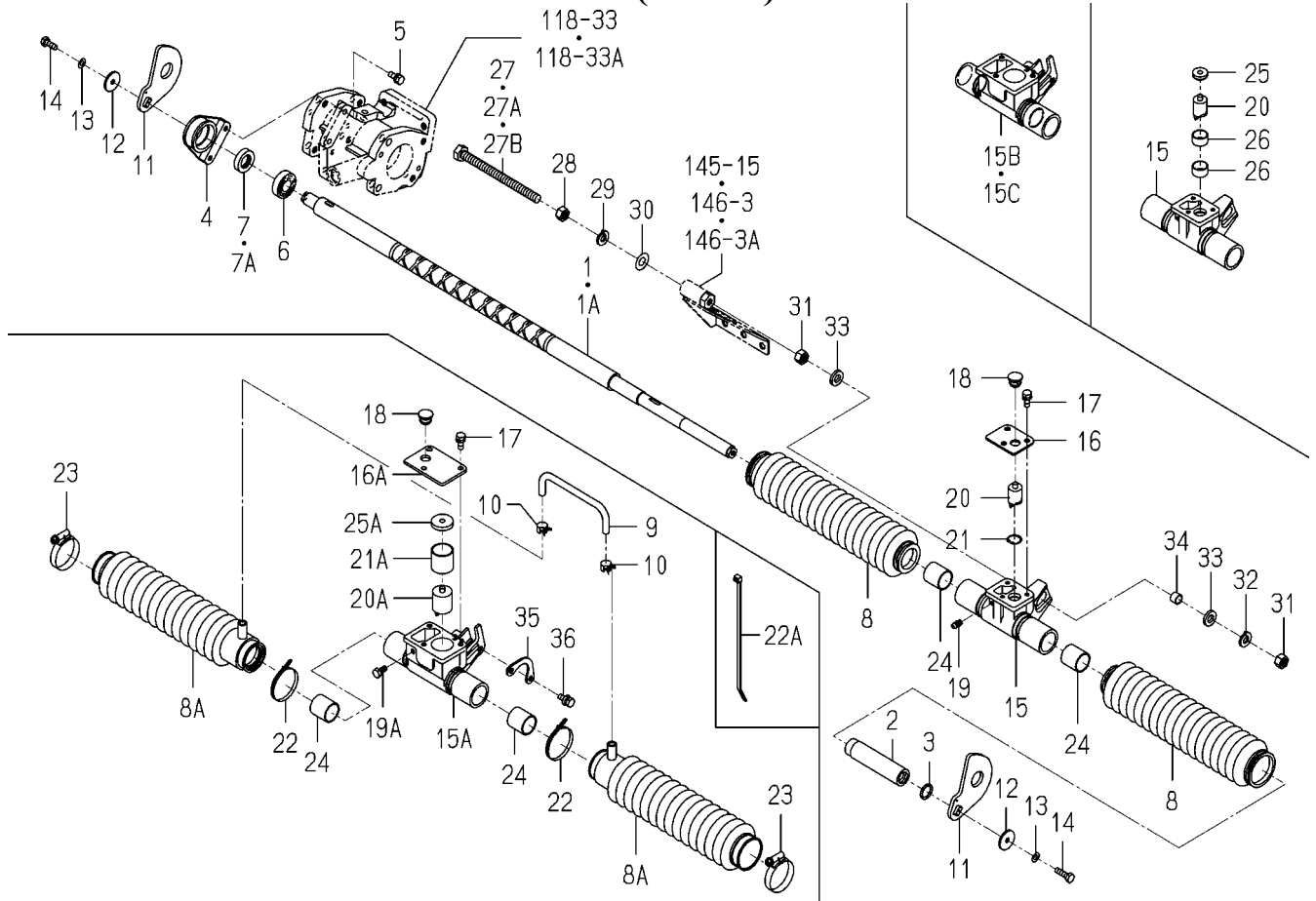
FIG.121 CAM(LEAD)SYSTEM
