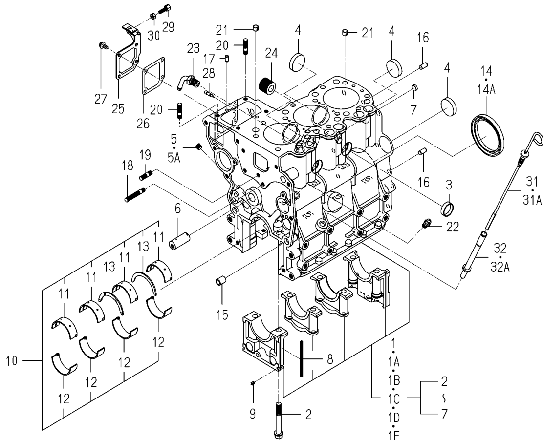
FIG. 5 CYLINDER BLOCK
