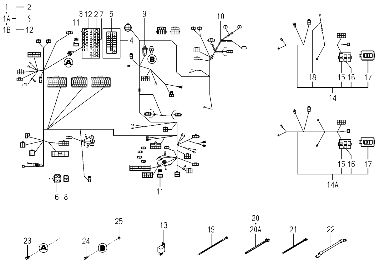
FIG.100 HARNESS (TRAVELING SECTION)SYSTEM(D TYPE EXCEPT F)
