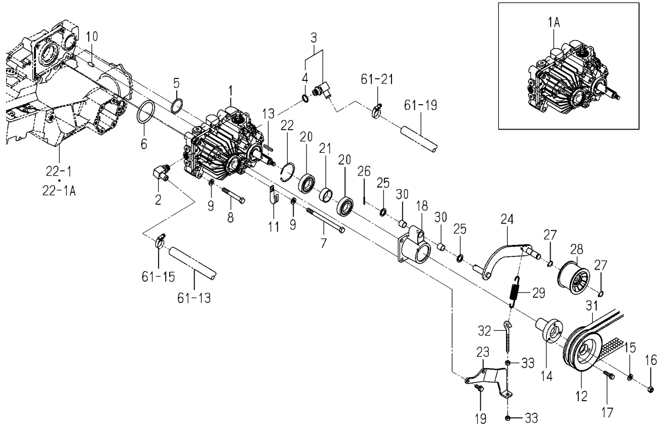
FIG. 15 HST SYSTEM(D TYPE)(NO.102350-)
