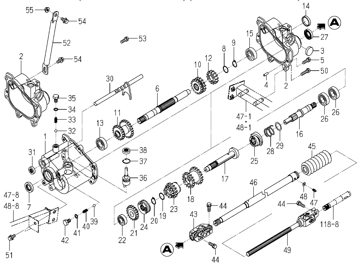
FIG. 68 CASE(PLANTING)SYSTEM (EXCEPT F TYPE)(NO.100001-101046)
