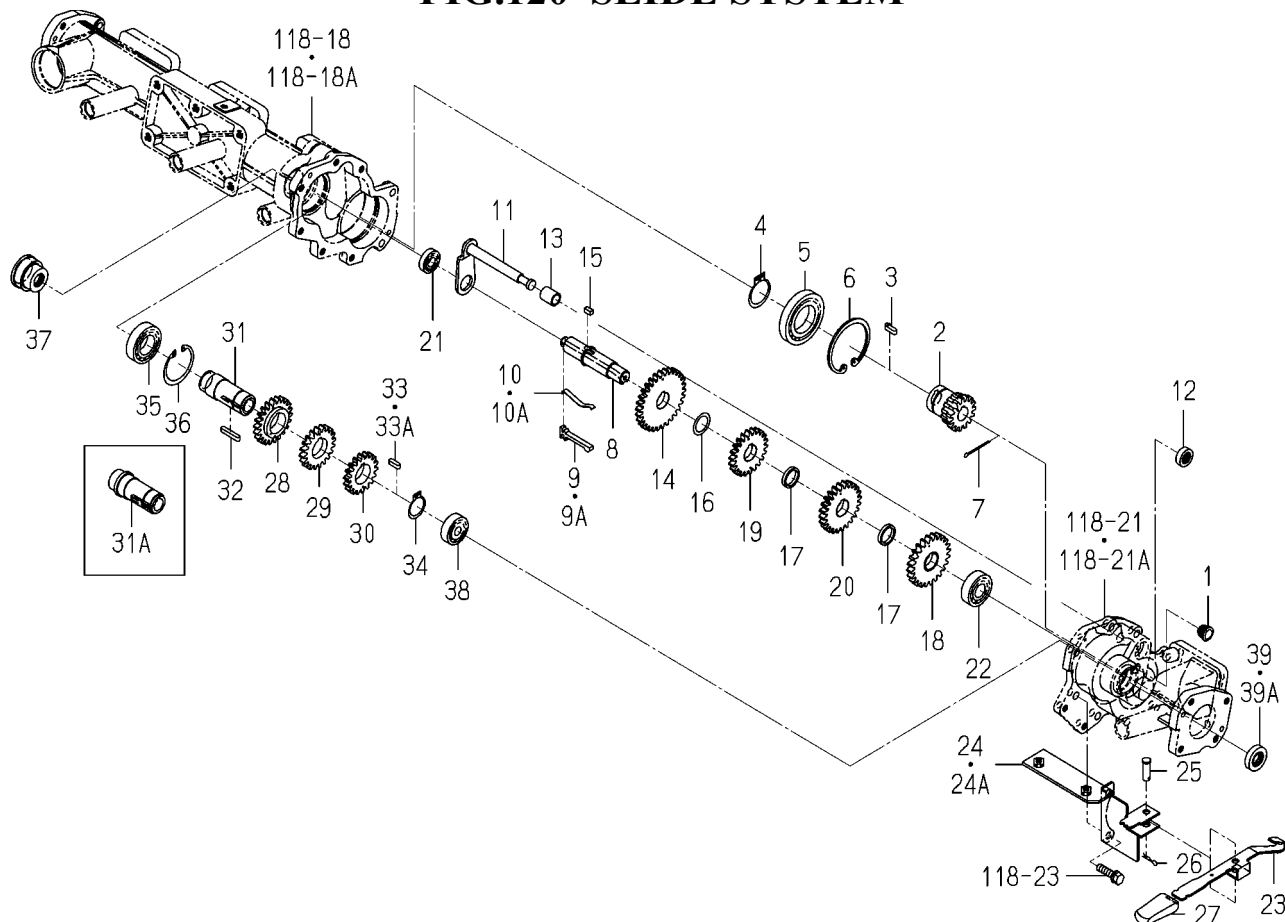
FIG.120 SLIDE SYSTEM
