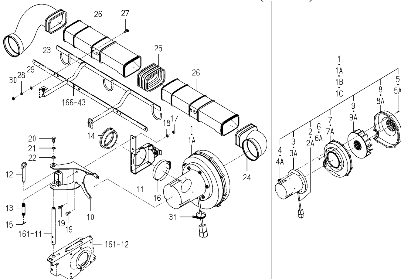
FIG.167 BLOWER SYSTEM(F TYPE)
