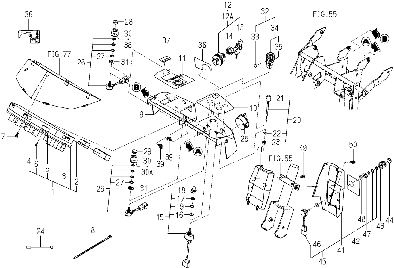
FIG. 97 PANEL(INSTRUMENT)SYSTEM(D TYPE)
