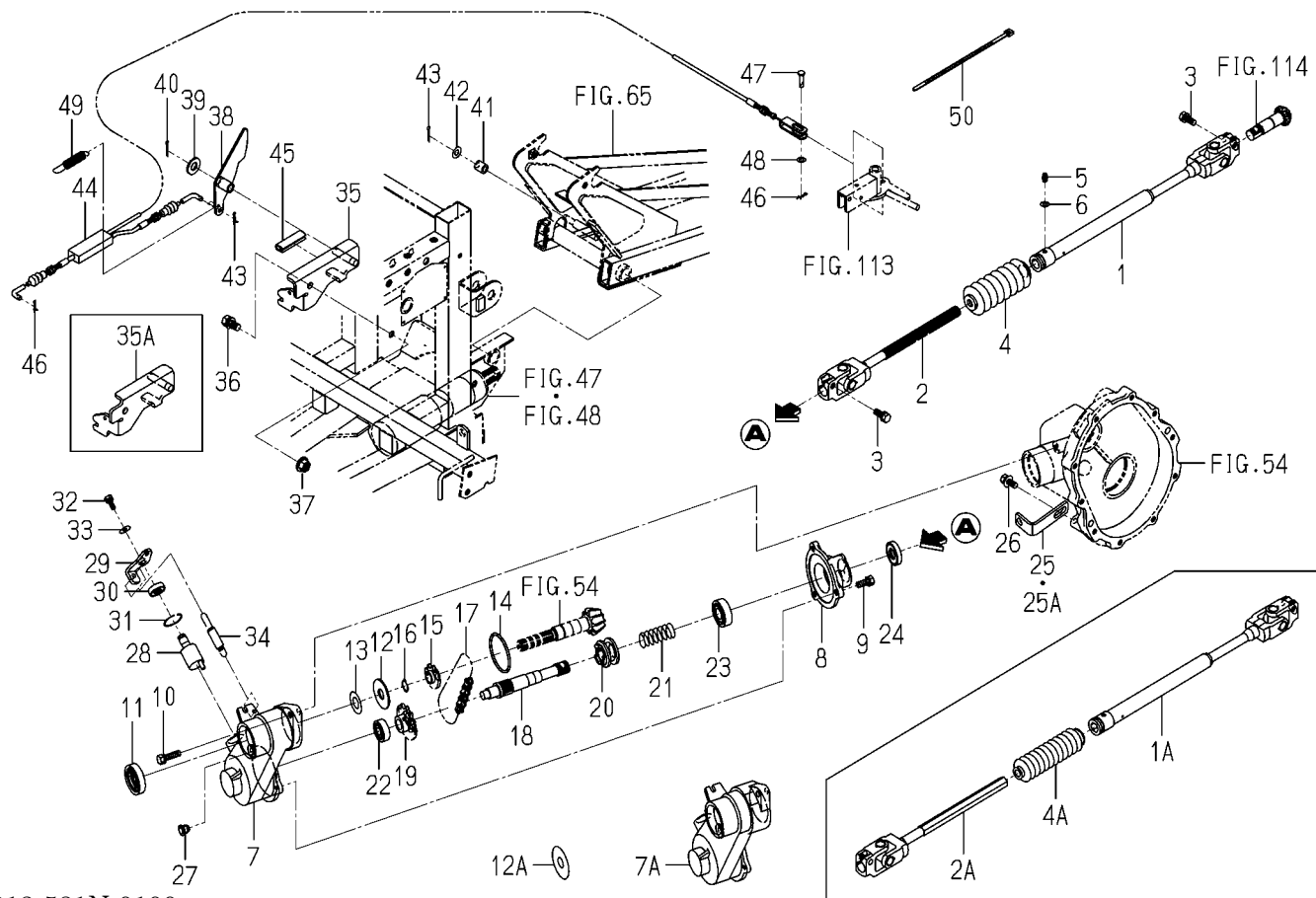
FIG.110 DRIVE(ROTOR)SYSTEM
