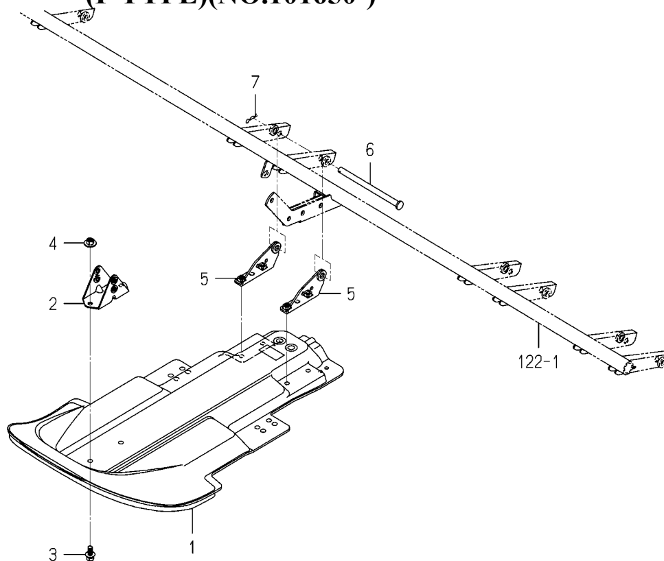
FIG.124 FLOAT(CENTER)SYSTEM (F TYPE)(NO.101650-)
