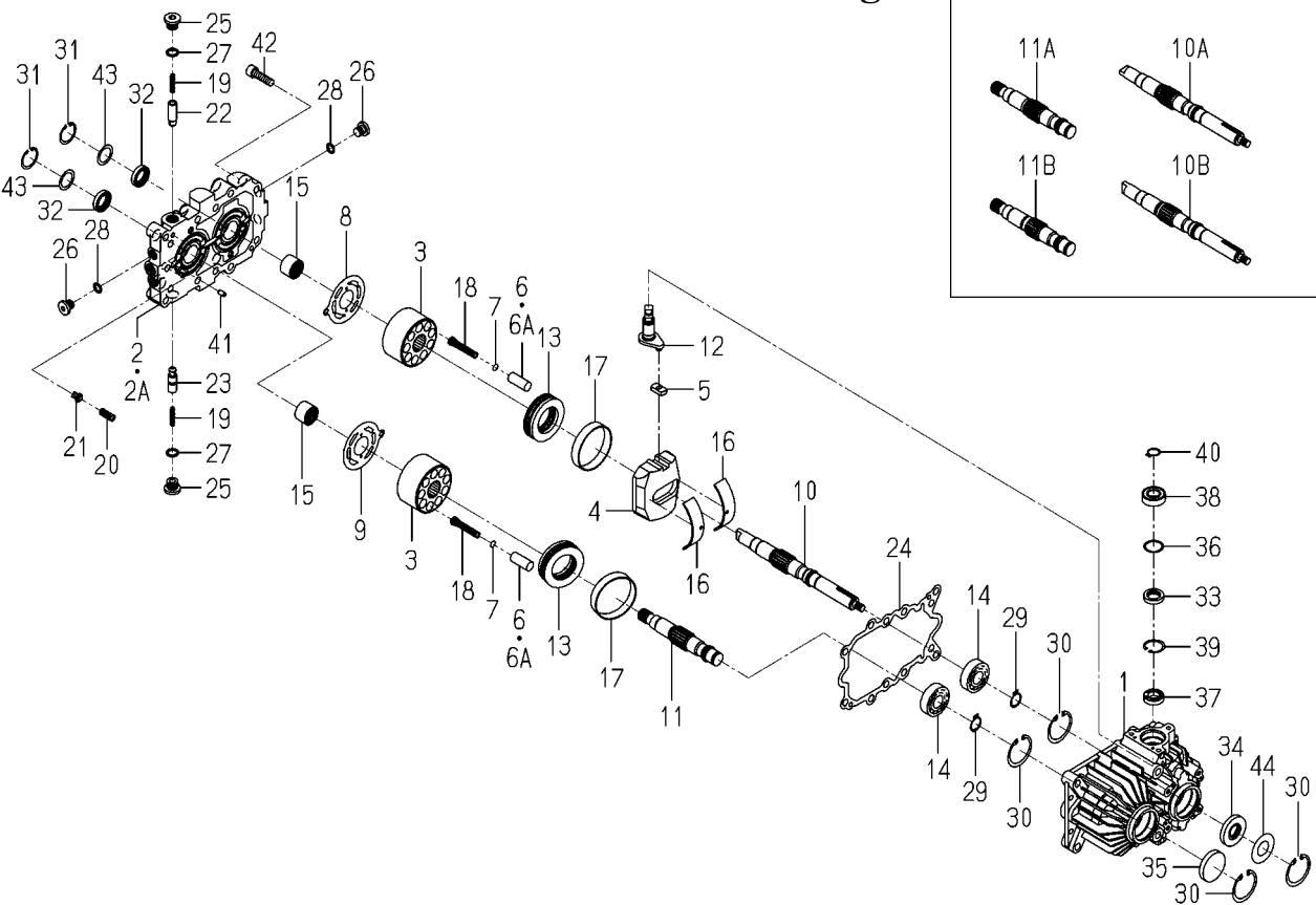
FIG.191 COMPONENT PARTS FOR K510-013-000-40 ON Fig.16□17
